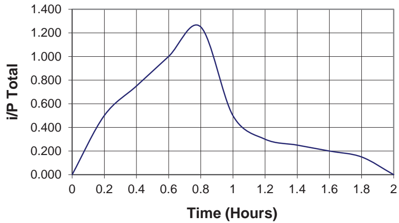
2 Hour Duration Intensity Curve
