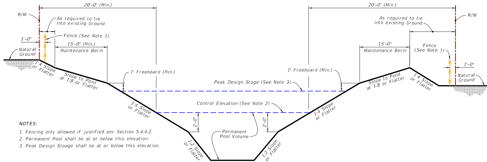
Figure 5-1: Minimum Clearance for Retention-Detention Ponds
