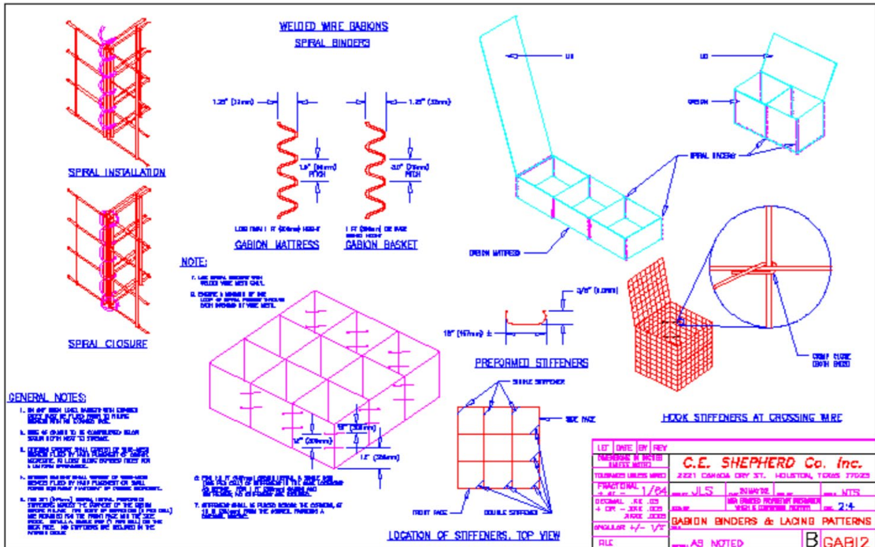
Figure 3.3-4: Gabion Binding
