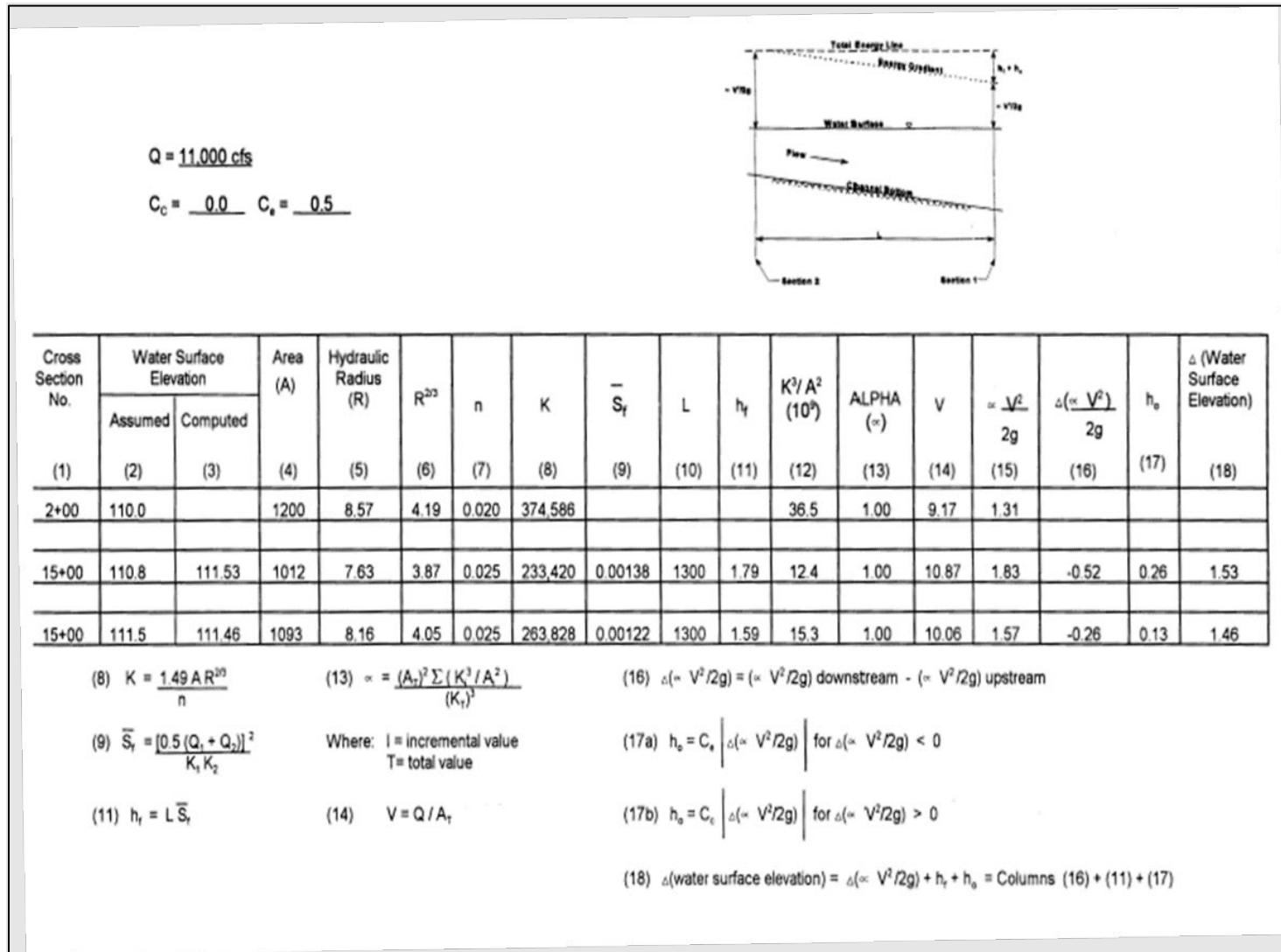
Example 5.2-4: Standard Step Backwater Computation (continued)
