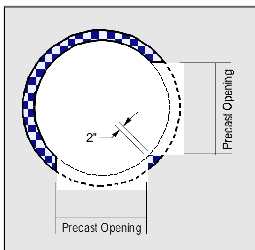
Figure 6.4-3: Adjacent Pipe Openings
