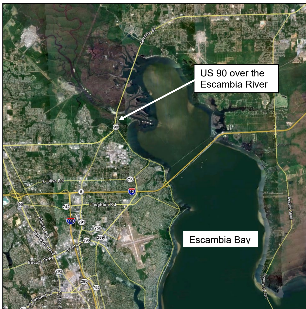
Figure 5.1-1: Example of a Bridge Requiring both Riverine and Tidal Analyses (US-90 over Escambia Bay)
