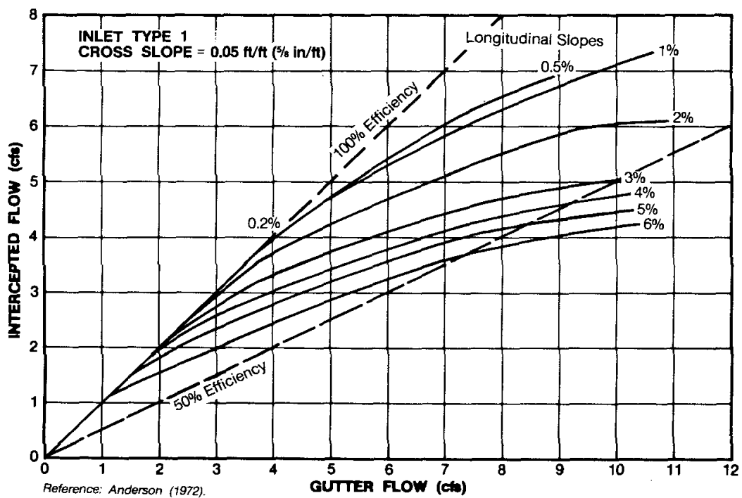
Figure I-4: Type 1, S_x = 0.05
