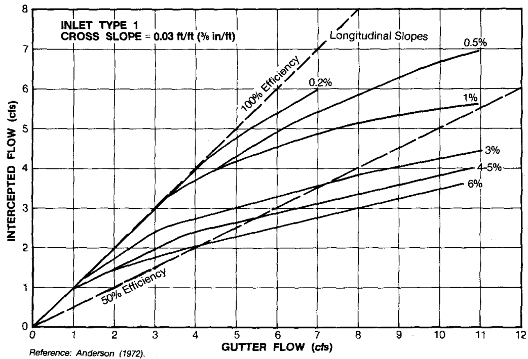
Figure I-2: Type 1, S_x = 0.03
