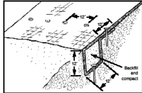
Figure 3.3-6: Initial Anchor
