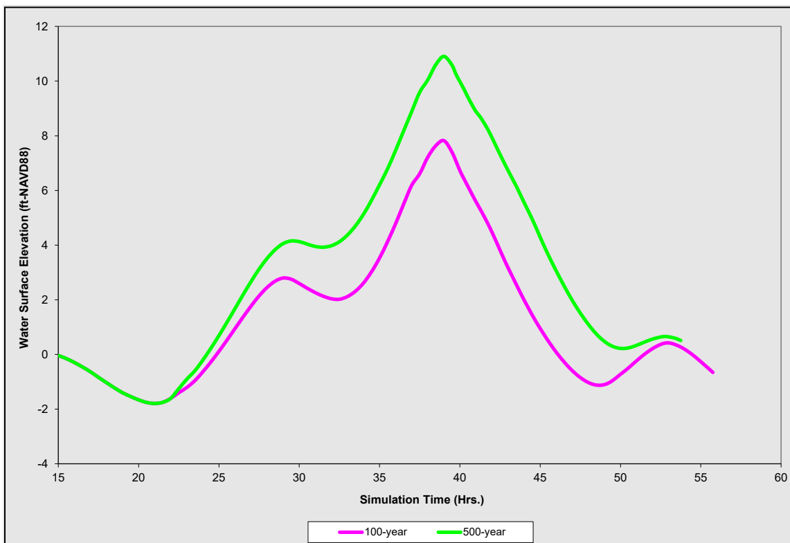
Figure 5.7-11: Water Surface Elevation Time Series during the Design and Check Event at the SR-A1A Bridge over the Loxahatchee River
