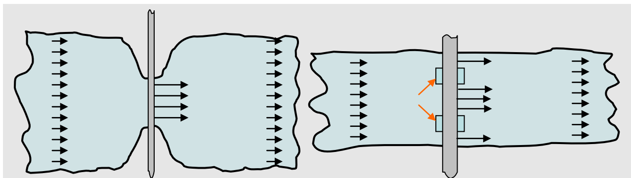
Figure 5.5-1: Examples of Contractions at Bridge Crossings
