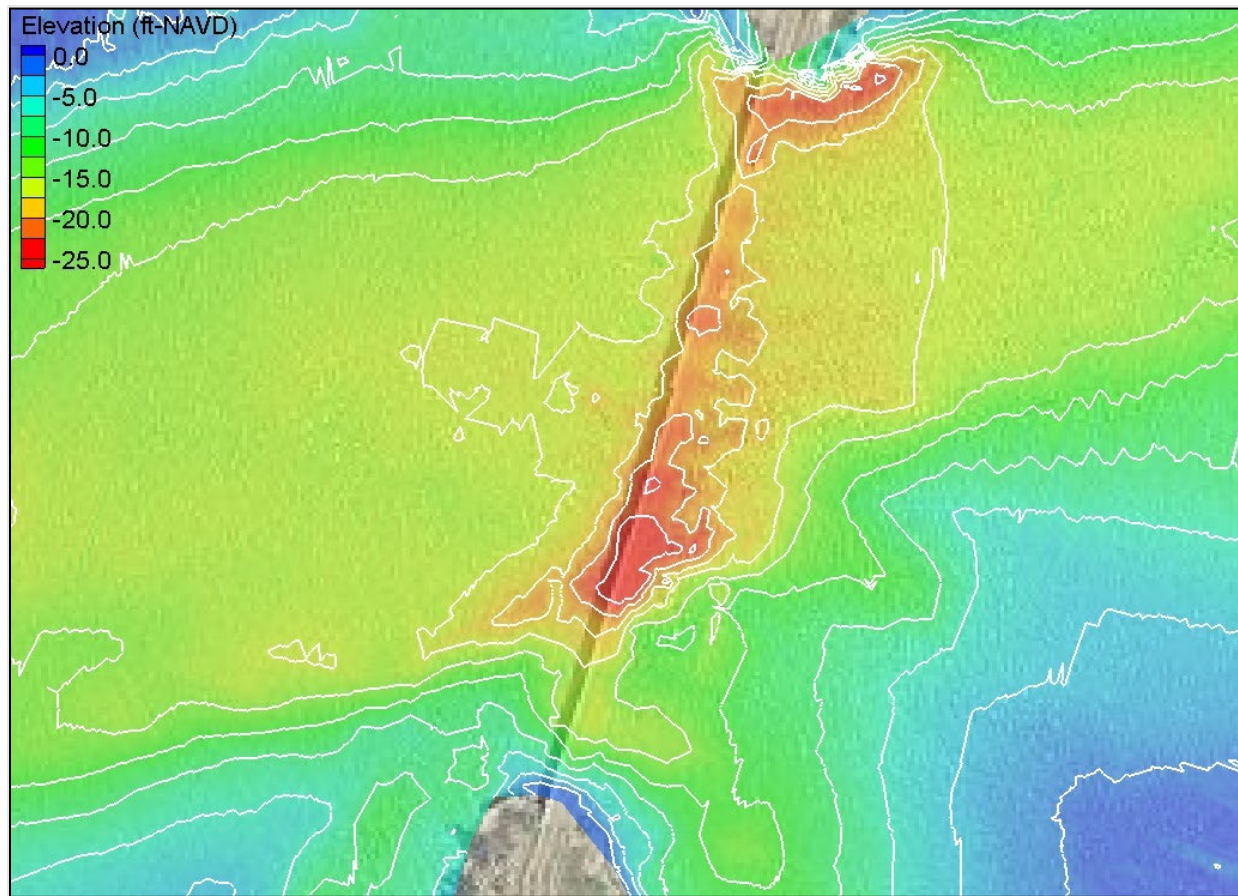
Figure 5.5-8: Example of Normal, Everyday Scour Holes from Survey Data
