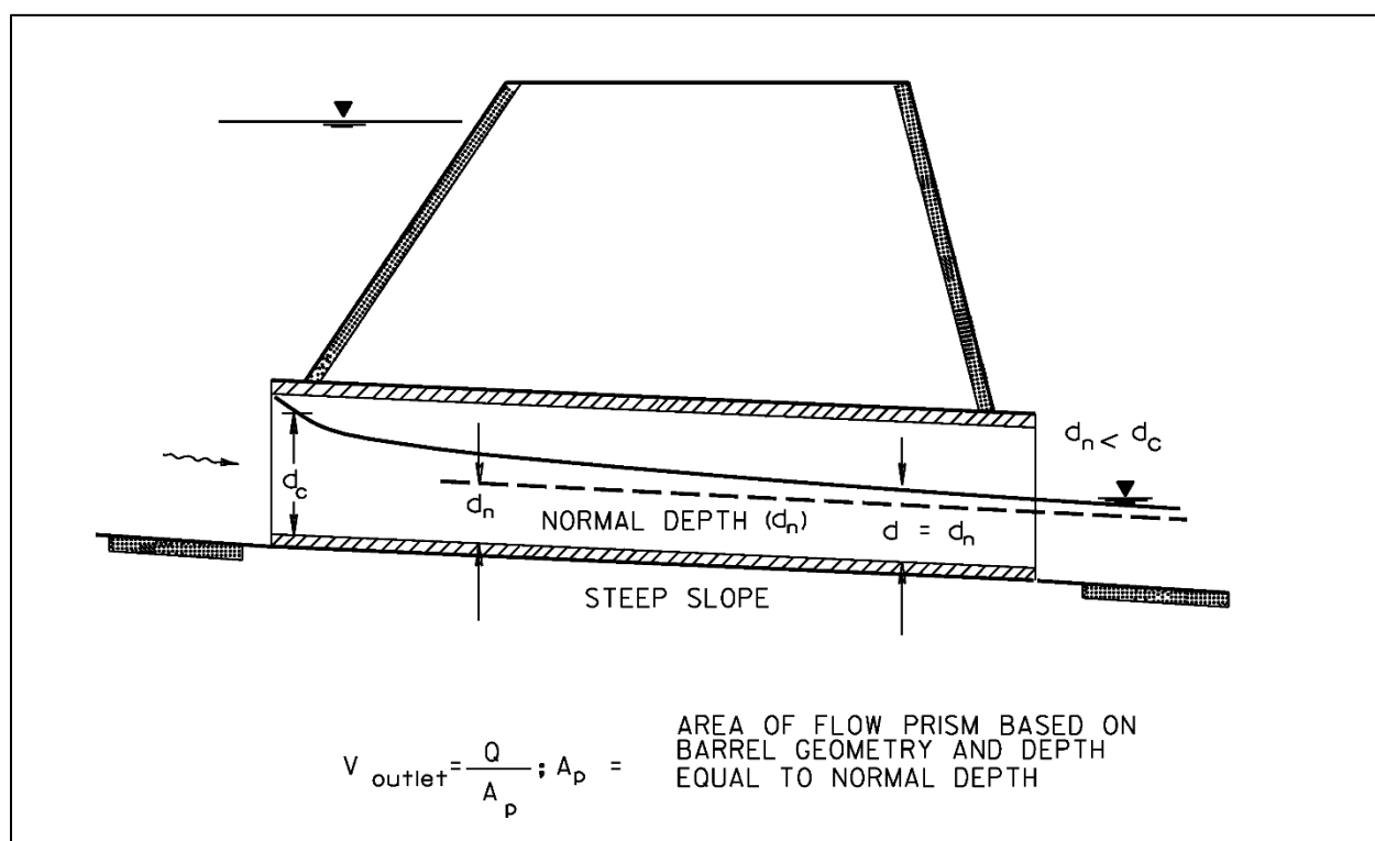
Figure 4.5-3: Outlet Velocity for Inlet Control
