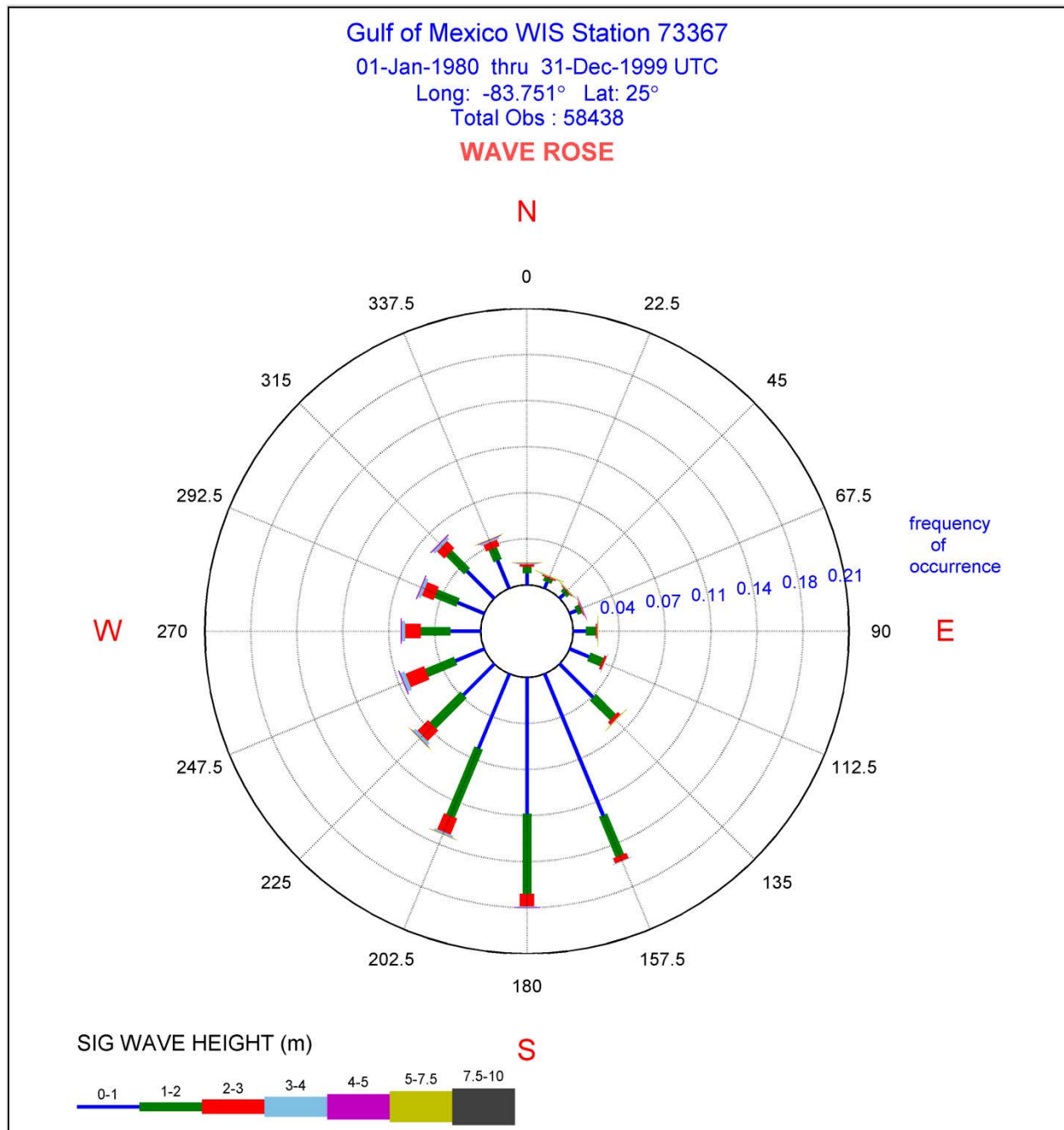
Figure 5.3-9: Example of Available WIS Data from: https://cirp.usace.army.mil/products/cms.php
