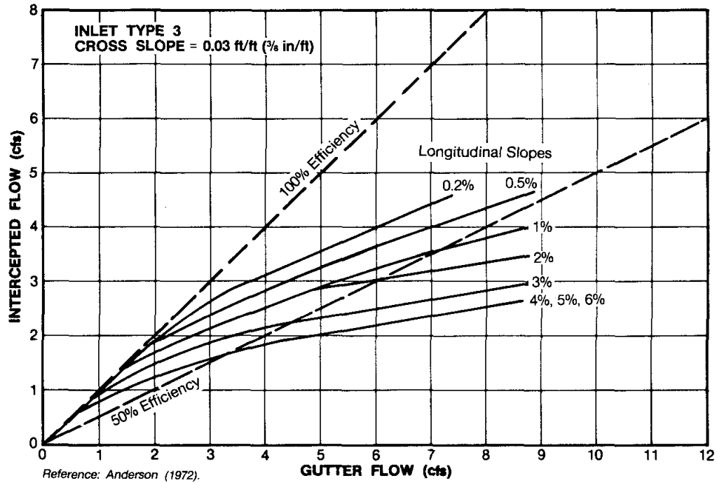
Figure I-7: Type 3, S_x = 0.03
