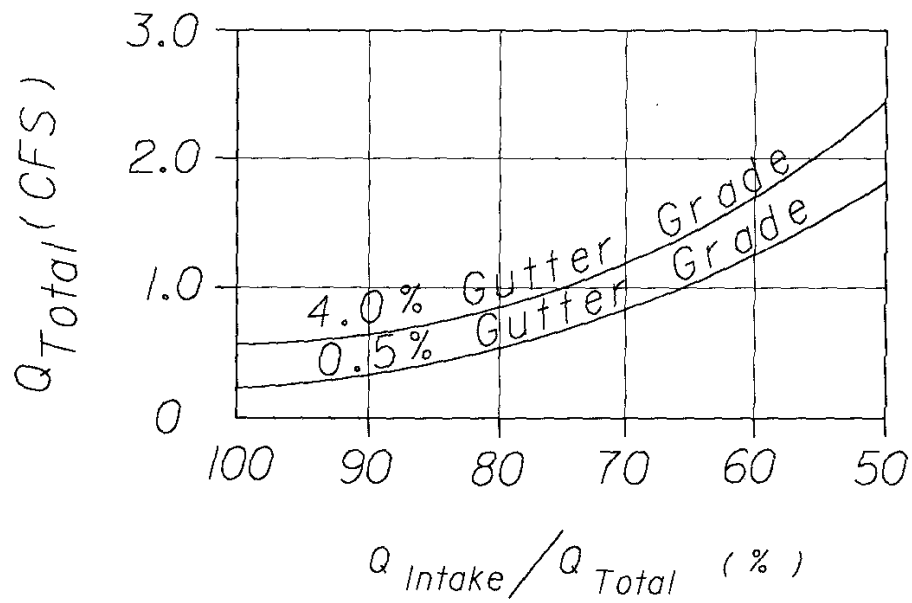
Figure I-21: Type 10 Inlet
