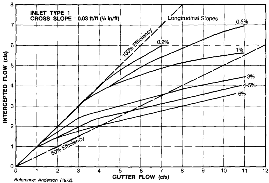
Figure I-2: Type 1, S_x = 0.03
