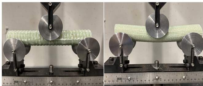
Horizontal shear test of No. 11 GFRP Bars from two different manufacturers.
