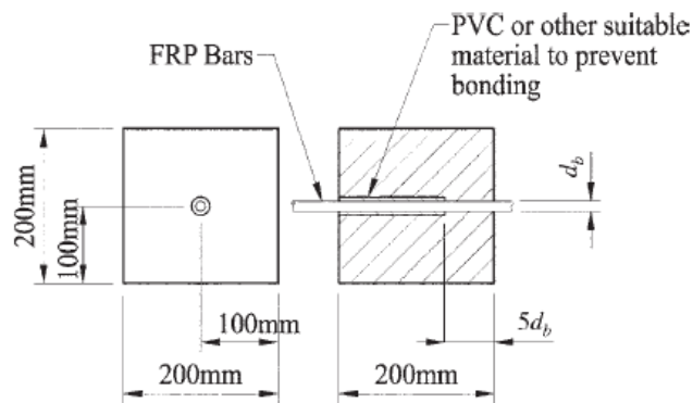
Figure 38. Concrete pullout bond specimen layout
