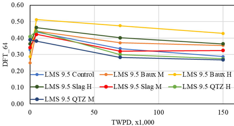
Figure 27: DFT Results – LMS FC-9.5 Mixes
