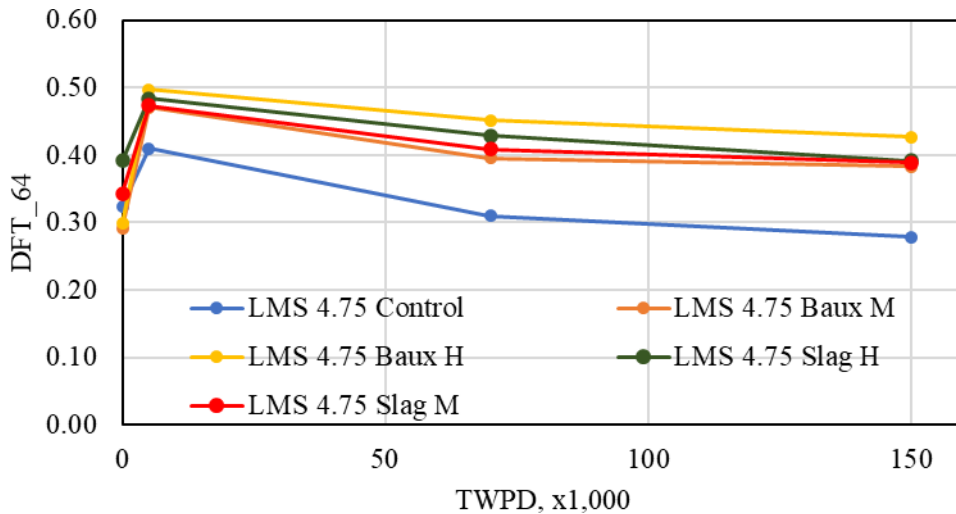
Figure 25: DFT Results – LMS FC-4.75 Mixes
