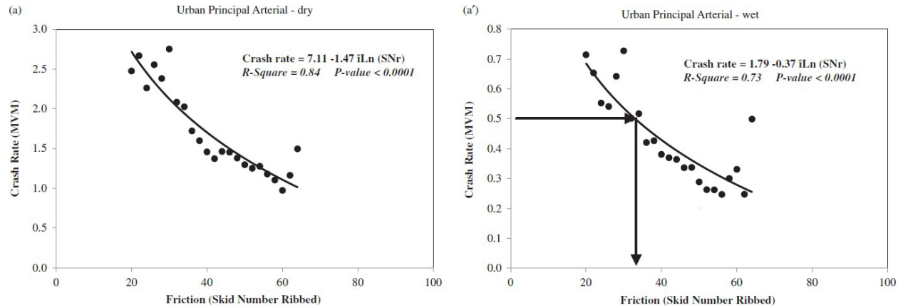
Figure 10: Example of Crash Rate vs. Friction from New Jersey (Najafi et al., 2017)
