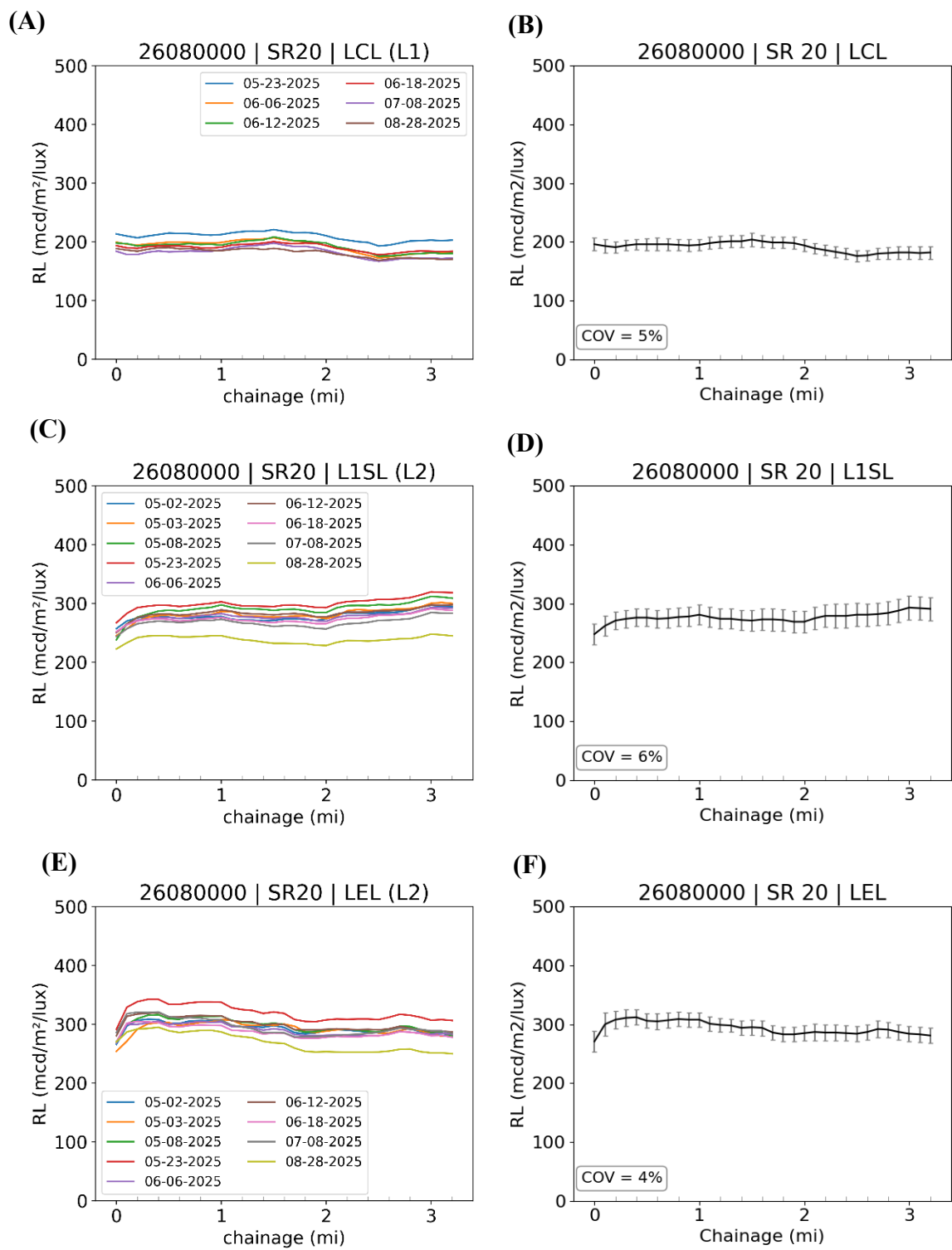
Figure 4.8 R_L statistics for SR-20 westbound lanes (3-mi section): 1-mi moving average, mean, COV, and standard deviation. Lanes include (A–B) LCL, (C–D) L1SL, and (E–F) LEL on Road ID 26080000.
