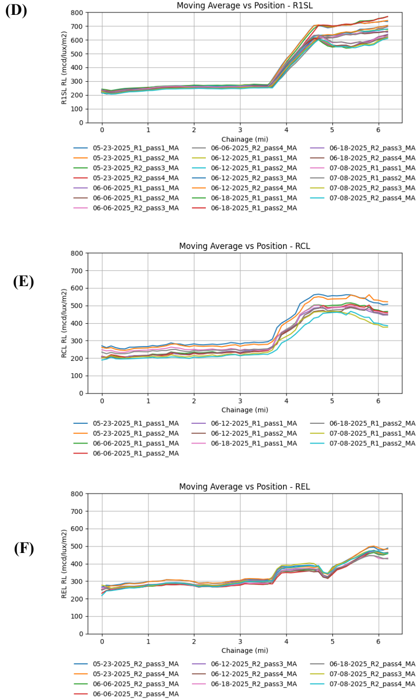
Figure C.1 (a-f). 1-mi moving average of R_L was measured across the entire lane in a single pass for each run on the 6-mi SR-20 test section, including both eastbound and westbound directions.
