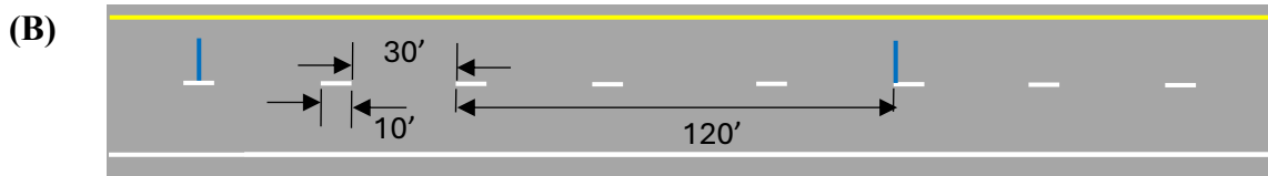
Typical handheld measurements at the skip lines (120 ft / 0.0227 mi between handheld measurements)
