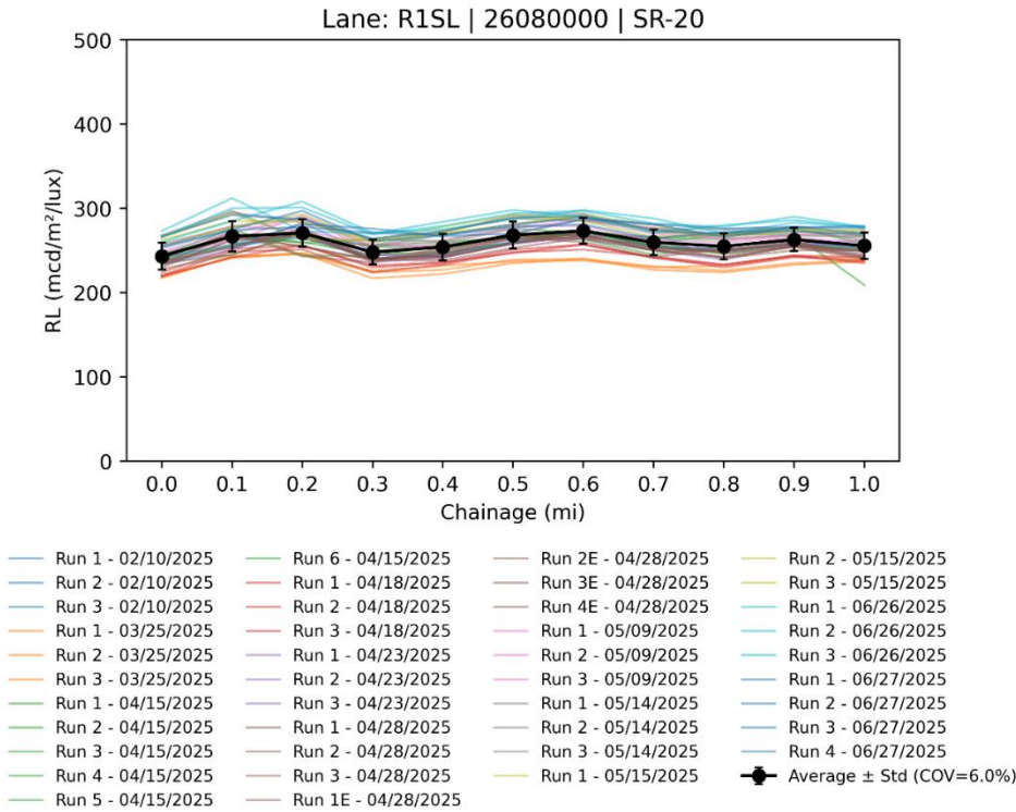
Figure 4.6 R_L measurements on 1-mi section on SR-20 eastbound for skip line (R1SL)
