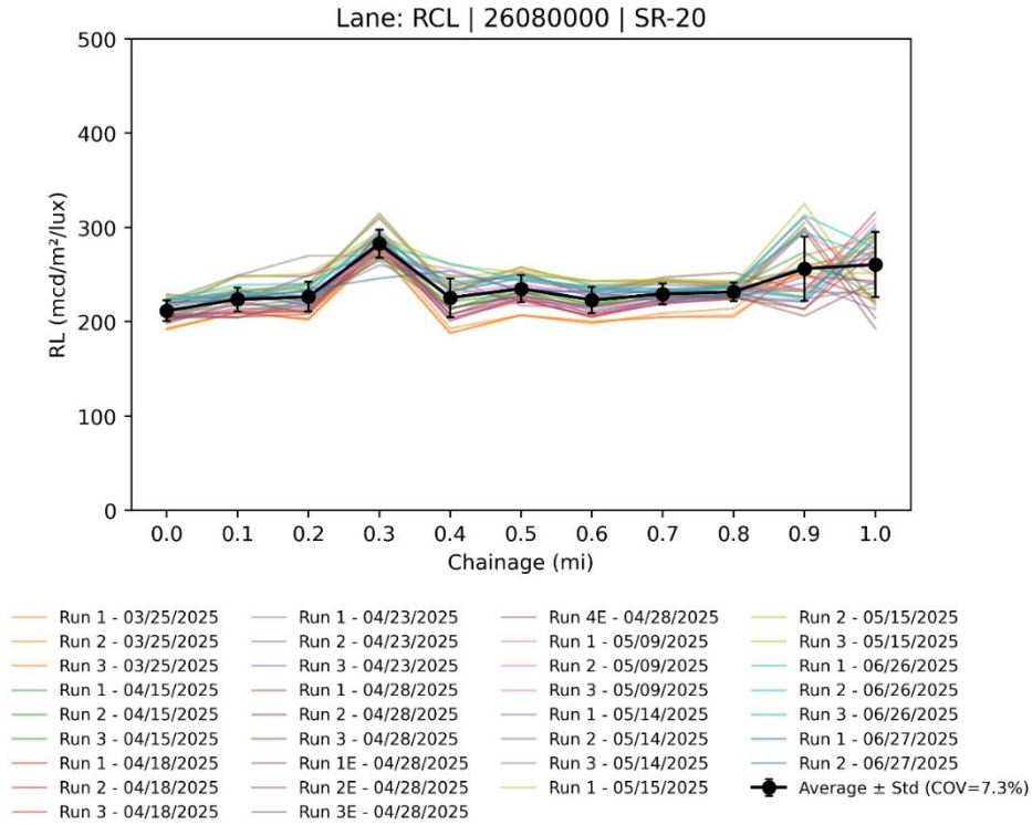
Figure 4.5 R_L measurements on 1-mi section on SR-20 eastbound for centerline (RCL)
