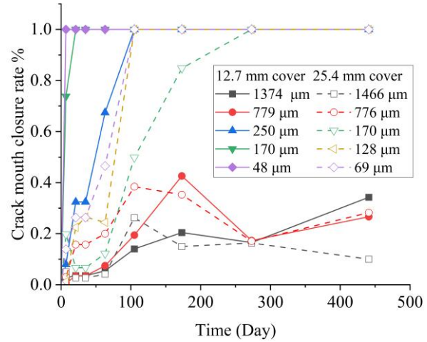
Figure 6-5 Self-healing behavior of Mixture B
