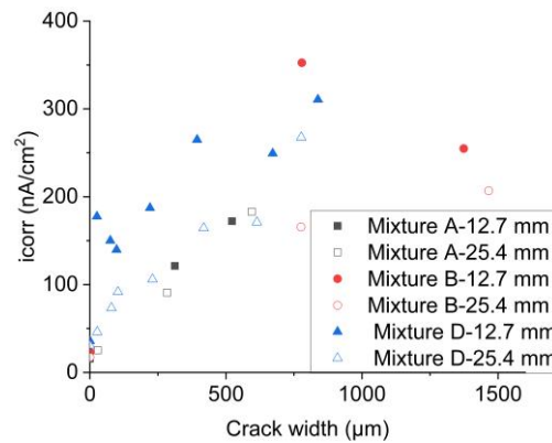
Figure 6-12 Relationship between i_{\text{corr}} and crack width for cracked reinforced UHPC specimen
