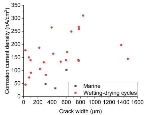
Figure 6-19 i_{\text{corr}} for specimens exposed to indoor wetting-drying cycles and realistic marine environment
