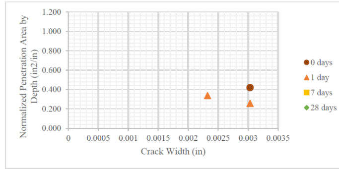
Figure 5-16 Penetration area normalized by penetration depth as a function of crack width for crack widths between 0.00197 in. and 0.00384 in. (50 and 100 \mu m)
