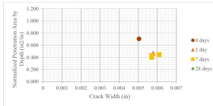
Figure 5-17 Penetration area normalized by penetration depth as a function of crack width for crack widths between 0.00384 and 0.00787 in. (100 and 200 \mu m)
