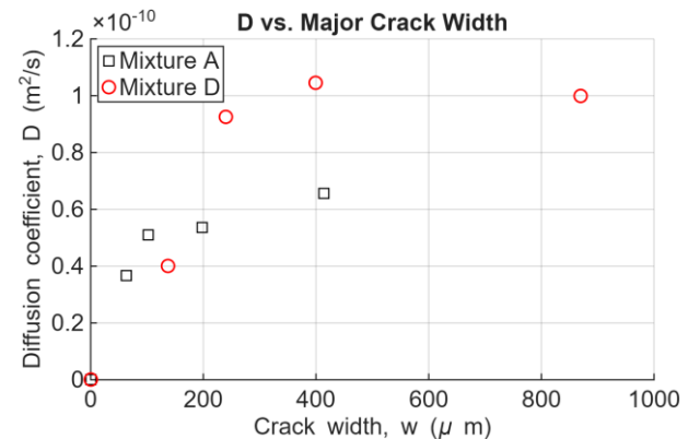
Figure 5-33 Chloride diffusion coefficient vs. crack width
