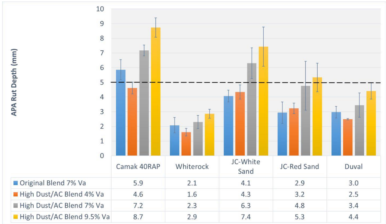
Figure 19. Summary of APA Results – Laboratory Rutting Evaluation
