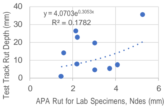
(c) APA for Specimens @ N des vs TT Rutting
