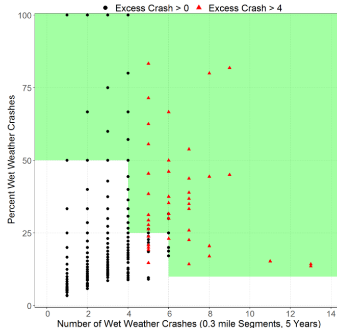
Figure 66. Percent Wet Weather vs. Total Wet Weather Crashes with Recommended Criteria (Excess Crash greater than 4 shown in Red Triangles)
