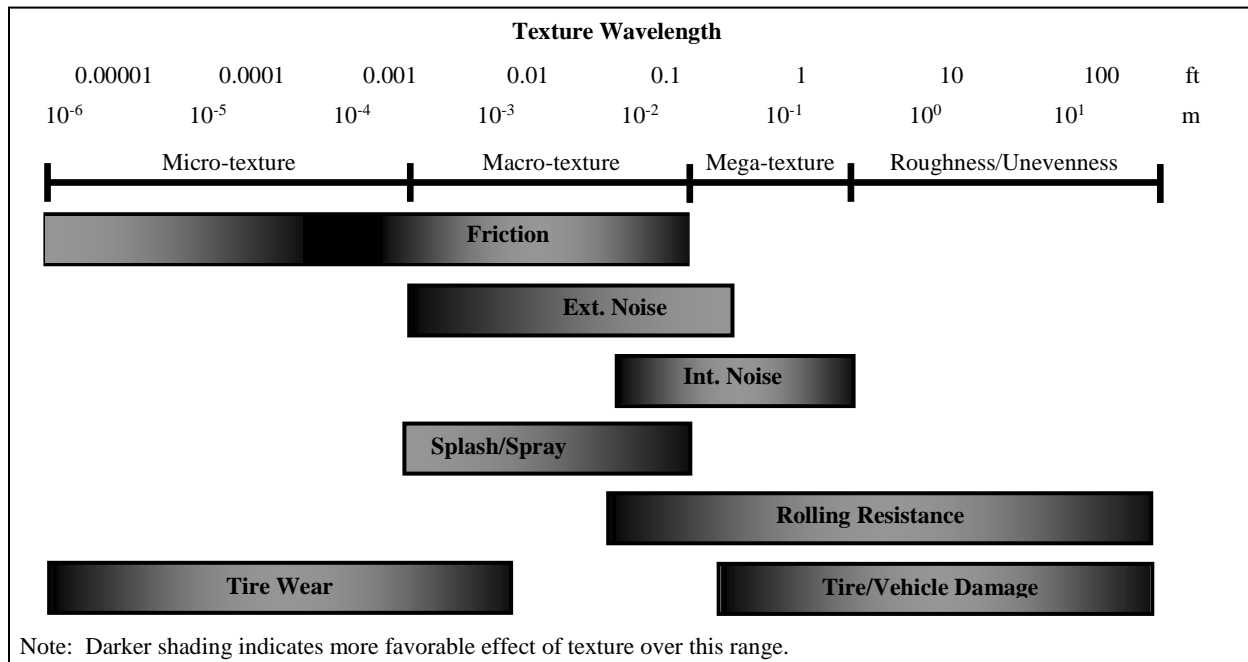
Figure 5. Texture wavelength influence on pavement-tire interactions (adapted from Henry, 2000).
