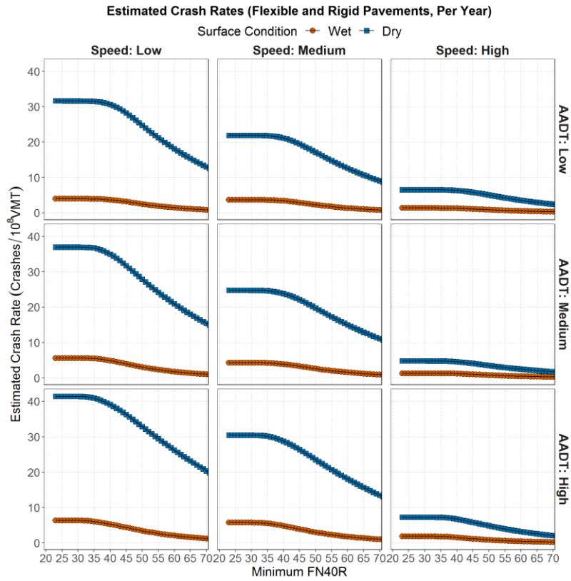
Figure 51. Estimated Crash Rates with Increasing FN40R Threshold
