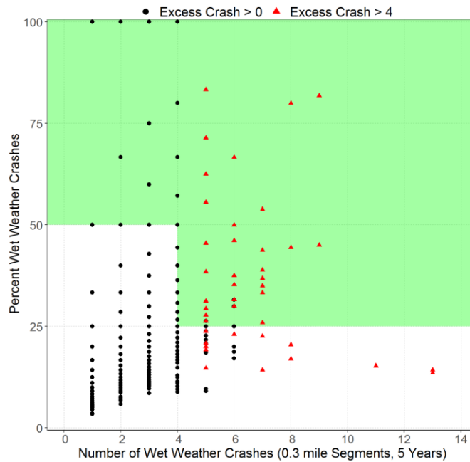
Figure 65. Percent Wet Weather vs. Total Wet Weather Crashes with FDOT's Existing Criteria (Excess Crash greater than 4 shown in Red Triangles)
