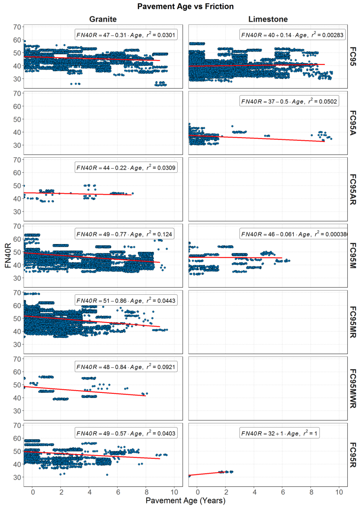
Figure 31. FN40R vs. Pavement age for FC95 mix family
