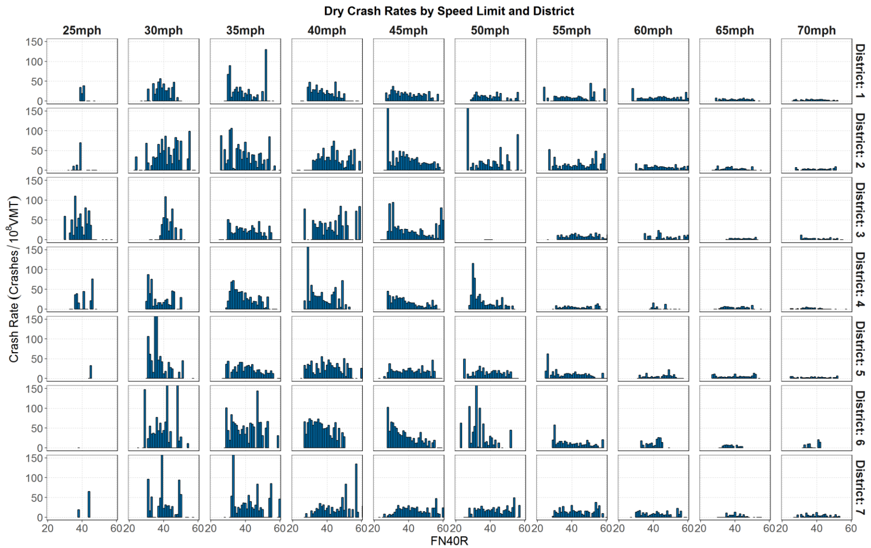
Figure 37. Dry Weather Crash Rate Distribution by Speed Limit and District (2011 – 2017)
