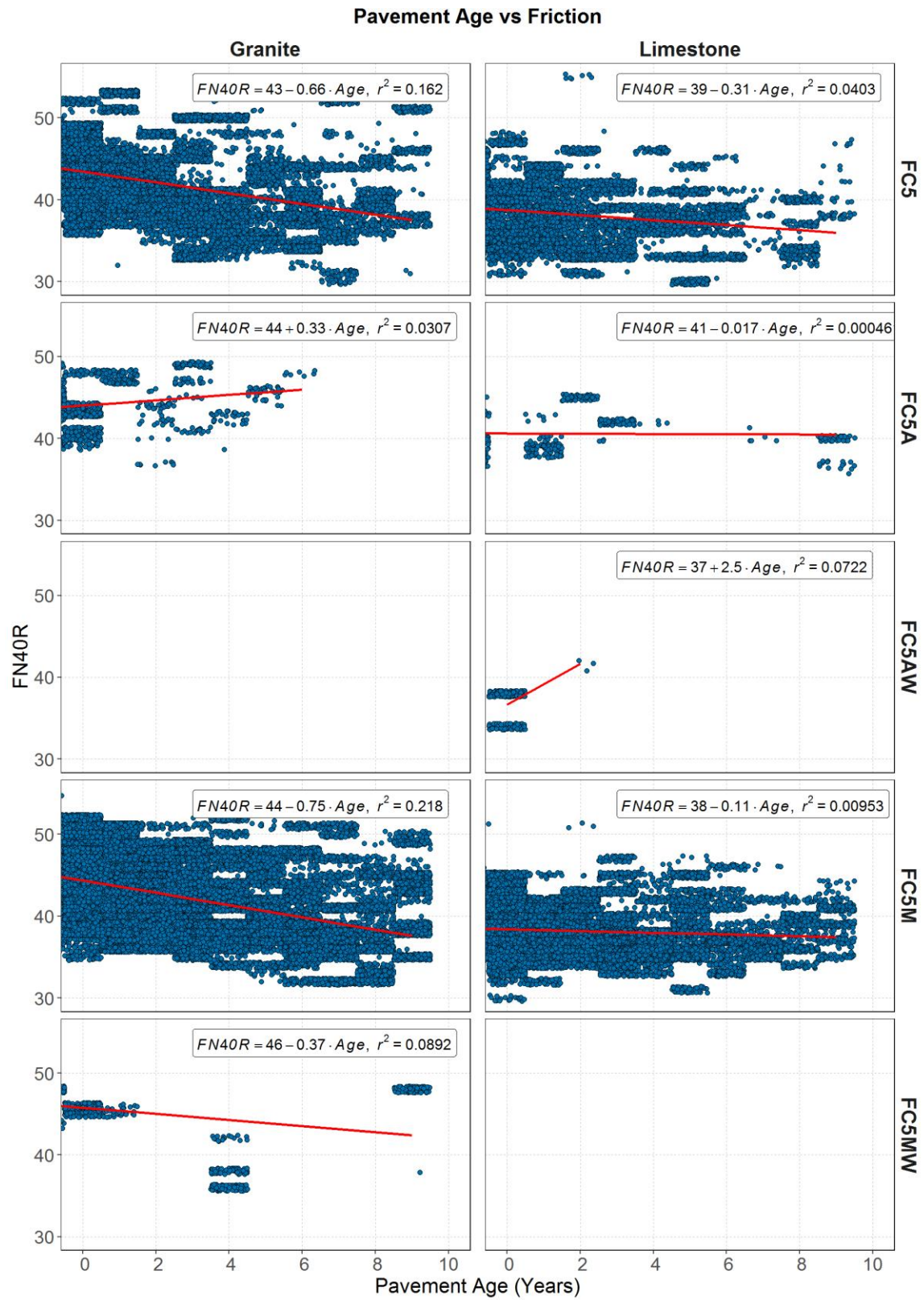
Figure 32. FN40R vs. Pavement age for FC5 mix family
