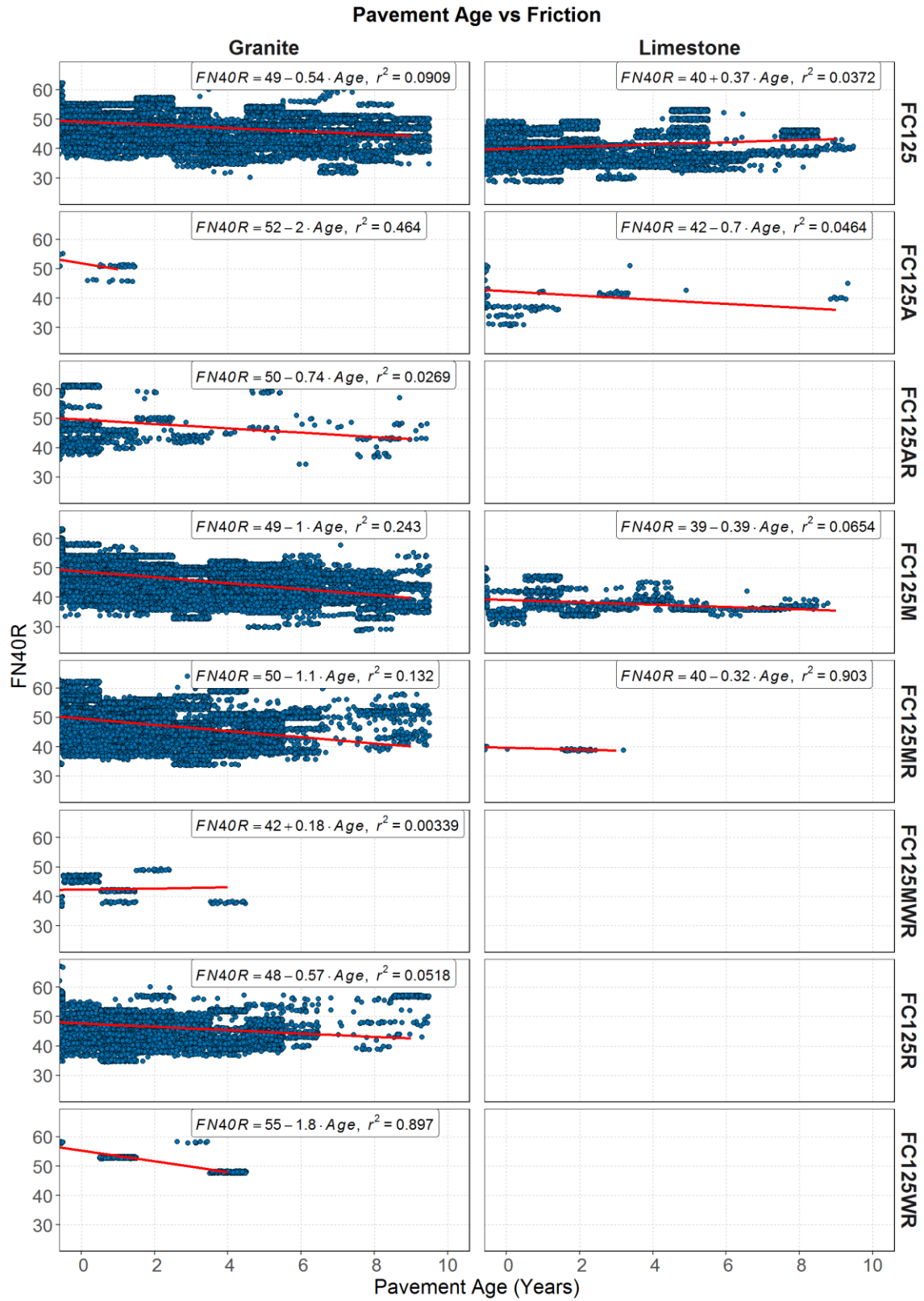
Figure 30. FN40R vs. Pavement age for FC125 mix family
