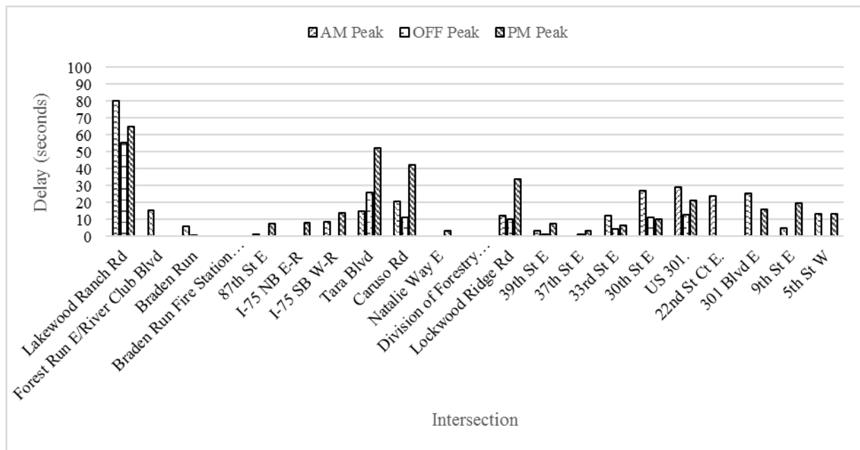
Figure G-3.5 Delay (s) for each intersection through movement along the WB direction – before study
