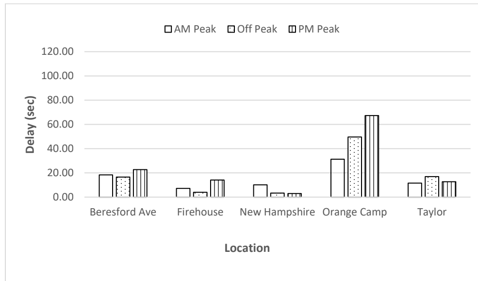
Figure B-3.4 Delay (sec) for each intersection through movement along the NB direction
