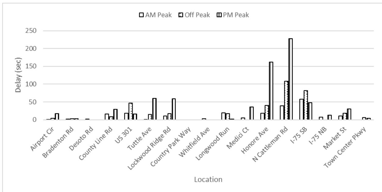
Figure D-3.4 Delay (sec) for each intersection through movement along the EB direction - after Table D-3.7 Delay (sec) for Each Intersection Through Movement along the WB Direction - after
