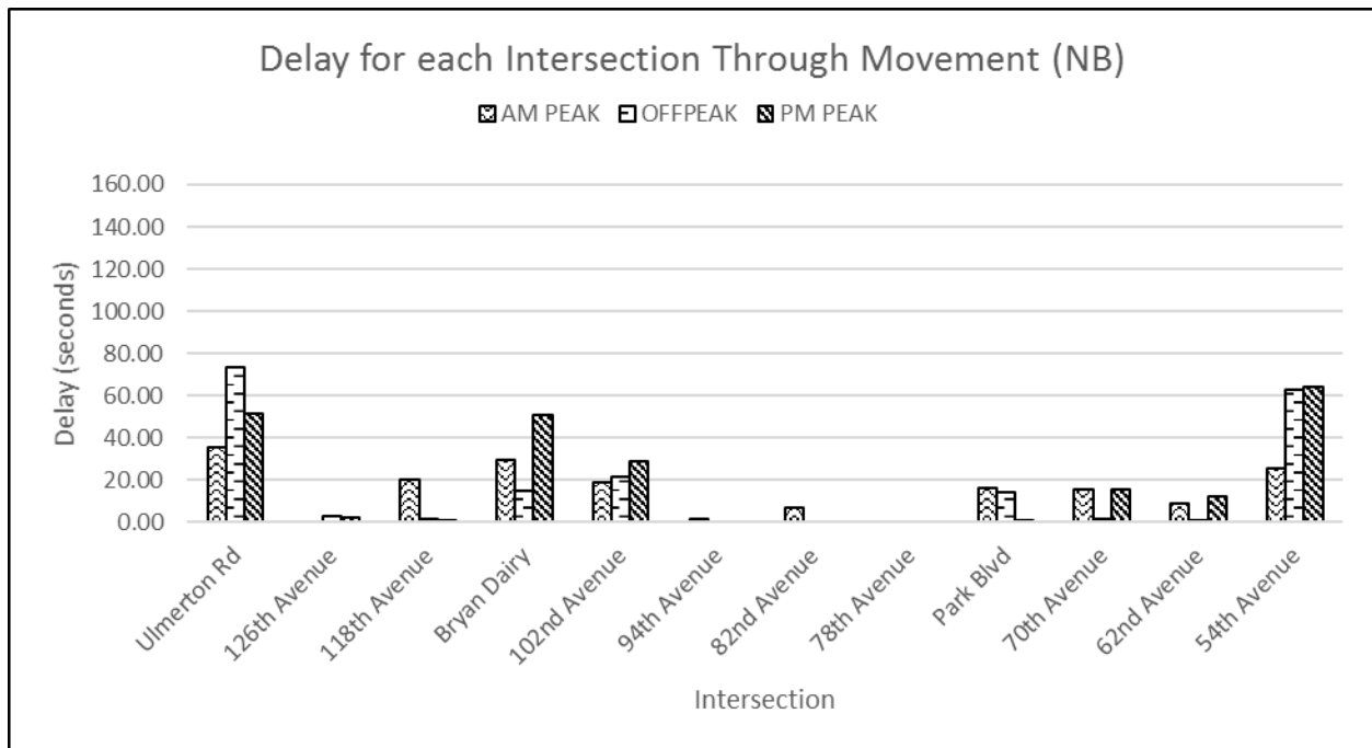
Figure F-3.5 Delay (sec) for each intersection through movement along the NB direction – after study
