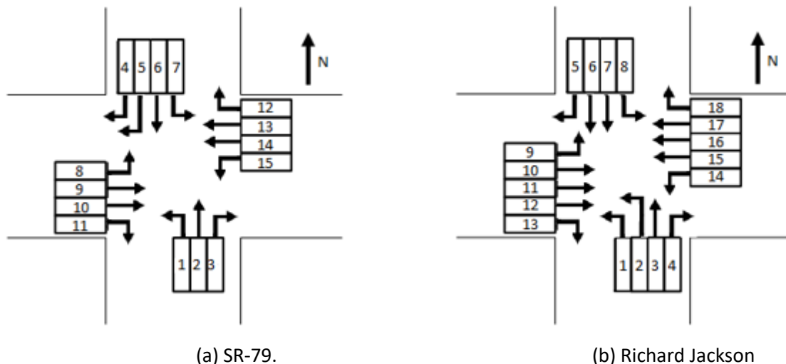
Figure C-3.9 Lane configuration of critical intersections
