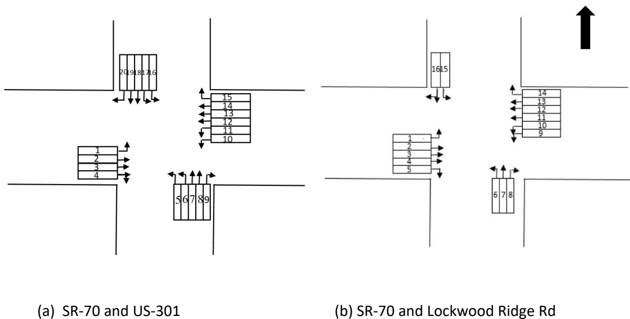
Figure G-3.12 Lane configuration of critical intersections
