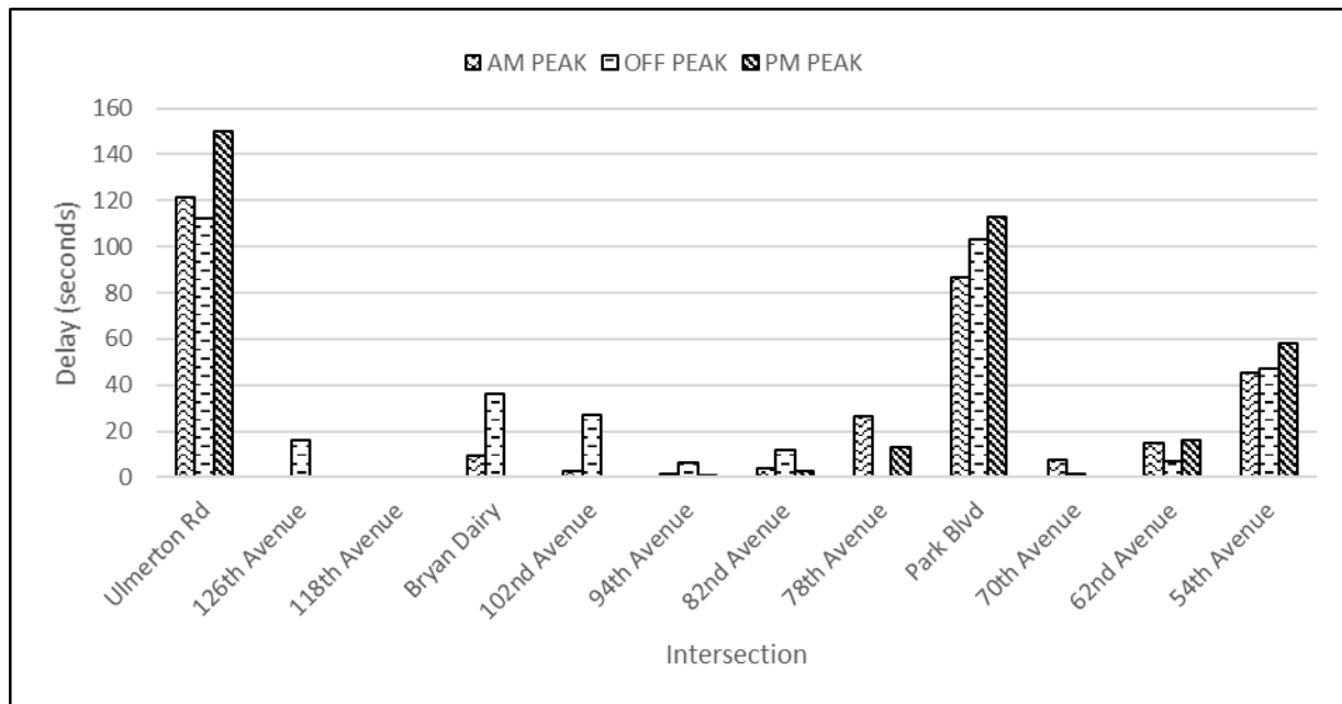
Figure F-3.2 Delay (s) for each intersection through movement along the SB direction-before study Table F-3.4 and Figure F-3.5 show the delays obtained by intersection for the NB. Figure F-3.3 shows the delay at each intersection for the through movement in the NB direction. The intersection delay in the NB direction is highest at Park Blvd during all study time periods (AM Peak, Off Peak and PM Peak). Delay at Ulmerton Rd is highest during the PM Peak period. The Off-Peak delays are higher than the PM Peak delays at six different intersections.
