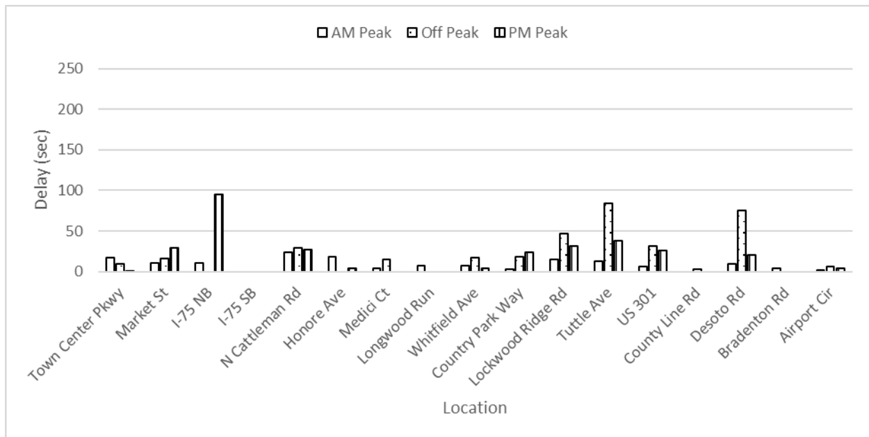
Figure D-3.5 Delay (sec) for each intersection through movement along the WB direction - after
