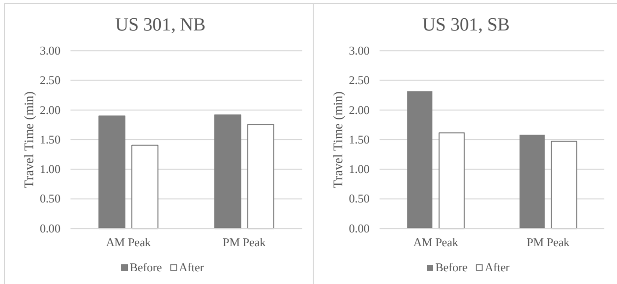
Figure G-3.3 Travel times along US-301
