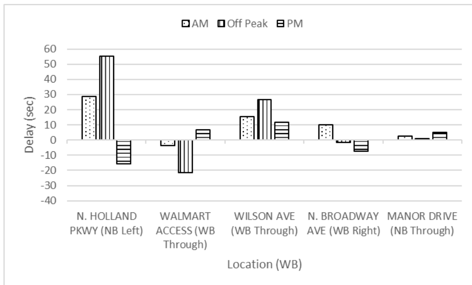
Figure H-3.7 Difference in delay (sec) for each intersection movement along the WB direction
