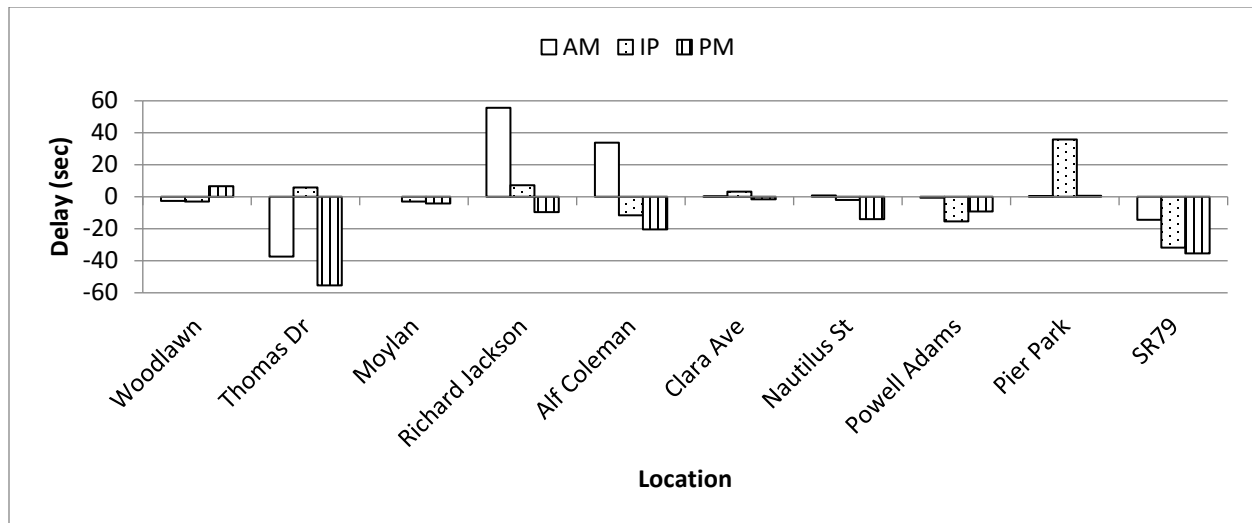
Figure C-3.7 Difference in delay (sec) for each intersection through movement along the WB direction
