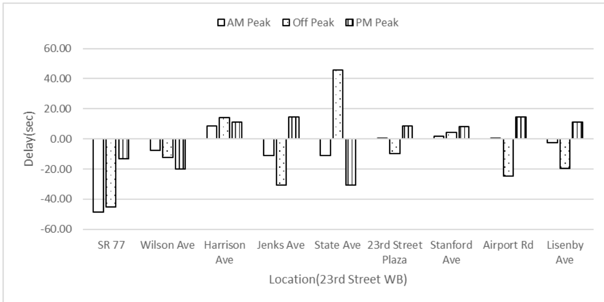
Figure E-3.8 Difference in delay (sec) for each intersection through movement along the WB direction
