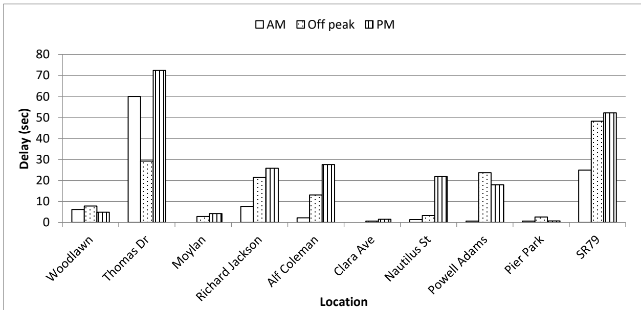
Figure C-3.3 Delay (sec) for each intersection through movement along the WB direction
