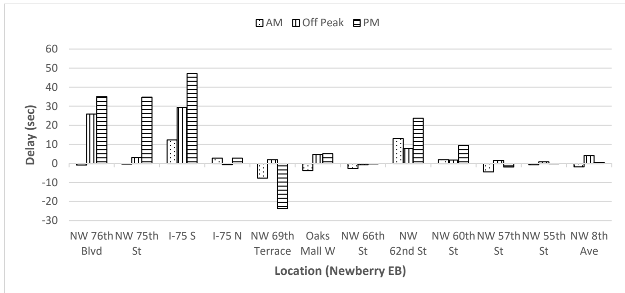
Figure A-3.6 Difference in delay (sec) for each intersection through movement along the EB direction
