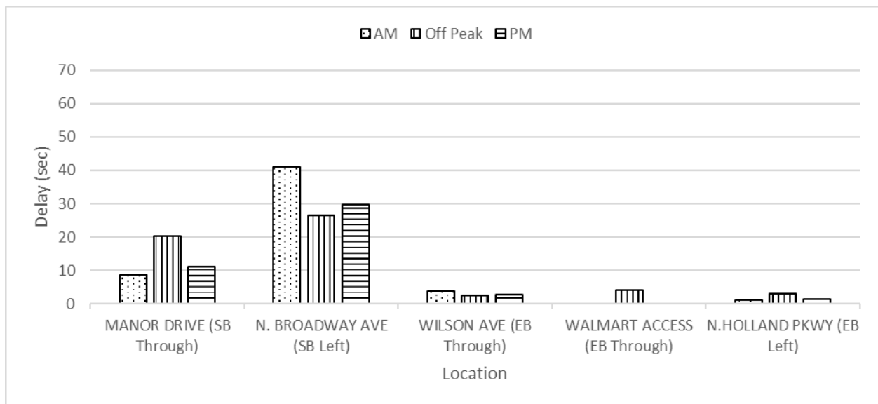
Figure H-3.4 Delay (sec) for each intersection movement along the EB direction – after study
