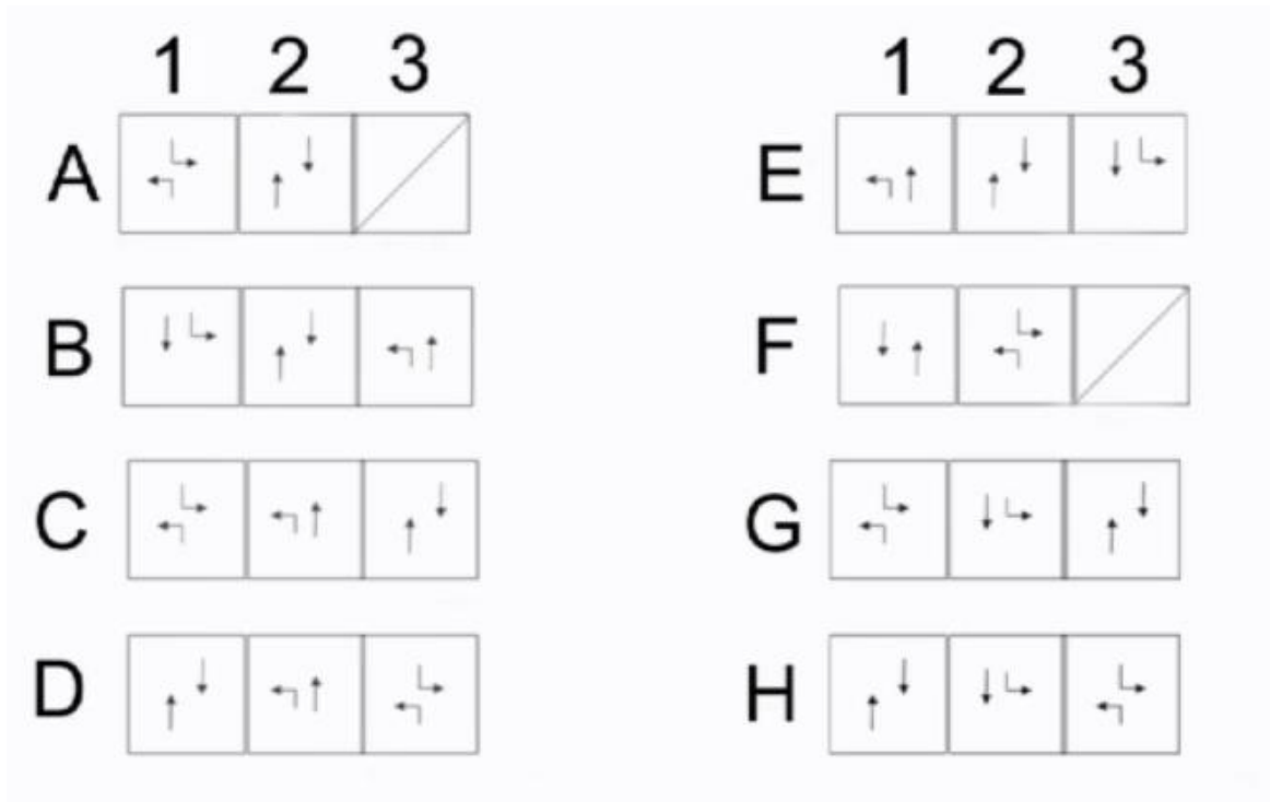
Figure 2.3 States and sequences digitally called in InSync [6]
