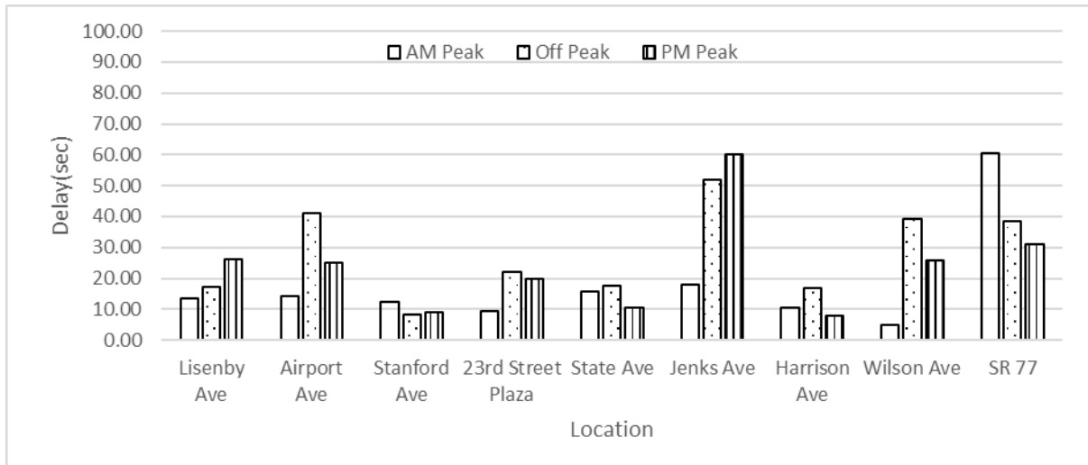
Figure E-3.5 Delay (sec) for each intersection through movement along the EB direction
