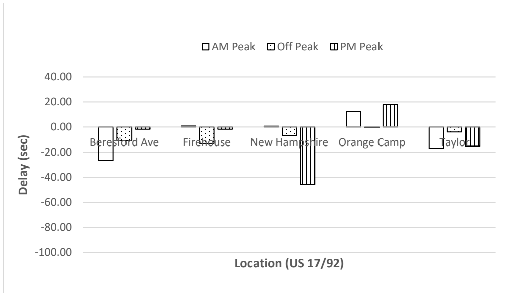
Figure B-3.6 Difference in delay (sec) for each intersection through movement along the NB direction
