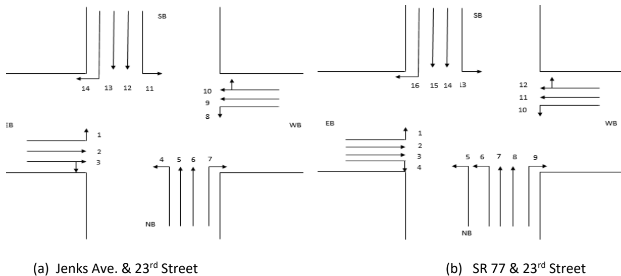
Figure E-3.9 Lane configuration of critical intersections
