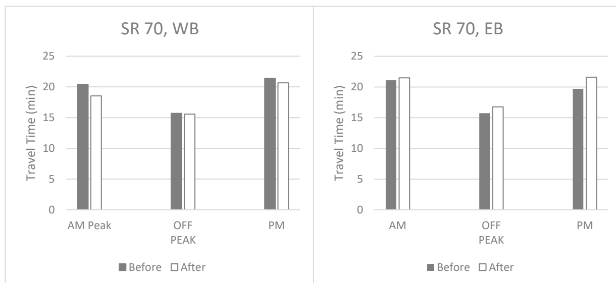
Figure G-3.1 Travel times along SR 70, Manatee County
