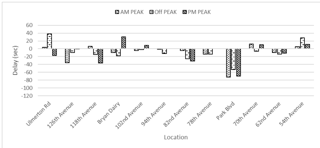
Figure F-3.7 Difference in delay (sec) for each intersection through movement along the NB direction
