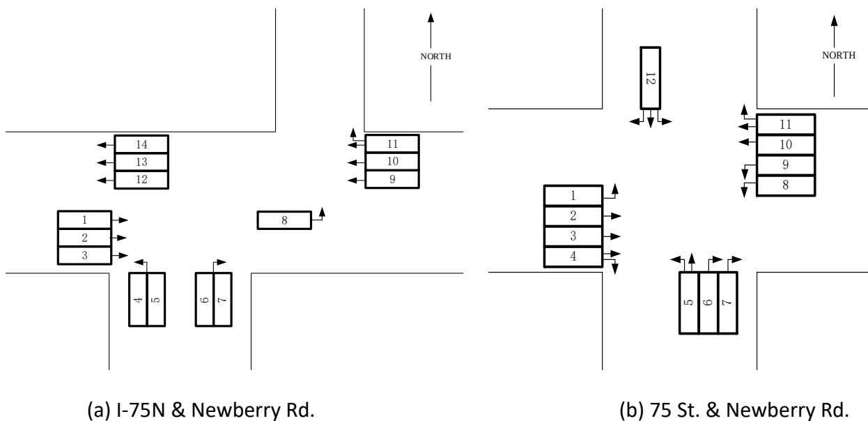
Figure A-3.8 Lane configuration of critical intersections
