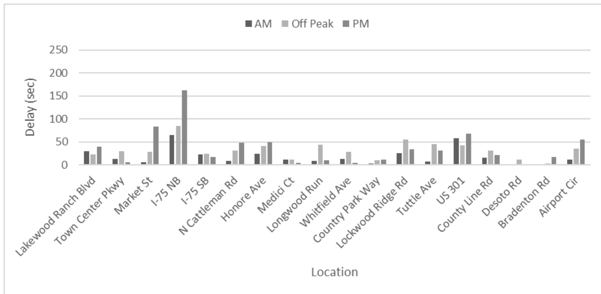
Figure D-3.3 Delay (sec) for each intersection through movement along the WB direction After Study (Mar.14 & Mar.15, 2017)
