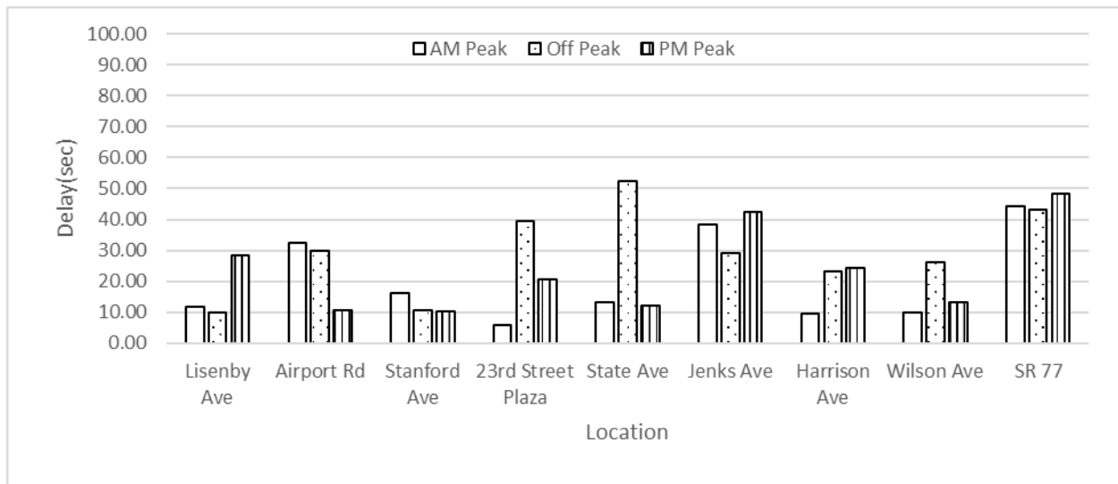
Figure E-3.3 Delay (sec) for each intersection through movement along the EB direction
