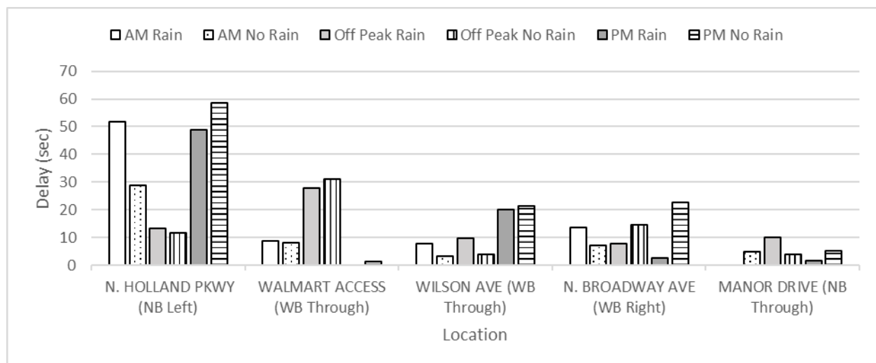
Figure H-3.3 Delay (sec) for each intersection movement along the WB direction
