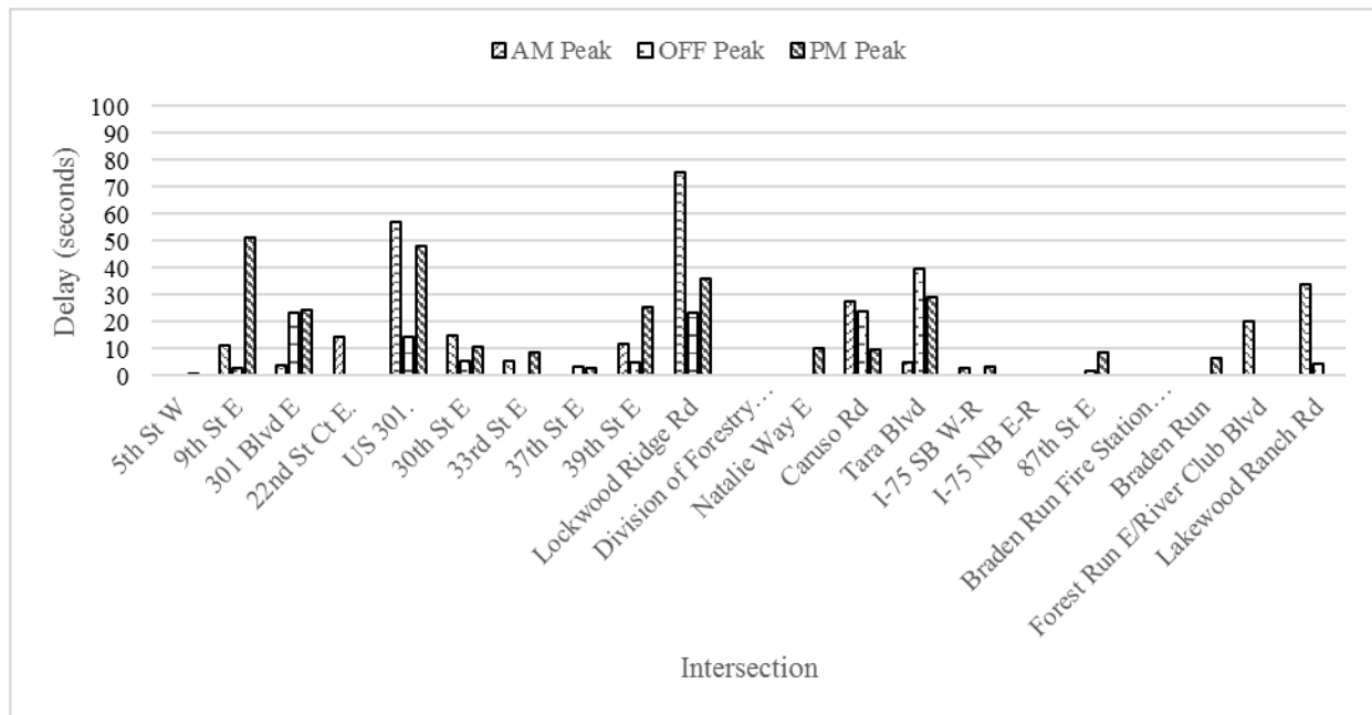
Figure G-3.4 Delay (s) for each intersection through movement along the EB direction – before study
