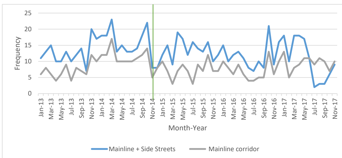
Figure 4.2 Temporal profile of total crashes along US-17/92 corridor
