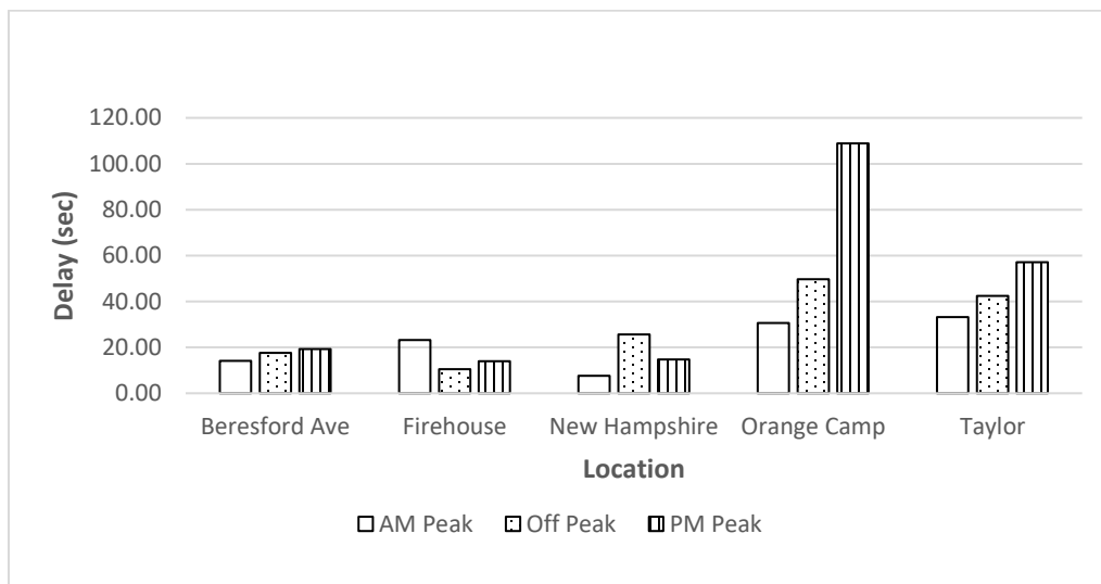
Figure B-3.3 Delay (sec) for each intersection through movement along the SB direction
