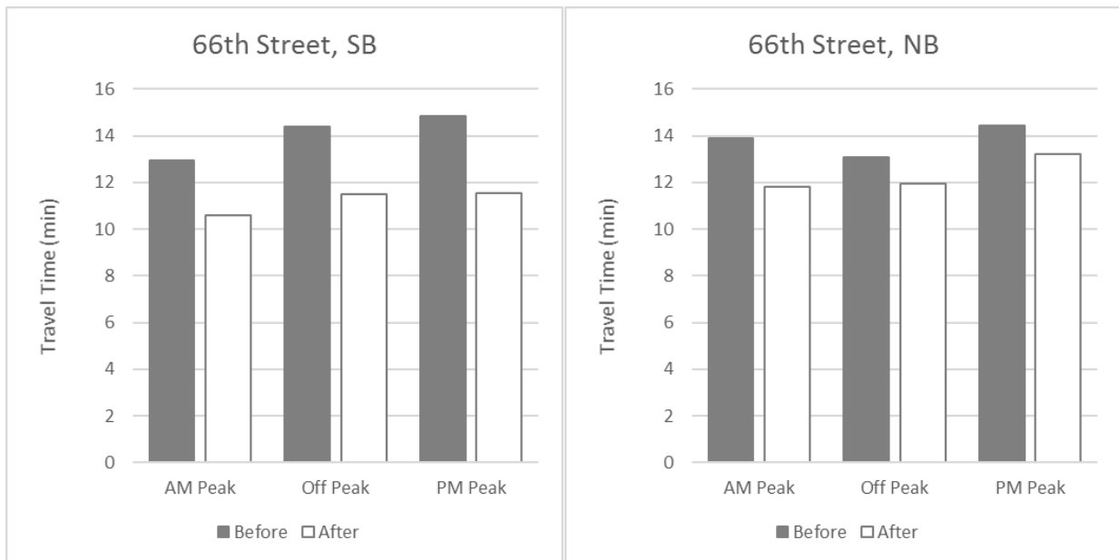
Figure F-3.1 Travel times along 66 th street, Pinellas County
