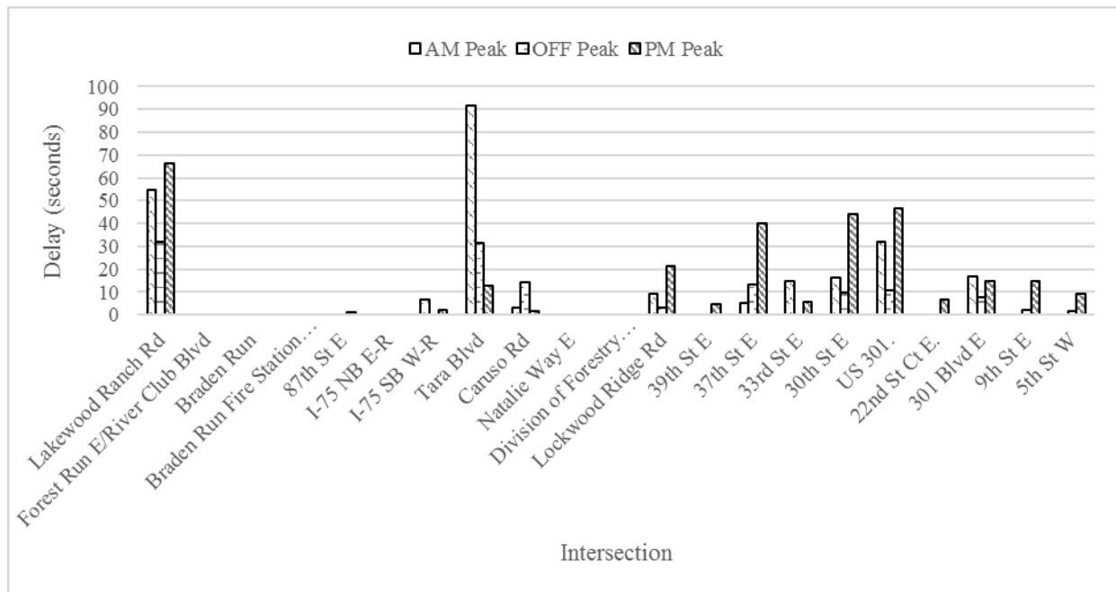
Figure G-3.7 Delay (s) for each intersection through movement along the WB direction – after study
