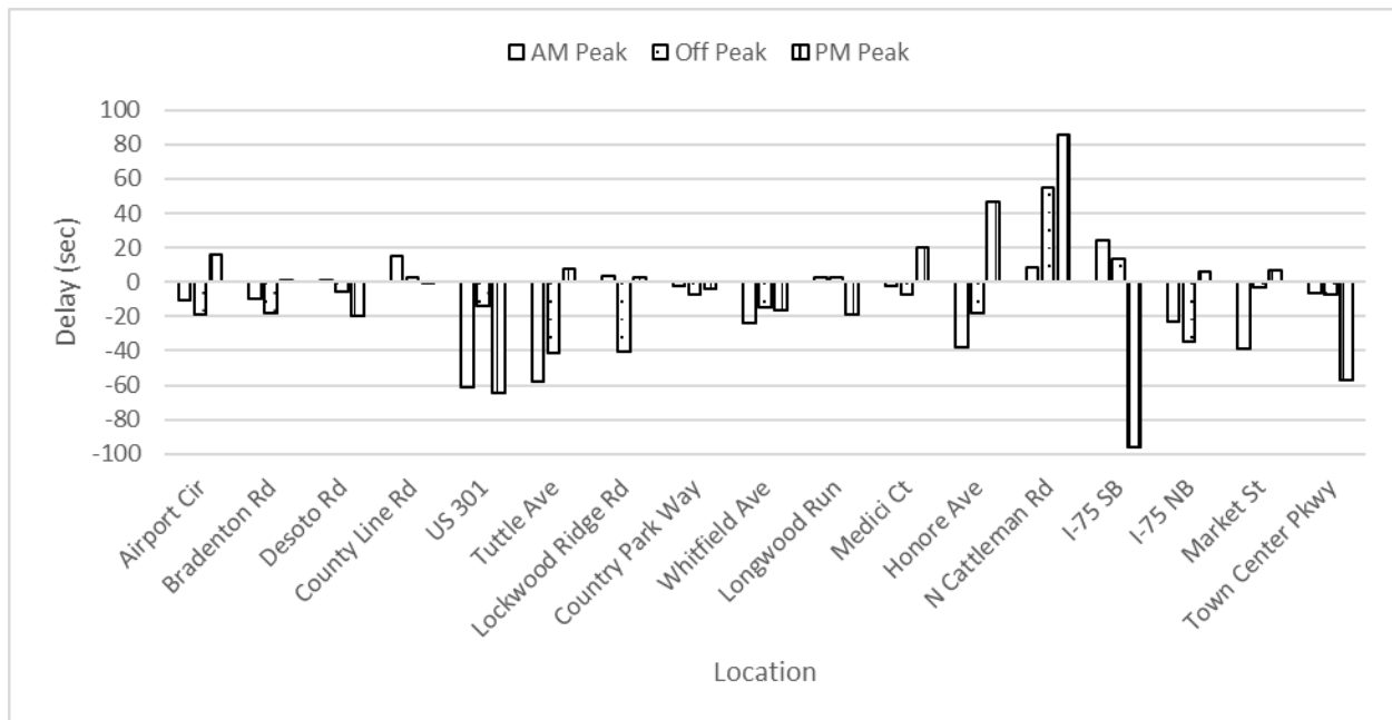
Figure D-3.6 Difference in delay (sec) for each intersection through movement along the EB direction
