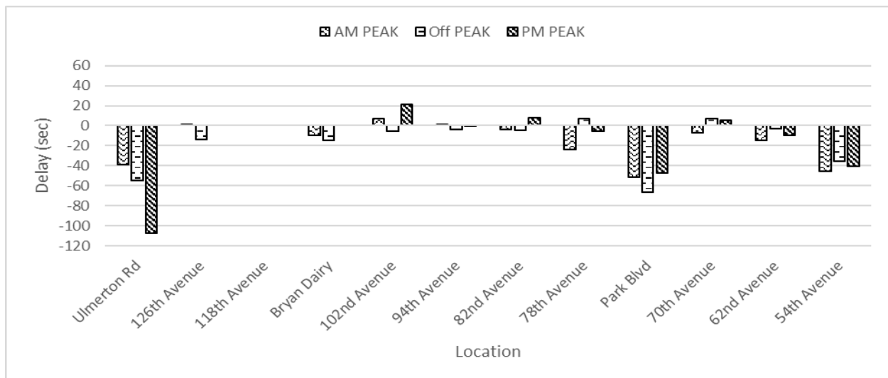
Figure F-3.6 Difference in delay (sec) for each intersection through movement along the SB direction
