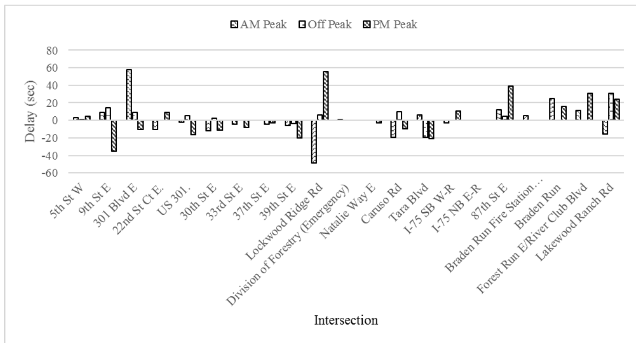
Figure G-3.8 Difference in delay (sec) for each intersection through movement along the EB direction
