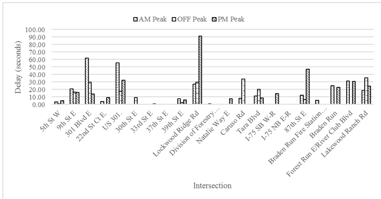
Figure G-3.6 Delay (s) for each intersection through movement along the EB direction – after study
