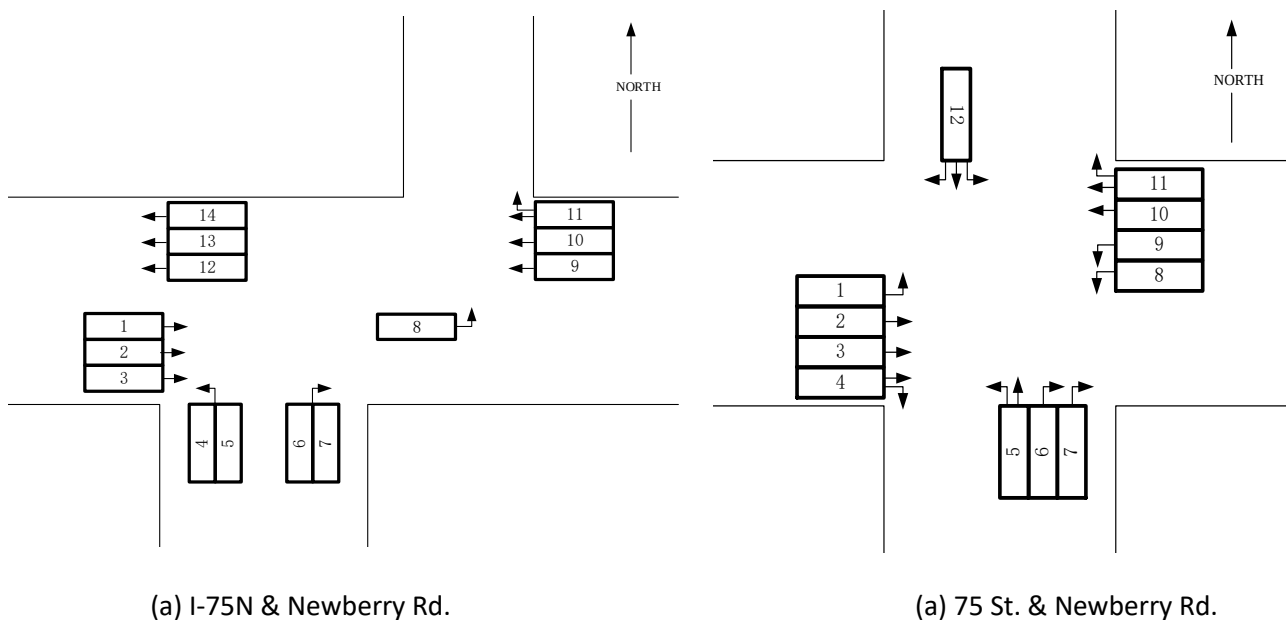
Figure A-3.9 Lane configuration of critical intersections
