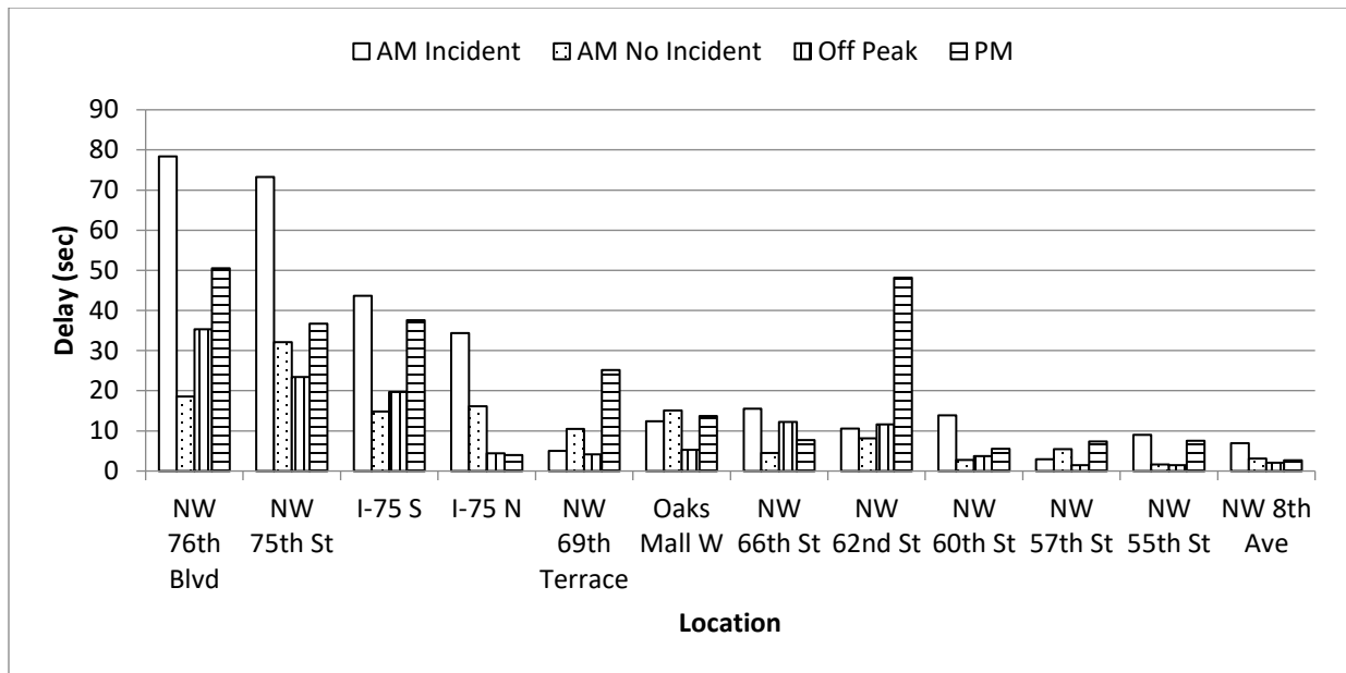
Figure A-3.2 Delay (sec) for each intersection through movement along the EB direction
