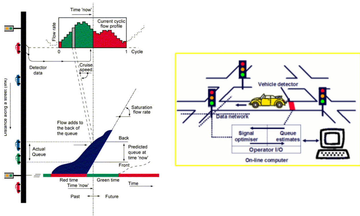
Figure 2.5 SCOOT operation procedure [22]
