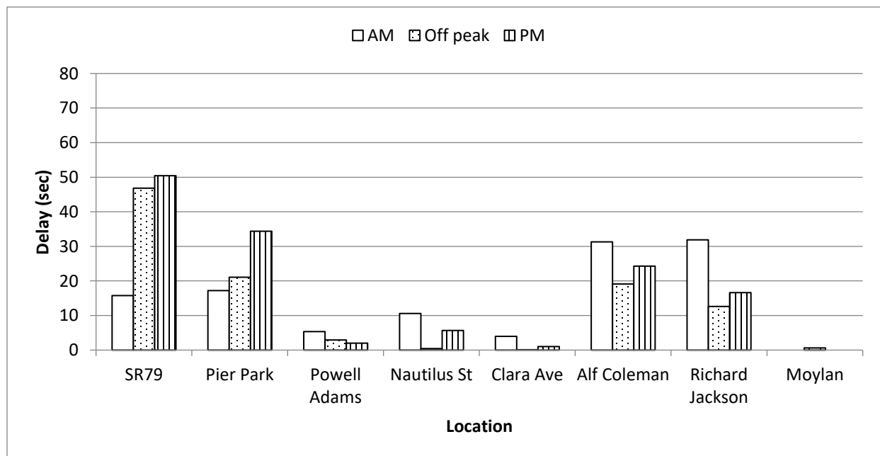
Figure C-3.2 Delay (sec) for each intersection through movement along the EB direction
