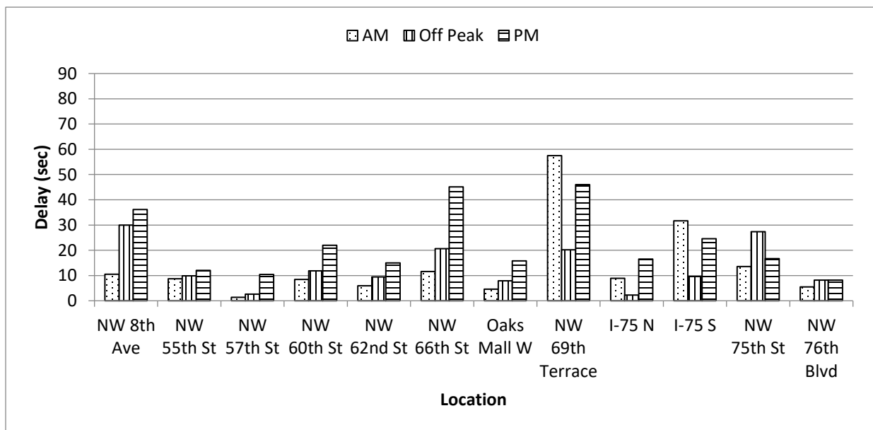
Figure A-3.5 Delay (sec) for each intersection through movement along the WB direction
