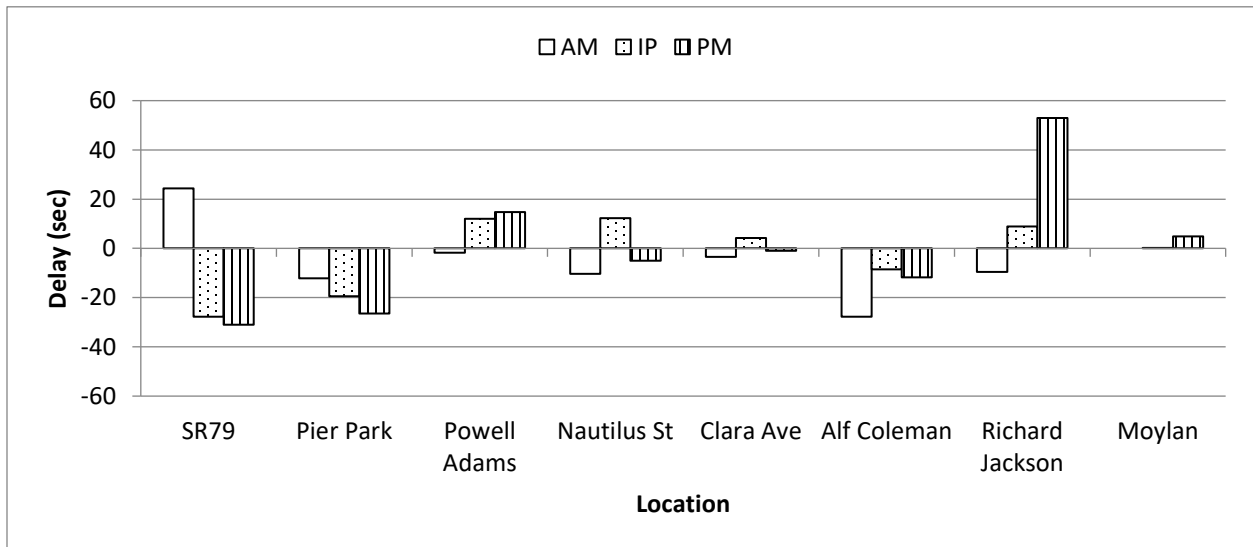
Figure C-3.6 Difference in delay (sec) for each intersection through movement along the EB direction
