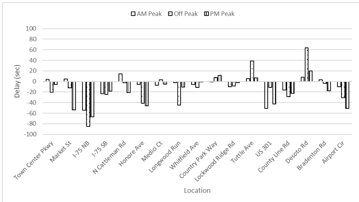
Figure D-3.7 Difference in delay (sec) for each intersection through movement along the WB direction
