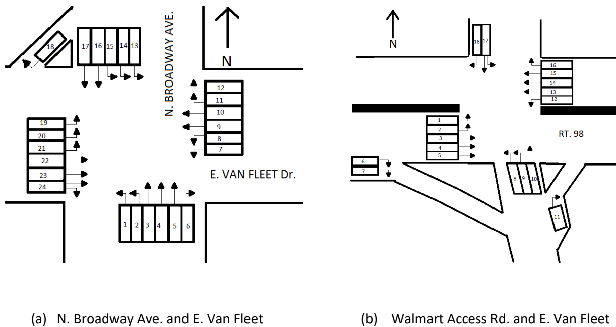
Figure H-3.8 Lane configuration of critical intersections
