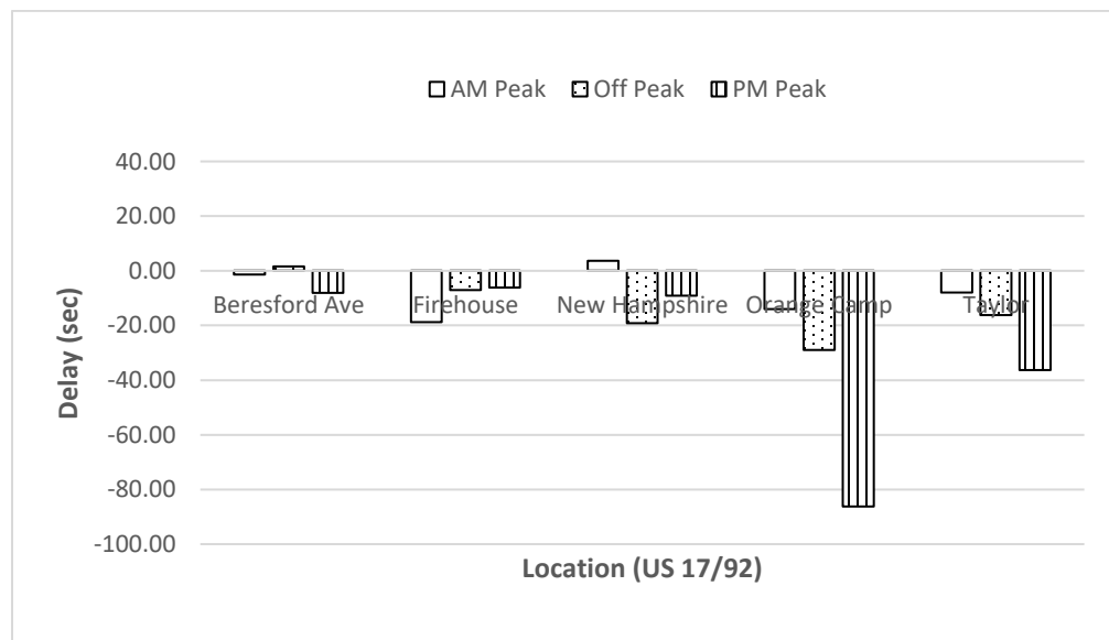
Figure B-3.7 Difference in delay (sec) for each intersection through movement along the SB direction
