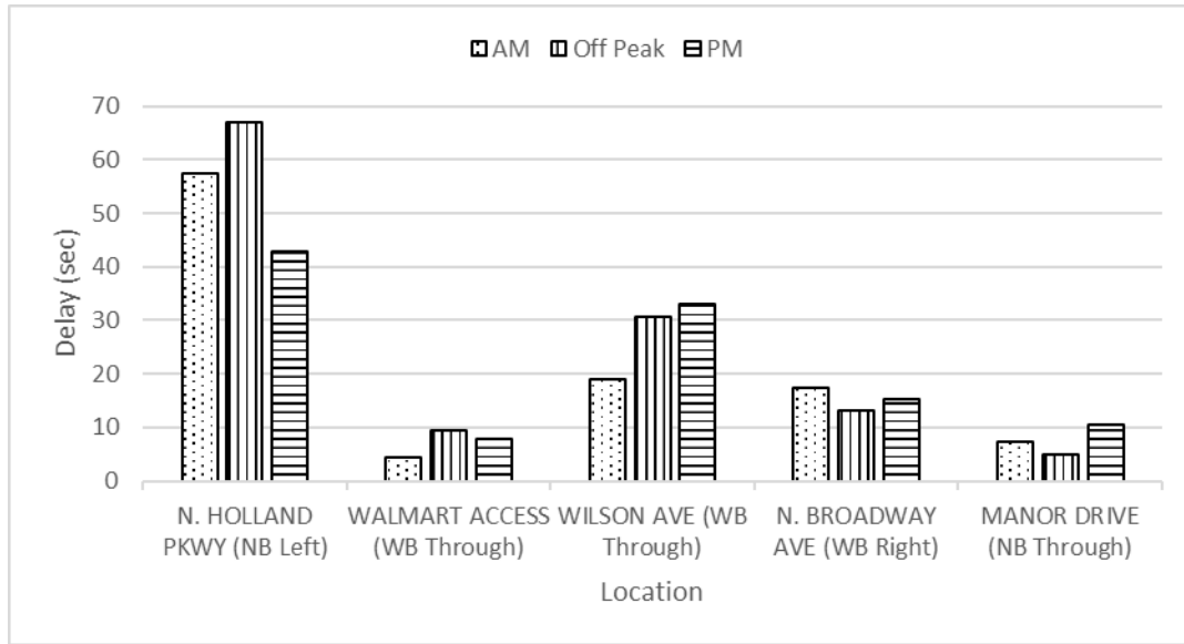
Figure H-3.5 Delay (sec) for each intersection movement along the WB direction – after study
