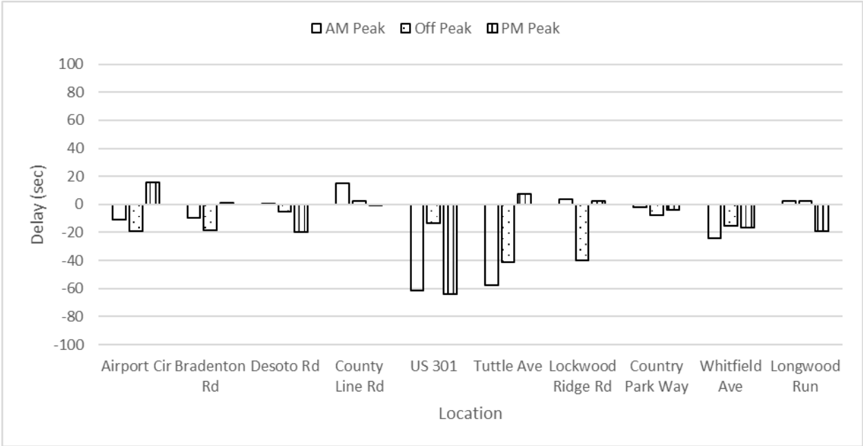
Figure D-3.8 Difference in delay (sec) for each intersection on western part of the corridor along the EB direction
