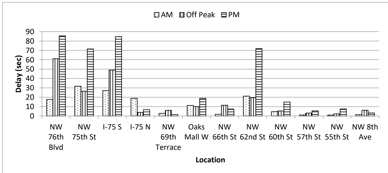
Figure A-3.4. Delay (sec) for each intersection through movement along the EB direction
