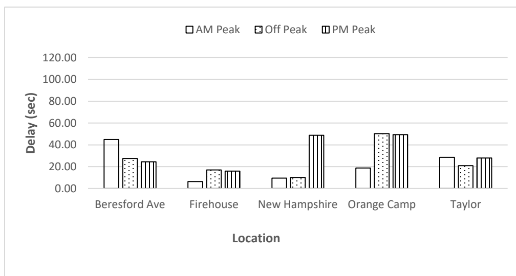
Figure B-3.2 Delay (sec) for each intersection through movement along the NB direction
