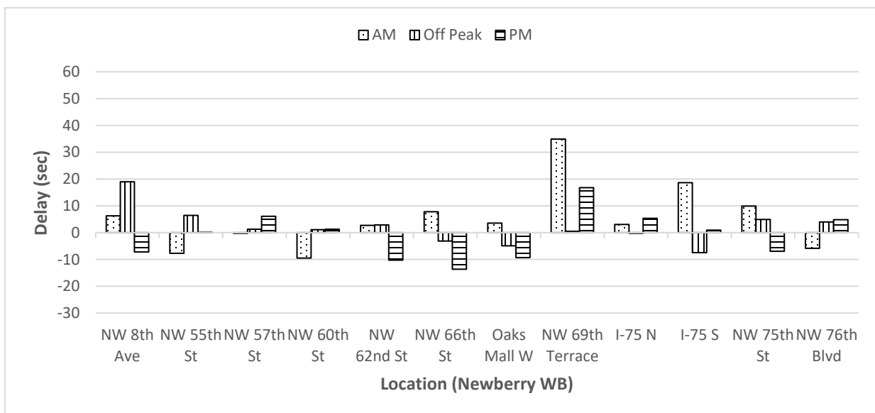
Figure A-3.7 Difference in delay (sec) for each intersection through movement along the WB direction
