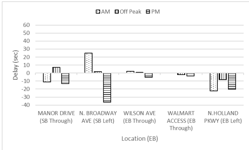
Figure H-3.6 Difference in delay (sec) for each intersection movement along the EB direction
