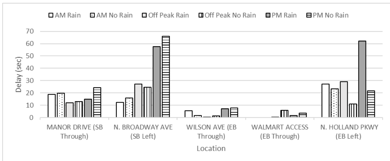
Figure H-3.2 Delay (sec) for each intersection movement along the EB direction
