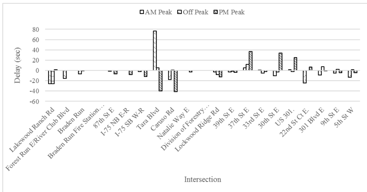
Figure G-3.9 difference in delay (sec) for each intersection through movement along the WB direction
