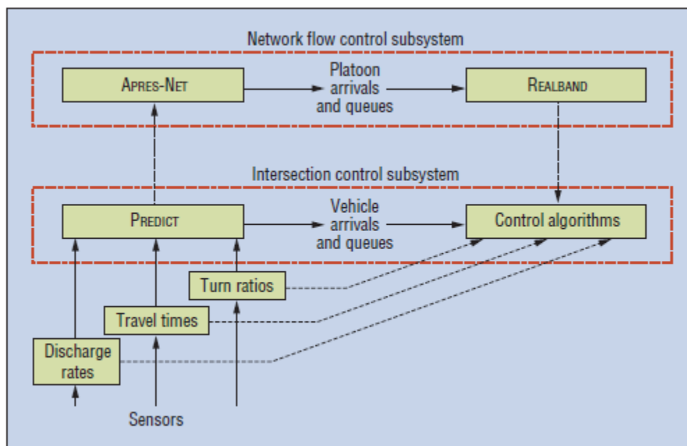
Figure 2.1 Middle and lower levels of RHODES architecture [26]
