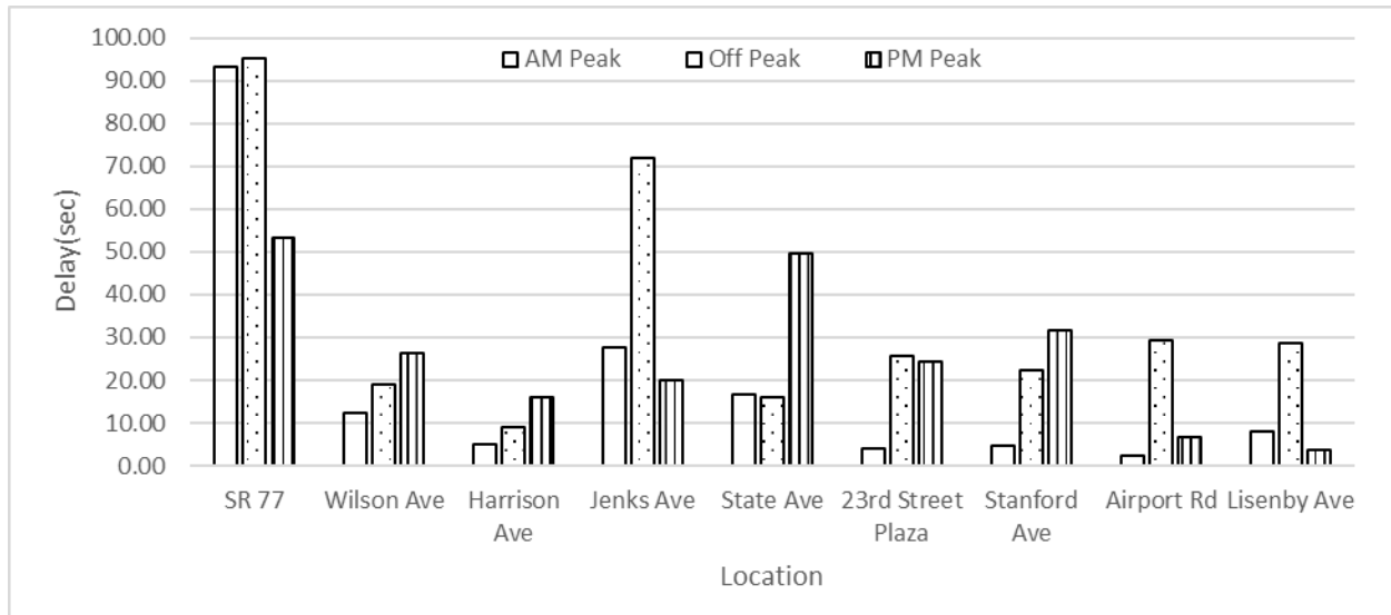
Figure E-3.4 Delay (sec) for each intersection through movement along the WB direction
