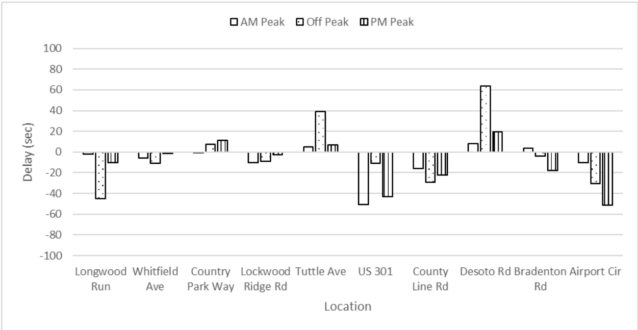
Figure D-3.9 Difference in delay (sec) for each intersection on western part of the corridor along the WB direction
