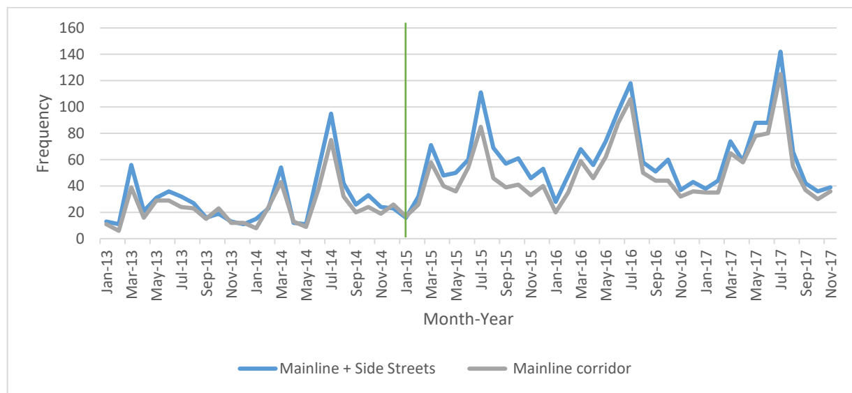
Figure 4.4 Temporal profile of total crashes along PCB Parkway corridor
