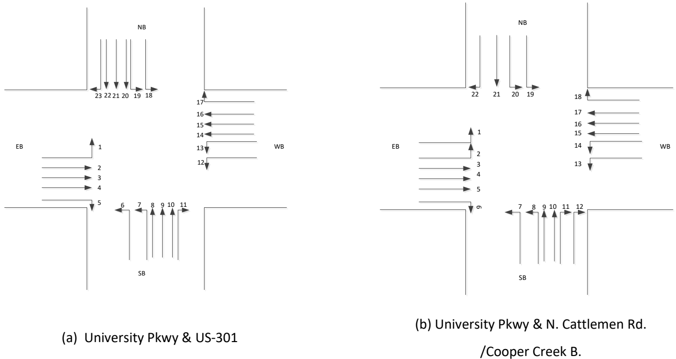
Figure D-3.11 Lane configuration of critical intersections
