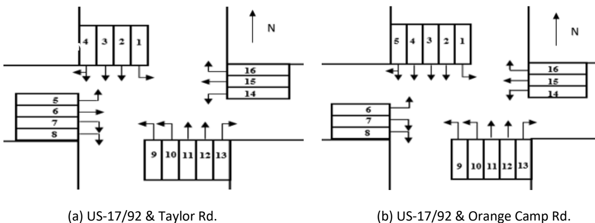
Figure B-3.8 Lane configuration of critical intersections
