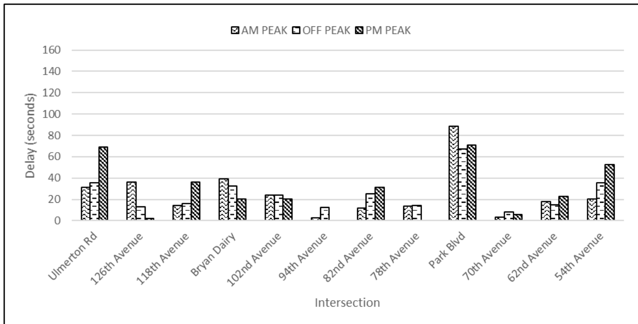
Figure F-3.3 Delay (s) for each intersection through movement along the NB direction – before study
