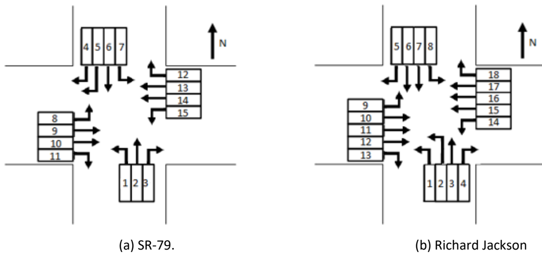
Figure C-3.8 Lane configuration of critical intersections
