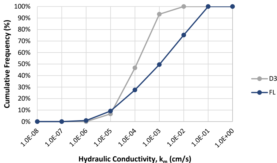
Figure 5-47. VIP cumulative frequency distributions for FDOT District 3 and Florida.
