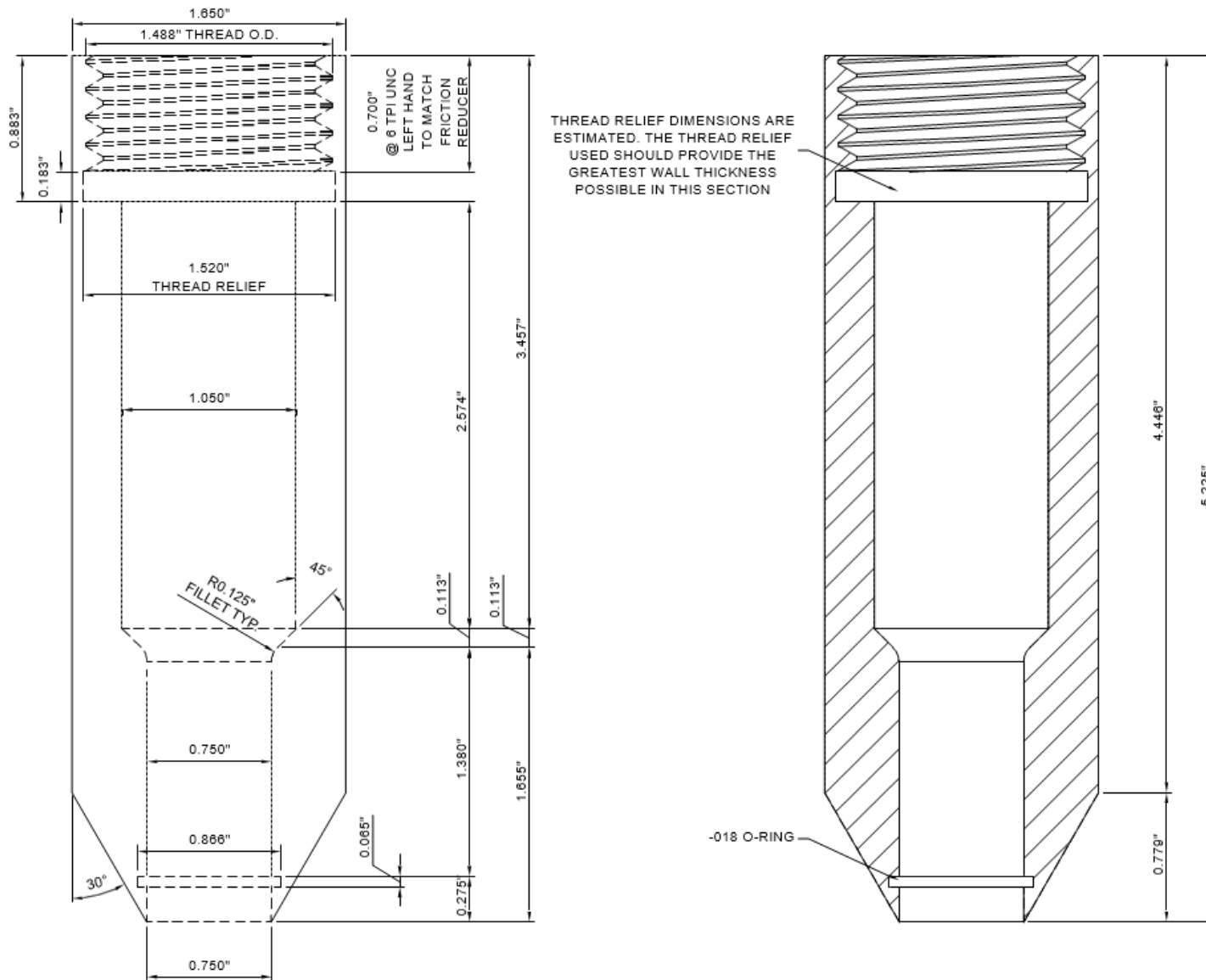
Figure 4-14. Nose cone.
