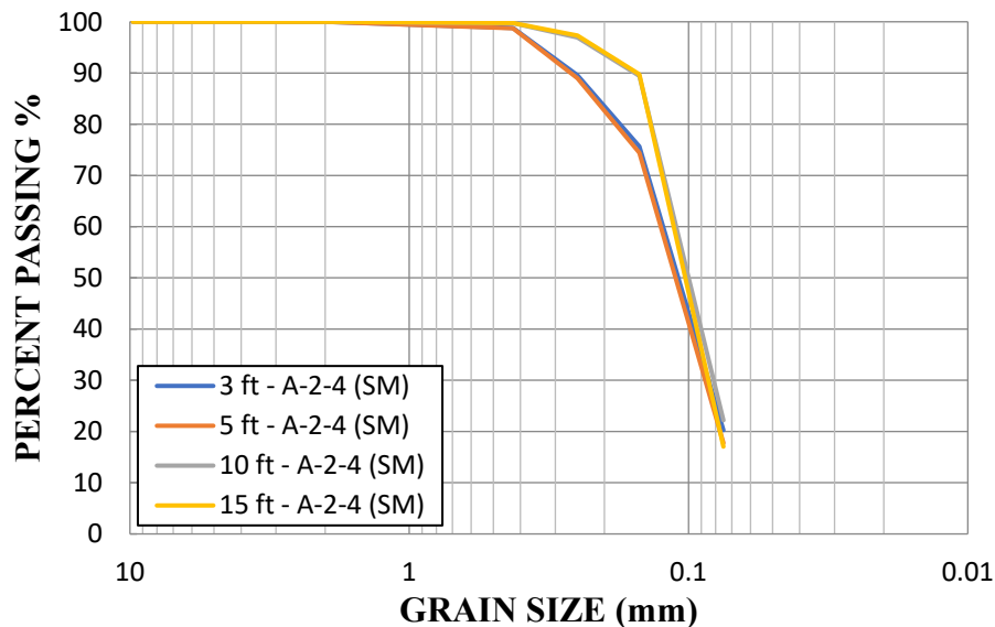
Figure 5-39. Brooksville Location P-1 and P-2 sieve analyses.
