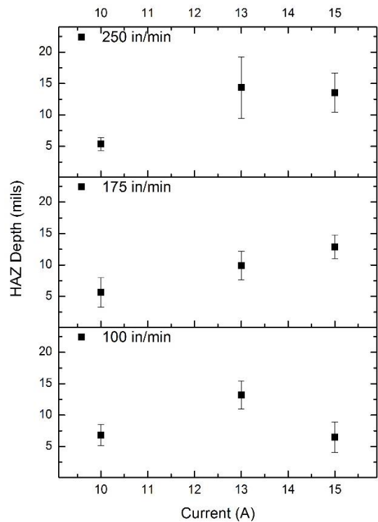
Figure 3-4. Average HAZ depth as function of amperage at discrete marking speeds (Plate A)
