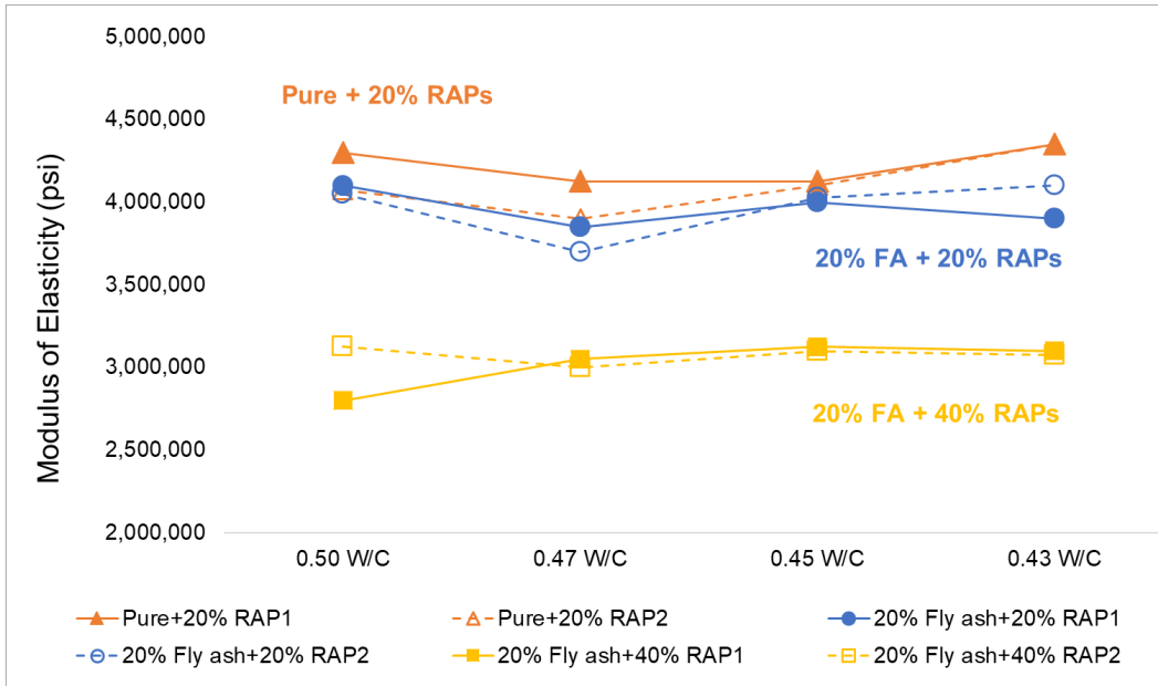
Figure 6-6. MOE versus w/c of concrete mixtures containing RAPs
