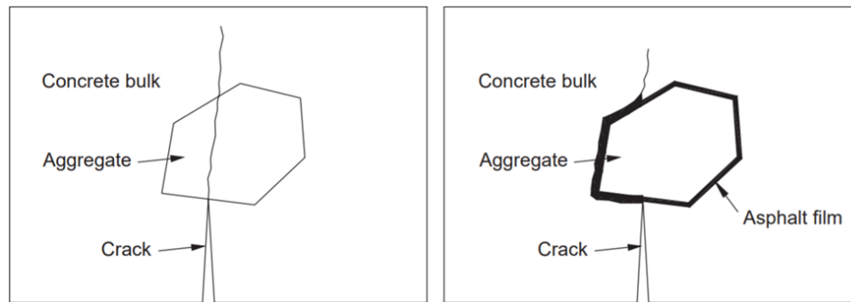
Figure 6-14. Propagation of crack through aggregate with and without asphalt film (Huang et al., 2006)
