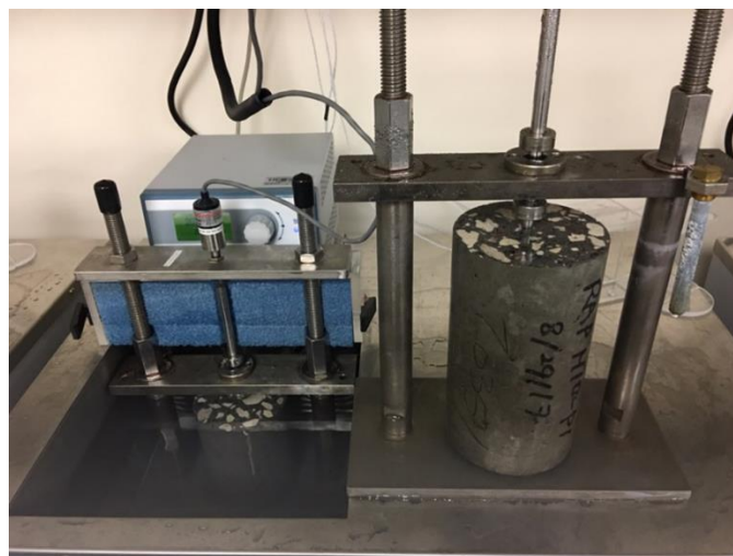
Figure 5-20. Coefficient of thermal expansion test
