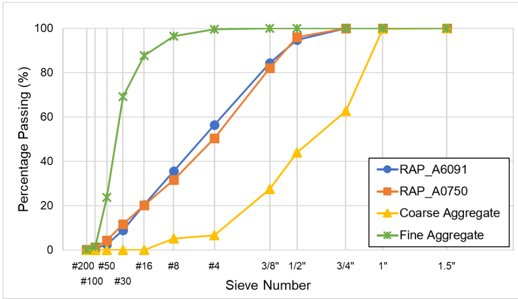
Figure 3-5. Gradation chart for selected RAPs versus virgin aggregates
