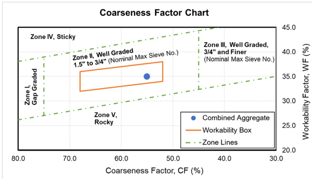
Figure 4-1. Example of coarseness factor chart
