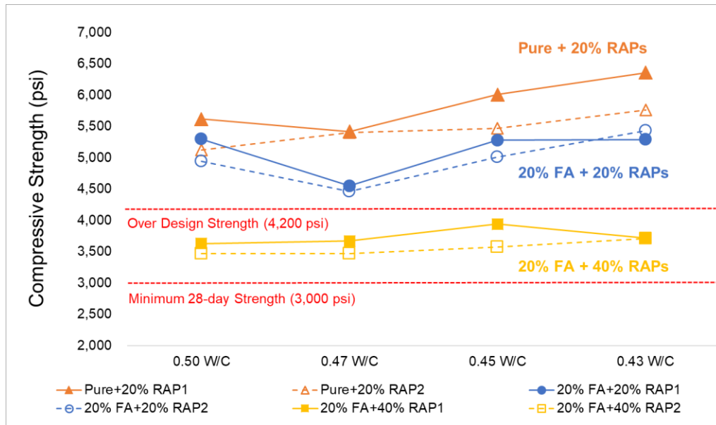
Figure 6-3. Compressive strength versus w/c of trial mixtures containing RAPs
