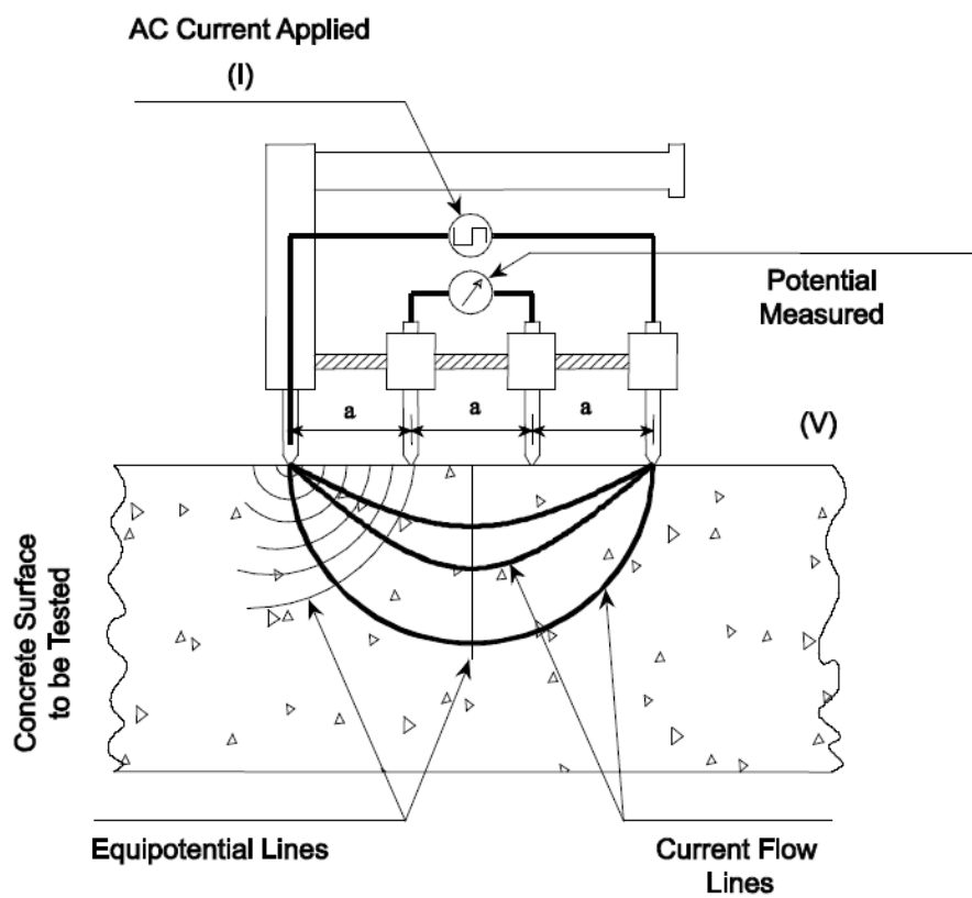
Figure 5-22. Four-point Wenner array probe set-up
