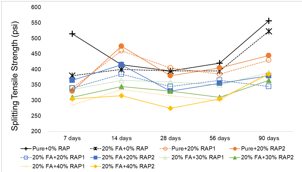
Figure 6-10. Development of splitting tensile strength in production mixtures at different curing times
