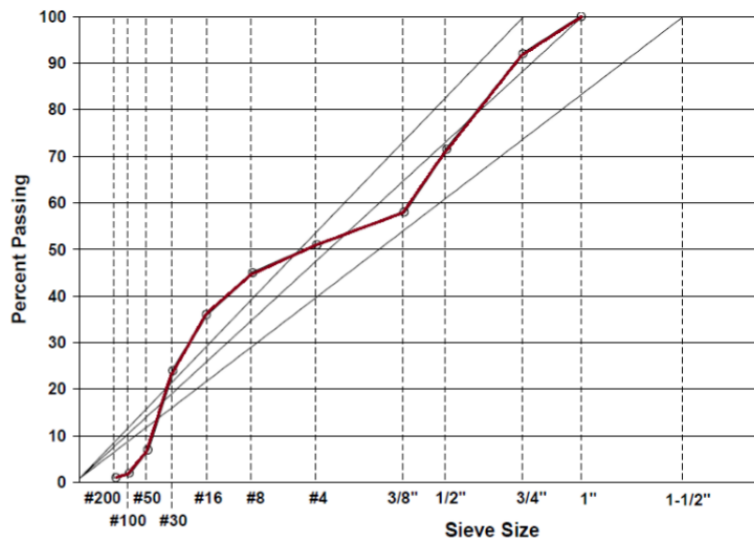
Figure 2-8. 0.45 power chart for a gap-graded mix
