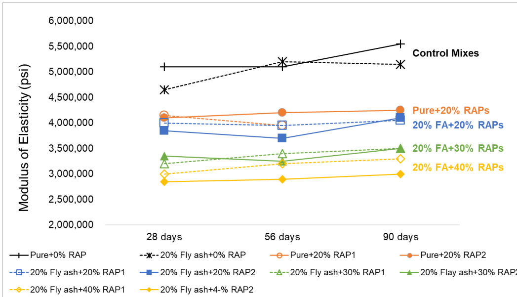
Figure 6-7. Development of modulus of elasticity at different curing times
