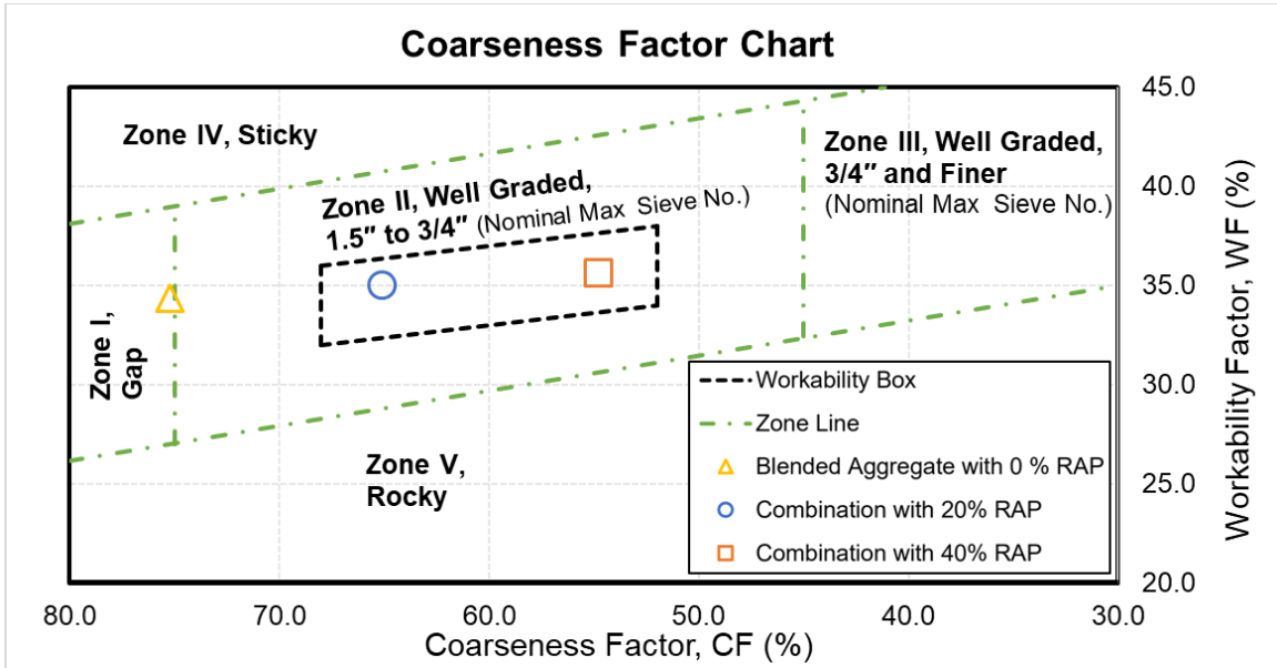
Figure 4-5. Coarseness factor chart for concrete mixtures containing RAP
