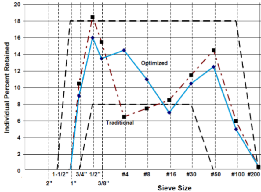
Figure 2-9. Individual percent retained for optimized mix
