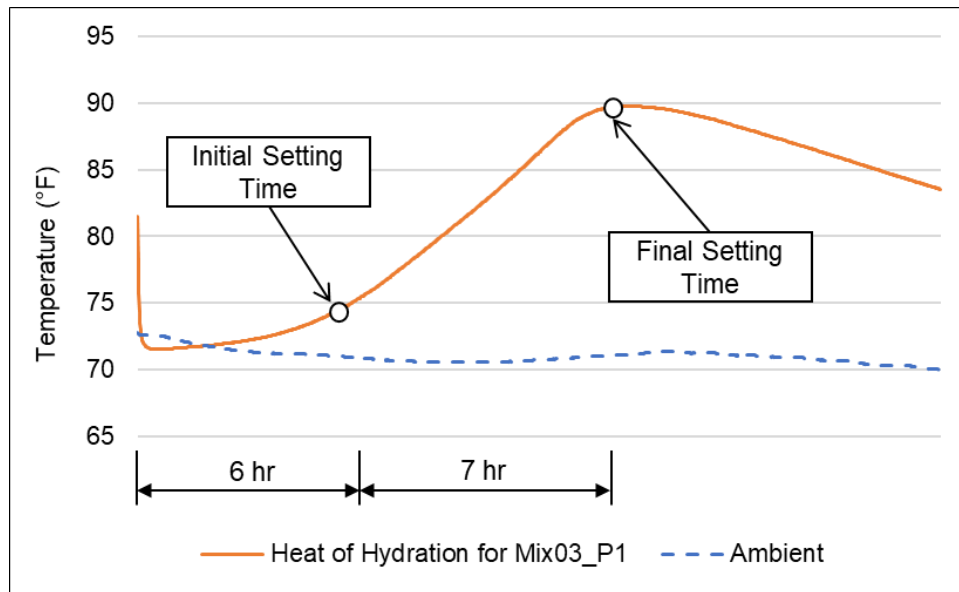
Figure 6-1. Heat of hydration of M03_P1 for measuring the initial and final setting time
