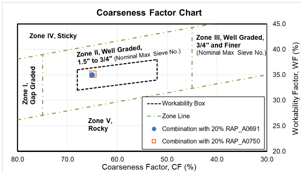
Figure 3-2. Coarseness factor chart of blended aggregates with 20% RAP
