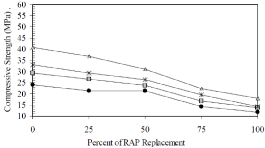
Figure 2-15. Compressive strength of concrete containing RAP (Al-Oraimi et al. 2009)
