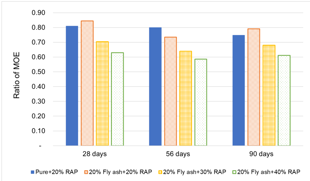
Figure 6-8. Ratios of modulus of elasticity at different curing times relative to the elastic modulus of the reference concrete
