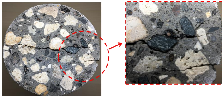
Figure 6-15. Observed crack propagation through the RAP concrete in splitting tensile strength test
