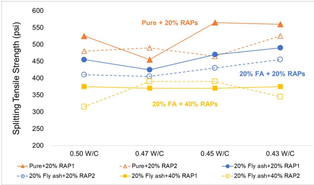
Figure 6-9. Splitting tensile strength versus w/c of trial mixtures containing RAPs
