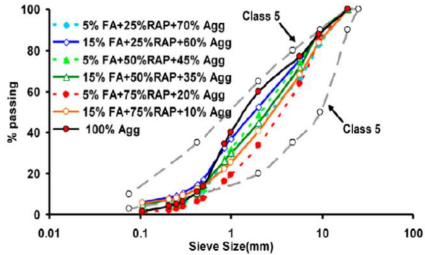
Figure 2-12. Particle size distribution of RAP and virgin aggregates (Kang et al. 2011)
