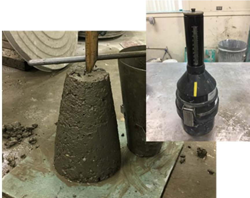
Figure 5-7. Testing of fresh concrete
