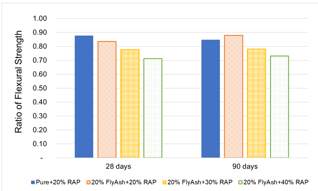
Figure 6-13. Ratio of flexural strength of production mixtures relative to the control mix
