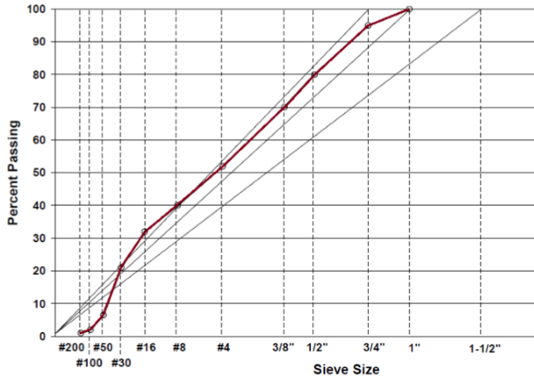
Figure 2-7. 0.45 power chart for a well graded mix
