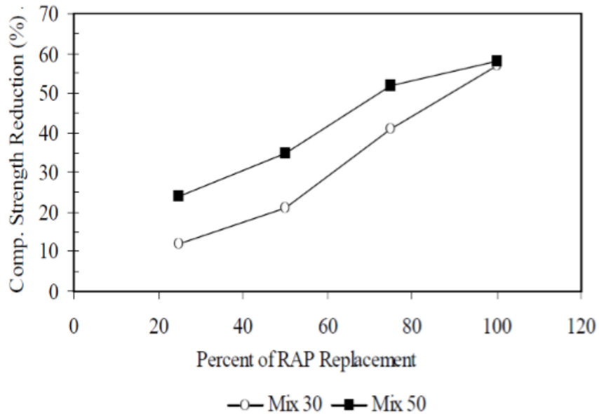
Figure 2-16. Reduction in compressive strength of concrete containing RAP (Al-Oraimi et al., 2009)
