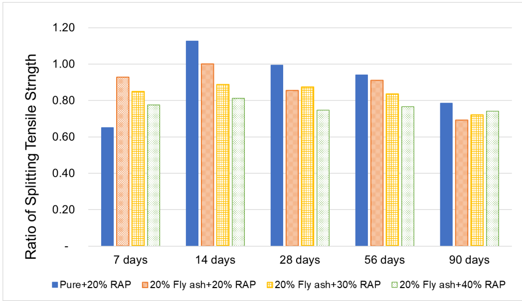
Figure 6-11. Ratios of splitting tensile strength of production mixtures relative to the control mix
