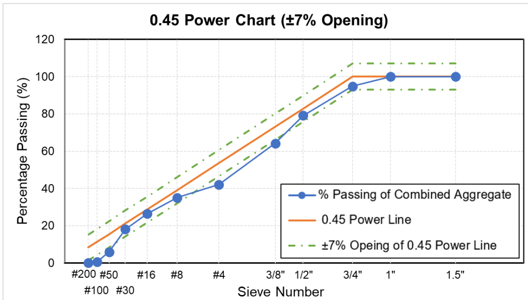
Figure 4-3. Example of 0.45 power chart
