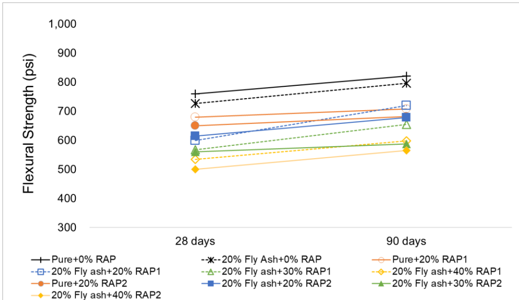
Figure 6-12. Flexural strength of production mixtures at different curing times
