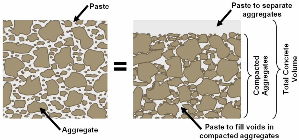
Figure 2-1. Representation of aggregate particles in paste (Koehler and Fowler, 2007)
