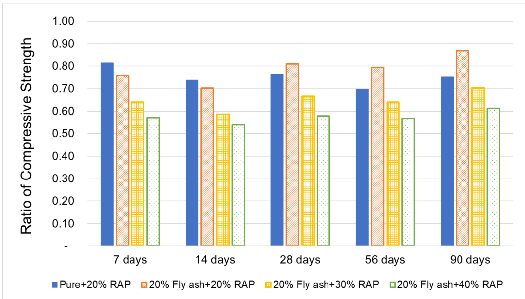
Figure 6-5. Ratios of compressive strength of RAP concrete relative to the control mix
