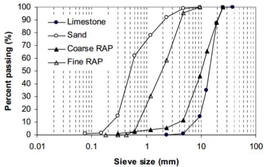
Figure 2-13. Gradation of aggregates and RAP (Huang et al., 2006)
