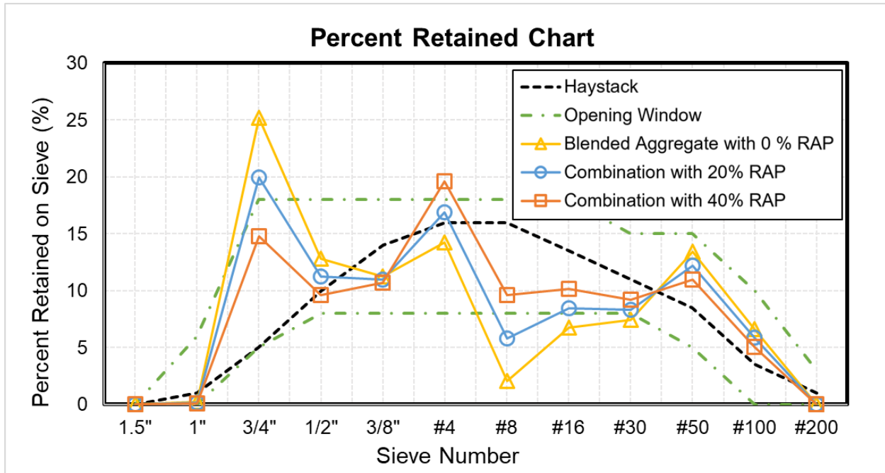
Figure 4-6. Percent retained chart for concrete mixtures containing RAP
