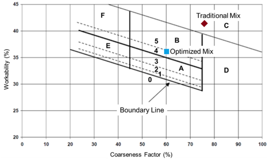
Figure 2-11. Coarseness factor chart for optimized mix
