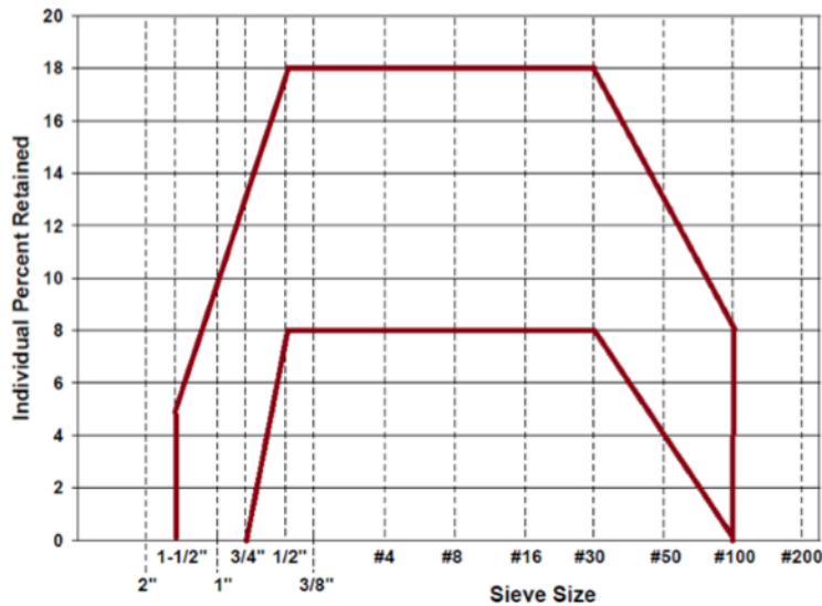
Figure 2-4. Shilstone 8-18 band chart
