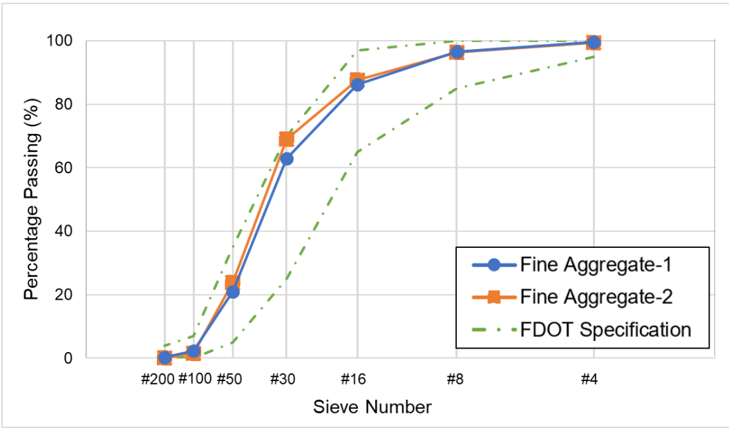
Figure 3-1. Gradation chart for virgin fine aggregates
