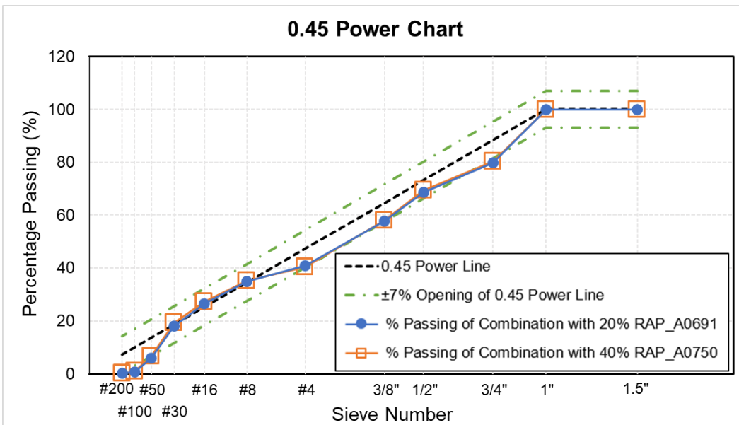
Figure 3-4. 0.45 power gradation chart of blended aggregates with 20% RAP
