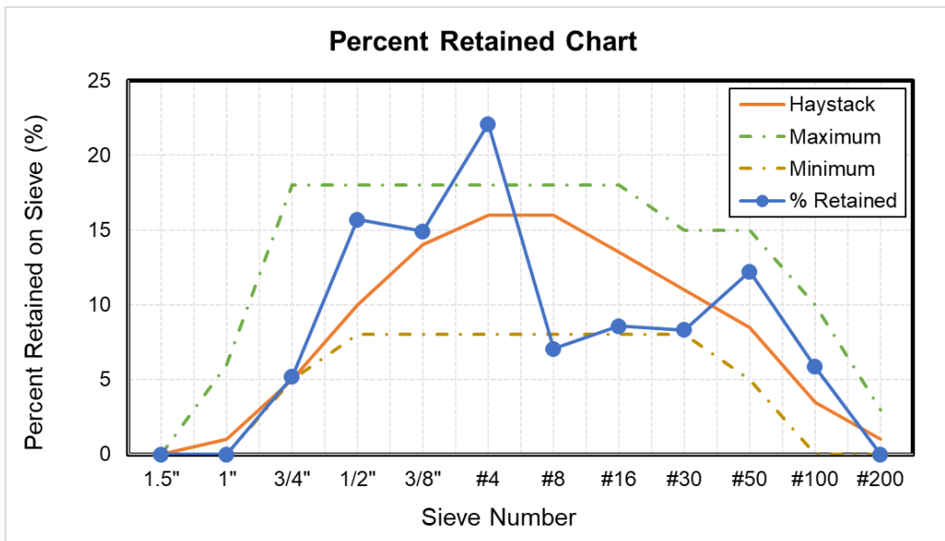
Figure 4-2. Example of percent retained chart
