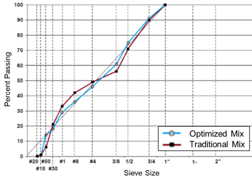
Figure 2-10. 0.45 power chart for optimized mix
