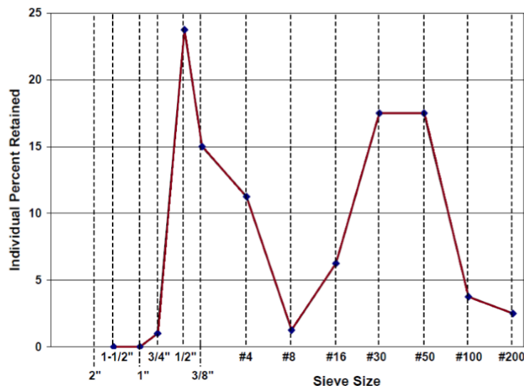
Figure 2-6. Problematic plot on individual percentage retained chart
