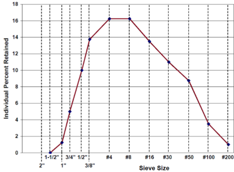
Figure 2-5. Ideal plot on individual percentage retained chart
