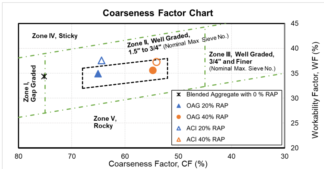
Figure 4-8. Coarseness factor chart of aggregate blends using OAG versus ACI procedure
