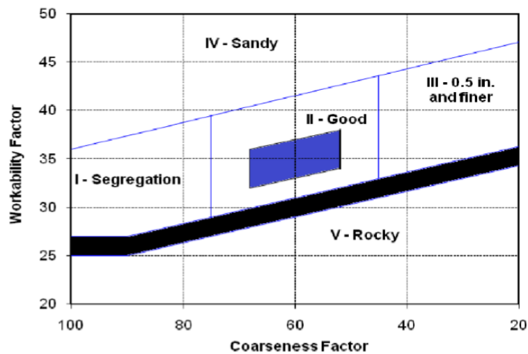
Figure 2-3. Coarseness factor chart proposed by Shilstone
