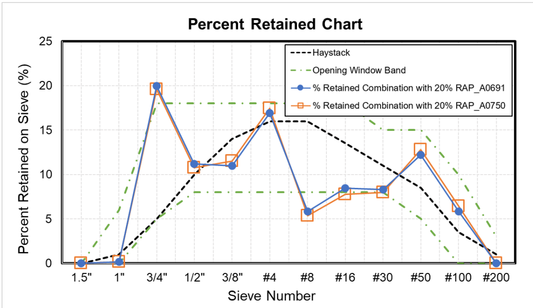
Figure 3-3. Percentage retained chart of blended aggregates with 20% RAP
