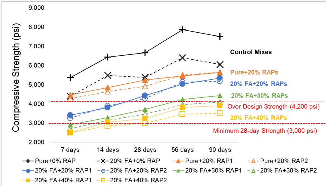
Figure 6-4. Development of compressive strength with curing time in production mixtures
