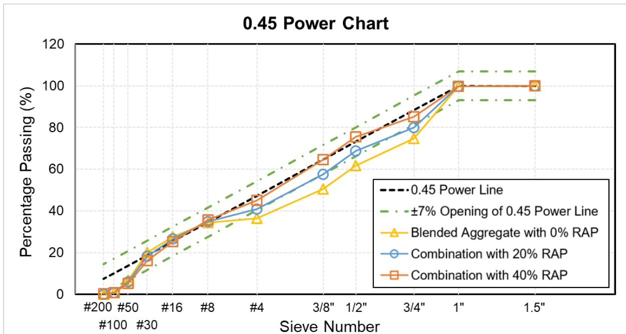
Figure 4-7. 0.45 power chart for aggregate gradation of concrete mixtures containing RAP
