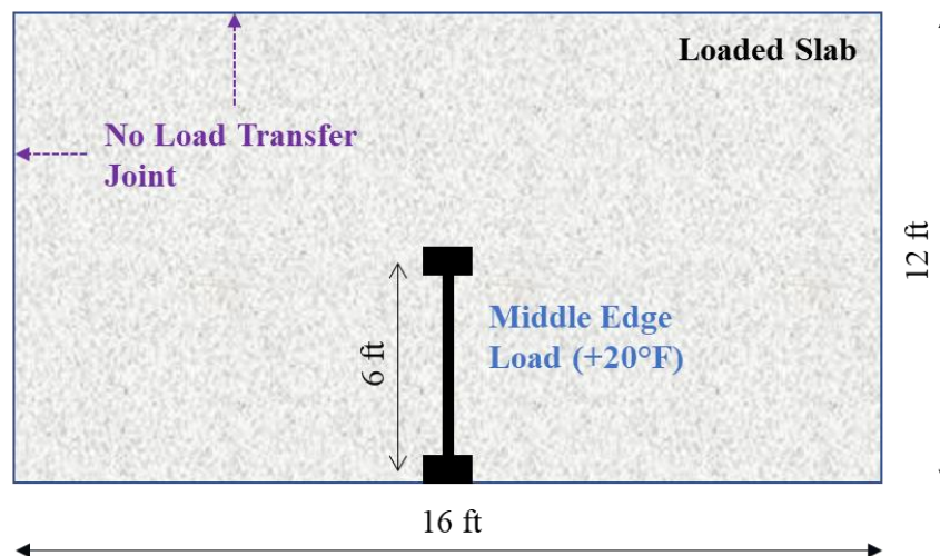
Figure 7-1. 3-D finite-element model for analysis of jointed plain concrete pavement under critical loading condition
