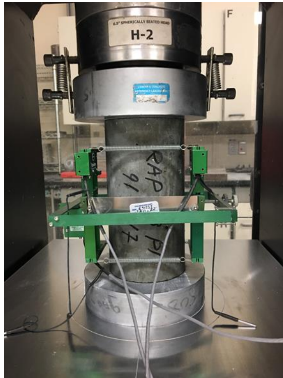
Figure 5-14. Modulus of elasticity and Poisson's ratio test equipment
