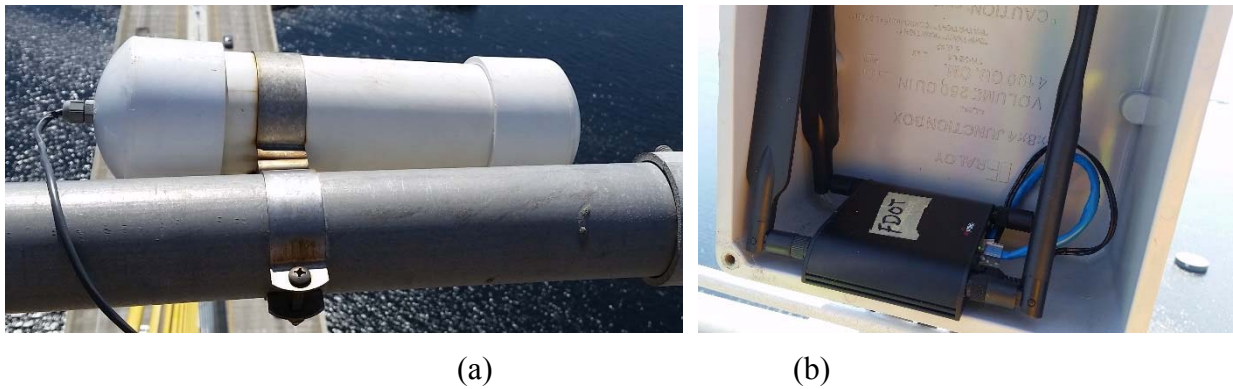
Figure 3-24. (a) North Tower RF modem housing and (b) Cradlepoint cellular modem.
