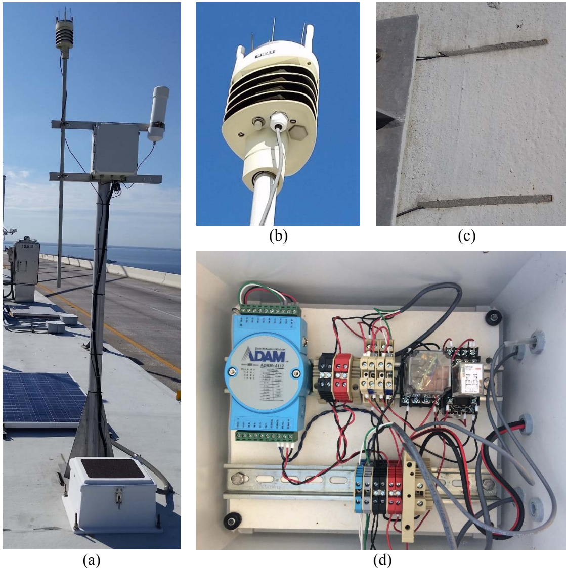
Figure 3-15. (a) Weather station, (b) integrated weather sensor, (c) embedded concrete thermocouples, and (d) interior of the EDS data acquisition and communication box.
