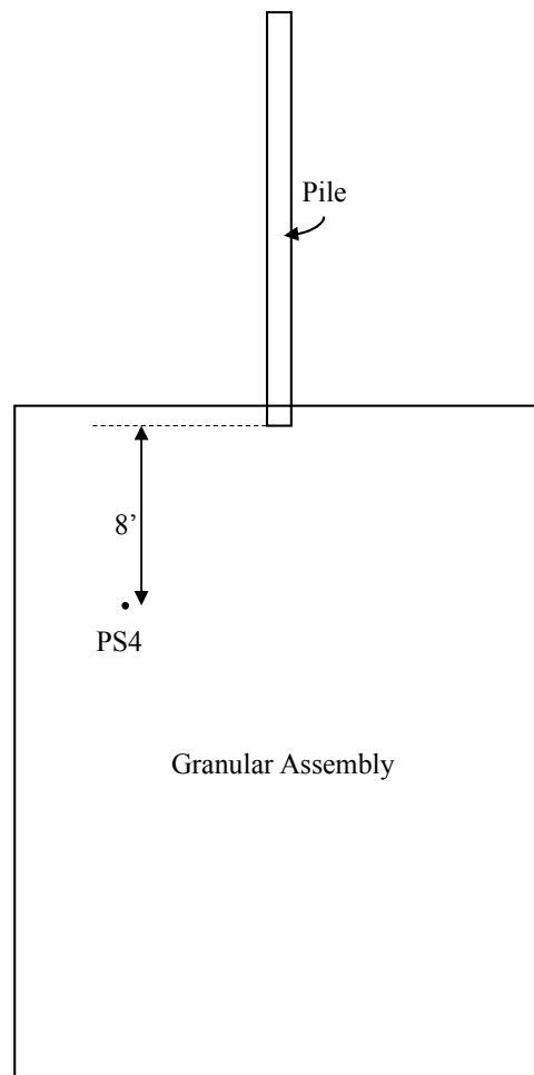
Figure 3.19 Schematic of pressure sensor PS 4 location (elevation)
