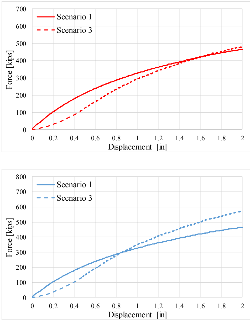
Figure 5.8 Scenario 1 and 3 top-down load-settlement behaviors at HOD of 5 ft (top; red curves) and 10 ft (bottom; blue curves) for the full SPW embedment case
