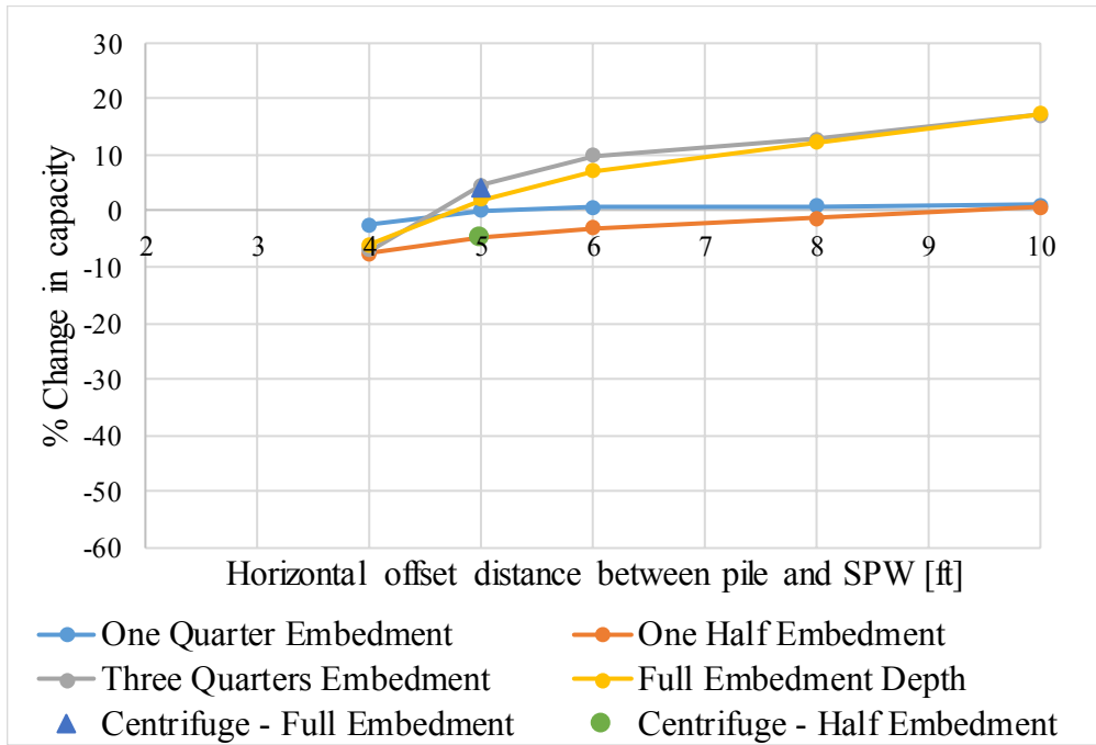
Figure 6.3 Variation of ultimate capacity in Scenario 3 with respect to horizontal offset distance (feet) and SPW embedment depth normalized by pile tip depth
