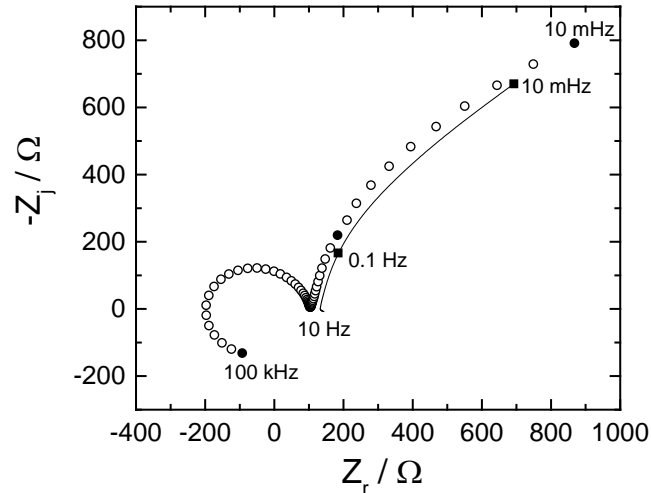
Figure 14. Simulated impedance results compared to the experimental results with an electrode configuration of 2356.
