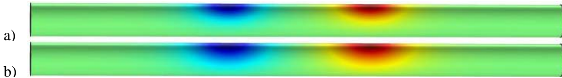
Figure 20. Current distribution on the steel surface at (a) 100 Hz and (b) 10 mHz for the active case.
