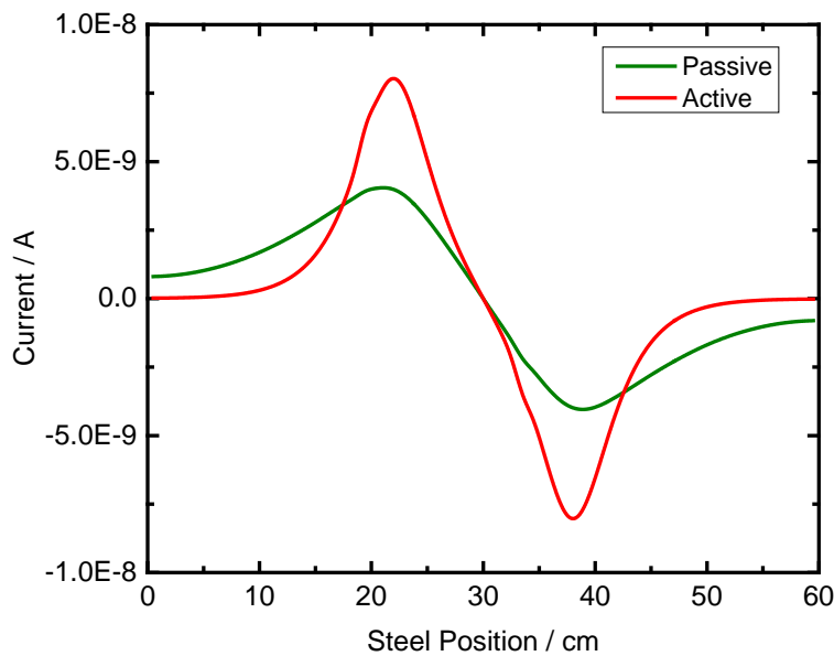
Figure 21. Current distribution on the steel surface at as a function of steel position at 10 mHz.
