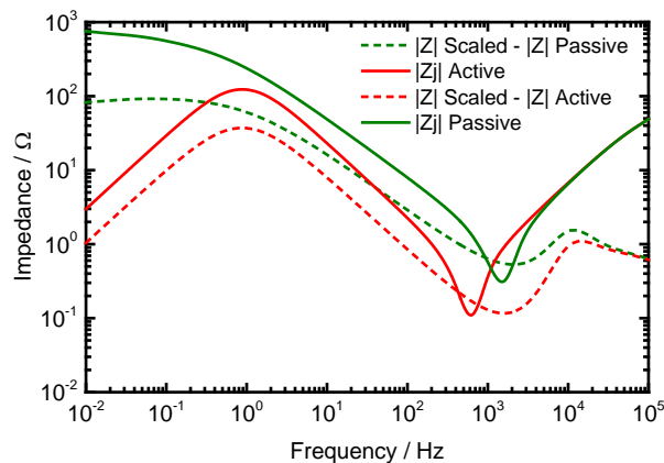
Figure 25. Difference in the magnitude of the potential scaled impedance and the magnitude of the impedance taken with the second reference point compared to the absolute value of the imaginary impedance taken with the second reference point as a function of frequency for the active and passive cases.
