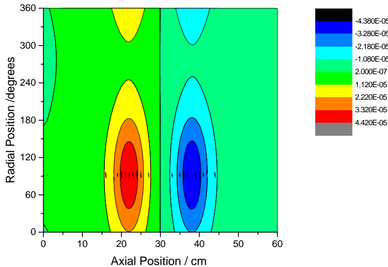
Figure 22. Current on the steel surface at 100 Hz.
