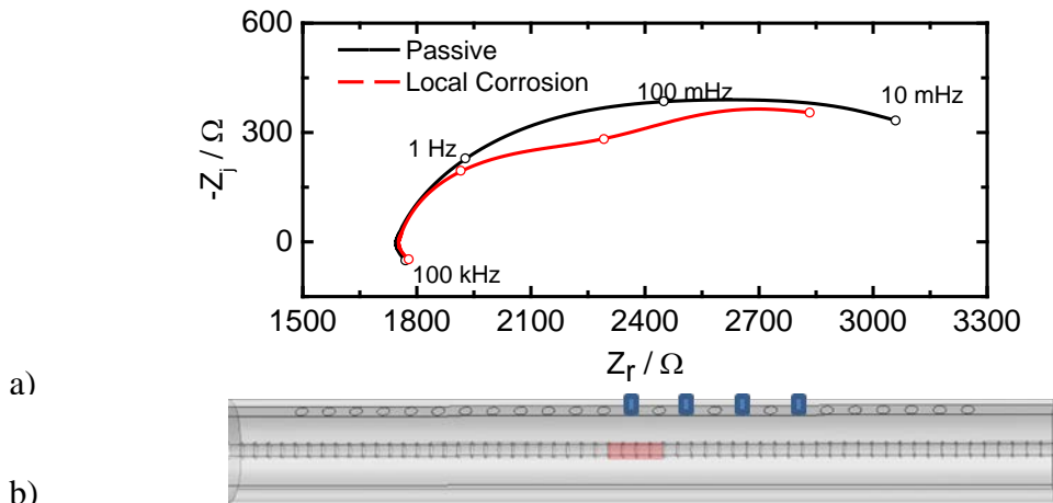
Figure 18. Simulated indirect impedance of a 2-ft model tendon containing one steel strand for a passive case and a locally corroding case of 4 cm at the midpoint of the steel strand. The centerline of the electrode array is 6 cm right of the centerline of the 2-ft tendon, and the working electrode is directly over the corroding area: a) impedance results; and b) schematic representation of the system geometry for a reference electrode spacing of 4 cm.
