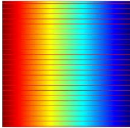
Figure 9. Current and potential distribution of a 1-cm-square, 10-Ohm-m resistivity grout model with current injecting electrodes placed on the vertical sides.
