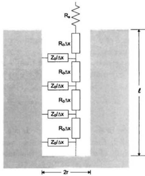
Figure 34. Schematic representations of a porous electrode: transmission line inside a cylindrical pore. Taken from Orazem and Tribollet. 18
