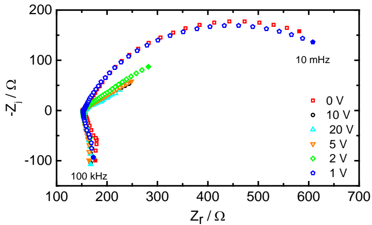
Figure 7. Four-point experimental impedance during the application of a constant potential difference between the steel and a surface electrode located at the center of the specimen.
