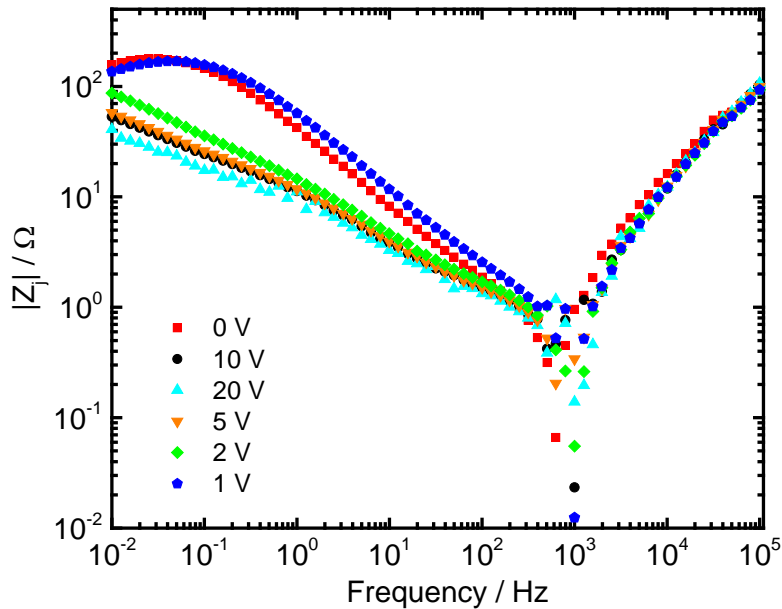
Figure 8. Four-point experimental imaginary impedance as a function of frequency during the application of a constant potential difference between the steel and a surface electrode located at the center of the specimen.
