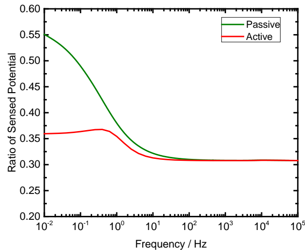
Figure 23. The ratio of the potential sensed between two impedance measurements where only the distance between reference electrodes is changed for the active and passive case.
