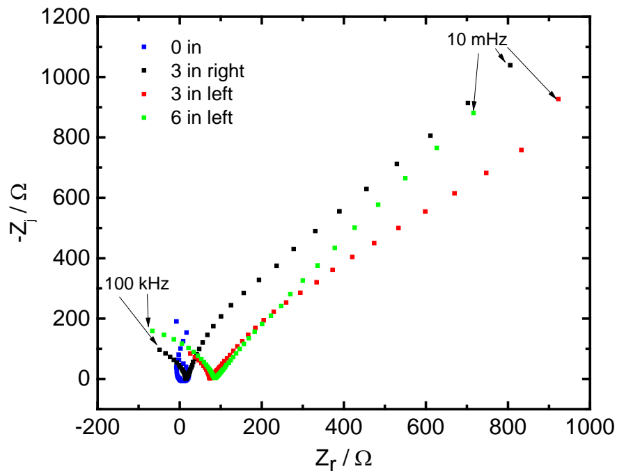
Figure 3. Three-point experimental impedance where the steel is the working electrode and the reference and counter electrodes are placed along the surface of the grout.
