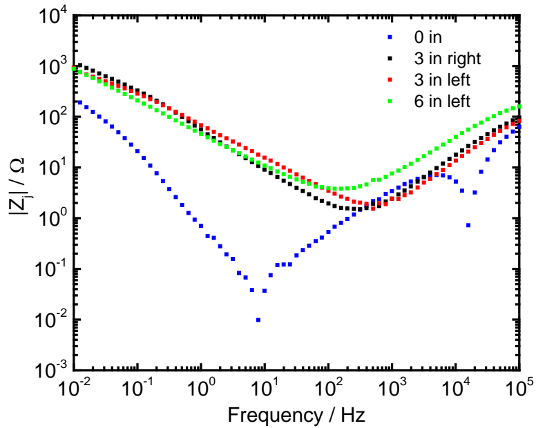
Figure 4. Three-point experimental imaginary impedance as a function of frequency where the steel is the working electrode and the reference and counter electrodes are placed along the surface of the grout.
