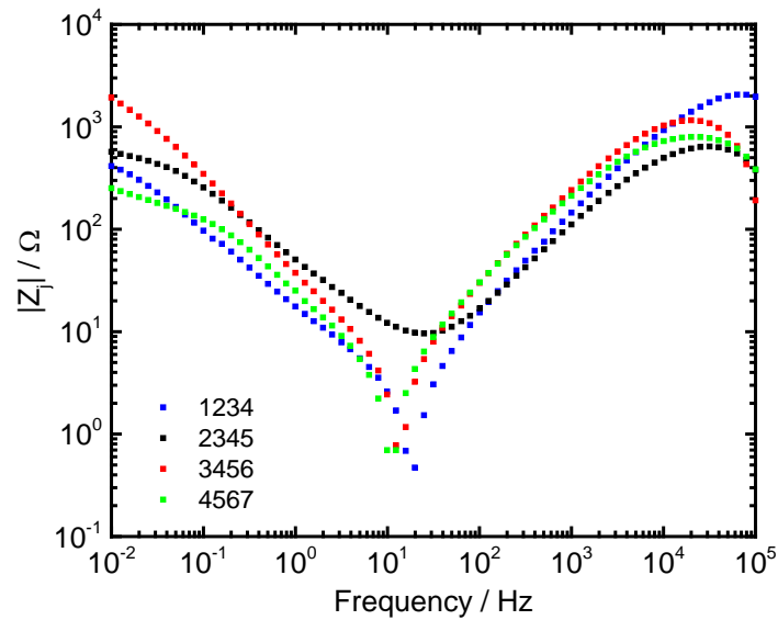
Figure 6. Four-point experimental imaginary impedance as a function of frequency where the outer two numbers in the legend indicate the positions of the current injection electrodes and the inner two numbers provide the positions of the potential-sense electrodes.
