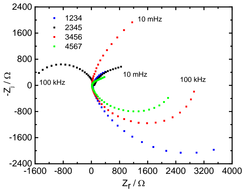
Figure 5. Four-point experimental impedance where the outer two numbers in the legend indicate the positions of the current injection electrodes and the inner two numbers provide the positions of the potential-sense electrodes.
