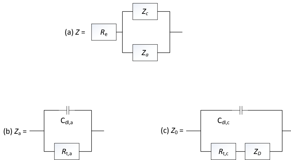
Figure 33. Equivalent circuit for (a) total impedance of the steel/simulated pore solution interface, (b) anodic impedance, (c) interfacial impedance of the micro-porous layer.
