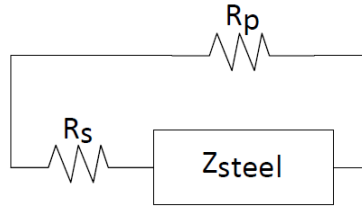
Figure 26. Circuit representation of indirect impedance.
