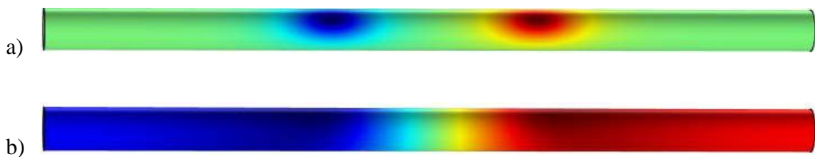
Figure 18. Simulated indirect impedance of a 2-ft model tendon containing one steel strand for a passive case and a locally corroding case of 4 cm at the midpoint of the steel strand. The centerline of the electrode array is 6 cm right of the centerline of the 2-ft tendon, and the working electrode is directly over the corroding area: a) impedance results; and b) schematic representation of the system geometry for a reference electrode spacing of 4 cm.
