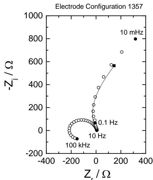
Figure 15. Simulated impedance results compared to the experimental results with an electrode configuration of 1357.
