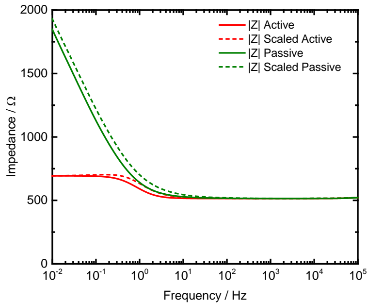
Figure 24. Magnitude of the impedance scaled by the potential ratio of two different reference points compared to the magnitude of the impedance measured with the second reference point as a function of frequency for the passive and active cases.
