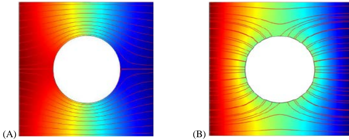
Figure 11. Current and potential distribution of a 1-cm-square grout model with a 0.25-cm radius steel placed in the center and current injecting electrodes placed on the vertical sides at the (A) low-frequency and (B) high-frequency limits.
