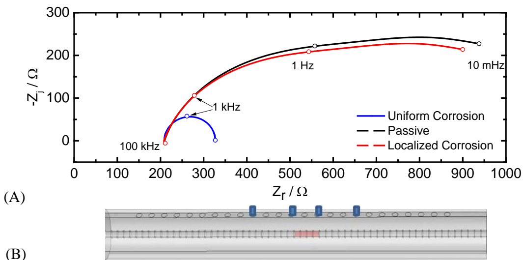
Figure 17. Simulated indirect impedance of a 2-ft model tendon containing one steel strand for a passive case, a locally corroding case of 4 cm at the midpoint of the steel strand, and a uniformly corroding steel: (A) impedance results; and (B) schematic representation of the system geometry for a reference electrode spacing of 4 cm.
