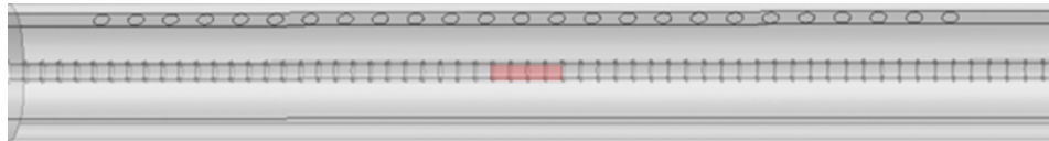
Figure 16. Tendon model with locally corroding section in the center of the steel.
