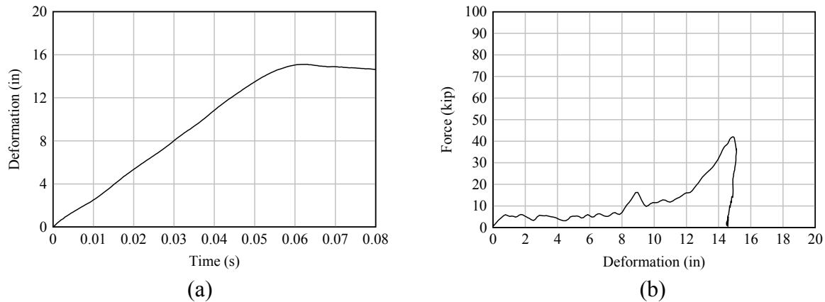
Figure 5.11 Crushable nose data from shear collar impact test: (a) Nose deformation vs. time; (b) Impact force vs. deformation
