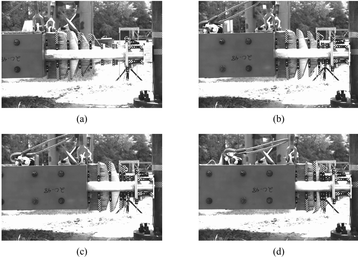
Figure 3.12 High speed video frames showing crushable nose deformation during rigid pole impact test
