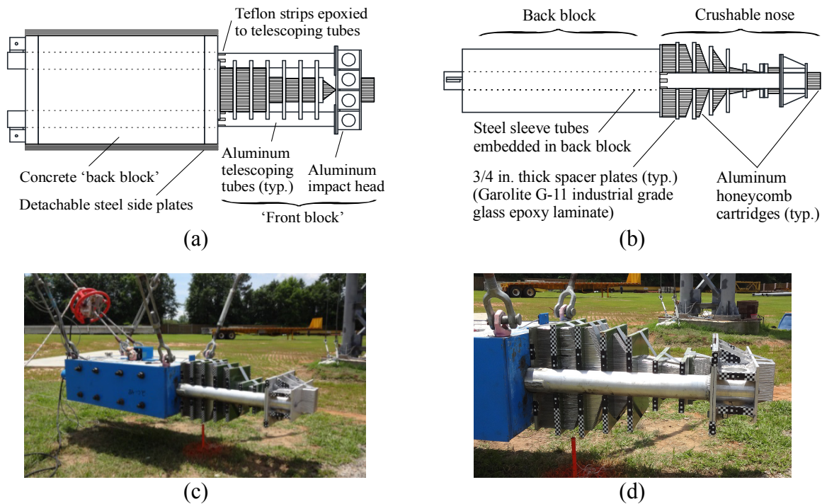
Figure 3.9 Crushable nose 1100C surrogate vehicle: (a) Plan view schematic; (b) Elevation view schematic; (c) Overview; (d) Crushable nose detail
