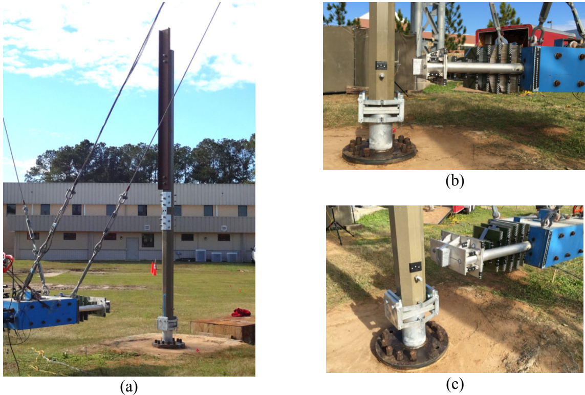
Figure 6.9 Head-on (0 deg.) impact test: (a) Fully-installed test article; (b) Elevation view; (c) Isometric view
