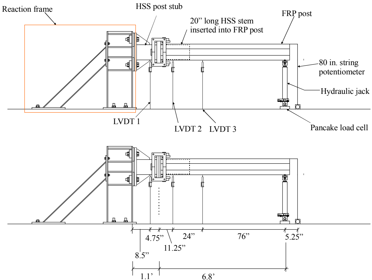
Figure 6.20 Schematic diagrams of static flexural test setup
