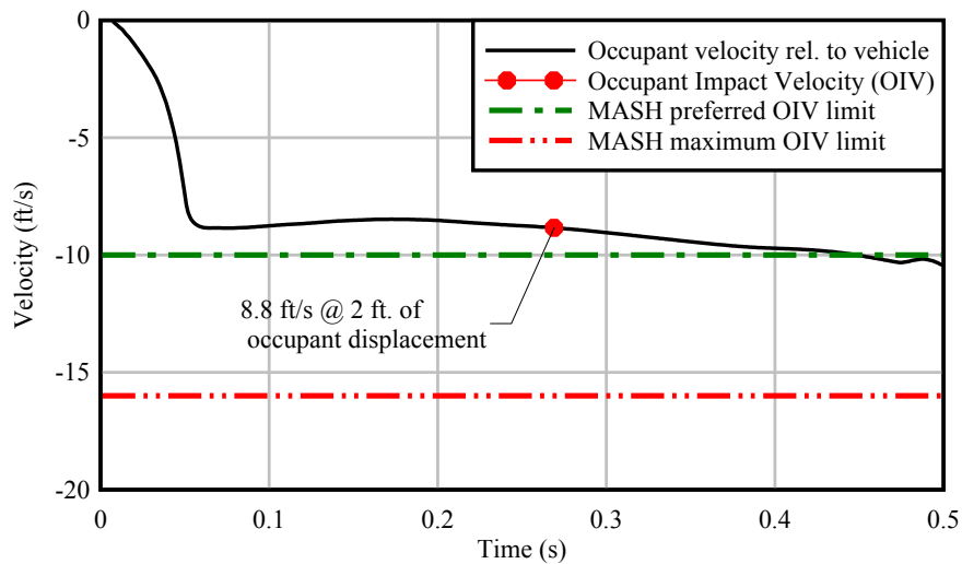
Figure 6.17 Occupant impact velocity (OIV) from oblique (25 deg.) 19-mph impact test
