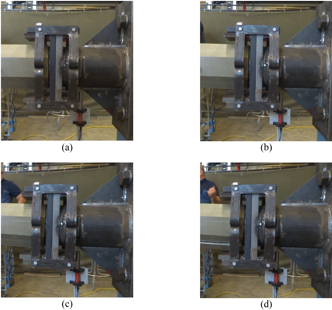
Figure 6.22 Deformations of FRP post, breakaway moment collar connection, and base stub during flexural testing
