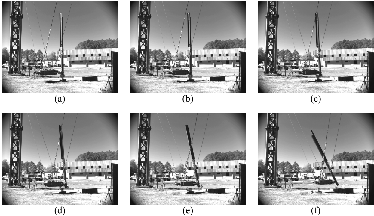
Figure 6.16 Wide angle high speed video frames from oblique (25 deg.) 19-mph impact test
