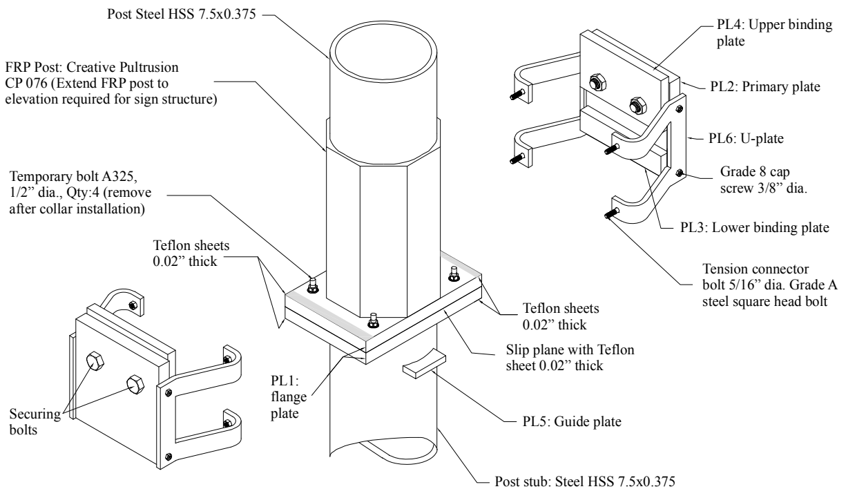
Figure 6.2 Exploded view of moment collar connection adapted for use with an FRP post
