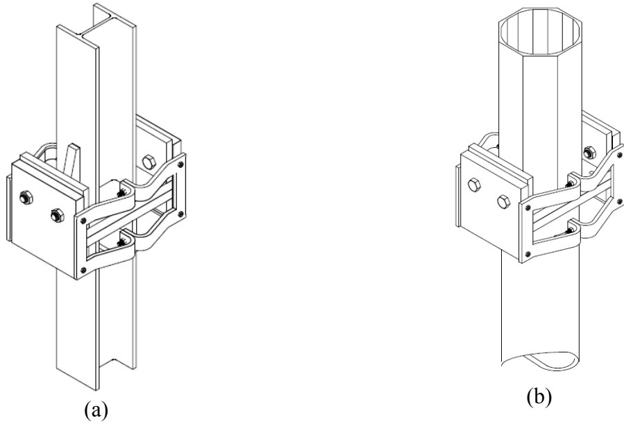
Figure 6.1 Adaptation of moment collar connection: (a) All-steel system with steel wide-flange post; (b) Hybrid system with steel HSS stem and FRP post
