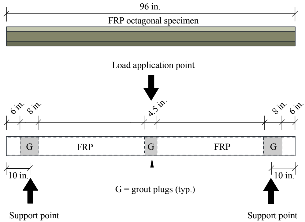
Figure 4.2 Schematic diagram of static three-point flexural test setup
