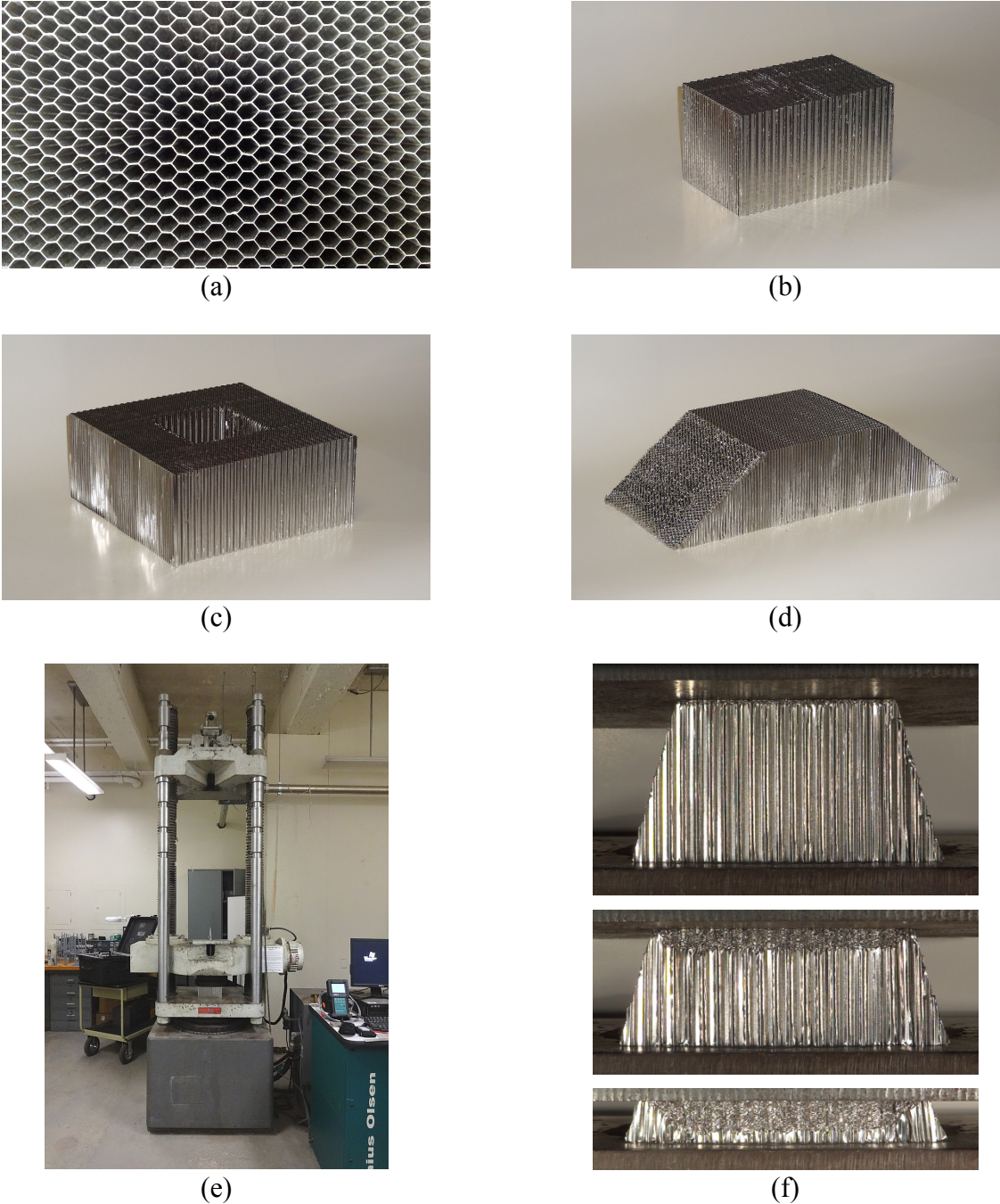
Figure 3.4 Aluminum honeycomb: (a) Hexagonal honeycomb cell structure; (b) Rectangular cartridge; (c) Rectangular cartridge with punch-out; (d) Trapezoidal cartridge; (e) Cartridge in test machine; (f) Compression test of tapered cartridge
