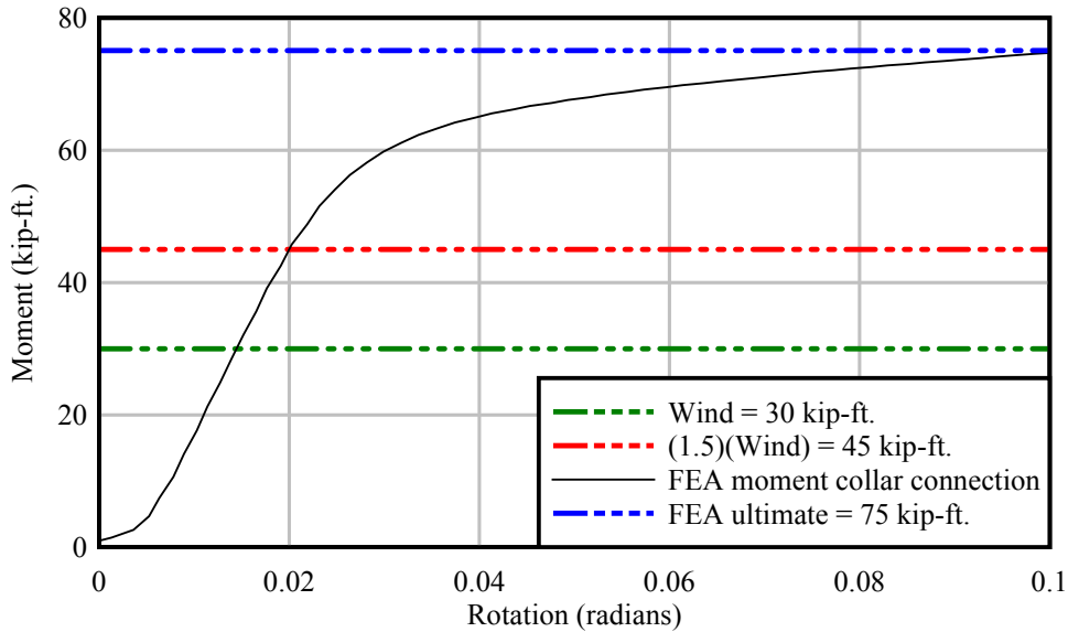
Figure 6.5 Pushover analysis results
