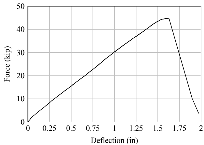
Figure 4.8 Static flexural test results
