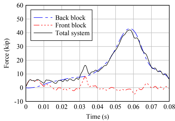
Figure 5.10 Contributing impact forces and total impact force
