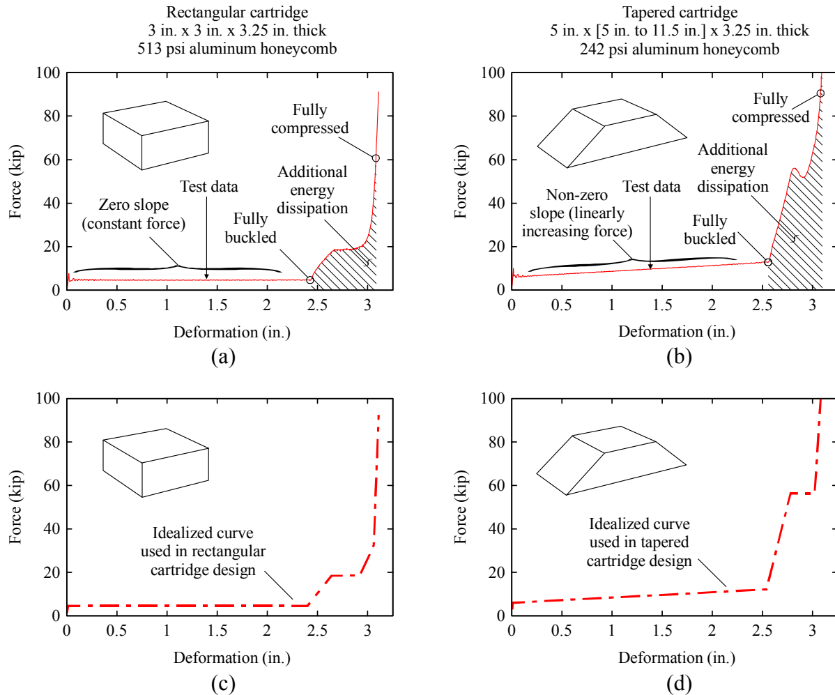
Figure 3.6 Compression test data and idealizations used in cartridge design: (a) Rectangular cartridge test data; (b) Tapered cartridge test data; (c) Rectangular cartridge idealization; (d) Tapered cartridge idealization
