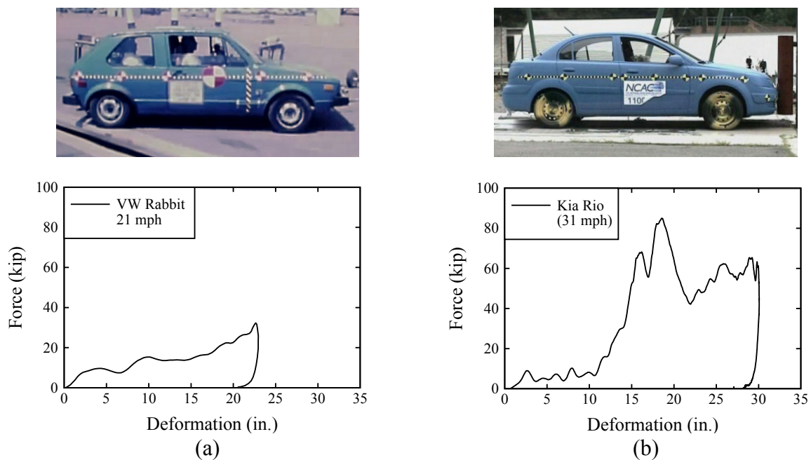
Figure 3.1 Production vehicles and force-deformation data: (a) 1979 VW Rabbit and 21-mph crash test results (National Highway Traffic Safety Administration and Federal Highway Administration); (b) 2006 Kia Rio and 31-mph crash test results (National Crash Analysis Center, Marzougui et al. 2011)
