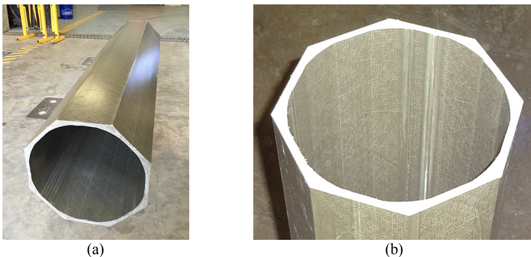
Figure 4.1 Octagonal CP076 FRP power pole manufactured by Creative Pultrusions: (a) Overview; (b) Detail of cross-sectional shape
