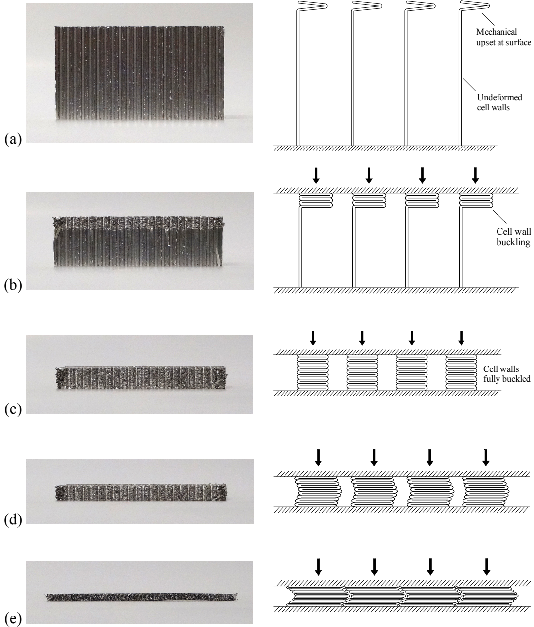
Figure 3.5 Stages of aluminum honeycomb compression behavior: (a) Surface of cartridge mechanically upset; (b) Cartridge buckling in progress; (c) Fully buckled stage; (d) Group buckling in progress; (e) Fully compressed stage
