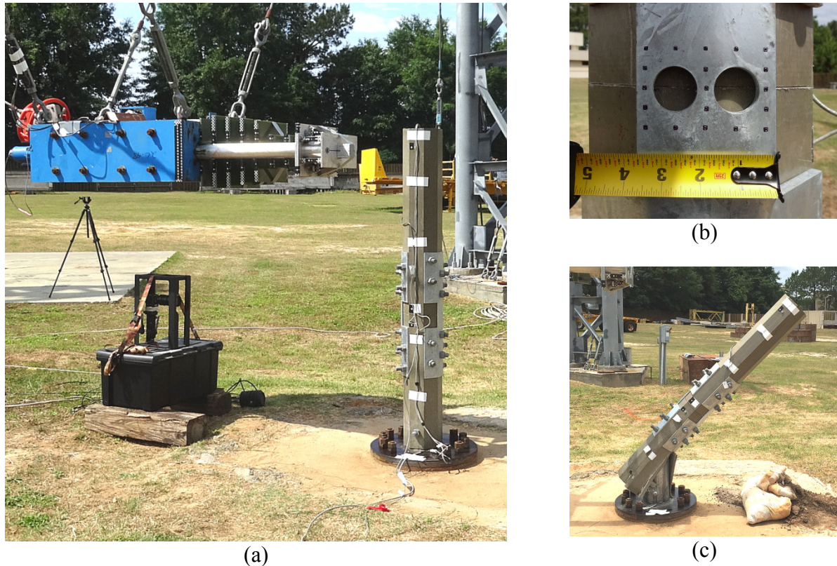
Figure 6.19 Fuse plate impact test: (a) Experimental test setup; (b) Fuse portion of plate with tracking points; (c) Flexural failure at base of FRP
