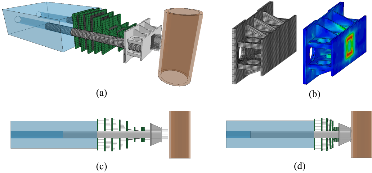
Figure 3.7 Finite element model of 1100C crushable nose surrogate vehicle: (a) Overview; (b) Impact head finite element mesh and typical stress results; (c) Prior to impact; (d) During impact
