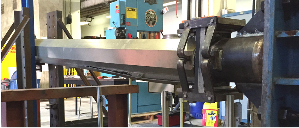
Figure 6.27 Longitudinal failure line along south side of FRP post
