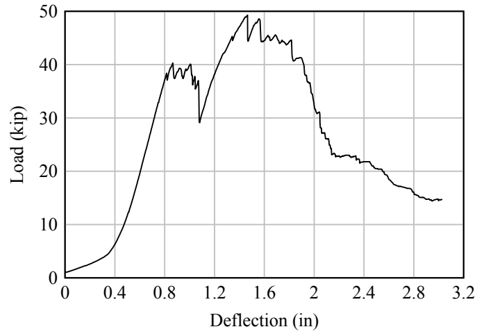
Figure D.4. Static double-shear test results
