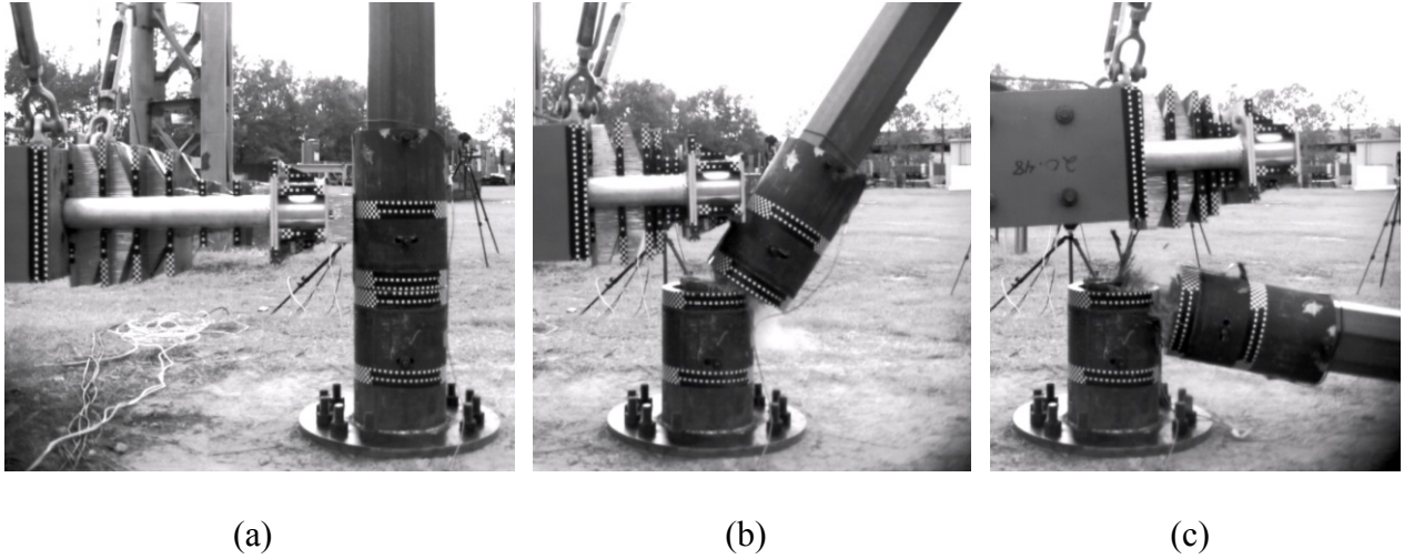
Figure 5.6 High speed video frames from impact testing of shear collar hybrid connection: (a) Initial contact; (b) Shearing of FRP; (c) Post breaks away from base
