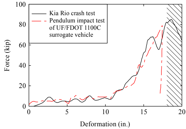
Figure 3.13 Comparison of production vehicle and surrogate vehicle response curves
