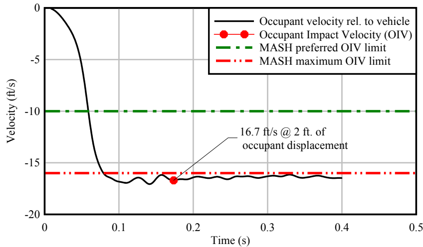
Figure 5.13 Occupant impact velocity (OIV) from head-on (0 deg.) 19 mph impact test
