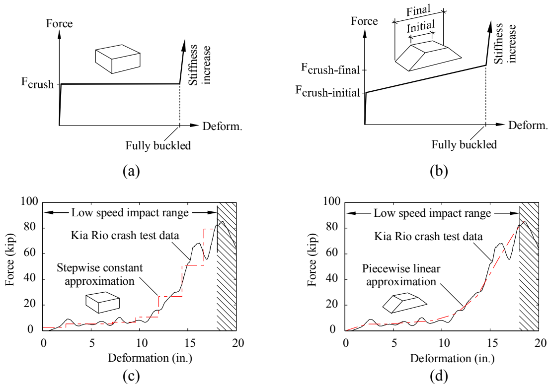
Figure 3.3 Simplified description of production vehicle force-deformation curve approximation: (a) Rectangular cartridge behavior; (b) Tapered (trapezoidal) cartridge behavior; (c) Stepwise constant approximation; (d) Piecewise linear approximation
