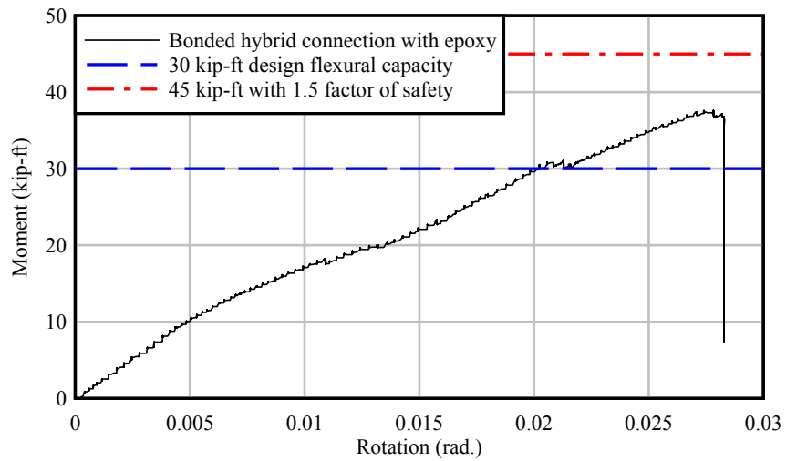
Figure 6.29 Results from static flexural capacity test of bonded (epoxied) hybrid system
