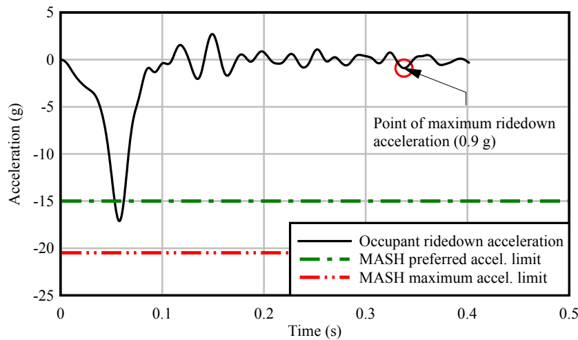
Figure 5.14 Occupant ride-down acceleration (ORA) from head-on (0 deg.) 19 mph impact test
