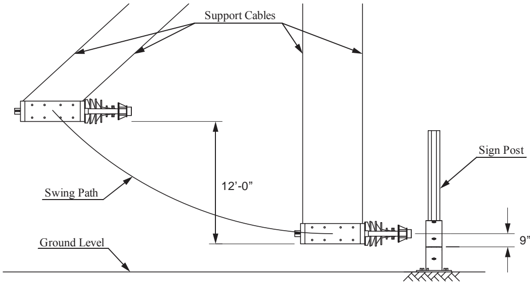
Figure 5.4 Schematic diagram of impact test for shear collar connection concept
