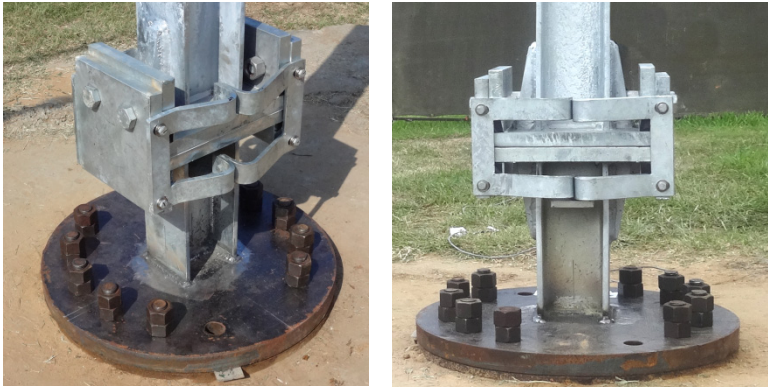
Figure 1.6 Low capacity moment collar breakaway connection developed in FDOT project BDV31-977-24
