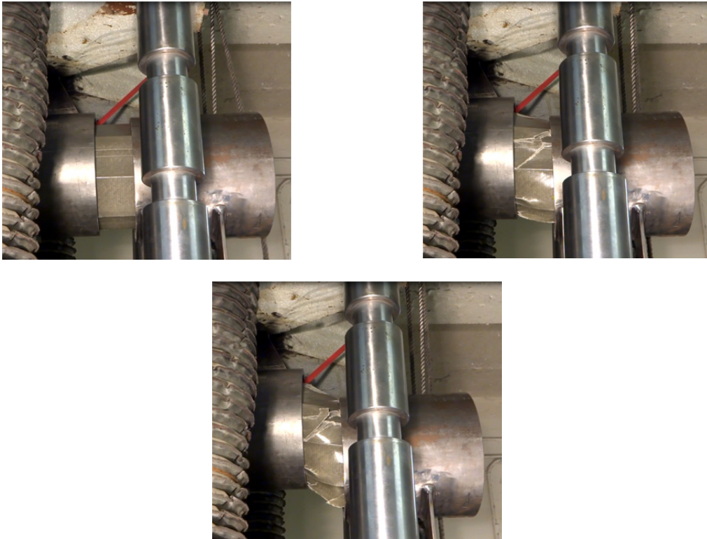
Figure D.3. Section deformation during static double-shear test
