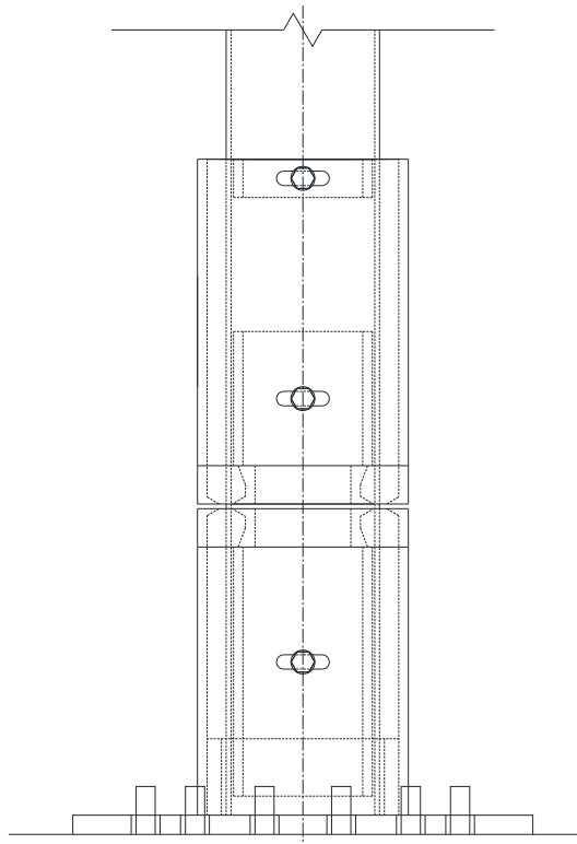
Figure 5.2 Shear collar hybrid breakaway system concept
