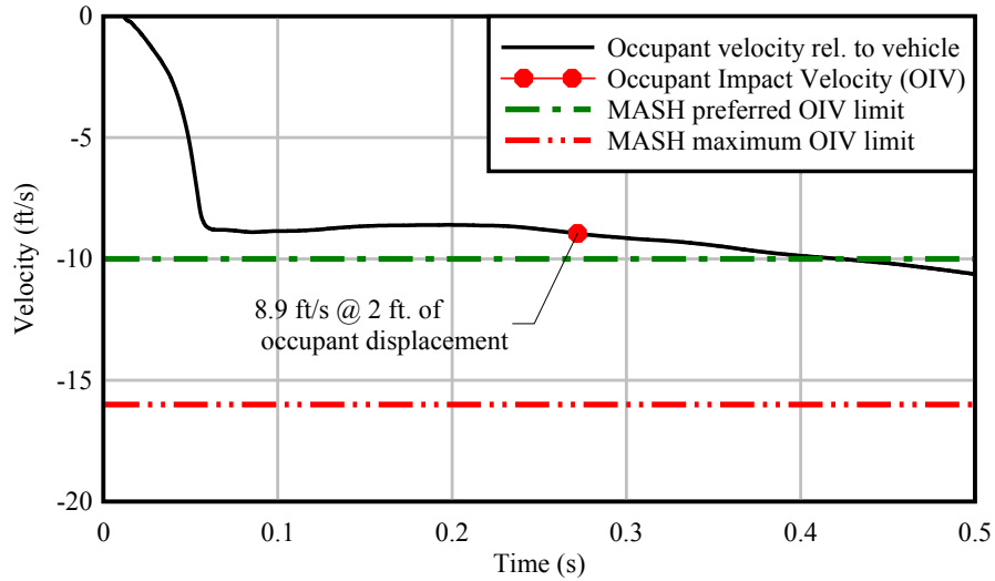
Figure 6.12 Occupant impact velocity (OIV) from head-on (0 deg.) 19-mph impact test
