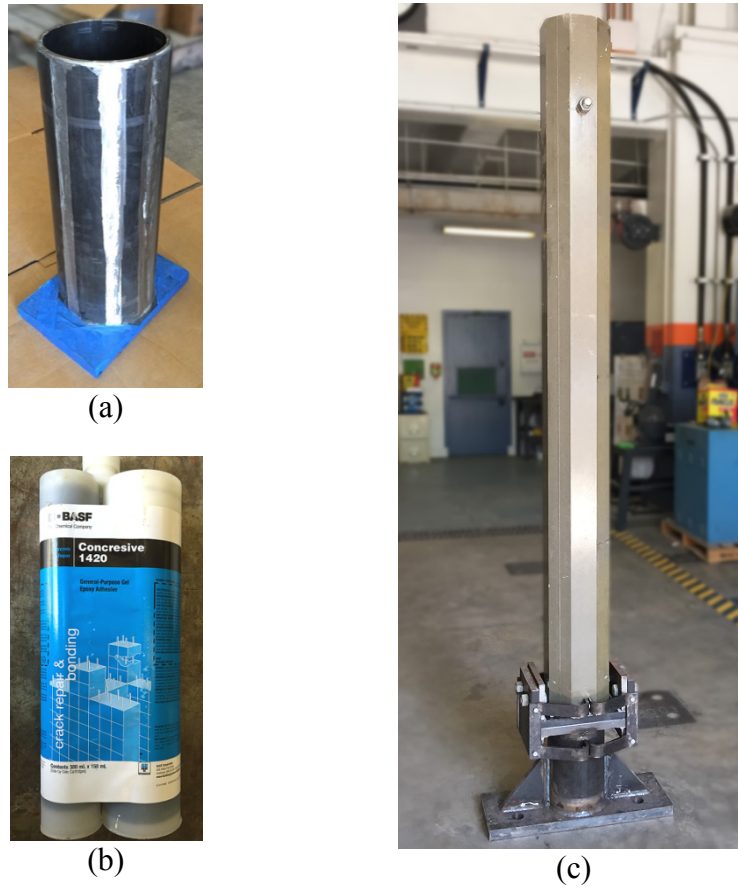
Figure 6.24 Preparation and installation of bonded test article: (a) Steel HSS stem chamfered at end and ground flat along eight (8) lines in accordance with inner geometry of FRP CP076 post; (b) ‘Concessive’ two-part epoxy used to bond steel stem to FRP post; (c) HSS stem epoxied into FRP post and attached to stub base with moment collar
