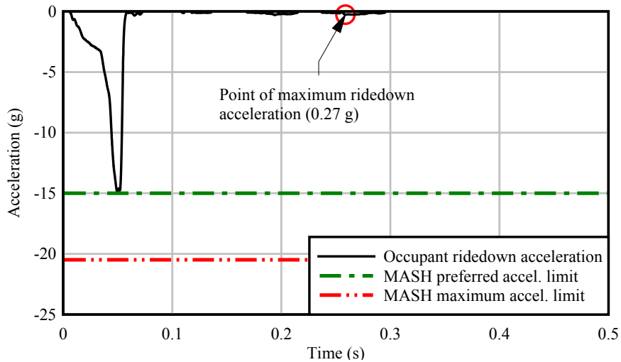
Figure 6.13 Occupant ride-down acceleration (ORA) from head-on (0 deg.) 19-mph impact test
