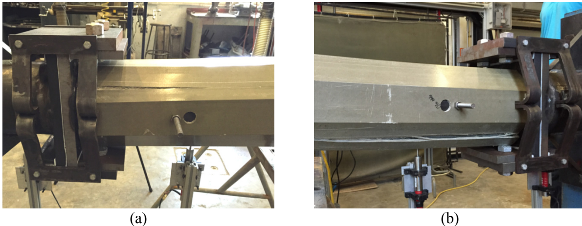
Figure 6.23 Longitudinal failure lines: (a) North side of FRP post; (b) South side of FRP post
