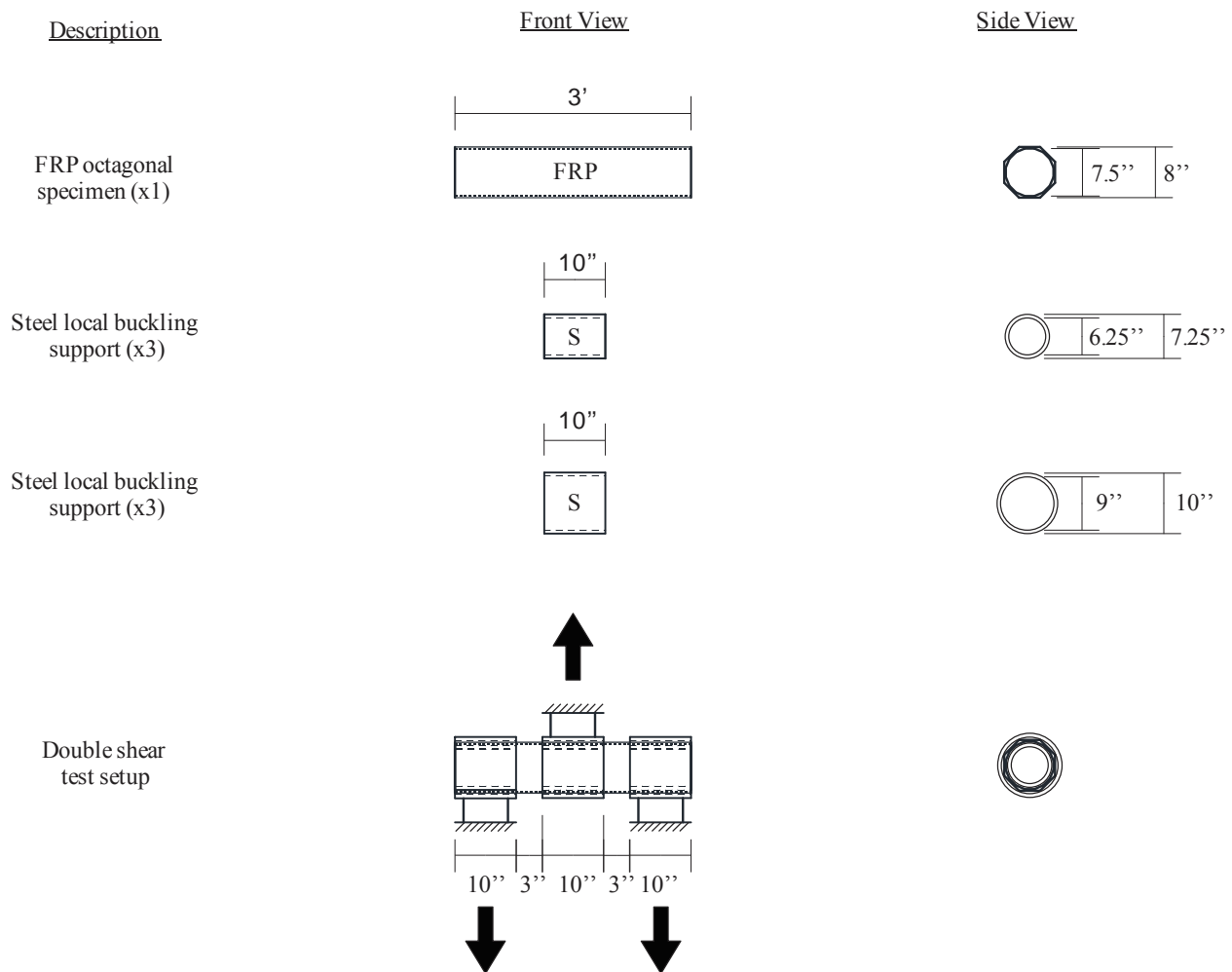
Figure D.1. Schematic diagram of static double-shear test setup
