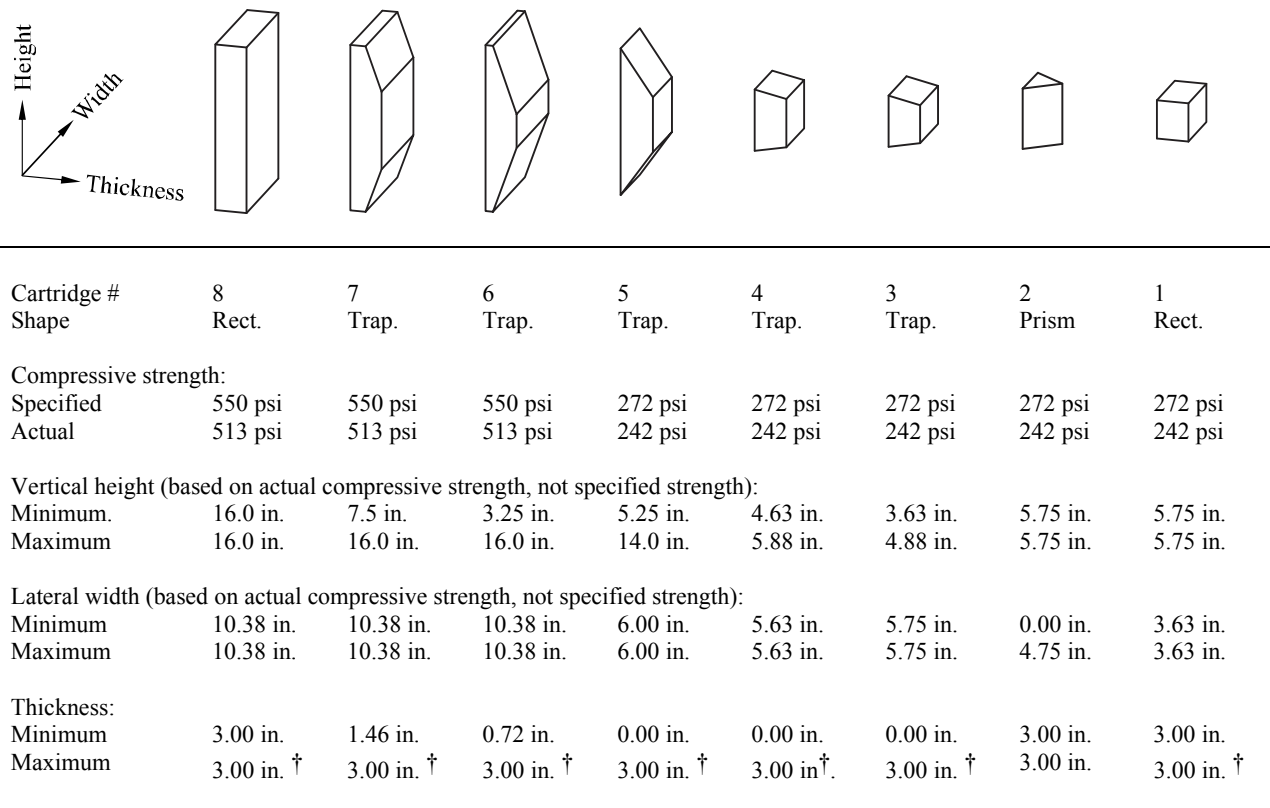
Figure 3.10 Aluminum honeycomb cartridge characteristics
