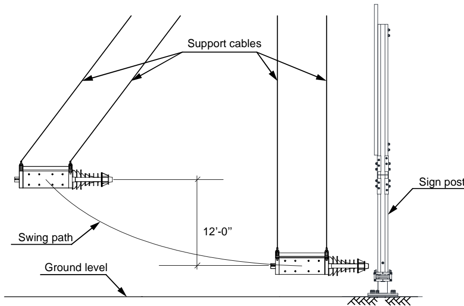
Figure 6.7 Schematic diagram of impact test
