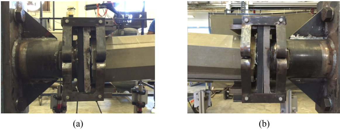
Figure 6.28 Longitudinal failure lines: (a) North side of FRP post; (b) South side of FRP post
