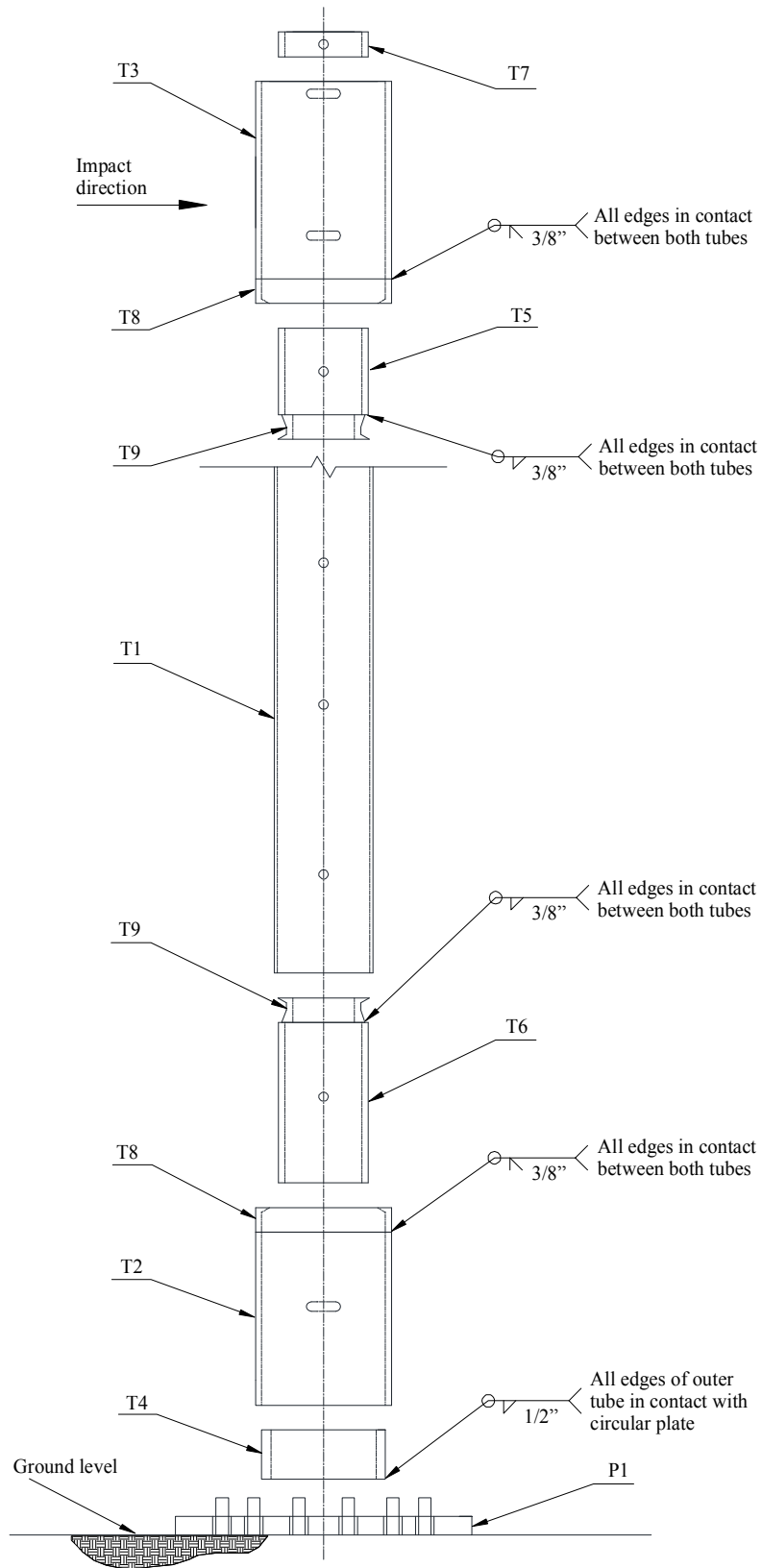
Figure 5.1 Hybrid breakaway system exploded view
