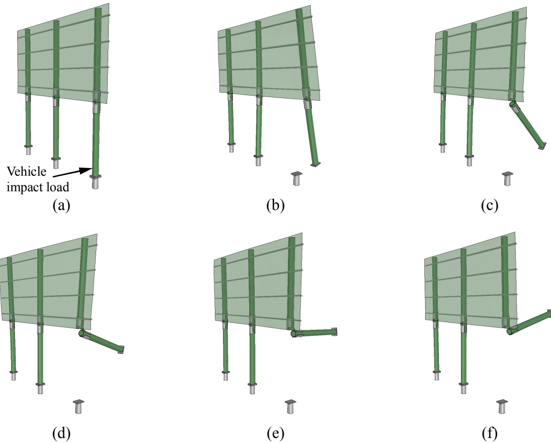
Figure 1.3 Intended system behavior of a three-post sign structure: (a) Impact load from vehicle (not shown) is applied to right most column; (b) Breakaway base connection disengages; (c) Fuse plate at top of lower segment ruptures; (d)-(e) Lower post segment rotates out of path of vehicle, but remains attached to the rest of the structure
