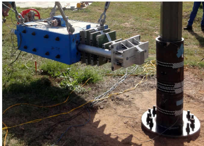
Figure 5.5 Impact test for shear collar connection concept
