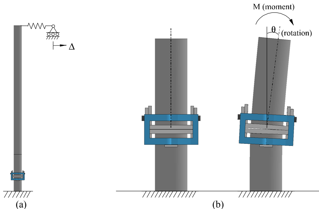
Figure 6.3 Finite element pushover analysis: (a) Overall model showing location of prescribed displacement; (b) Relationship between moment and section rotation
