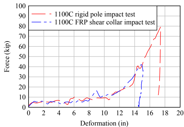
Figure 5.12 Comparison of vehicle force-deformation data from breakaway shear collar test and rigid pole test
