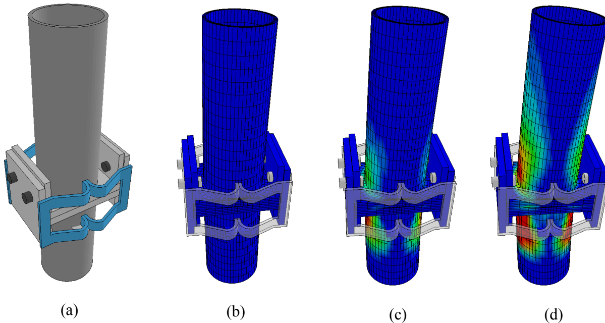
Figure 6.4 Plastic strains from pushover analysis of moment collar with HSS stem: (a) Unstressed model; (b) Initial loading; (c) Yielding of HSS stem; (d) Maximum flexural capacity (Legend: blue = \epsilon_p = 0 \text{ in/in} ; red = \epsilon_p = (10)\epsilon_Y )
