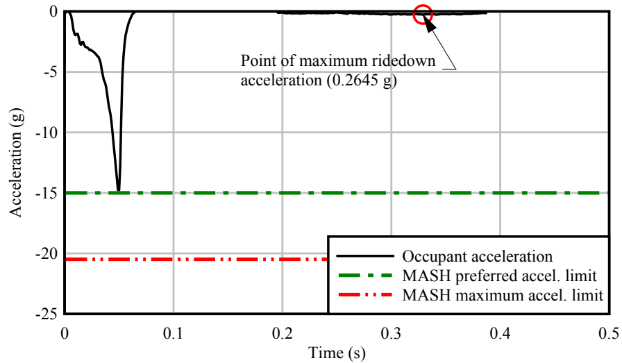
Figure 6.18 Occupant ride-down acceleration (ORA) from oblique (25 deg.) 19-mph impact test
