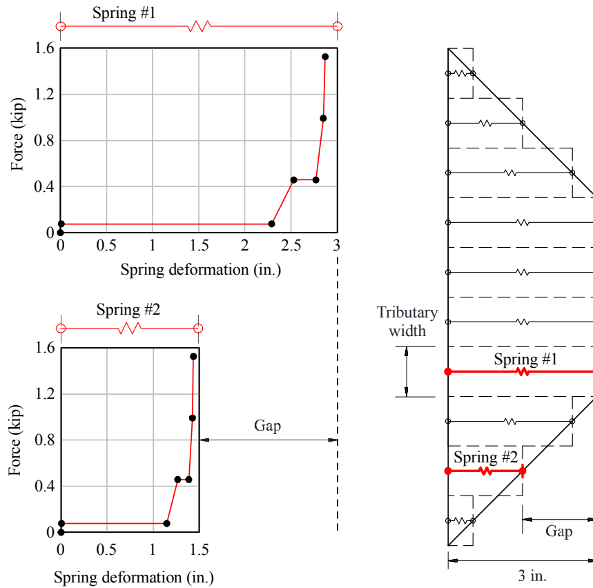
Figure 3.8 Use of nonlinear springs to efficiently model the compression behavior of an aluminum honeycomb cartridge
