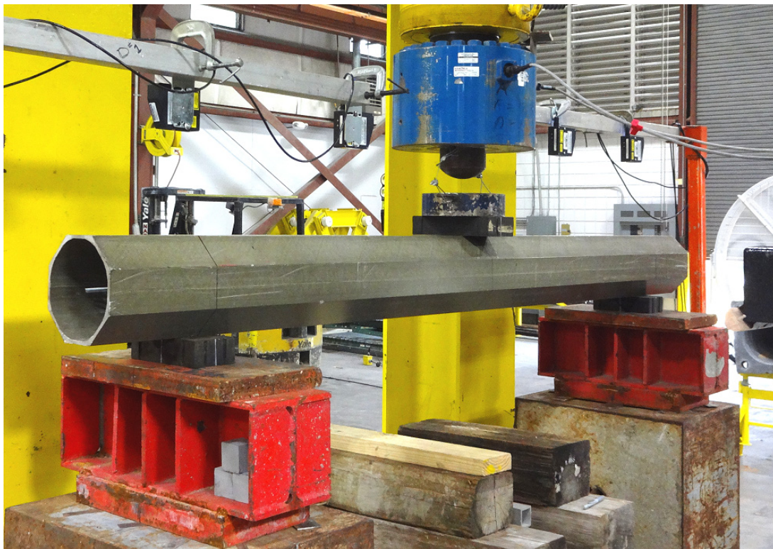
Figure 4.3 Flexural testing of CP076 FRP composite post at FDOT Structures Research Center
