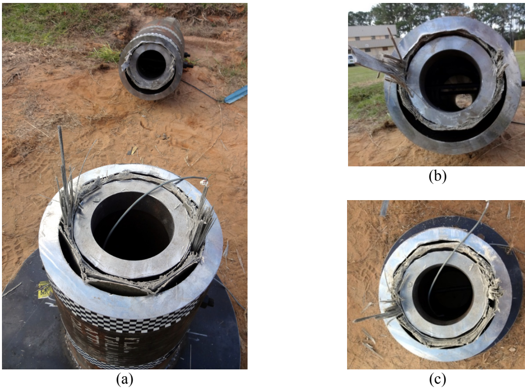
Figure 5.7 Condition of FRP post and cutting edges after impact test: (a) Overview with lower portion (stub base) in foreground and sheared upper post in background; (b) Upper portion of post; (c) Lower portion (stub base) of post
