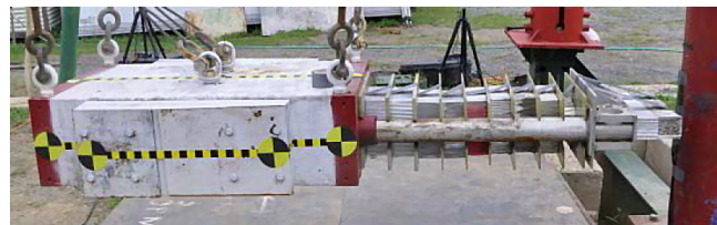
Figure 3.2 NCAC-FOIL 1100C crushable nose impactor (National Crash Analysis Center, Marzougui et al. 2013)
