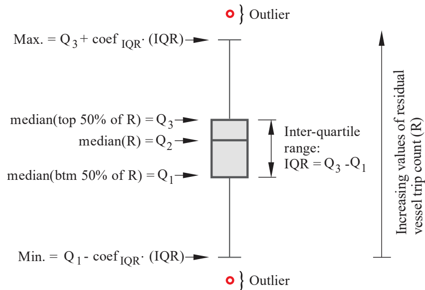
Figure 4.2 Illustration of the ‘box-and-whiskers’ outlier detection approach
