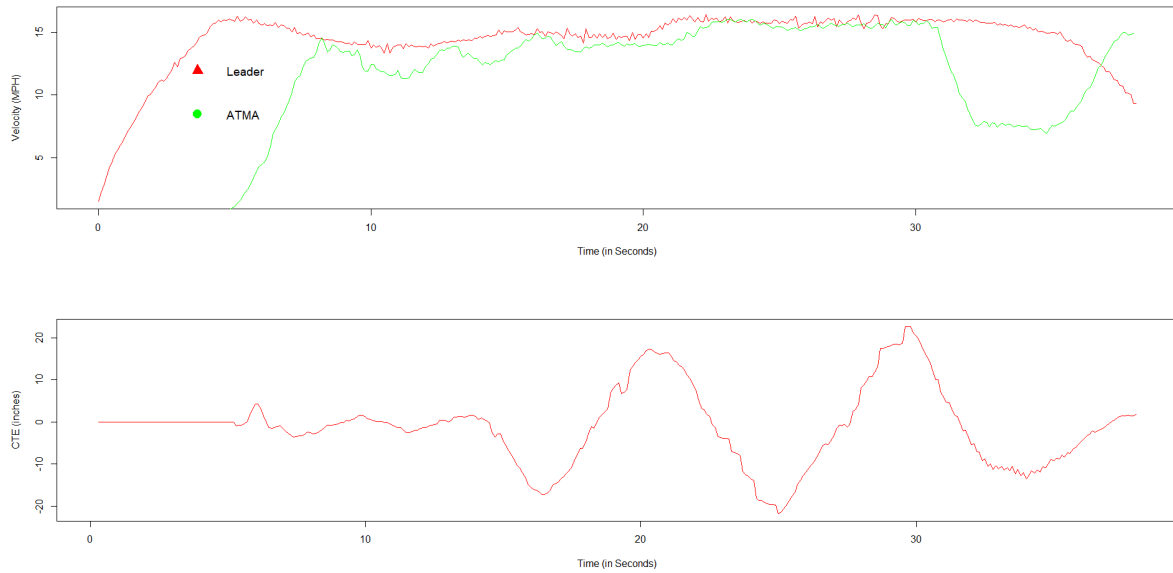
Figure 6-42. Test Case 7, Run 7: follower truck velocity (top); cross track error (CTE) (bottom)
