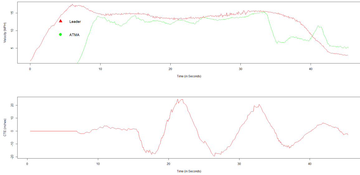
Figure 6-41. Test Case 7, Run 6: follower truck velocity (top); cross track error (CTE) (bottom)
