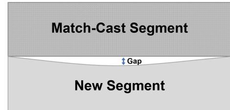
Bowing distortion caused by the heat of hydration in the new segment.
