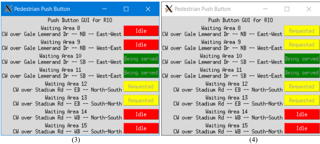
Figure 4-3: Pedestrian push-button GUI with (3) one and (4) two walk light requests.
