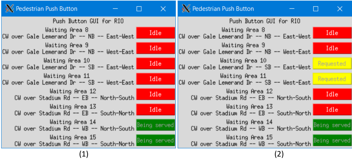
Figure 4-2: Pedestrian push-button GUI (1) idle and (2) with one walk light request.
