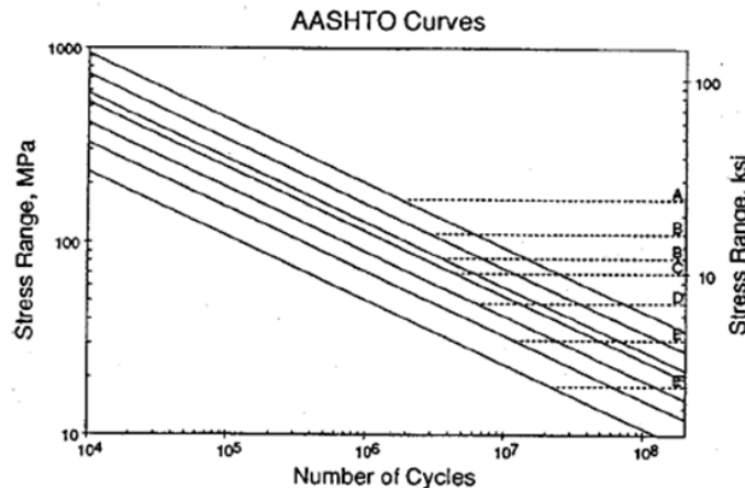
Figure 2-2. AASHTO fatigue strength categories.[6]
