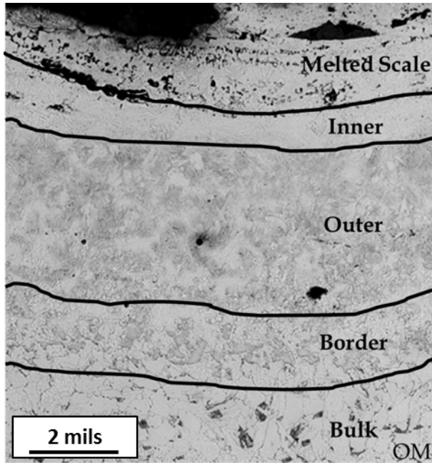
Figure 4-10. Enlarged micrograph of the HAZ caused by the plasma mark.
