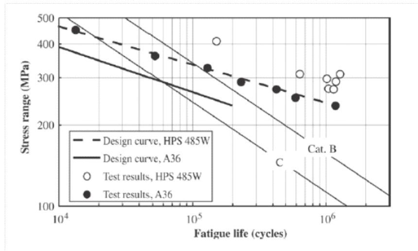
Figure 2-5. Fatigue life data from conventional (labeled A36) and HPS 70W (labeled HPS 485W) weathering steels with drilled holes represented as solid and open circles, respectively.[20]
