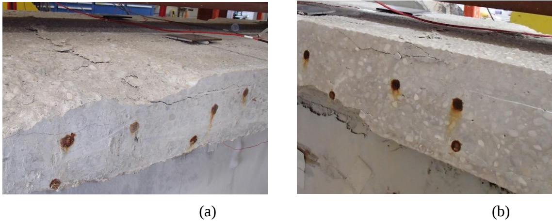
Figure 196—Crushing of concrete in compression (Girder 4-3): (a) west elevation (b) east elevation
