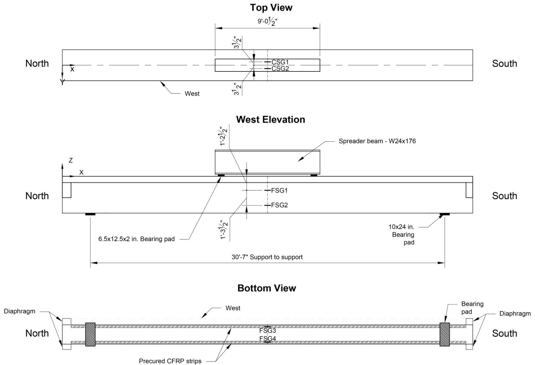
Figure 170—Instrumentation plan indicating the strain gage locations for girders with FRP
