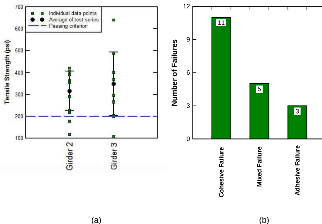
Figure 237—Direct pull-off testing: (a) tensile strength comparison and (b) failure modes
