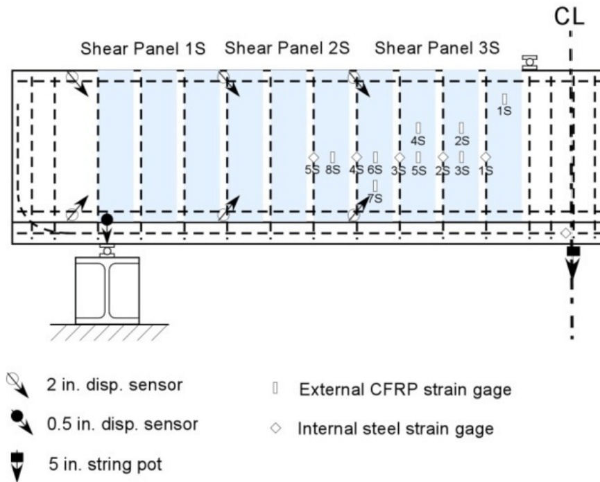
Figure 57—Typical instrumentation plan (Higgins et al., 2009)
