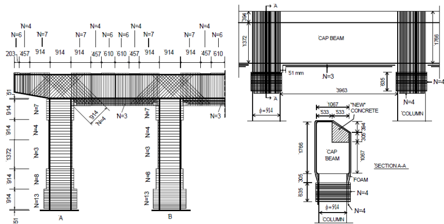
Figure 53—Typical bent CFRP strengthening scheme; N = number of CFRP layers (Pantelides et al., 2006)
