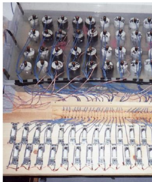
Figure 274—Spainhour and Wootton (2008): Test configuration
