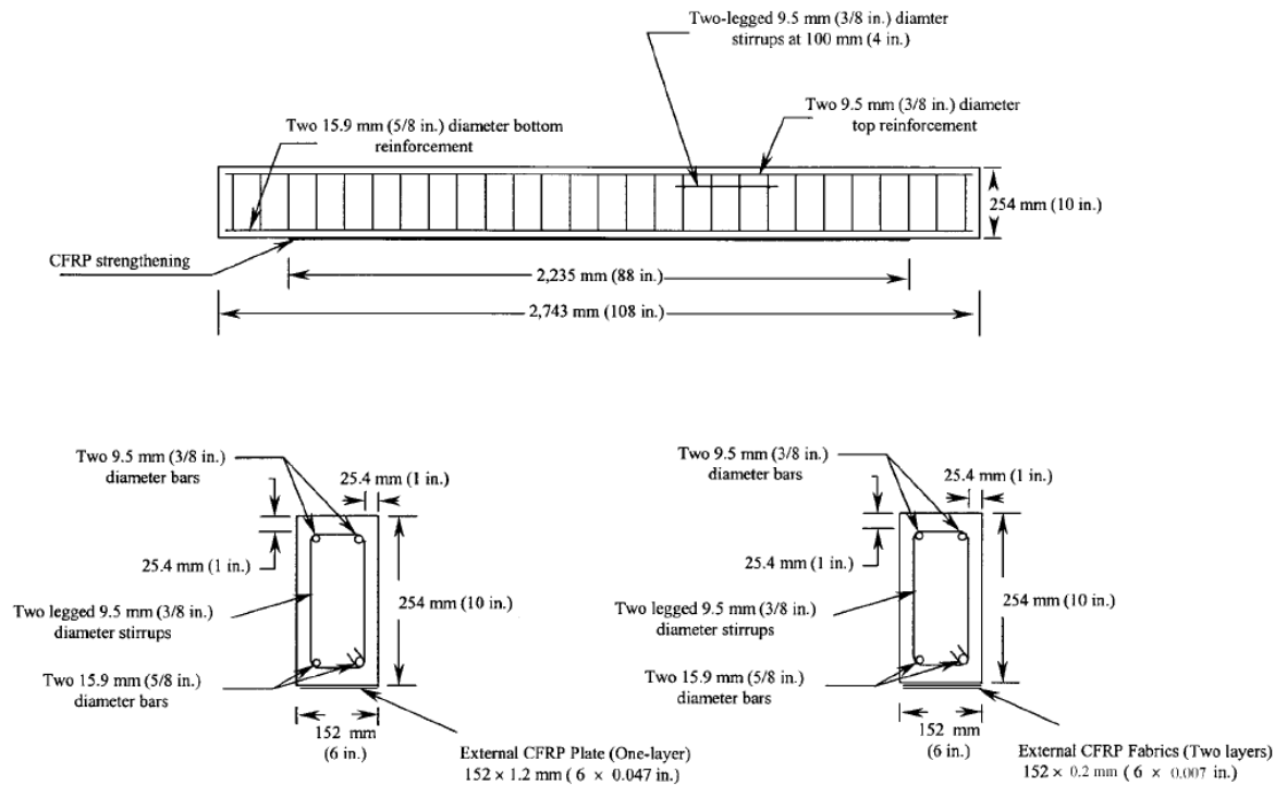
Figure 12—Drawings of test specimen (Grace and Singh, 2005)
