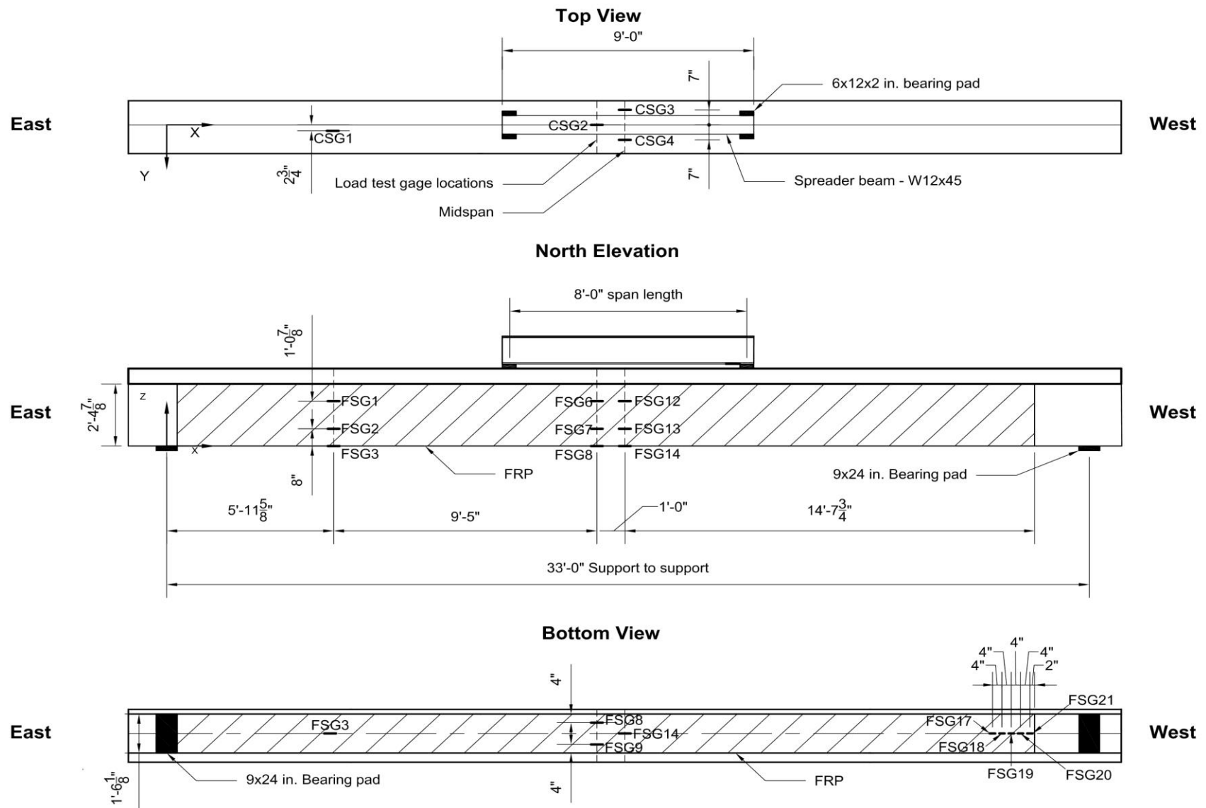
Figure 108—Girder #1 – Instrumentation plan representing the locations for the strain gages
