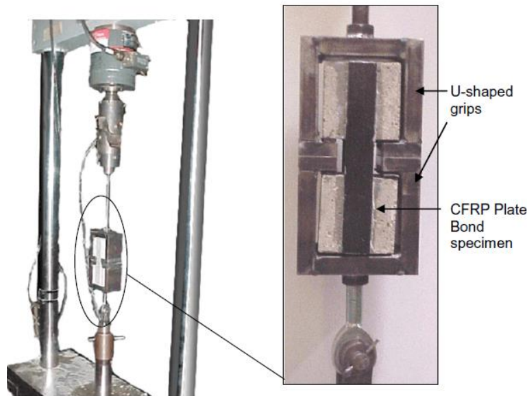
Figure 22—Bond test setup
