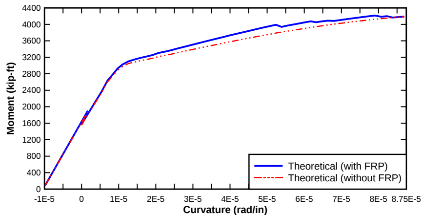
Figure 260—Girder 3 comparison of the theoretical ultimate capacity with and without FRP
