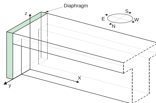
Figure 84—Axisymmetric view of east end of typical girder with specified coordinate system location
