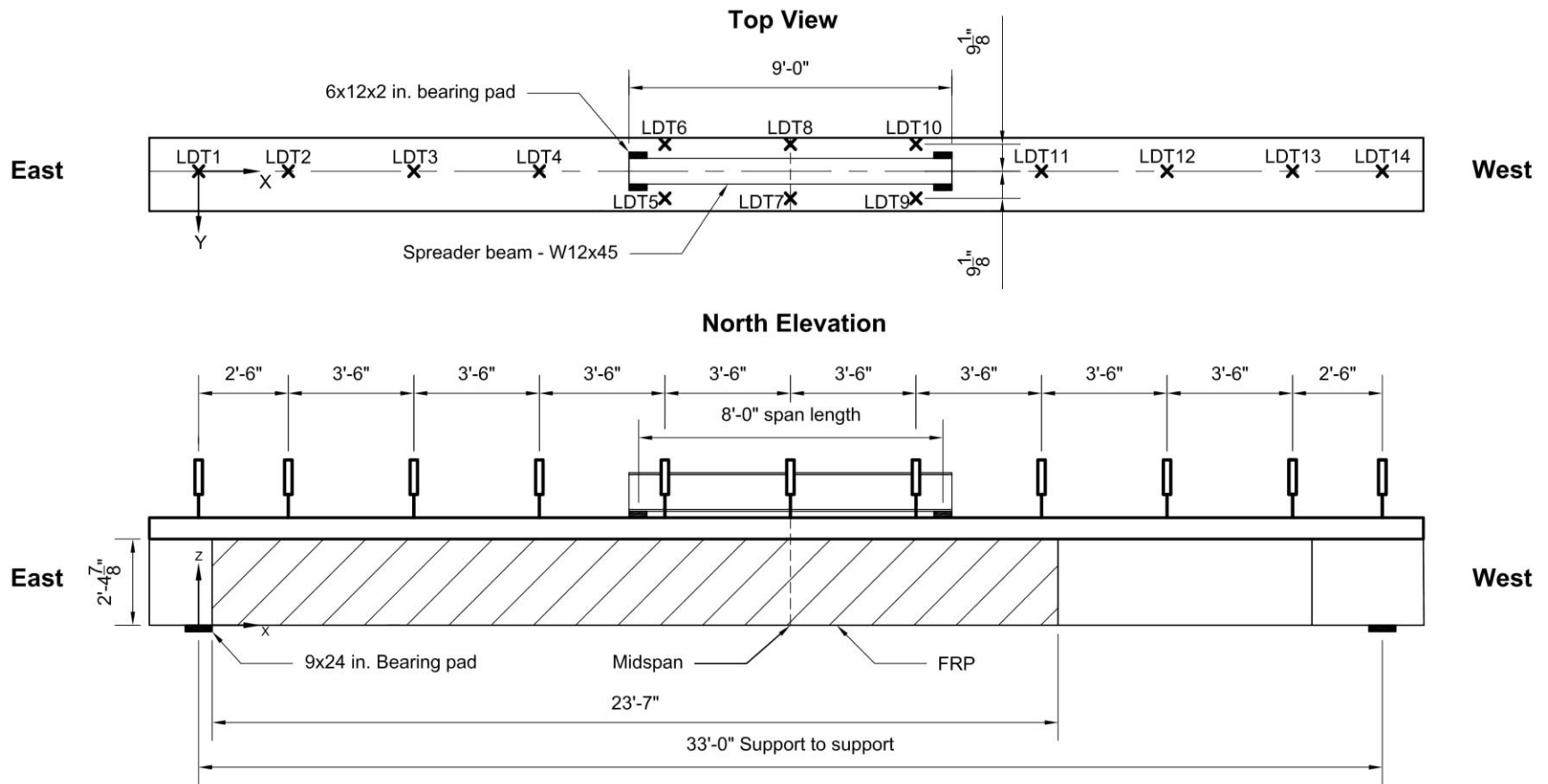
Figure 107—Girder #2 – Instrumentation plan representing the locations for the laser displacement transducers
