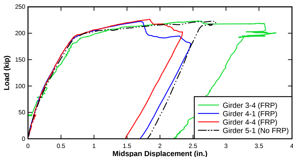
Figure 171—Load-displacement of exterior test girders
