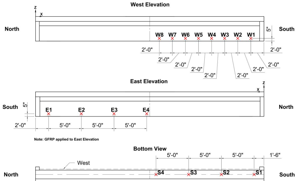
Figure 142—Potential testing locations for Girder 3-1
