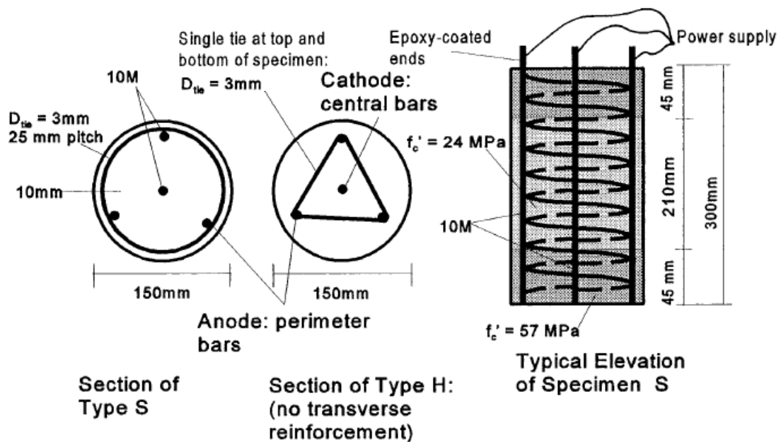
Figure 273—Pantazopoulou et al. (2001): typical specimen geometry
