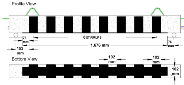
Figure 35—Wrapping scheme 3 (Davalos et al., 2012)
