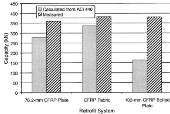
Figure 42—Comparison between measured and calculated capacity as per ACI 440
