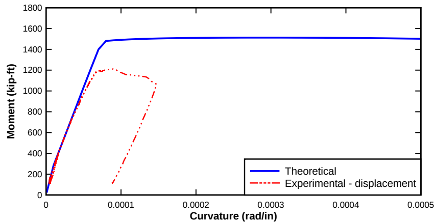
Figure 209—Moment curvature of Girder 5-2
