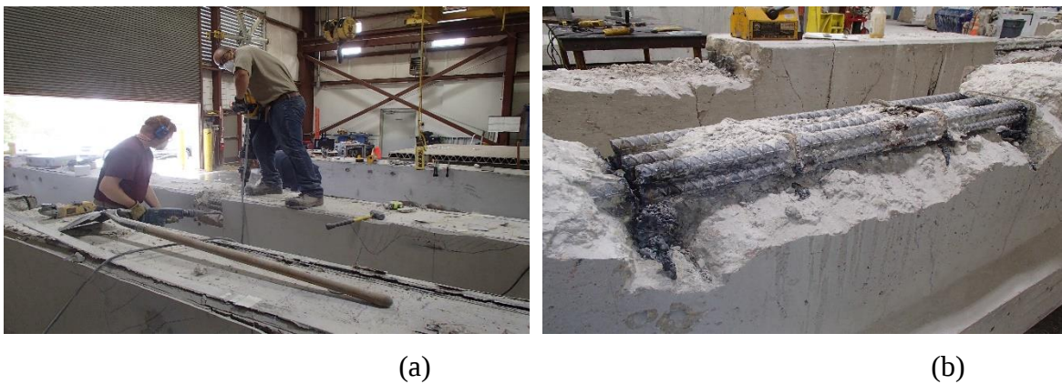
Figure 216—(a) Jackhammering concrete surrounding the reinforcing bars and (b) bridge girder in upside-down position with steel reinforcement exposed
