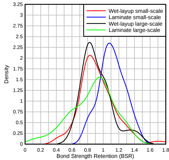
Figure 30—Comparison of distributions for different groups of data from literature
