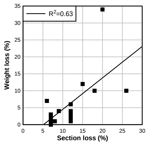
Figure 148—Correlation between weight loss and section loss
