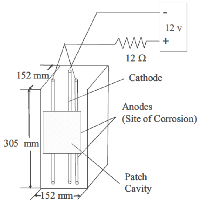
Figure 272—Nossoni and Harichandran (2010): Specimen design
