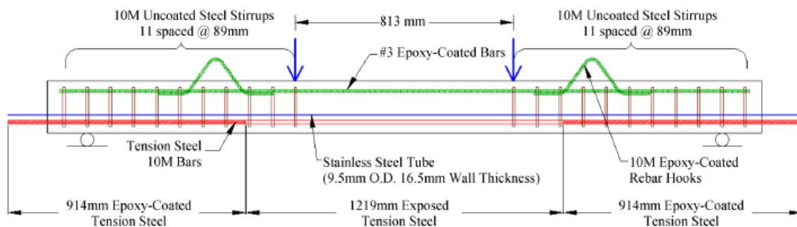
Figure 31—Substrate repair method study test specimen (Davalos et al., 2012)
