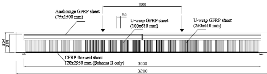
Figure 271—Masoud and Suodki (2006): A schematic for FRP repair schemes I and II
