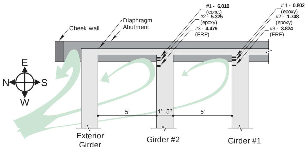
Figure 129—Wind and wave action on bridge girders near abutment (plan view)
