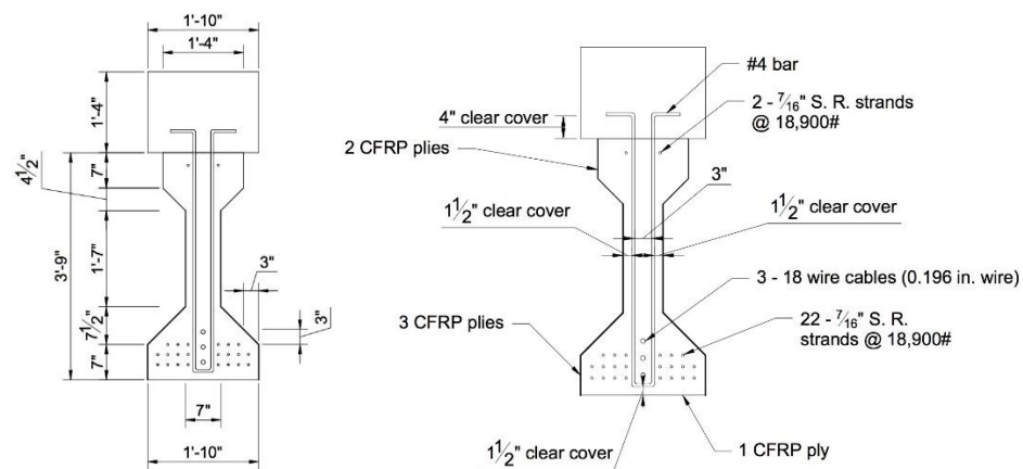
Figure 228—Typical beam section (a) original and (b) with CFRP repair
