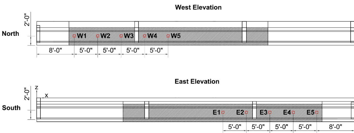
Figure 236—Direct pull-off testing locations for Girder 3
