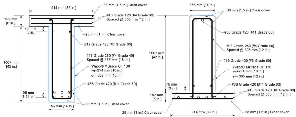
T Specimen (Typical)
