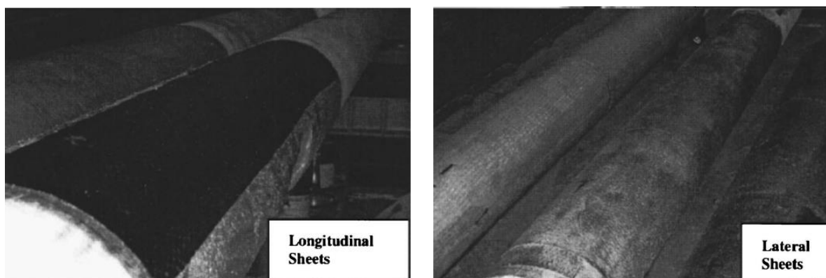
Figure 37—Longitudinal flexure sheets and lateral confinement sheets application (Maaddawy et al., 2006)
