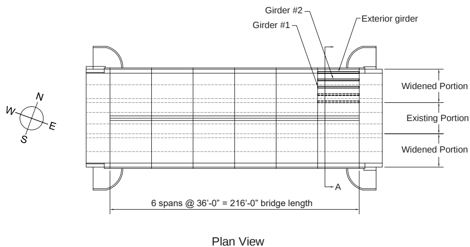
Figure 78—Plan view of Indian River Bridge
