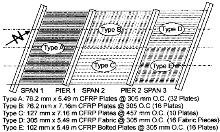
Figure 39—Locations of FRP repair systems (Shahrooz and Boy, 2004)
