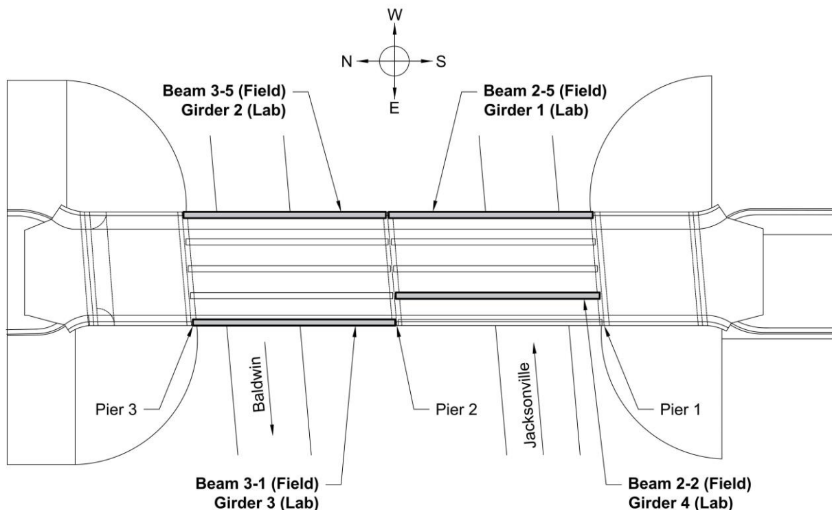
Figure 226—Plan view of Chaffee Road Bridge with salvaged girders identified
