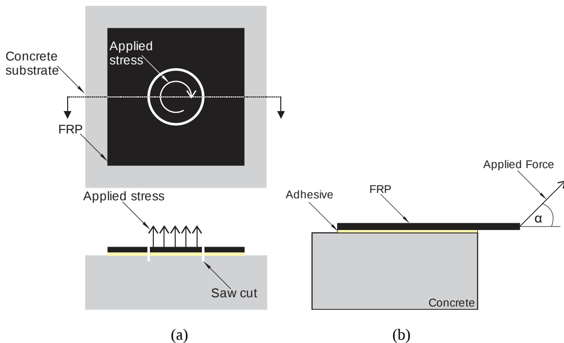
Figure 3—(a) Direct pull-off (bottom) and direct torsion (top) test; and (b) direct shear ( \alpha=0^\circ ), peel ( \alpha=90^\circ ) and mixed-mode ( 0^\circ < \alpha < 180^\circ ) test
