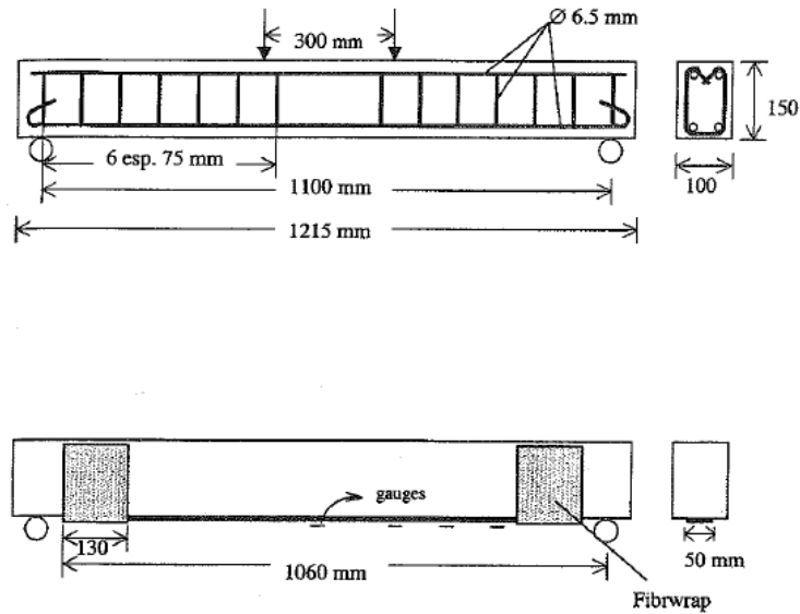
Figure 9—Four-point bending test setup (Beaudoin et al., 1998)
