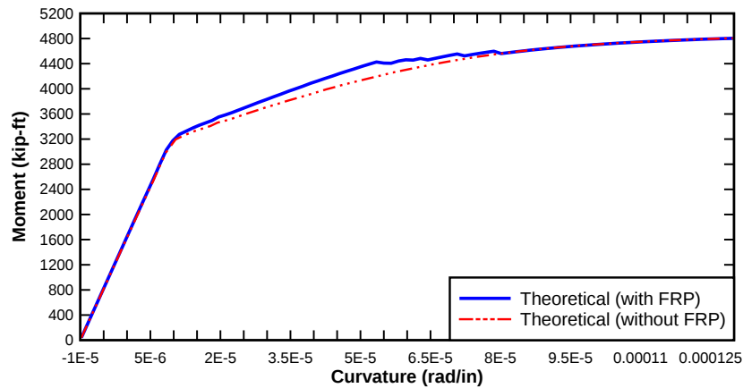
Figure 259—Girder 2 comparison of the theoretical ultimate capacity with and without FRP
