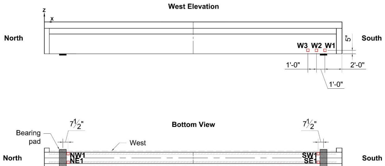
Figure 154—Direct pull-off testing locations for interior girders
