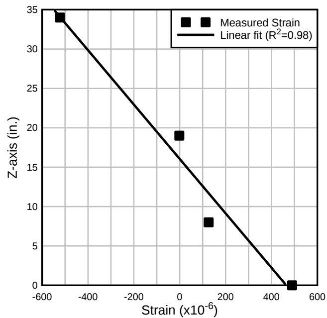
Figure 114—Typical strain profile along the girder depth
