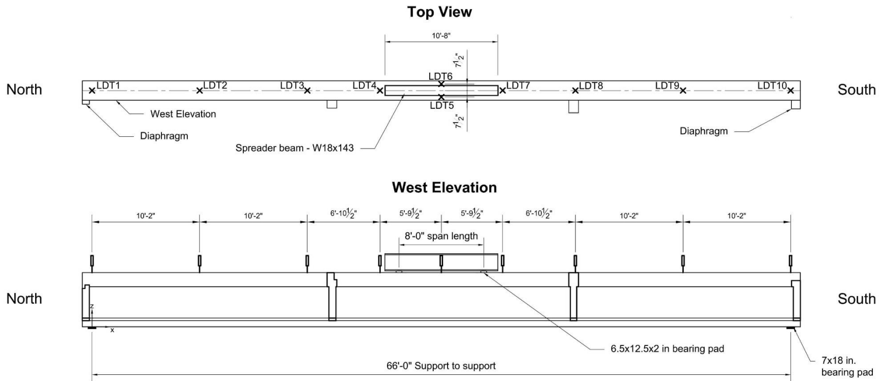
Figure 239—Typical instrumentation plan representing the locations for the laser displacement transducers
