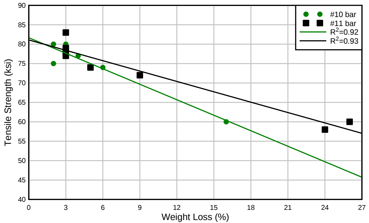
Figure 98—Correlation between tensile strength and measured weight loss
