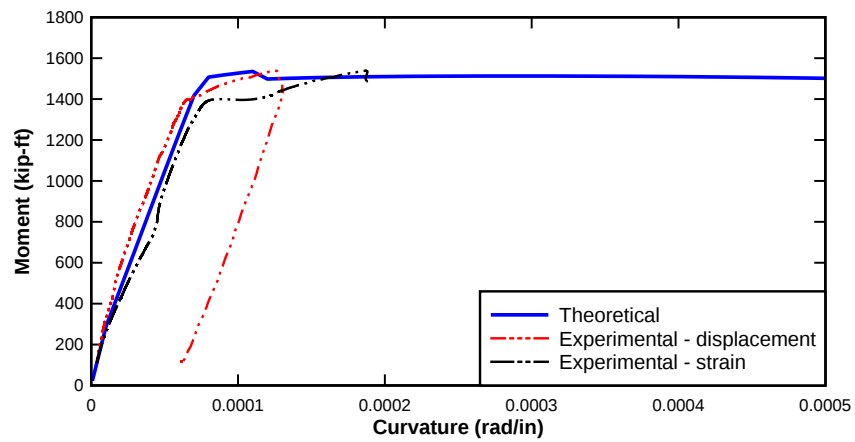
Figure 207—Moment curvature of Girder 4-2
