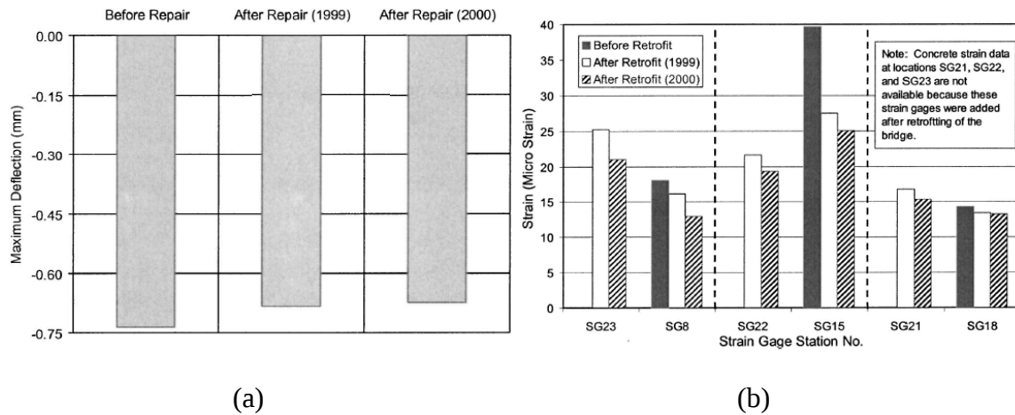
Figure 41—(a) Maximum slab deflection (b) maximum strains in slab and FRP (Shahrooz and Boy, 2004)
