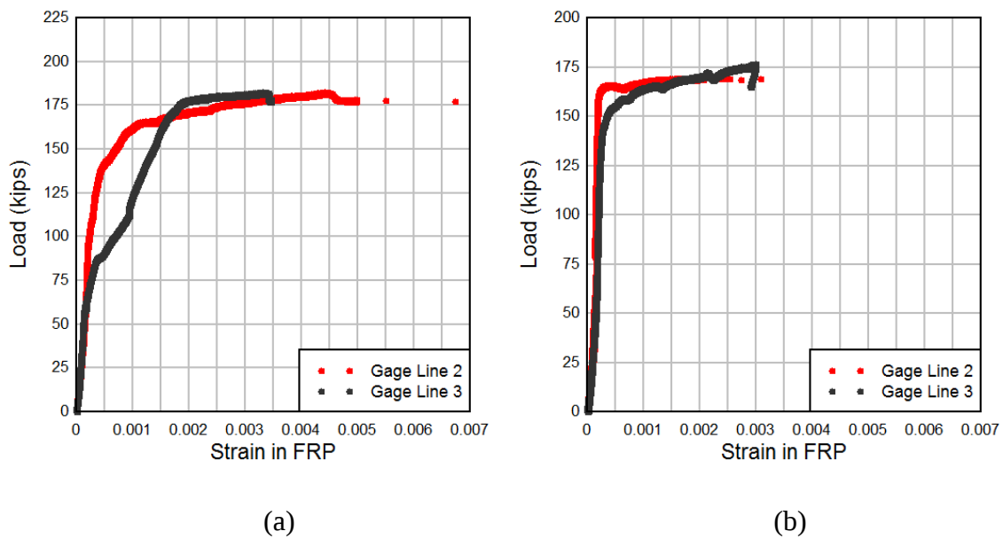
Figure 116—Development of strain in CFRP at the bottom of (a) Girder #1, and (b) Girder #2
