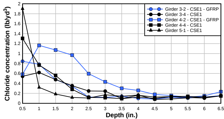
Figure 221—Chloride penetration profiles at specified locations
