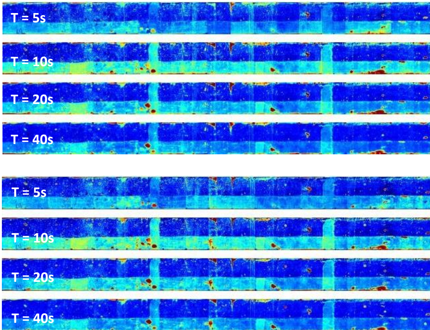
Figure 86—Girder #1 – south face: prior to structural test (top), and after structural test (bottom)
