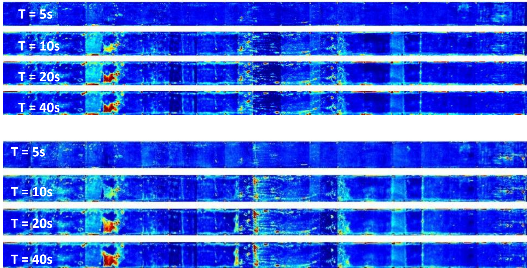
Figure 91—Girder #2 – bottom: prior to structural test (top), and after structural test (bottom)
