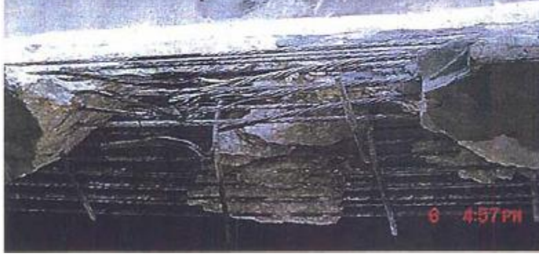
Figure 248—Severed strands on Girder 2 after impact in 2001 (Green et al., 2004)
