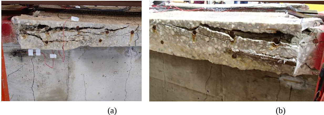
Figure 201—Crushing of concrete (Girder 5-2): (a) west elevation and (b) east elevation
