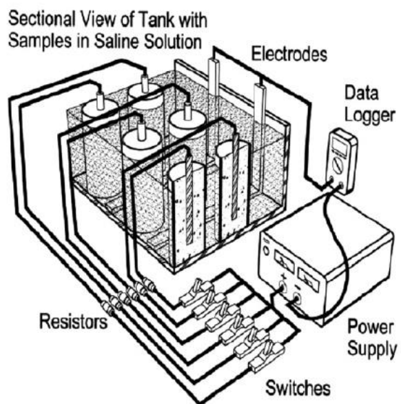
Figure 274—Spainhour and Wootton (2008): Test configuration
