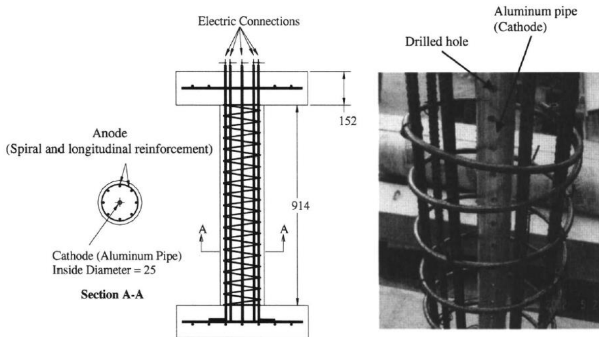
Figure 266—Bae and Belarbi (2009): Midscale RC columns
