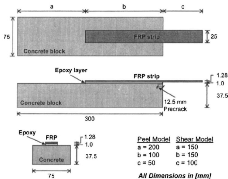
Figure 14—Direct shear/peel test specimen (Au and Buyukozturk, 2006)
