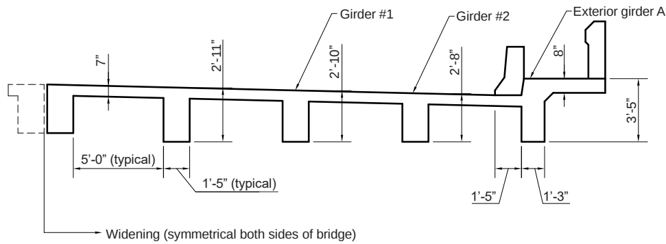
Section A
