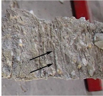
Figure 180—Crack front appearing on concrete substrate of debonded CFRP (Girder 4-1)
