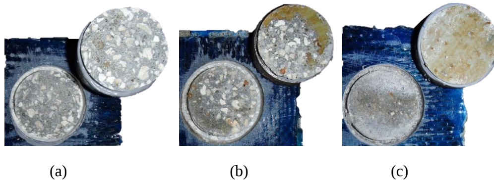
Figure 73—Typical failure modes in direct tension pull-off test: (a) cohesive (0% adhesive) (b) 30% adhesive and (c) 100% adhesive
