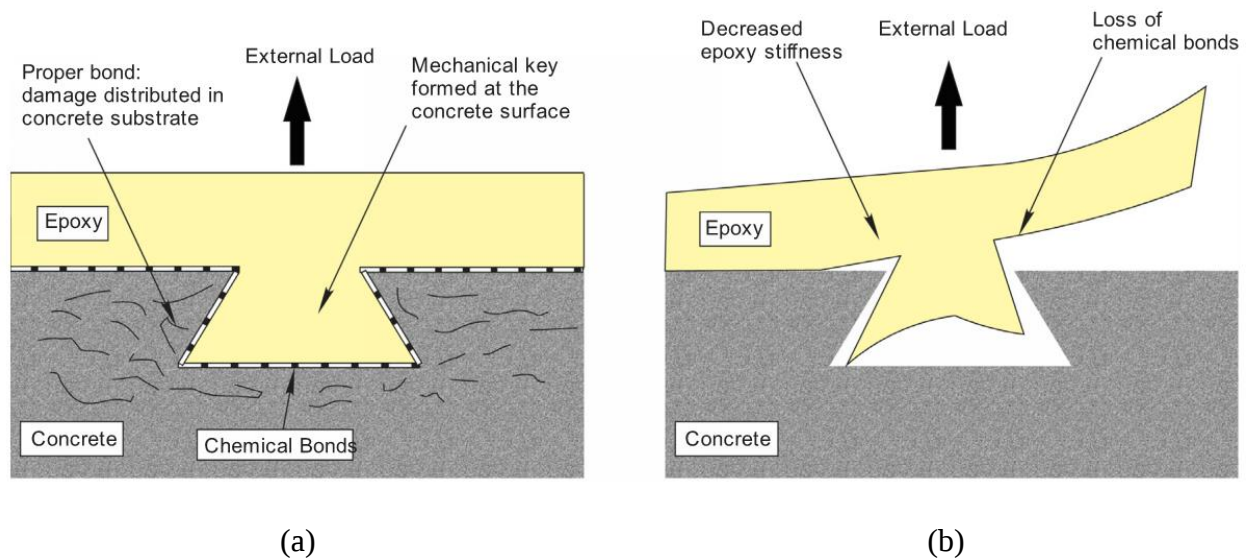
Figure 2—Graphical representation of (a) chemical and mechanical bond mechanisms for adhesively bonded FRP composites and (b) loss of bond due to loss of individual bond mechanisms (Blackburn et al., 2015)
