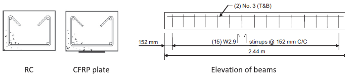
Figure 23—Beam flexure specimen (Cromwell et al., 2011)
