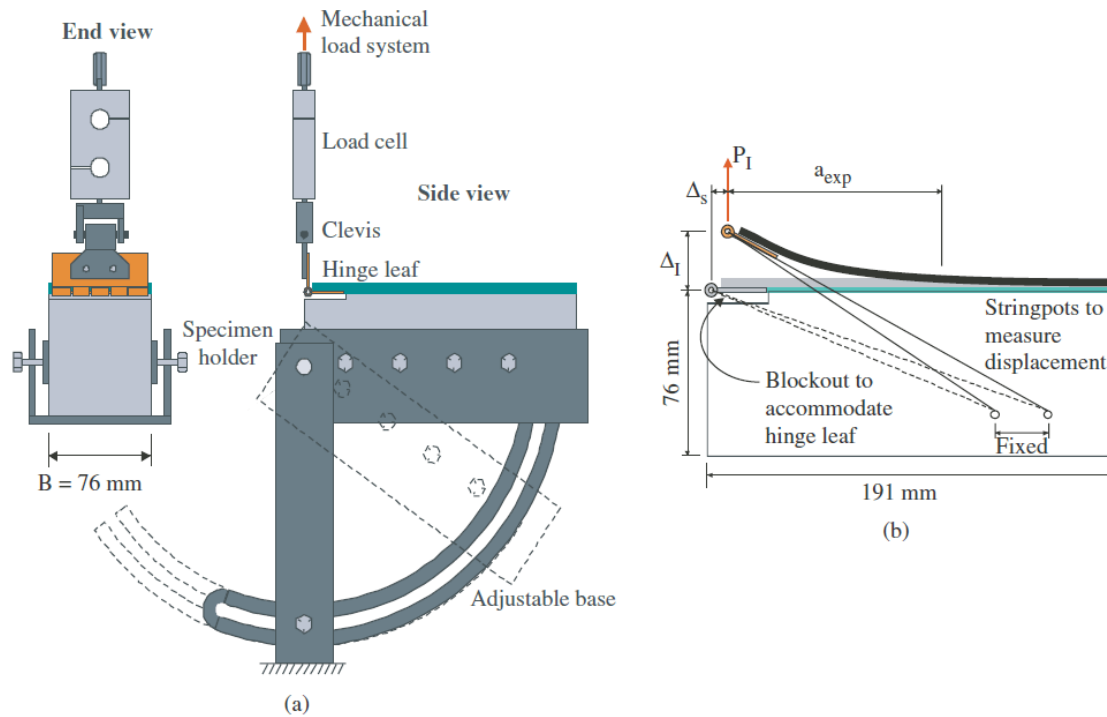
Figure 15—Mixed mode peel test setup (Wan et al., 2006)
