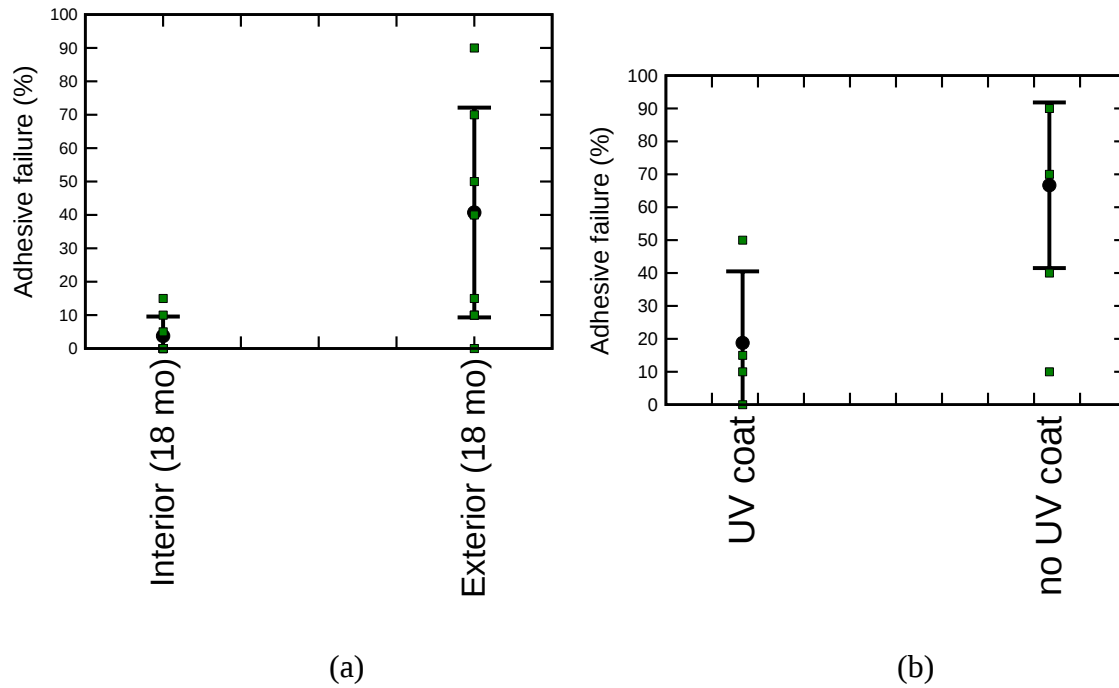
Figure 74—(a) Distribution of adhesive failure modes amongst the test groups (b) distribution of adhesive failure mode characteristics on exterior girder
