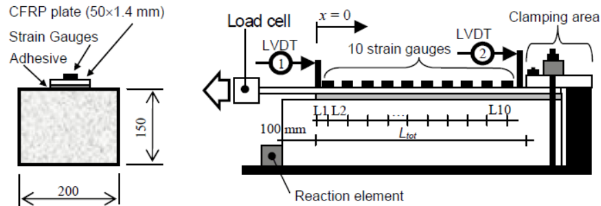
Figure 17—Direct shear test setup (Fava et al., 2007)
