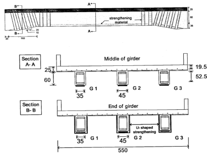
Figure 45—FRP strengthening details (Sim et al., 2006)
