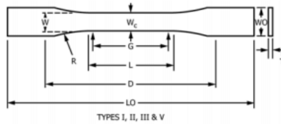
Figure 156—Specimen dimensions based on thickness T as per ASTM D638
