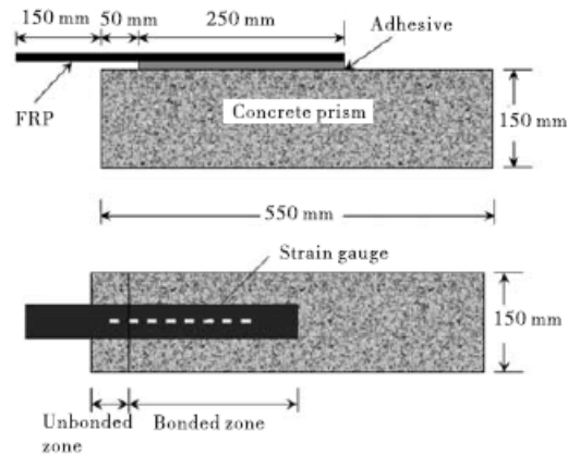
Figure 20—Direct shear test specimen (Pan et al., 2010)
