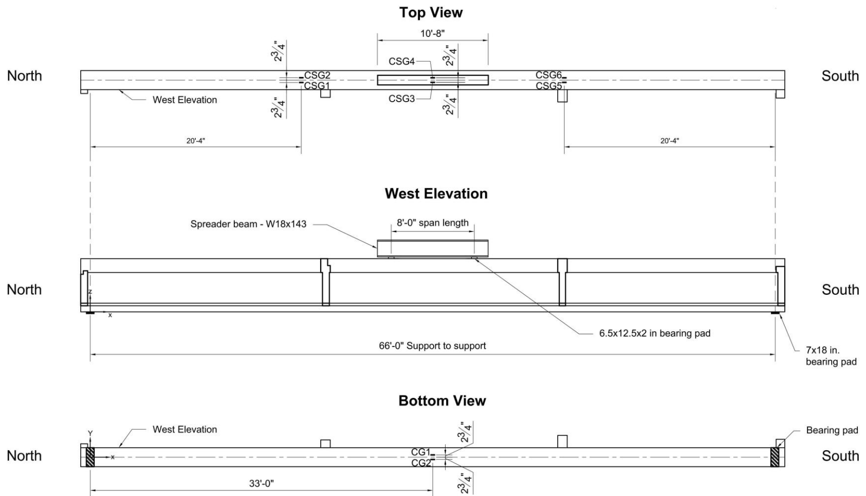
Figure 241—Typical instrumentation plan indicating the strain gage locations for girders without FRP
