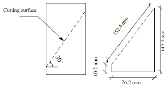
Figure 16—Slant shear test specimen (Frigione et al., 2006)
