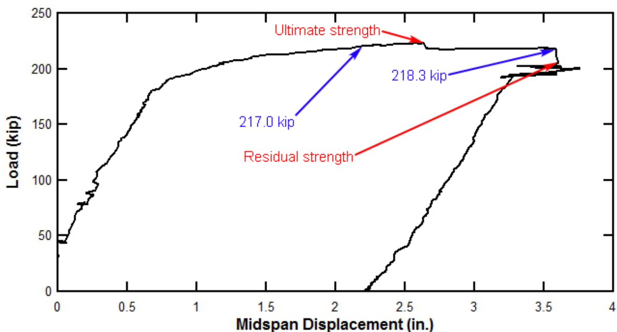
Figure 172—Load vs. displacement plot for Girder 3-4
