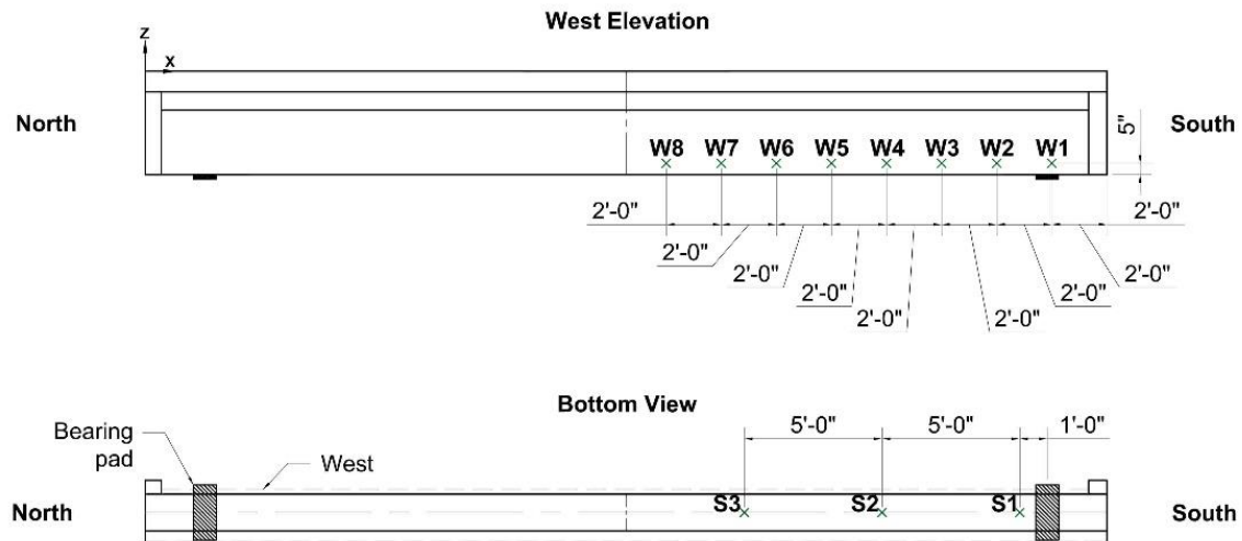
Figure 140—Typical potential testing locations for exterior girders and control
