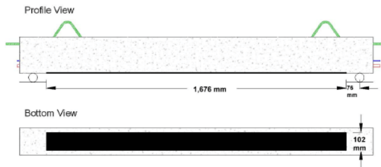
Figure 33—Wrapping scheme 1 (Davalos et al., 2012)
