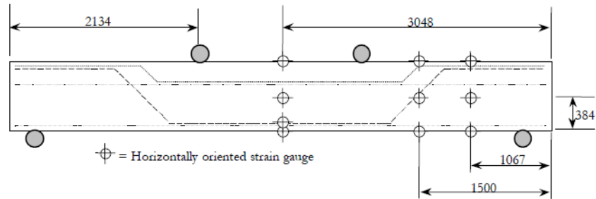
Figure 51—Location of electrical resistance strain gauges (Kachlakev and McCurry, 2000)
