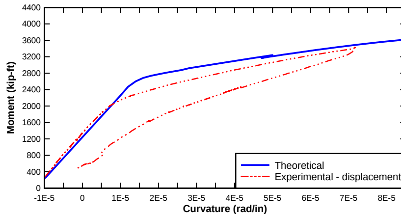
Figure 256—Moment curvature of Girder 4
