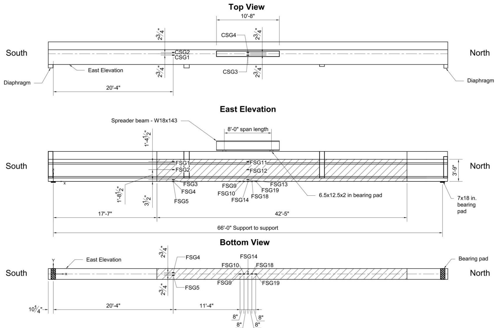
Figure 243—Instrumentation plan indicating the strain gage locations for Girder 3
