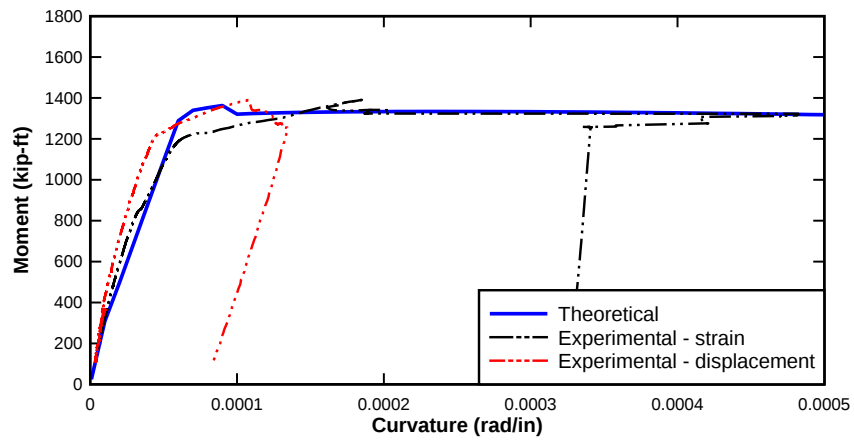
Figure 204—Moment curvature of Girder 4-4
