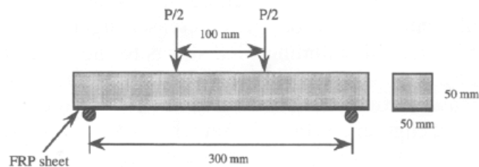
Figure 8—Four-point bending test setup (Toutanji and Gomez, 1997)
