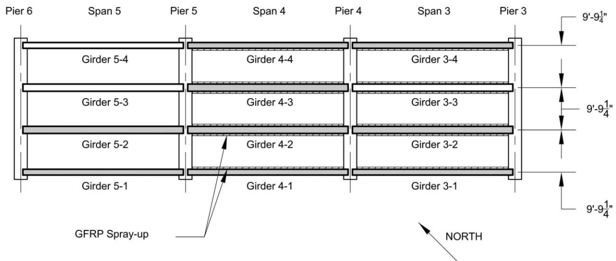
Figure 133—Plan view of spans 3, 4, and 5 chosen for evaluation
