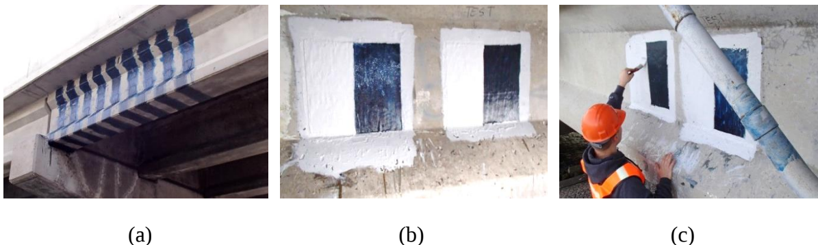
Figure 72—(a) Repair of Sunshine Skyway Bridge (b) interior girder test patches and (c) exterior girder test patches
