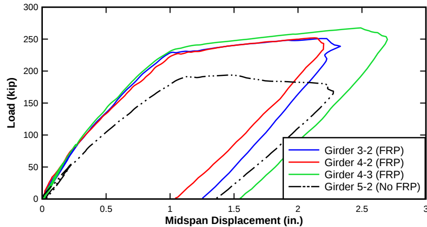
Figure 189—Load-midspan displacement of interior test girders
