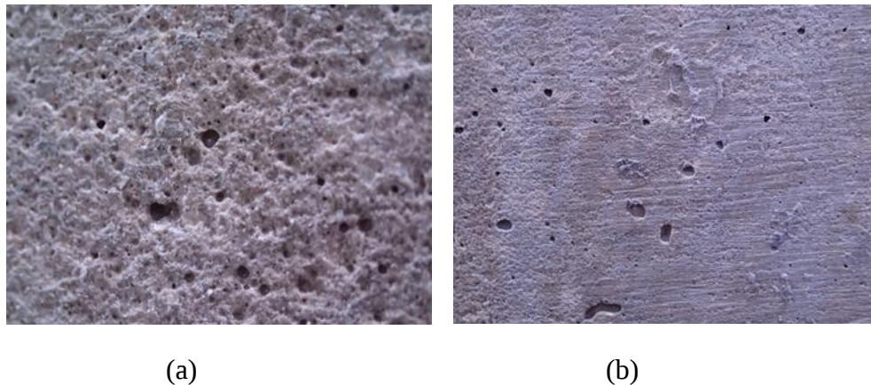
Figure 120—Difference between: (a) sandblasted concrete surface and (b) concrete surface without surface preparation
