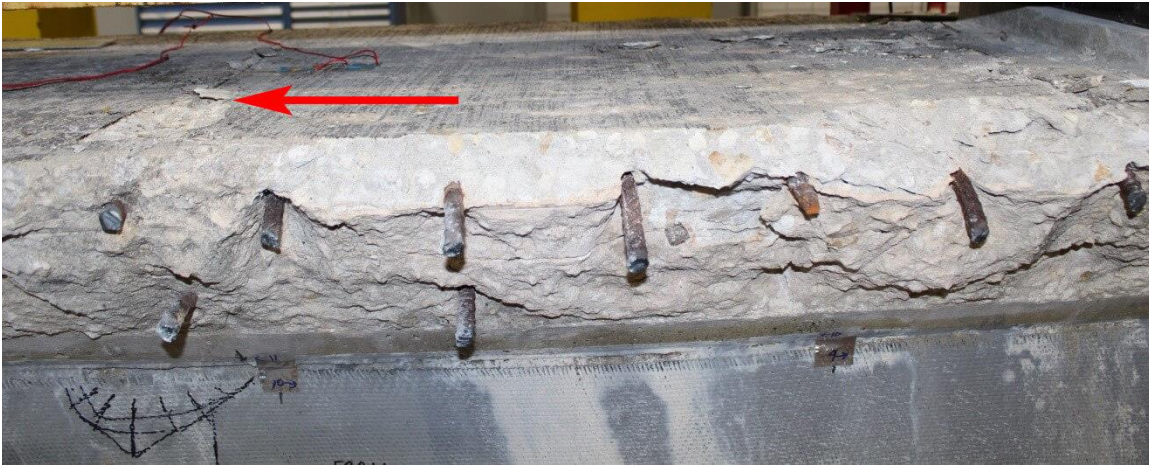
Figure 112—Failure of concrete in compression indicated by red arrow
