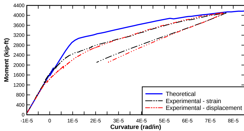
Figure 255—Moment curvature of Girder 3
