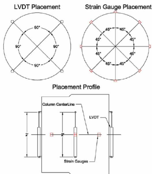
Figure 55—Instrumentation plan (Pantelides et al., 2011)
