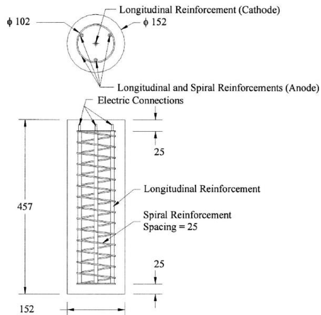
Figure 264—Small-scale columns (Bae and Belarbi, 2009): Specimen details of small-scale RC columns (dimensions in mm)
