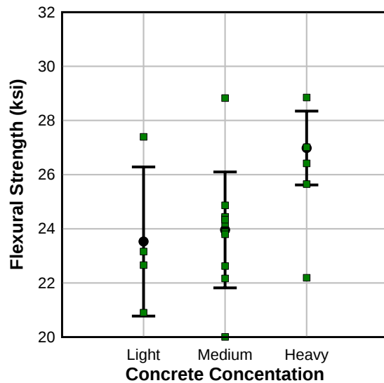
Figure 215—Comparison between debonded concrete concentration and flexural strength
