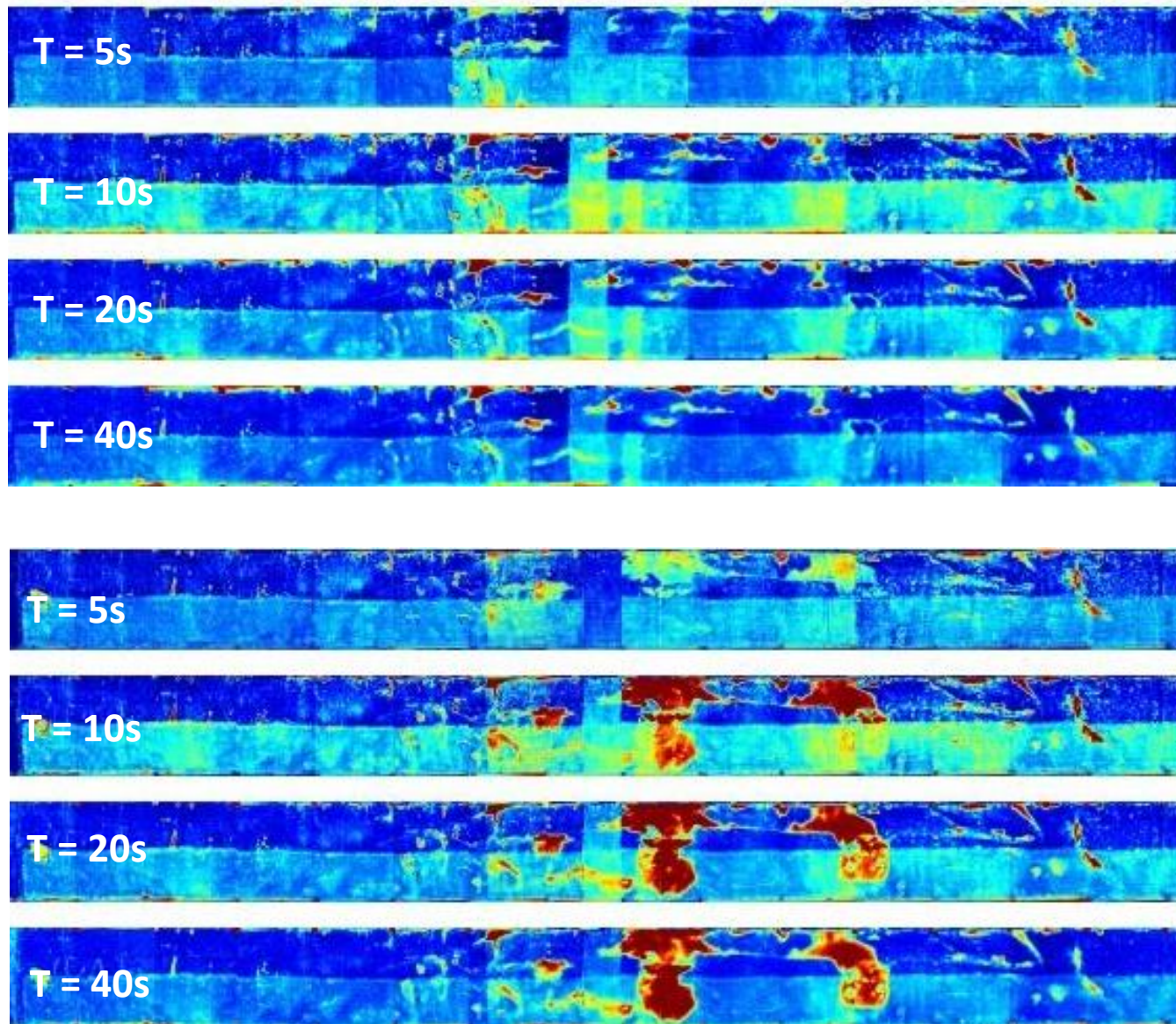
Figure 90—Girder #2 – north face: prior to structural test (top), and after structural test (bottom)
