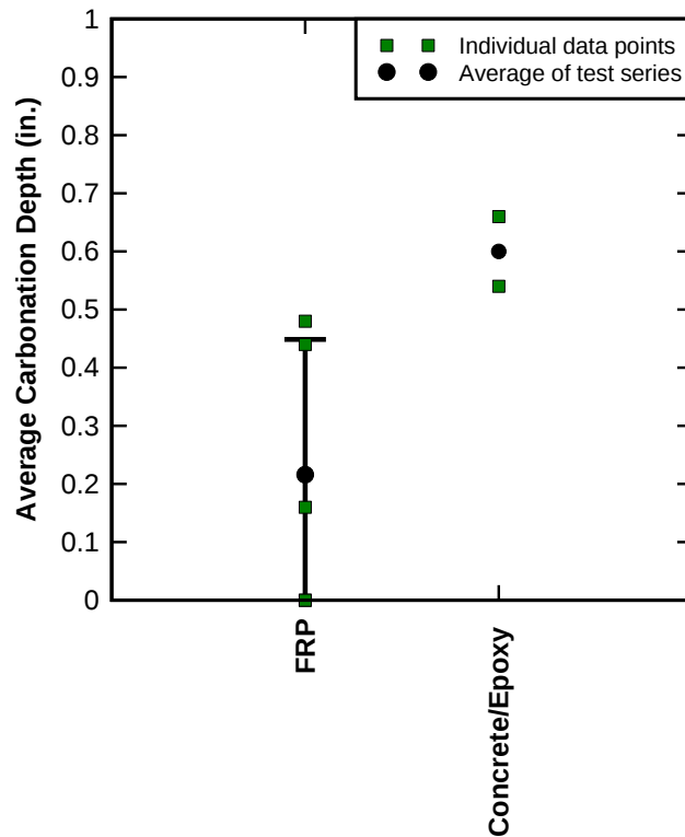
Figure 96—Carbonation depth measurements (error bars represent one standard deviation)
