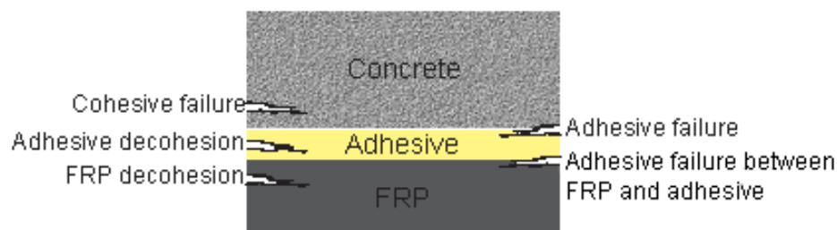
Figure 1—Possible failure modes in FRP-concrete bond system
