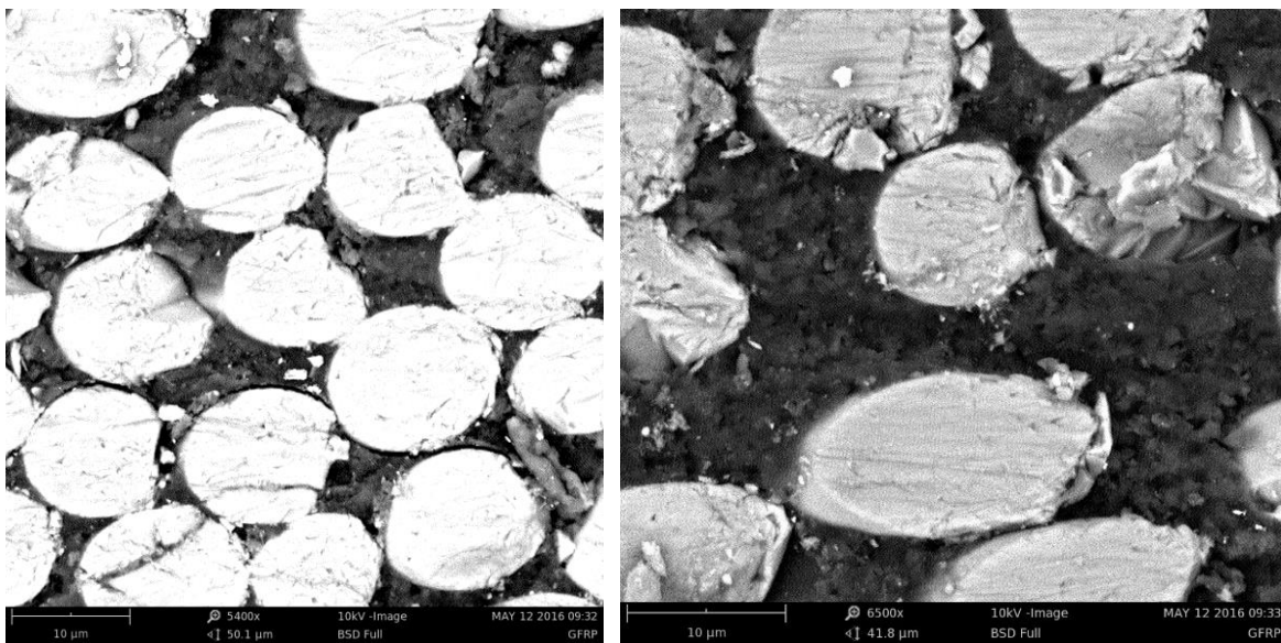
Figure 165—Magnified SEM images of fiber-matrix interface
