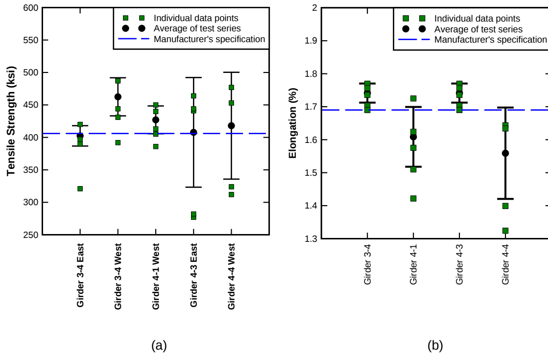
Figure 150—Correlation between the theoretical and experimental (a) tensile strength and (b) elongation
