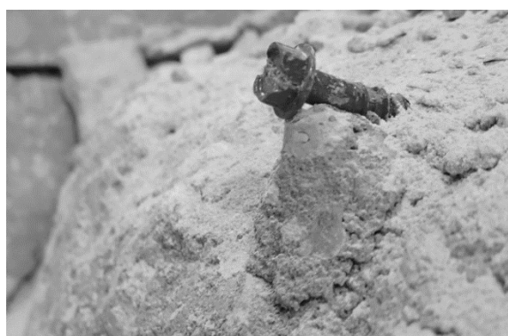
Figure 127—Concrete screw at the interface between new and old concrete
