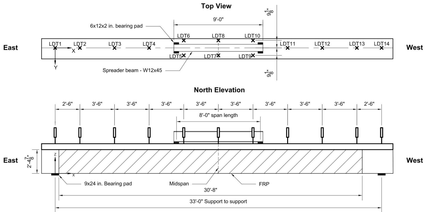
Figure 106—Girder #1 – Instrumentation plan representing the locations for laser displacement transducers
