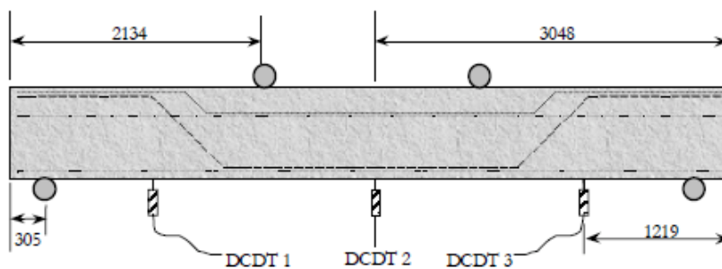
Figure 50—Location of displacement transducers (Kachlakev and McCurry, 2000)
