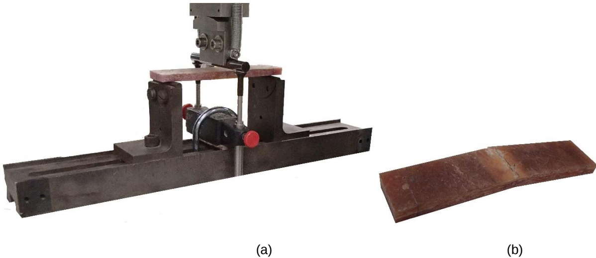
Figure 162—(a) GFRP coupon flexural test setup (b) typical failure mode of test coupon
