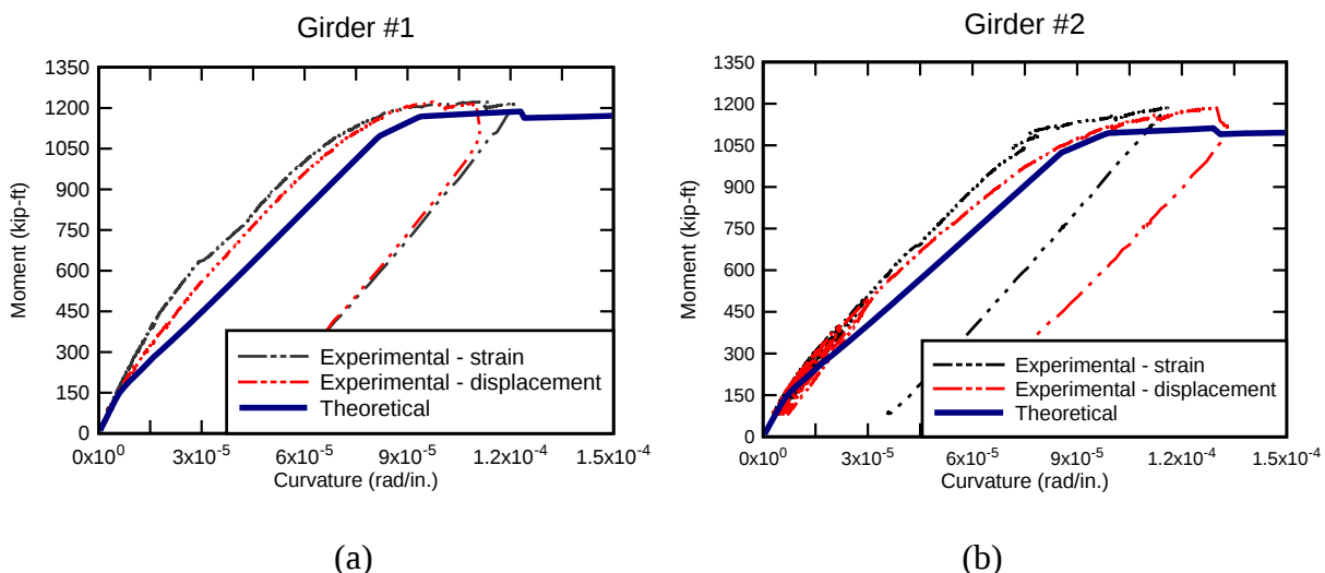
Figure 118—Moment curvature for: (a) Girder #1 and (b) Girder #2
