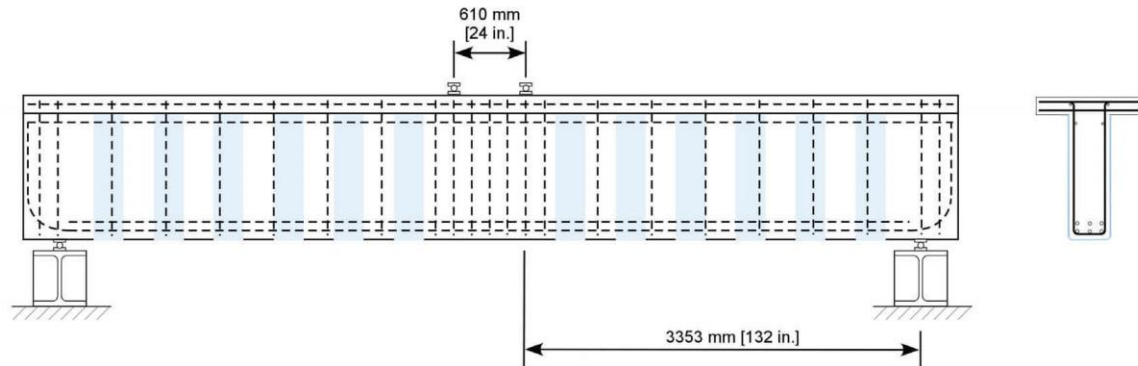
T Specimen (Typical)
