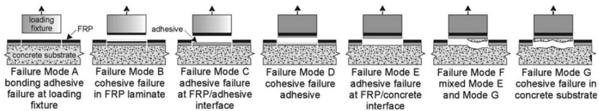
Figure 60—Failure modes for pull-off test (ASTM D7522)
