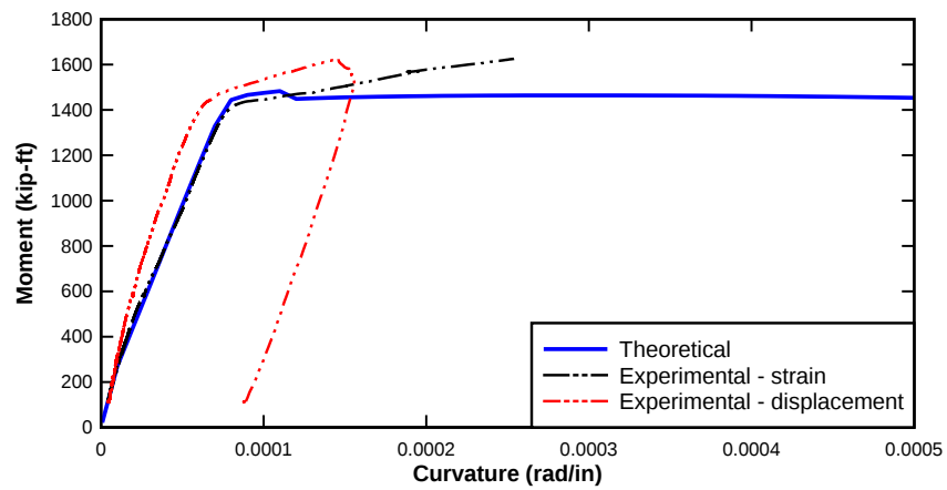
Figure 208—Moment curvature of Girder 4-3
