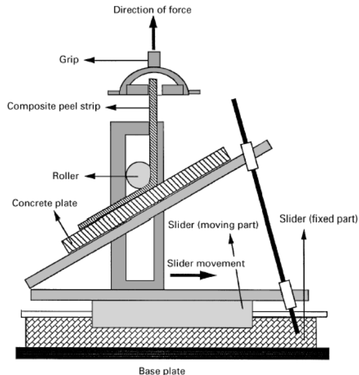
Figure 7—Mixed mode peel test setup (Karbhari and Engineer, 1996)
