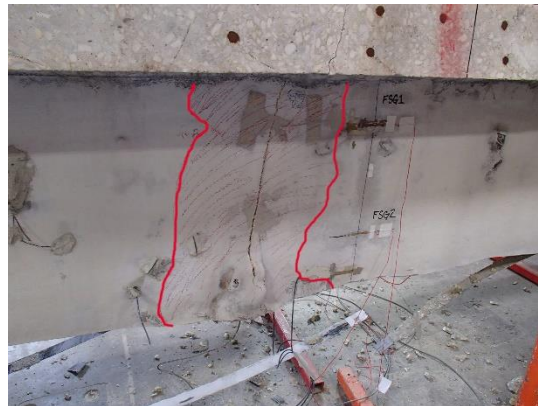
Figure 179—GFRP rupture (Girder 4-1) with debonded GFRP region outlined in red
