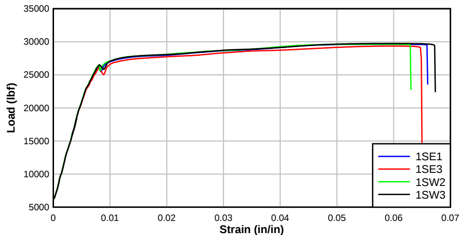
Figure 233—Typical load vs. strain plot
