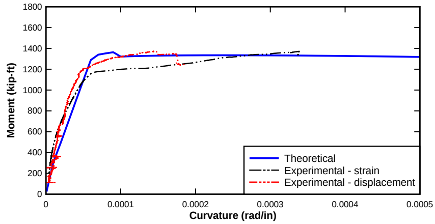
Figure 202—Moment curvature for Girder 3-4
