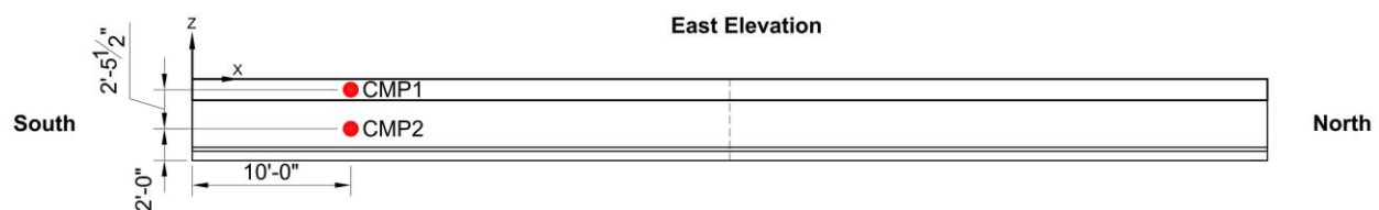
Figure 230—Typical coring locations for compression cores
