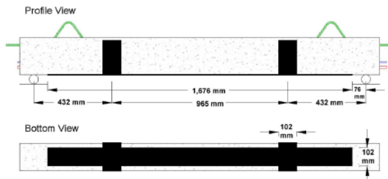
Figure 33—Wrapping scheme 1 (Davalos et al., 2012)
