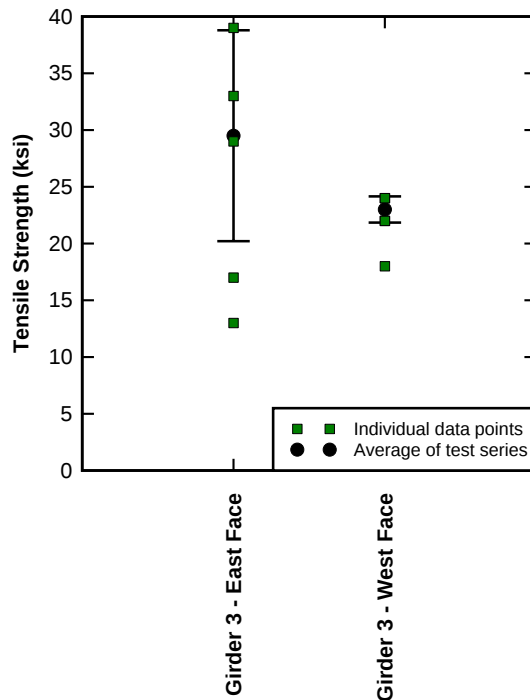
Figure 234—Comparison of tensile strength of the tested samples (error bars represent one standard deviation)
