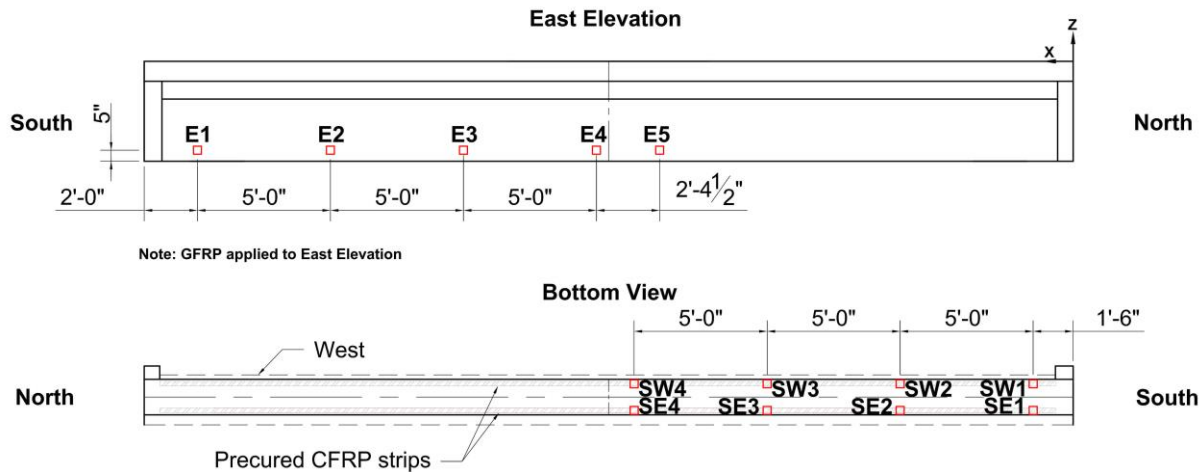
Figure 151—Direct pull-off testing locations for Girder 3-1
