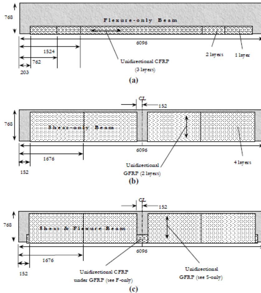
Figure 49—FRP strengthened girder: (a) flexure-only beam (b) shear-only beam; and (c) shear and flexure beam (Kachlakev and McCurry, 2000)
