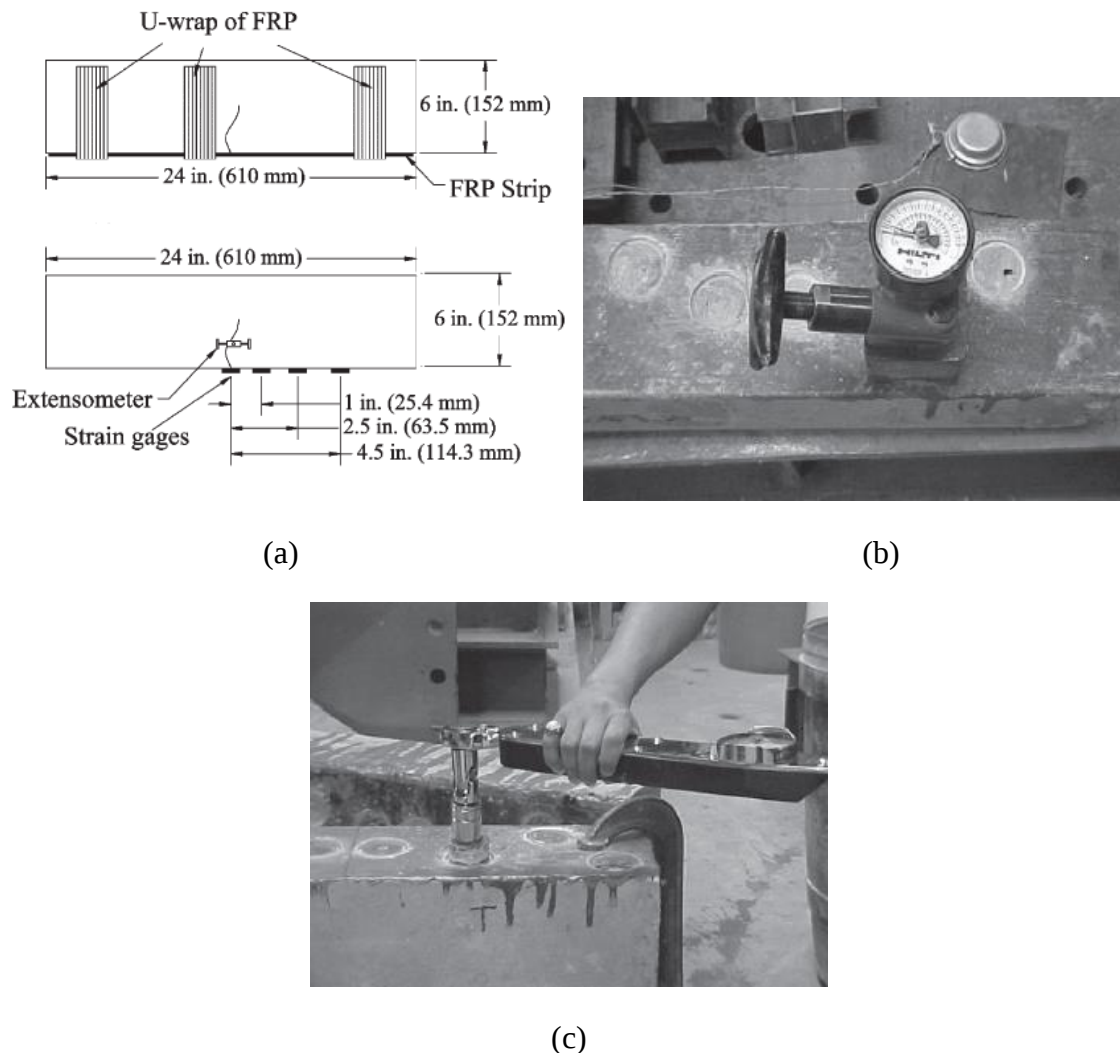
Figure 11—Myers and Ekenel (2005): (a) flexural specimens; (b) direct pull-off test setup; (c) direct torsion test setup
