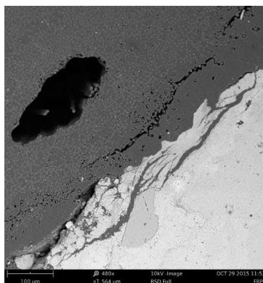
Figure 105—Large void and initiation of debonding of CFRP near CFRP-concrete interface
