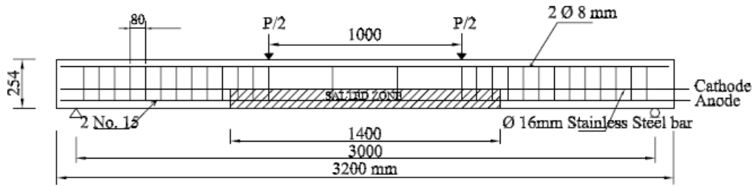
Figure 270—Masoud and Soudki (2006): Typical dimension and reinforcement details of the test specimen
