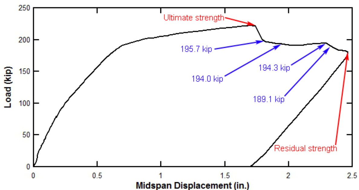
Figure 176—Load vs displacement plot for Girder 4-1
