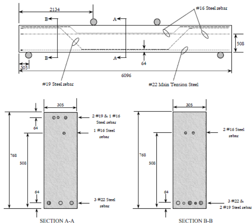
Figure 48—Reinforced concrete control specimen design (Kachlakev and McCurry, 2000)
