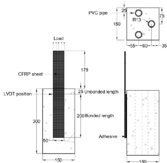
Figure 25—Direct shear test specimen (Srestha et al., 2013)
