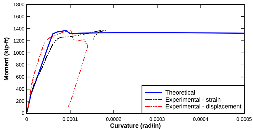
Figure 203—Moment curvature of Girder 4-1
