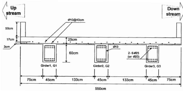
Figure 44—Cross-section view of test bridge girders (Sim et al., 2006)
