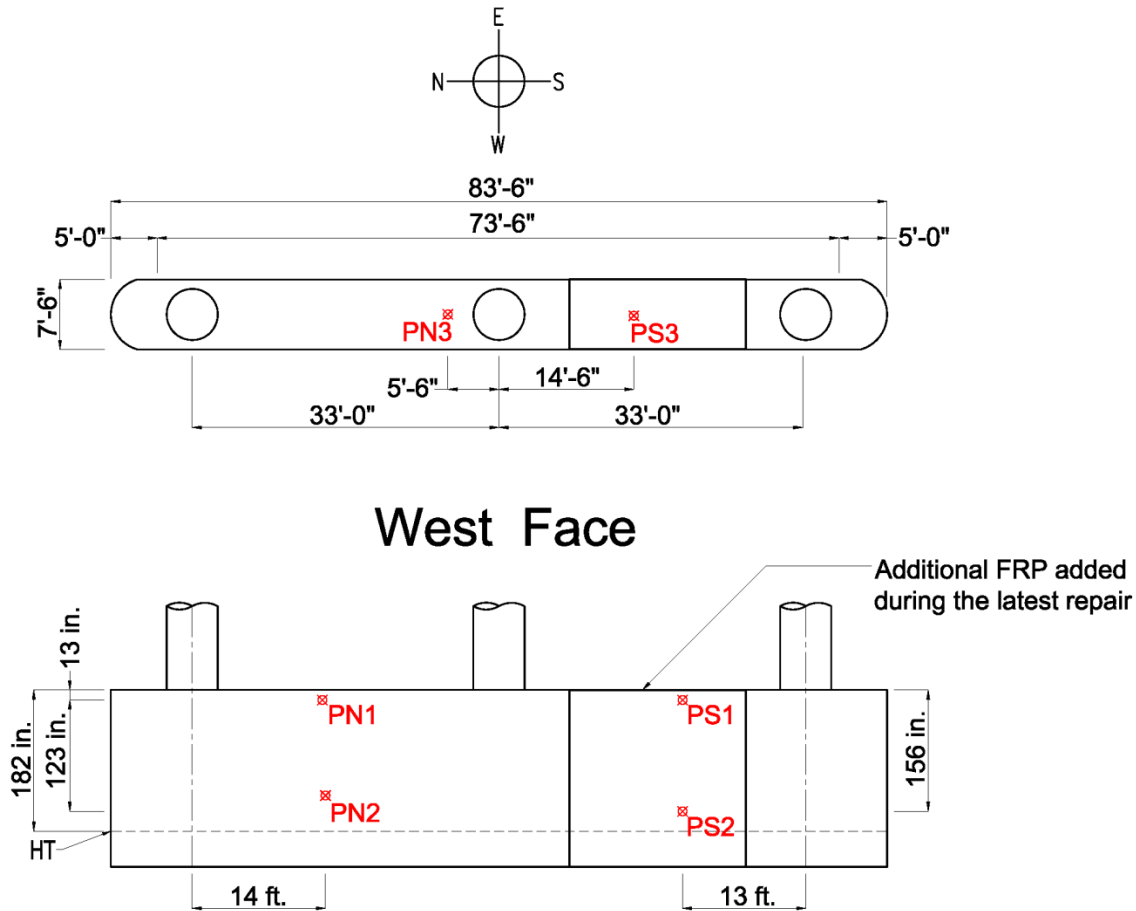
Figure 277—Pull-off test locations on Pier 8
