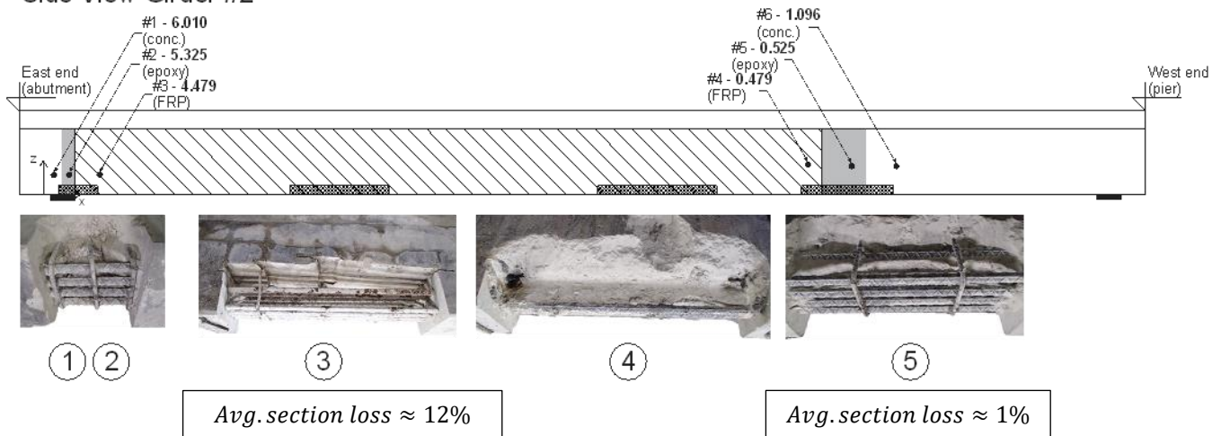
Figure 125—State of reinforcement and chloride contents (pcy) at specified locations along the north face of Girders #1 and #2
