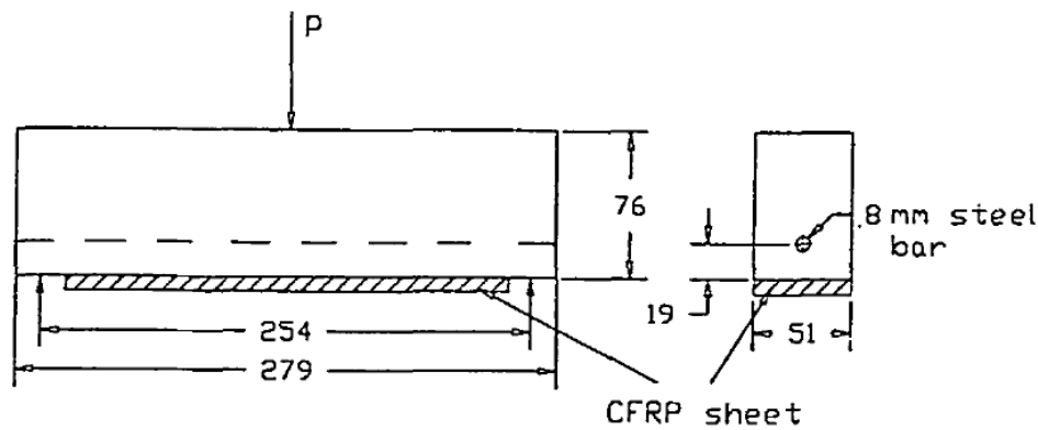
Figure 5—Three-point bending test setup (Xie et al., 1995)
