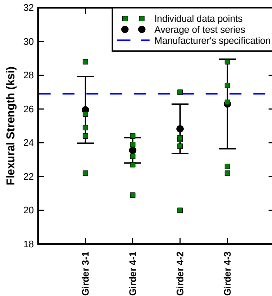
Figure 163—Comparison of the experimental flexural strength and manufacturer's specified flexural strength (error bars represent one standard deviation)
