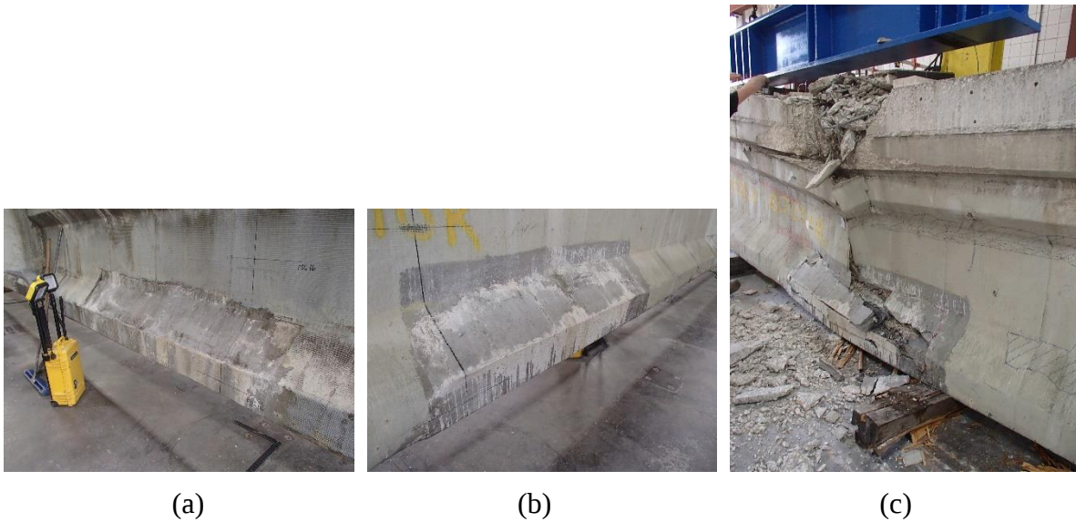
Figure 249—Repaired region of Girder 2: (a) west face initially before testing (b) east face initially before testing (c) east face after failure
