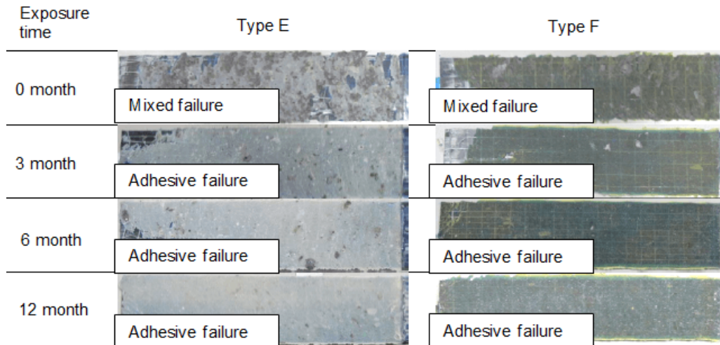
Figure 27—Failure surfaces for high strength concrete (Srestha et al., 2013)
