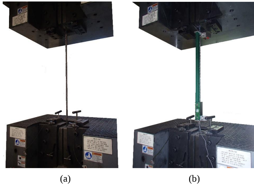
Figure 231—(a) Strand in tensile test setup (b) strand in tensile test setup with extensometer
