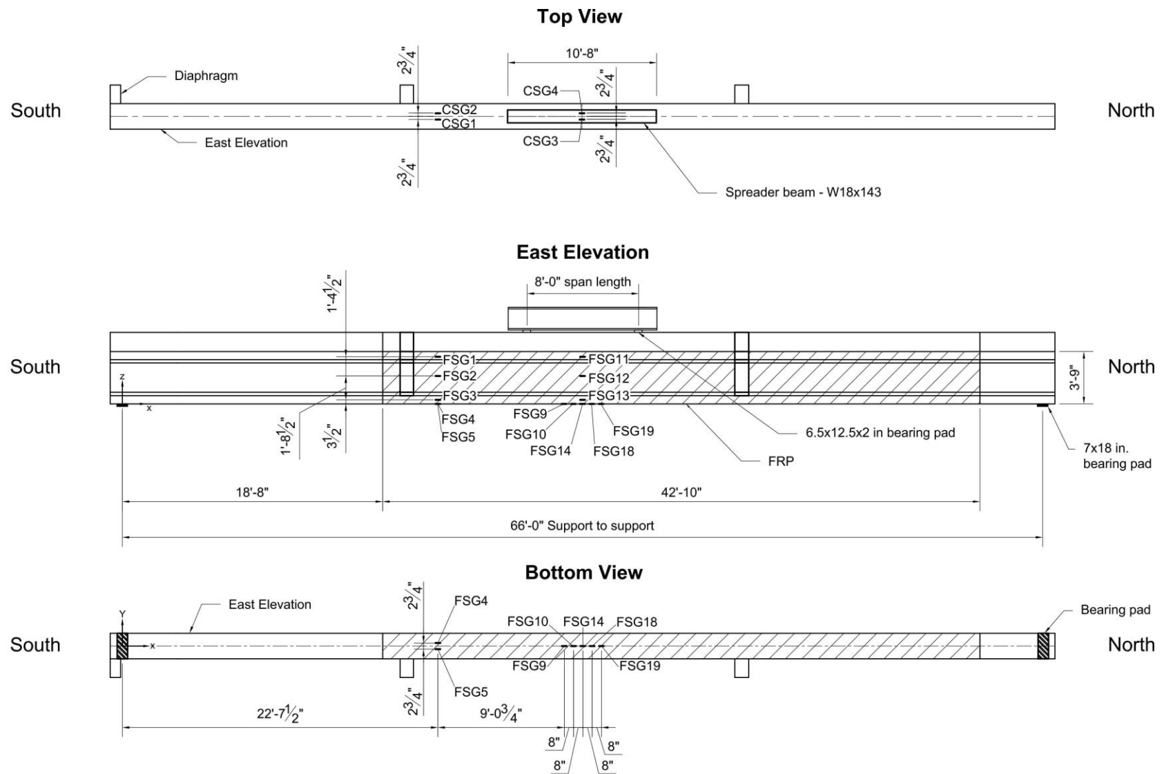
Figure 242—Instrumentation plan indicating the strain gage locations for Girder 2
