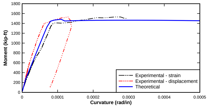
Figure 206—Moment curvature of Girder 3-2
