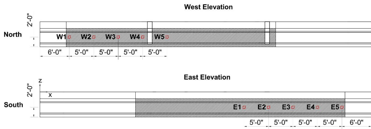
Figure 235—Direct pull-off testing locations for Girder 2
