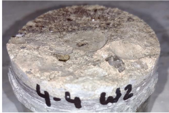
Figure 153—Pull-off testing sample from Girder 4-4 with multiple voids in concrete
