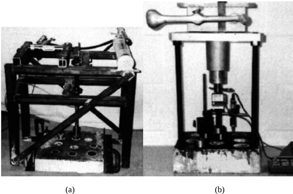
Figure 10—Sen et al. (1999): (a) torsion test setup; (b) pull-off test setup
