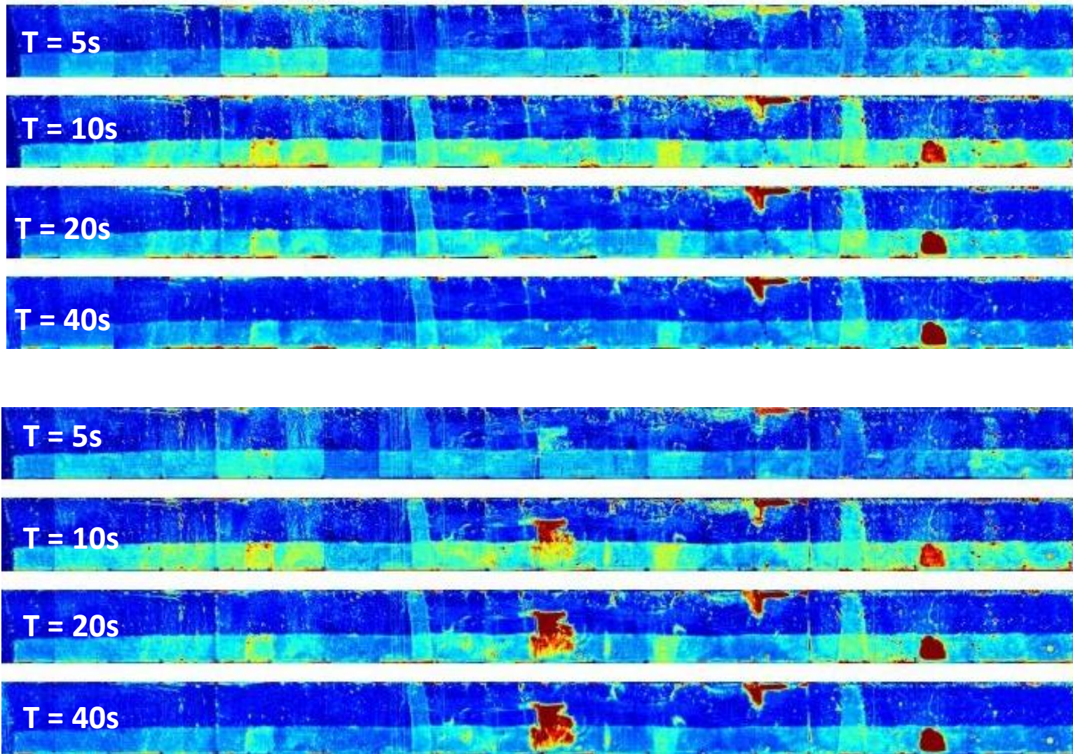
Figure 87—Girder #1 – north face: prior to structural test (top), and after structural test (bottom)
