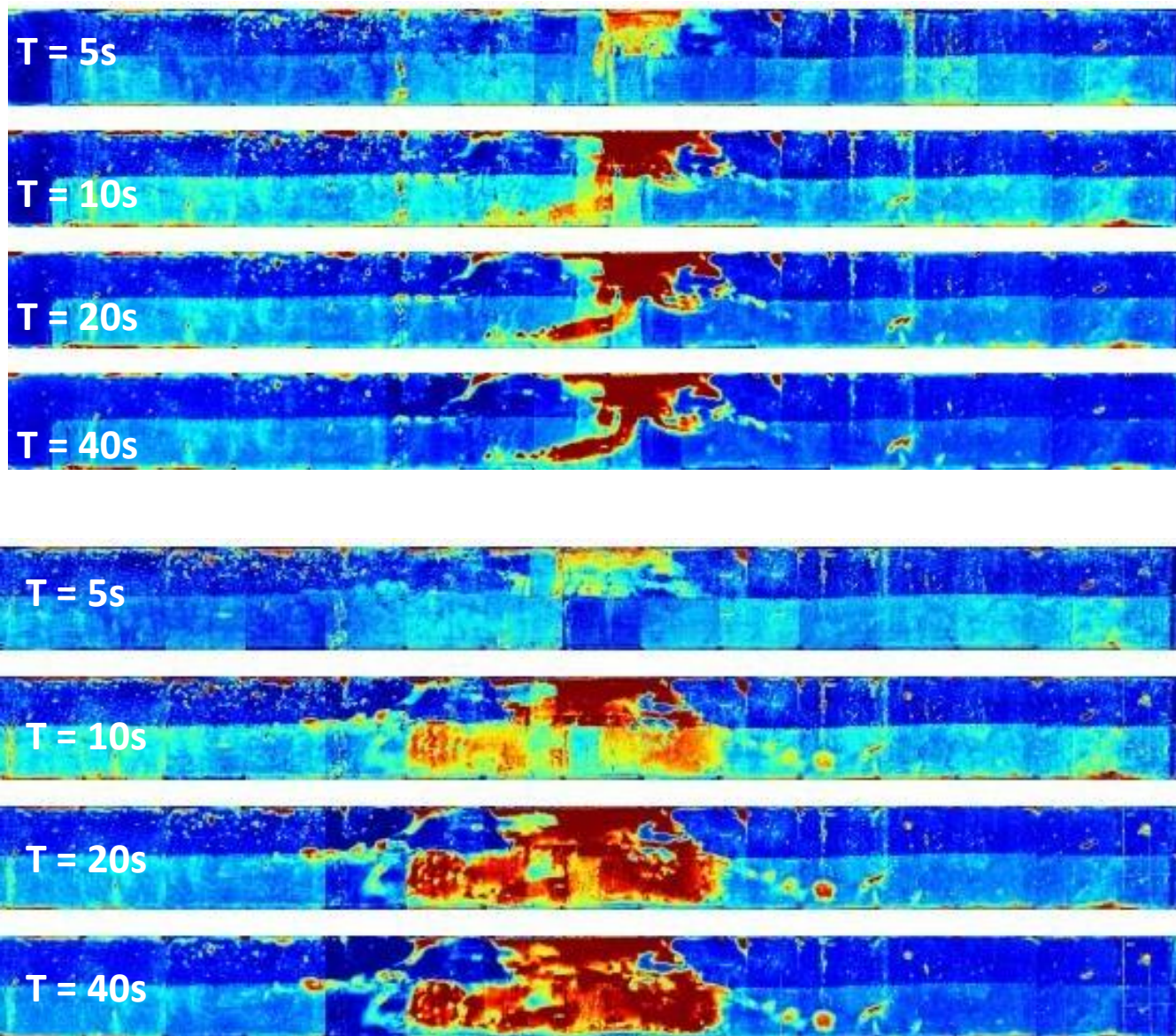
Figure 89—Girder #2 – south face: prior to structural test (top), and after structural test (bottom)
