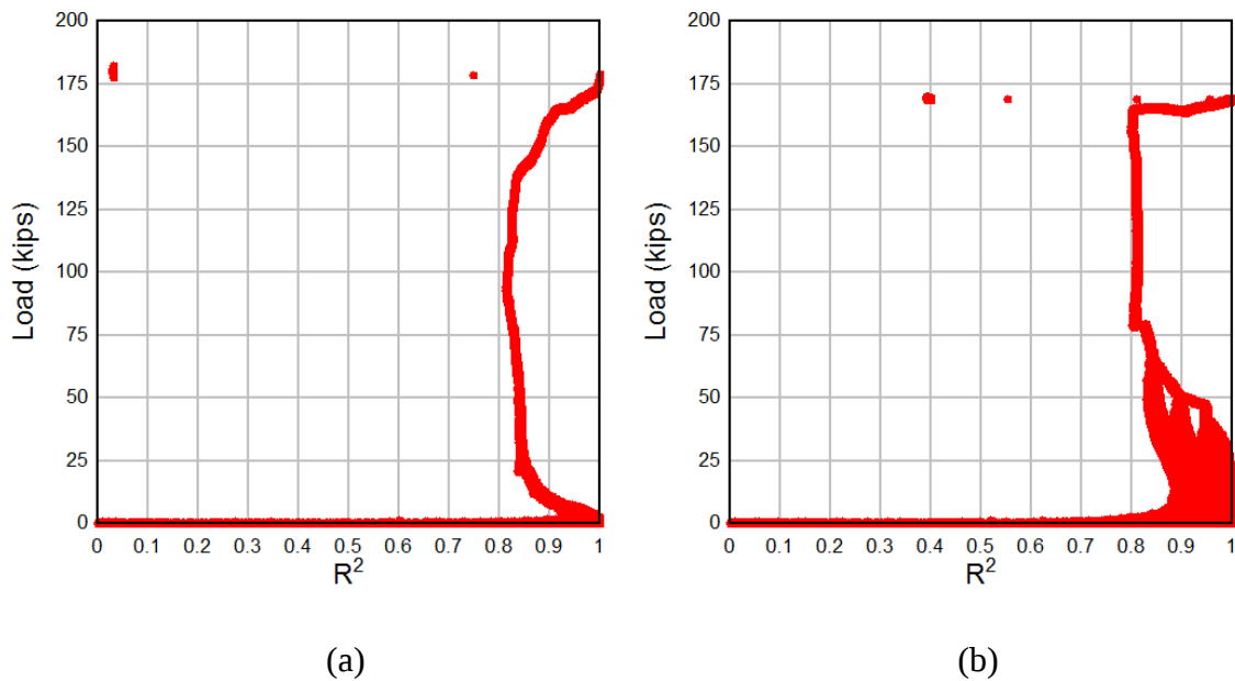
Figure 115—Goodness of linear fit with respect to applied load for gage line 2 on (a) Girder #1, and (b) Girder #2
