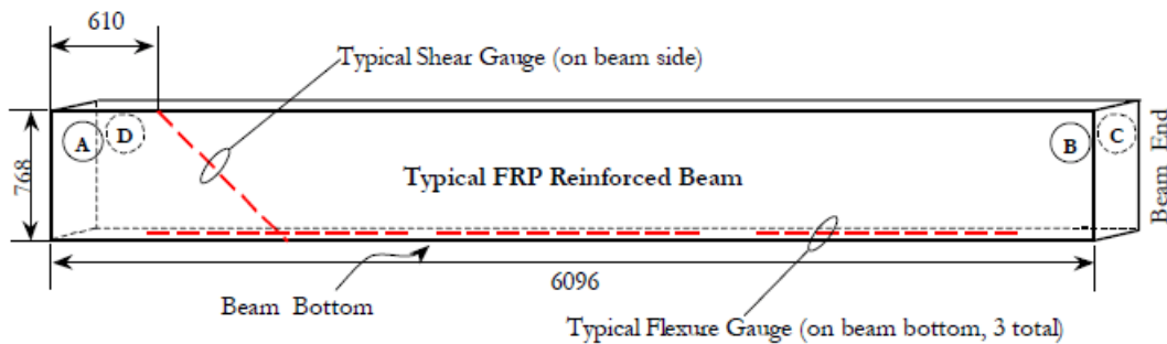
Figure 52—Location of fiber optic strain gauges (Kachlakev and McCurry, 2000)
