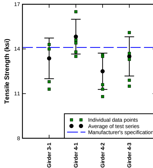
Figure 158—Comparison of experimental tensile strength and manufacturer's specified tensile strength (error bars represent one standard deviation)
