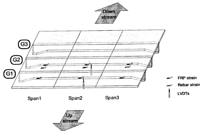
Figure 46—Location of instrumentation (Sim et al., 2006)
