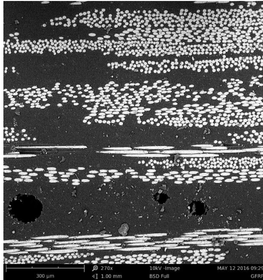
Figure 164—SEM image showing non-uniform distribution and preferential orientation of fibers within the GFRP composite matrix
