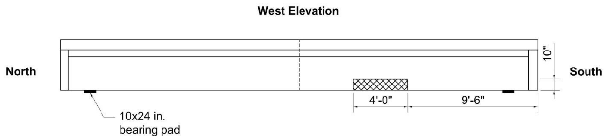
Figure 217—Typical steel reinforcement extraction location
