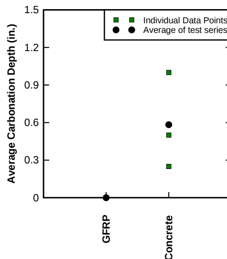
Figure 139—Carbonation depth measurements
