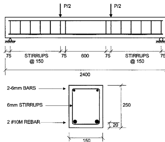
Figure 18—Four-point bending test beam design (Soudki et al., 2007)
