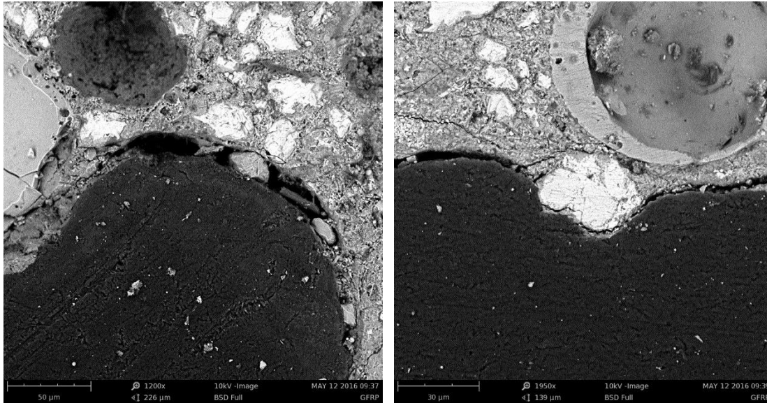
Figure 166—SEM image of interface between concrete (top) and GFRP composite (bottom)
