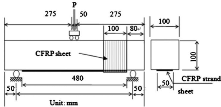
Figure 21—Three-point bending test setup (Dai et al., 2010)
