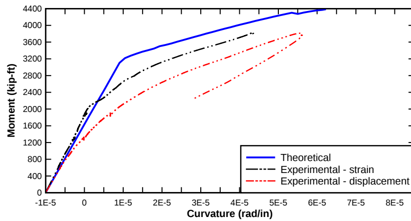
Figure 254—Moment curvature of Girder 2
