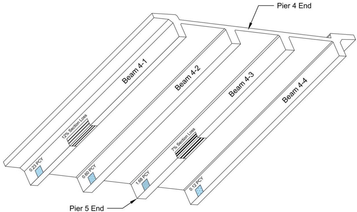
Figure 222—Chloride ion contamination levels and section loss in steel reinforcement in Span 4
