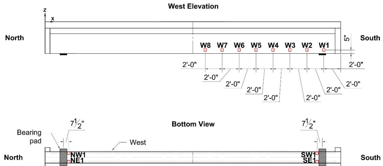
Figure 152—Direct pull-off testing locations for exterior girders
