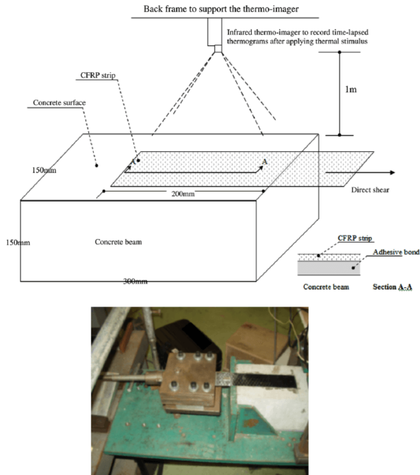
Figure 24—Direct shear test setup (Lai et al., 2009)
