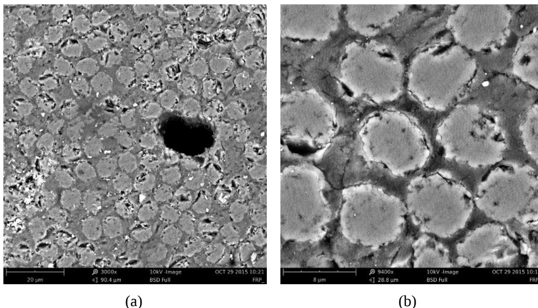
Figure 104—SEM images of defects present within the CFRP composite including (a) voids and (b) epoxy microcracking
