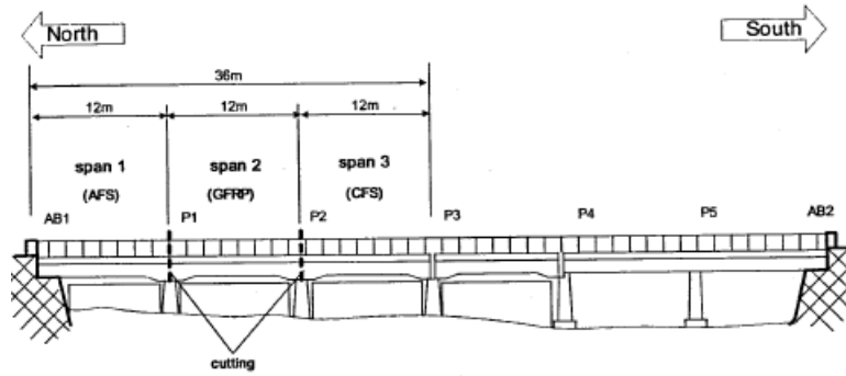
Figure 43—Bridge elevation view (Sim et al., 2006)
