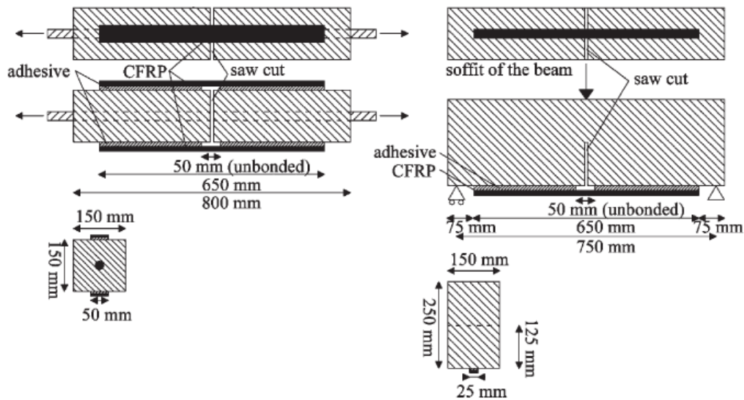
Figure 13—Double lap shear test setup (left); and three-point bending test setup (right) (Klamer et al., 2005)
