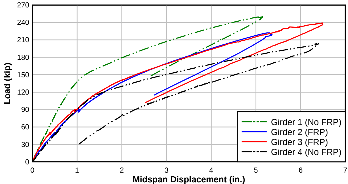
Figure 244—Load-midspan displacement of test girders
