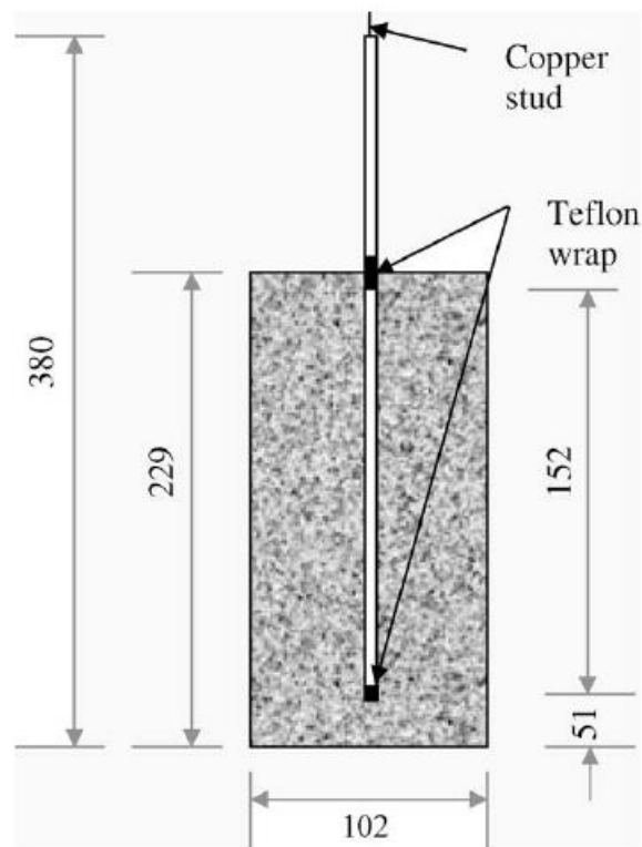
Figure 267—Gadve et al. (2009): Cylindrical reinforced concrete specimen
