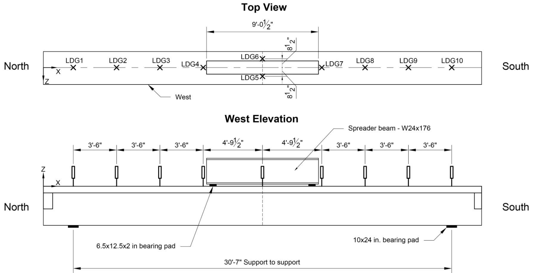
Figure 168—Typical instrumentation plan representing the locations for the laser displacement transducers
