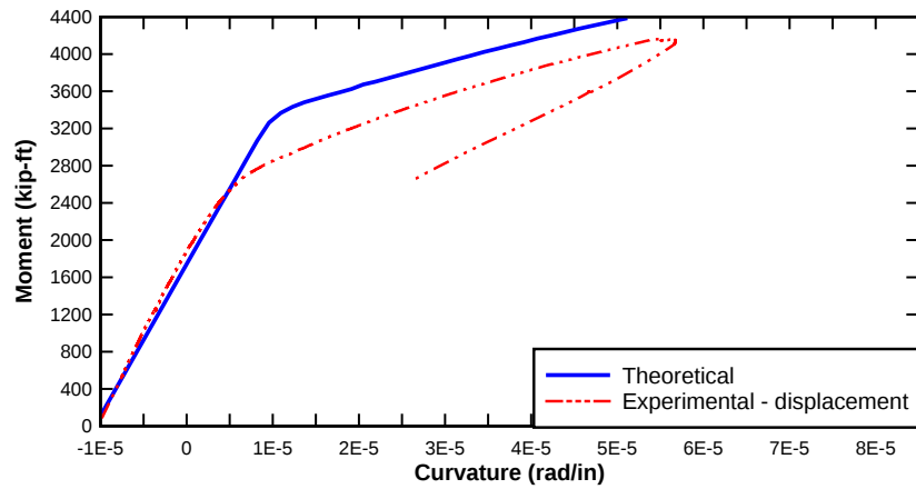
Figure 253—Moment curvature for Girder 1
