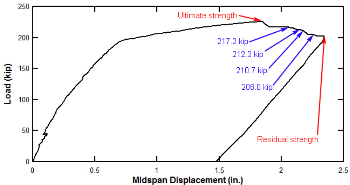
Figure 182—Load vs Displacement plot for Girder 4-4
