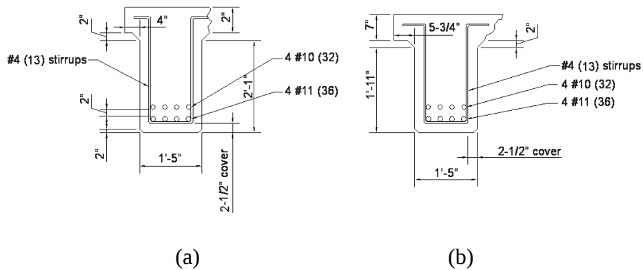
Figure 83—Cross-section of (a) Girder #1, and (b) Girder #2
