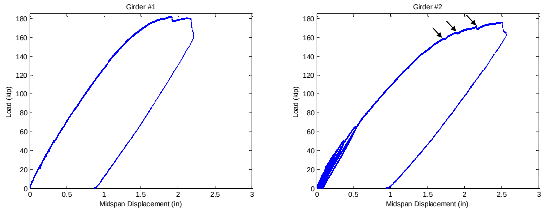
Figure 111—Load-midspan displacement of test girders
