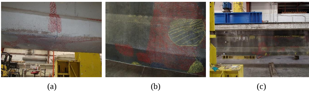
Figure 251—FRP damage on Girder 3: (a) close-up of rupture on east face (b) close-up of rupture on west face (c) rupture location on west face
