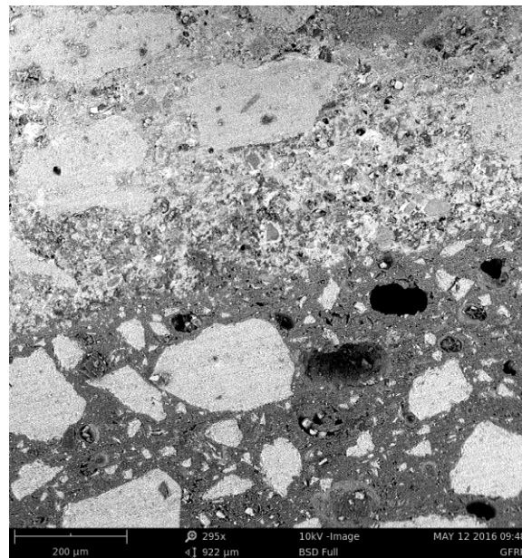
Figure 160—SEM image of interface between concrete (top) and epoxy (bottom).
