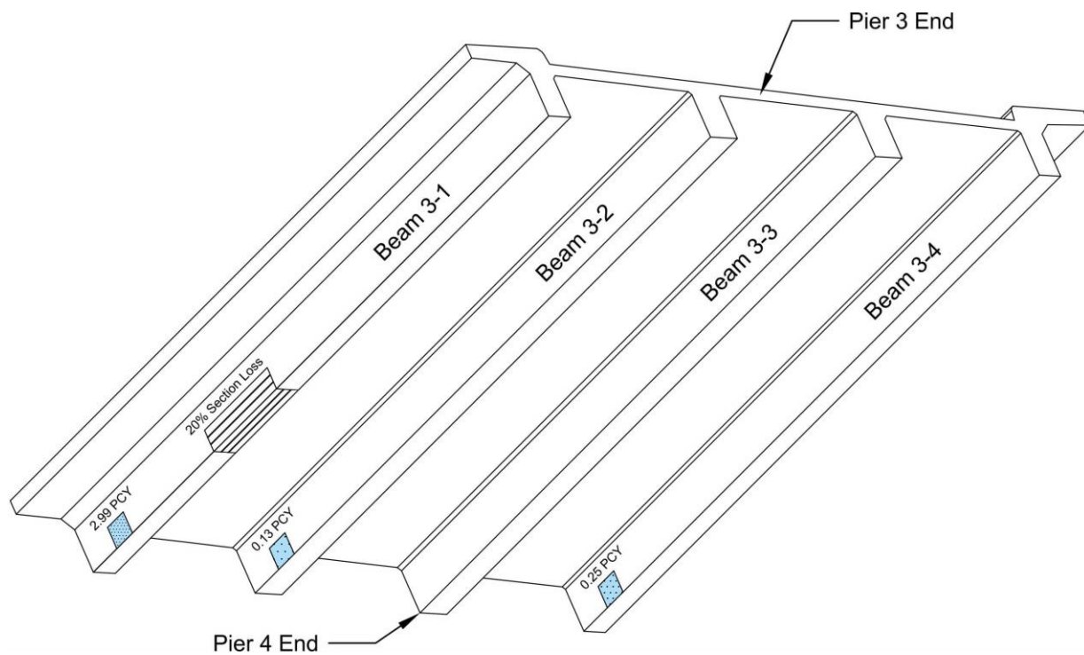
Figure 223—Chloride ion contamination levels and section loss in steel reinforcement in Span 3
