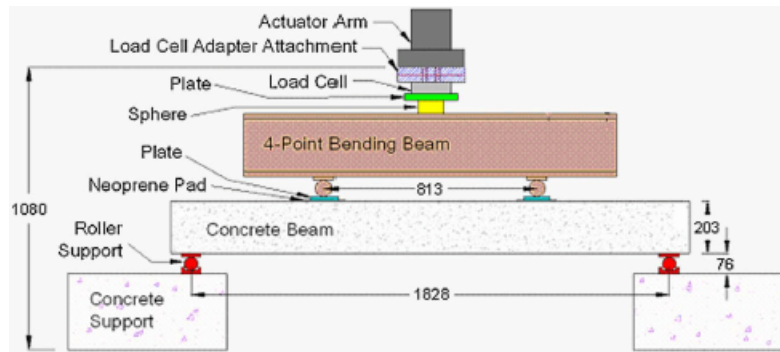
Figure 32—Anchorage scheme method study test specimen (Davalos et al., 2012)
