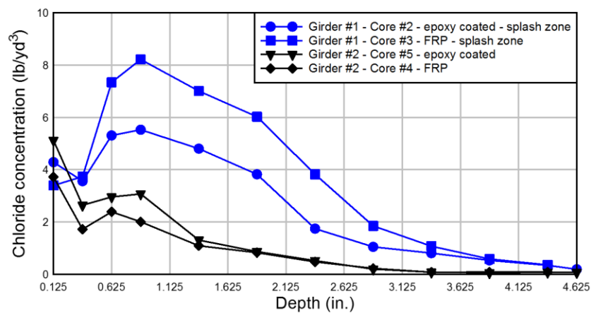
Figure 128—Chloride penetration profiles at specified locations
