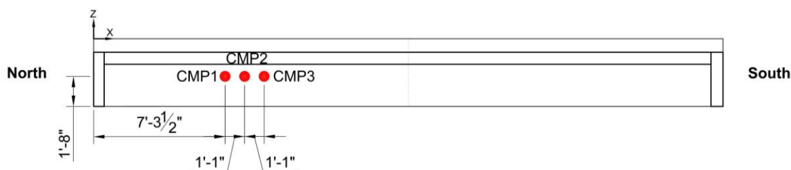
Figure 137—Typical coring locations for compression cores
