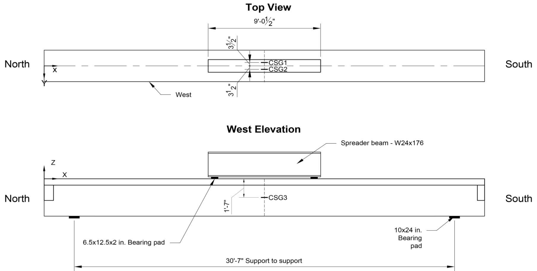
Figure 169—Instrumentation plan indicating the strain gage locations for girders without FRP
