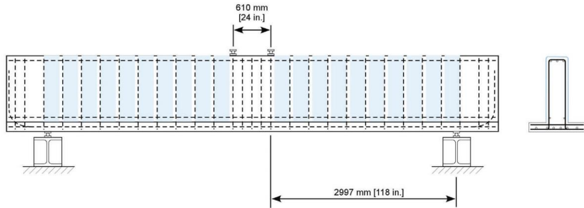
IT Specimen (Typical)
