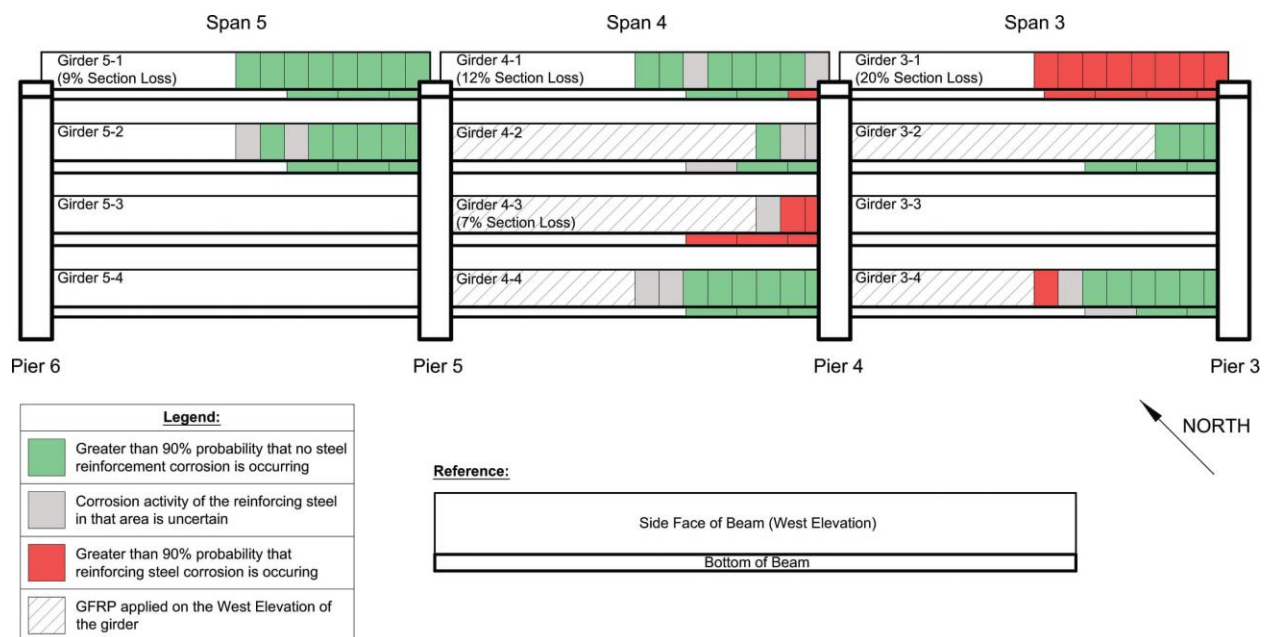
Figure 225—Corrosion potential mapping on girders in spans 3, 4, and 5
