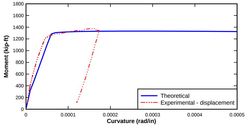
Figure 205—Moment curvature of Girder 5-1
