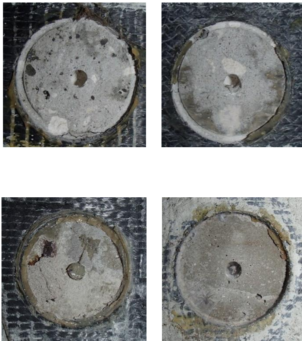
Figure 66—Pull-off test locations on Phillips Lane Bridge indicate adhesive failure modes. It is not known when these pull-off tests were conducted
