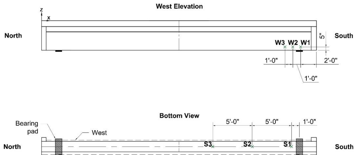
Figure 141—Typical potential testing locations for interior girders
