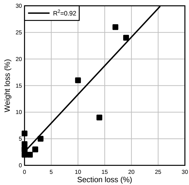
Figure 99—Correlation between weight loss and section loss
