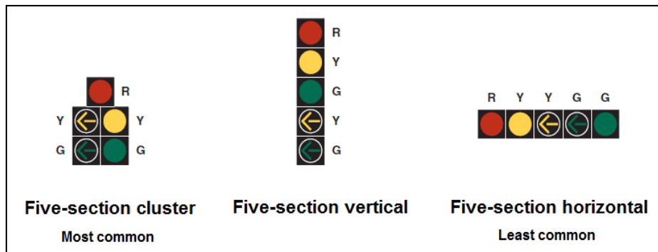
Figure 40. Signal head configurations used in PPLT displays.
