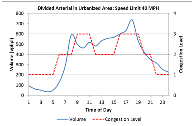
Figure E.3. Time of Day Relationship between Hourly Volumes and Congestion Levels in Divided Urbanized Arterials with Speed Limit 40 MPH
