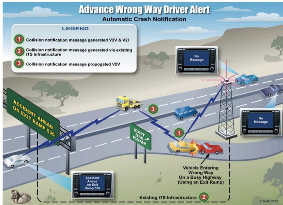
Figure 2-6: Advance Wrong-way Driver Alert – Automatic Crash Notification (Randolph, 2014)
