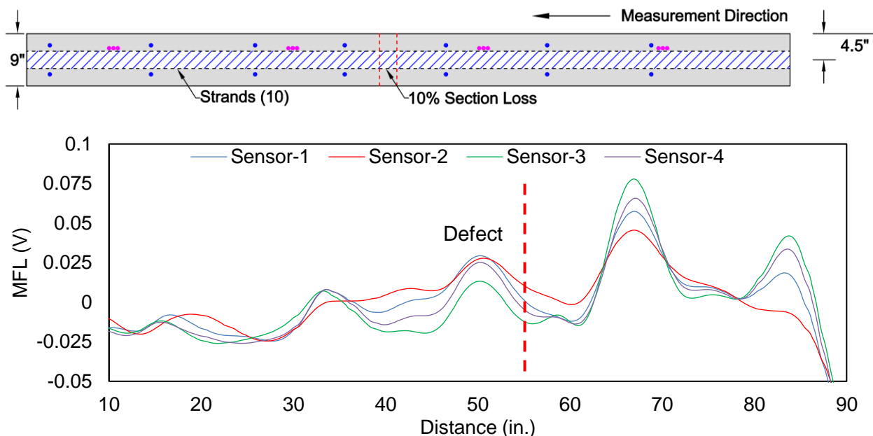
Figure 4-18: Test configuration 15.
