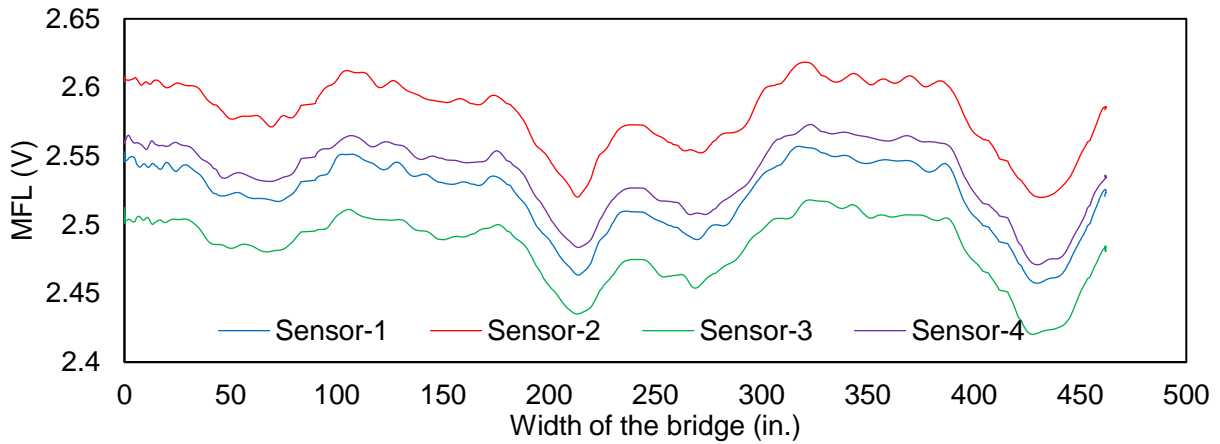
Figure B-8: Span 3, PT rod 1 (test I-S-3-1).
