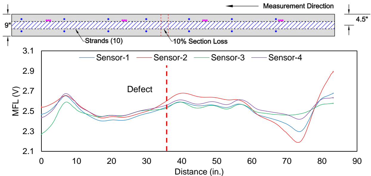
Figure 4-13: Test configuration 11.
