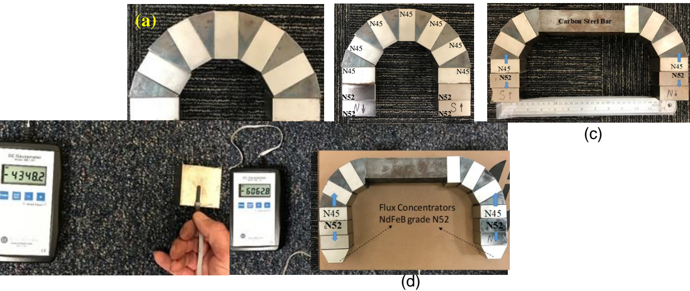
Figure 2-8: Modifications to an earlier version of the magnet.
