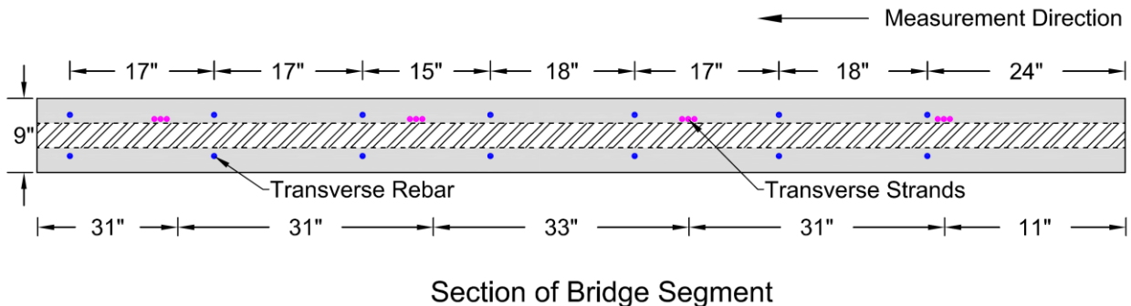
Figure A-9: Location of transverse reinforcement and bundled strands in bridge.
