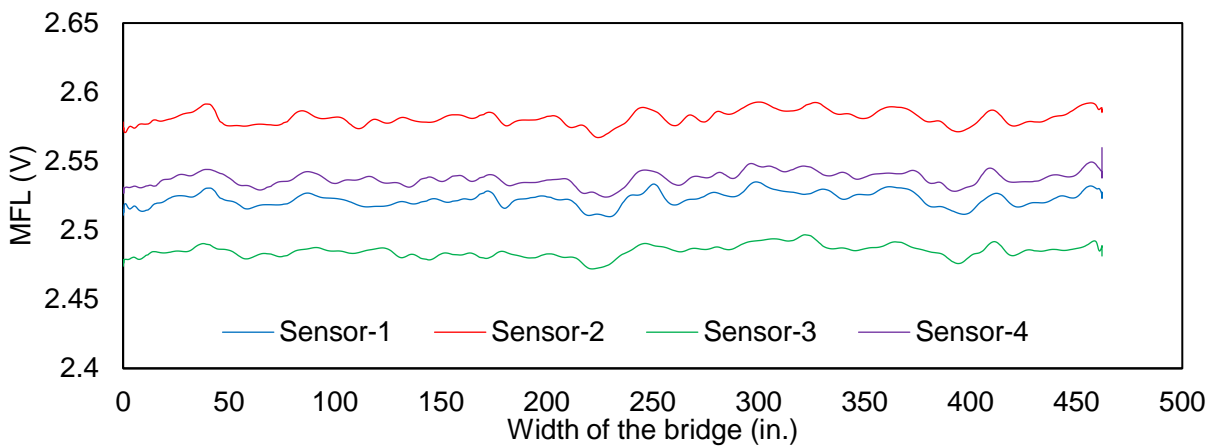
Figure B-9: Span 3 between PT rods (test I-S-3-0).
