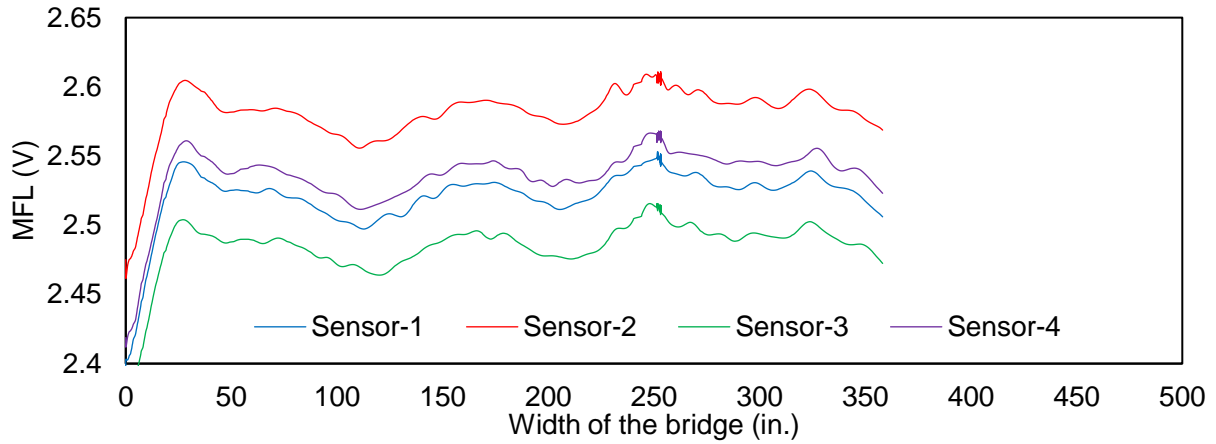
Figure B-7: Span 2, PT rod 2 (test I-S-2-2).
