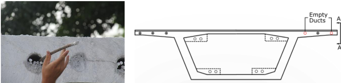
Figure A-8: Empty ducts for testing.
