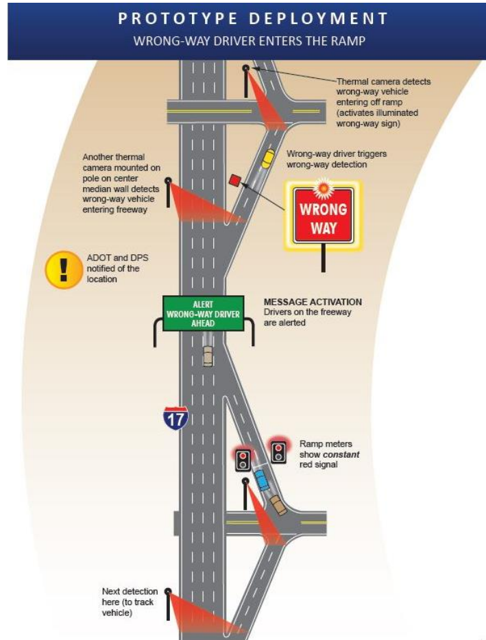
Figure 2-1: Wrong-way Driver Thermal Detection System (ADOT 2017)
