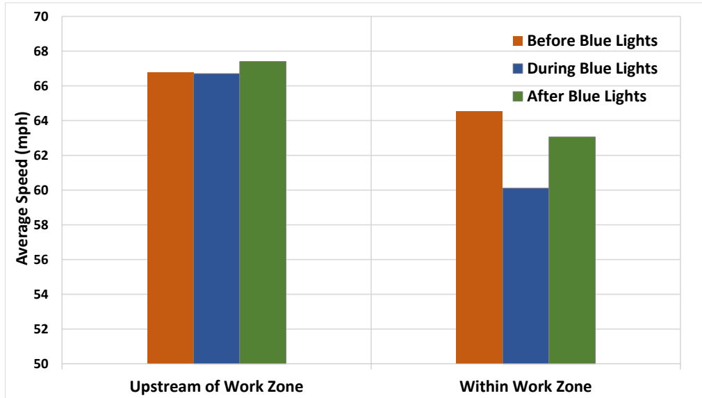
Figure 3-11. Overall Average Speeds Upstream of and within Work Zone
