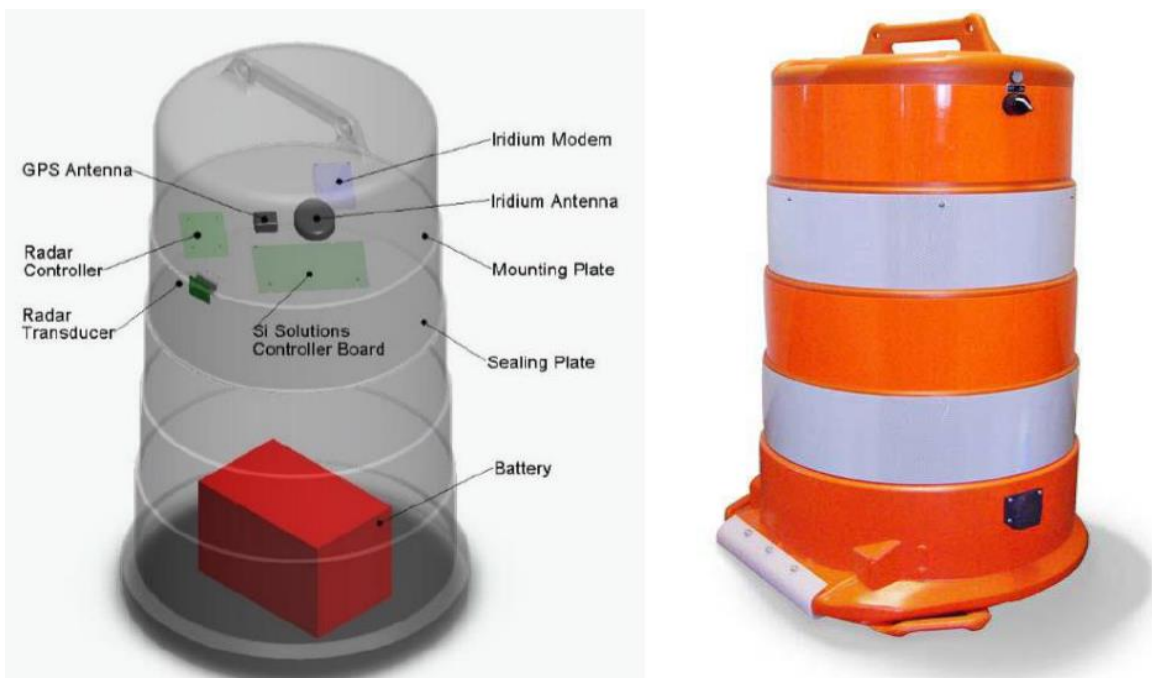
Figure 2-1. iCone Components
