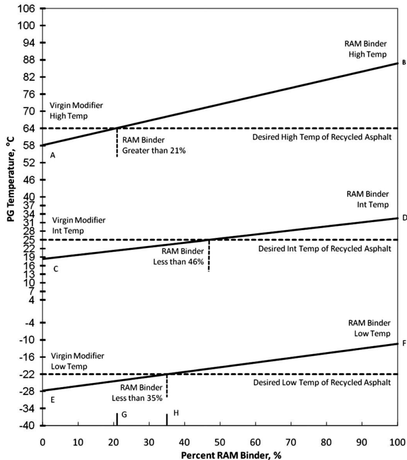
Figure 1-3 Allowed percentage of RAM (RAP) binder based on PG measurements.
