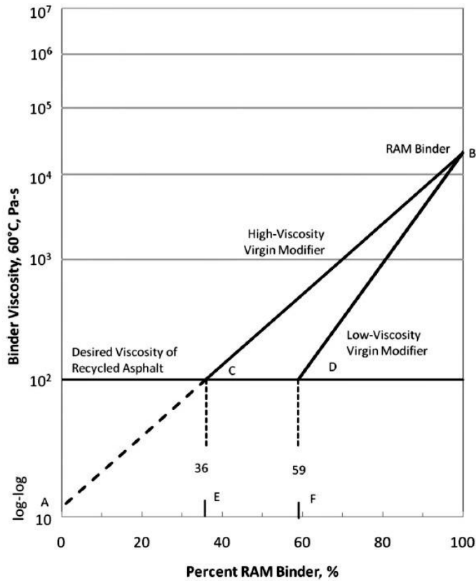
Figure 1-2 Allowed percentage of RAM (RAP) binder based on viscosity (ASTM D4887).
