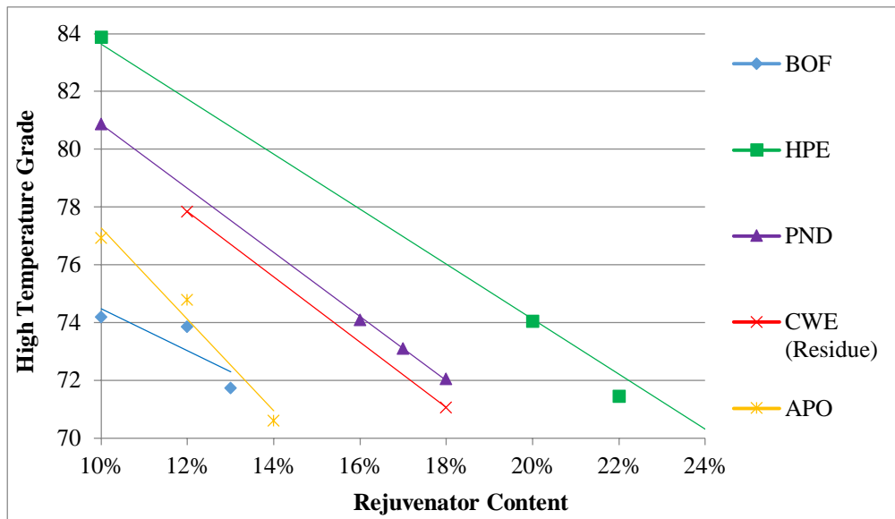
Figure 3-3 Rejuvenator Softening Curves -Binder 1
