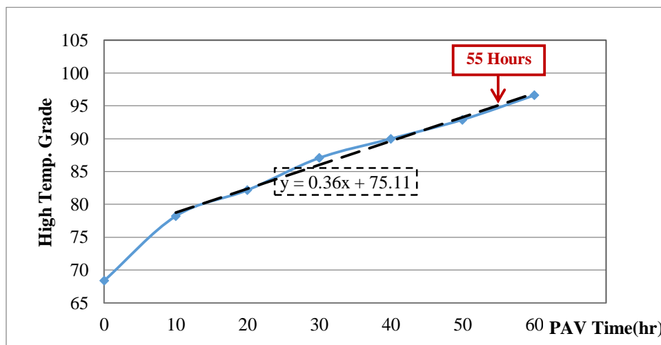
Figure 3-1 Variations of high temperature Grade with PAV time - Binder 1
