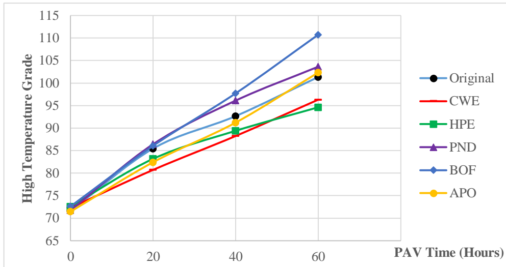
Figure 3-6 Re-aging of rejuvenated binder samples - Binder 2
