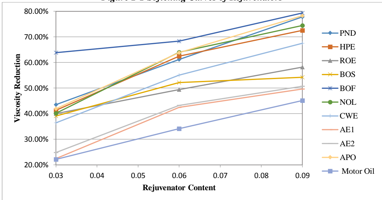
Figure 2-2 Viscosity Reduction of Rejuvenators
