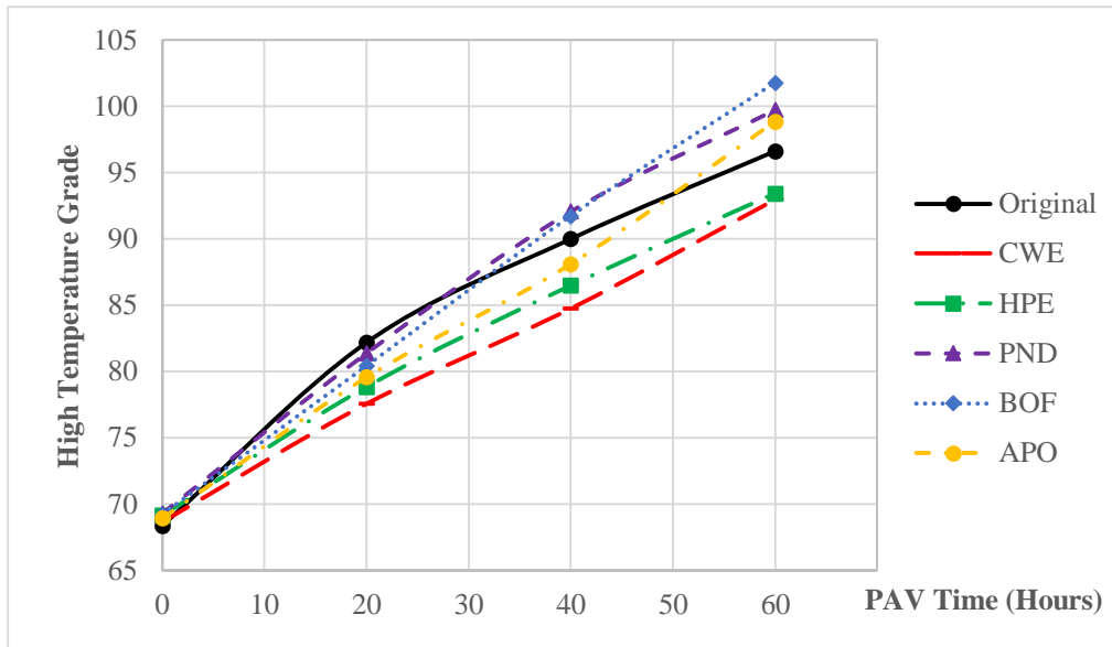
Figure 5-1 Aging of Recycled Binders - Binder1
