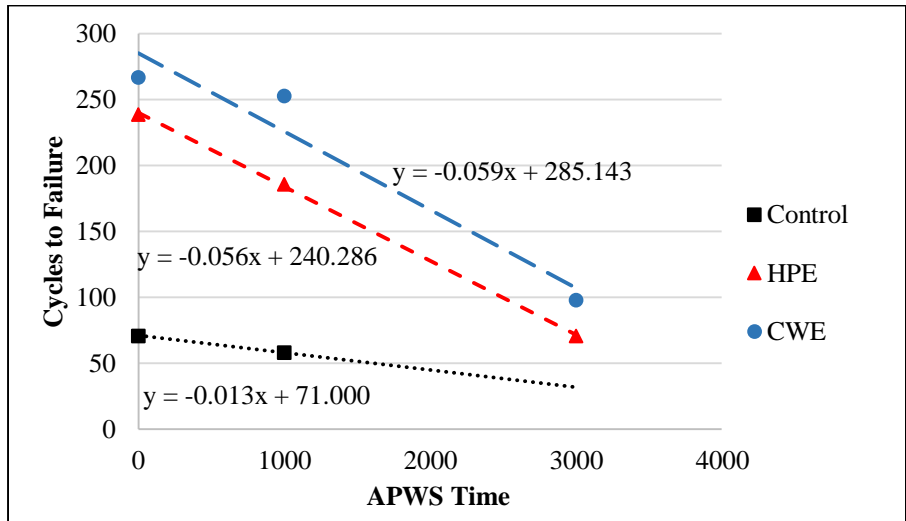
Figure 4-3 Variations of average number of Texas Overlay cycles to failure with APWS aging time
