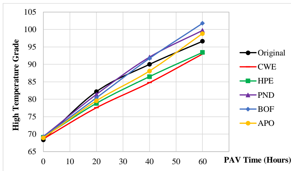
Figure 3-5 Re-aging of rejuvenated binder samples - Binder 1
