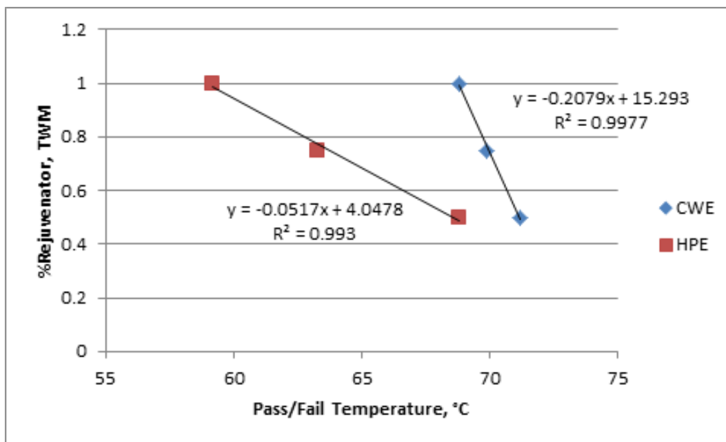
Figure 4-2 Softening curves of rejuvenators mixed with recovered RAP
