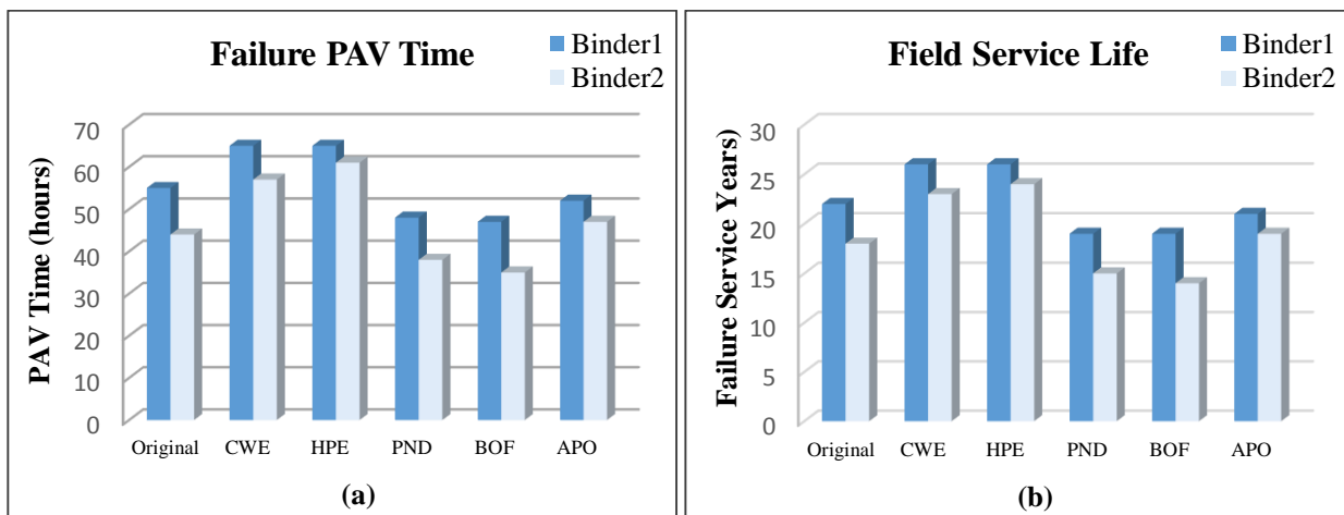
Figure 3-7 Longevity of Rejuvenated Binders Based on (a) Failure PAV Time and (b) Failure Service Years
