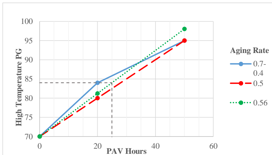
Figure 5-2 Schematic aging behavior of virgin and recycled binders
