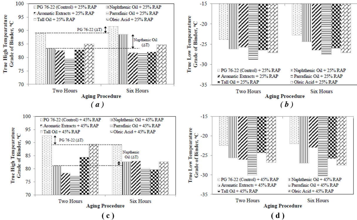
Figure 1-5 True Temperature PG Results for Control and Rejuvenated Binders Extracted from Mixtures Containing 25% RAP; (a) High Temperature PG with 25% RAP, (b) Low Temperature PG with 25% RAP (c) High Temperature PG with 45% RAP, (d) Low Temperature PG with 45% RAP, [32].
