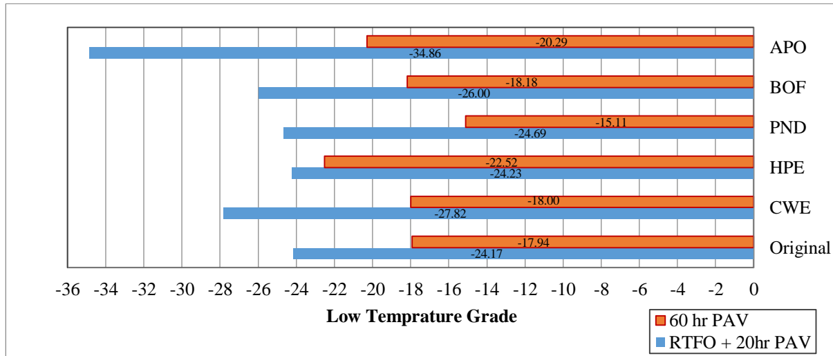
Figure 3-9 Low Temperature Grade Based on BBR m-value – Binder 2
