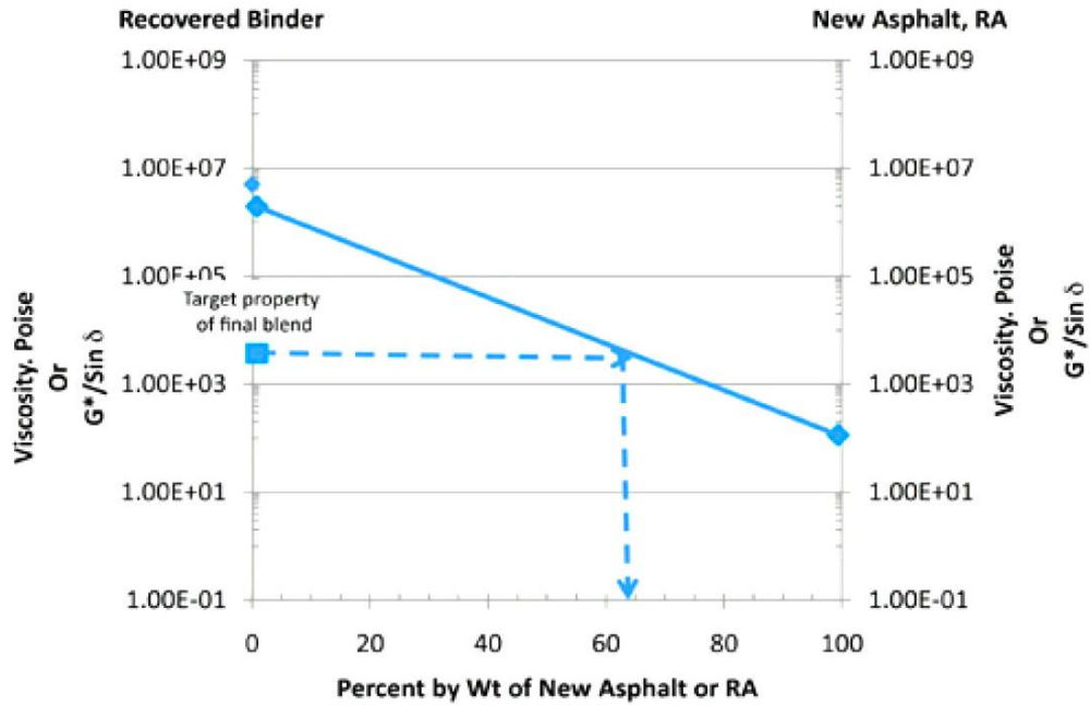
Figure 1-1 Blending chart used to select the percent of new asphalt or RA needed to provide the desired binder properties (based on FHWA 1997) [8].
