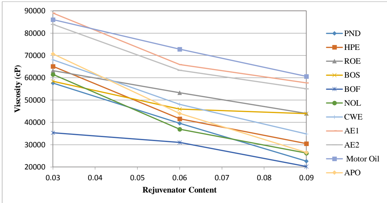
Figure 2-1 Softening Curves of Rejuvenators
