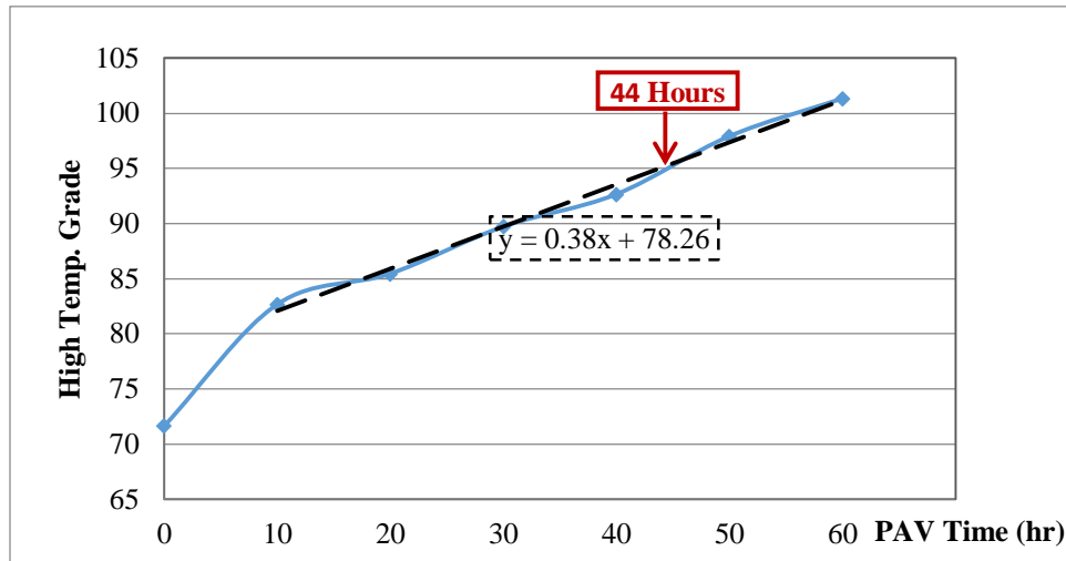
Figure 3-2 Variations of high temperature Grade with PAV time - Binder 2
