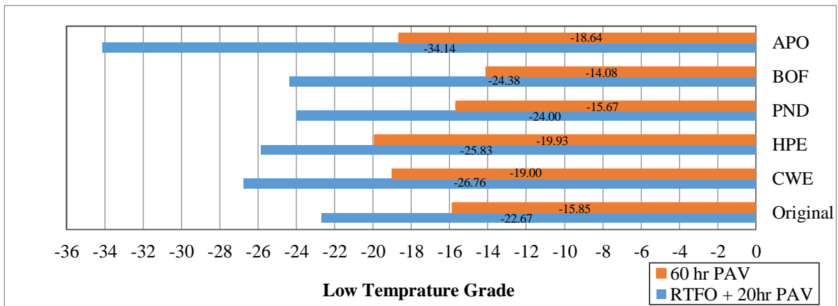
Figure 3-8 Low Temperature Grade Based on BBR m-value – Binder 1
