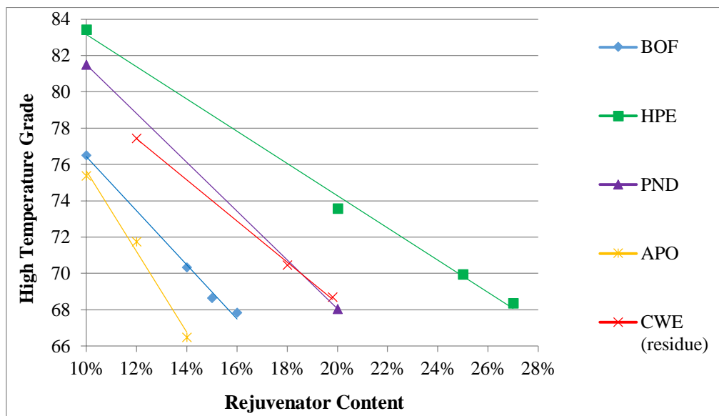
Figure 3-4 Rejuvenator Softening Curves -Binder 2
