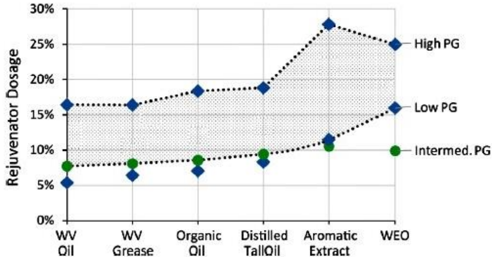
Figure 1-4 Minimum Rejuvenator Dose to Reach PG and Penetration of PG64-22 binder [14]
