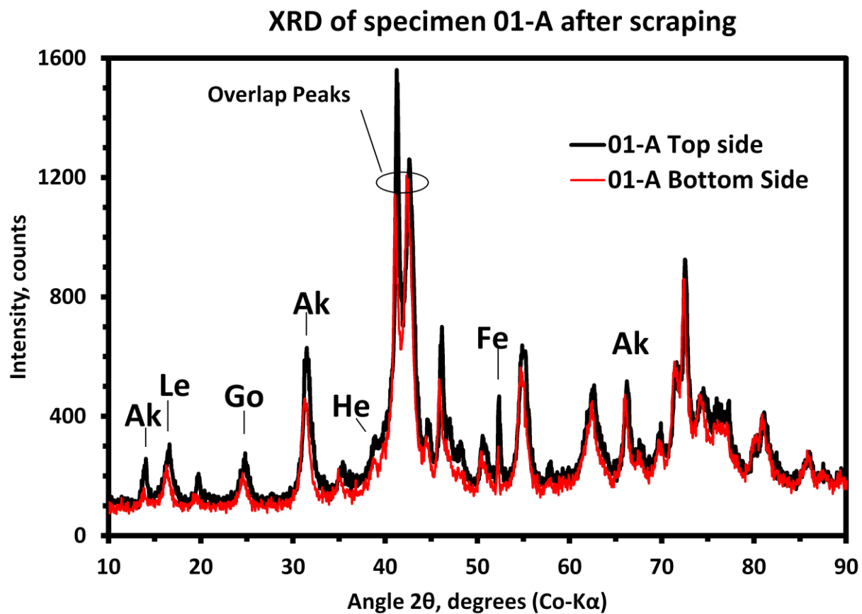
Figure 15: Corrosion products associated with peaks: Ak (akaganeite), Le (lepidocrocite), Go (goethite), He (hematite) and Fe (iron substrate). XRD pattern for top side of specimen (Black) and (Red) for the bottom side. The bottom side showed slightly lower intensities than the top side.
