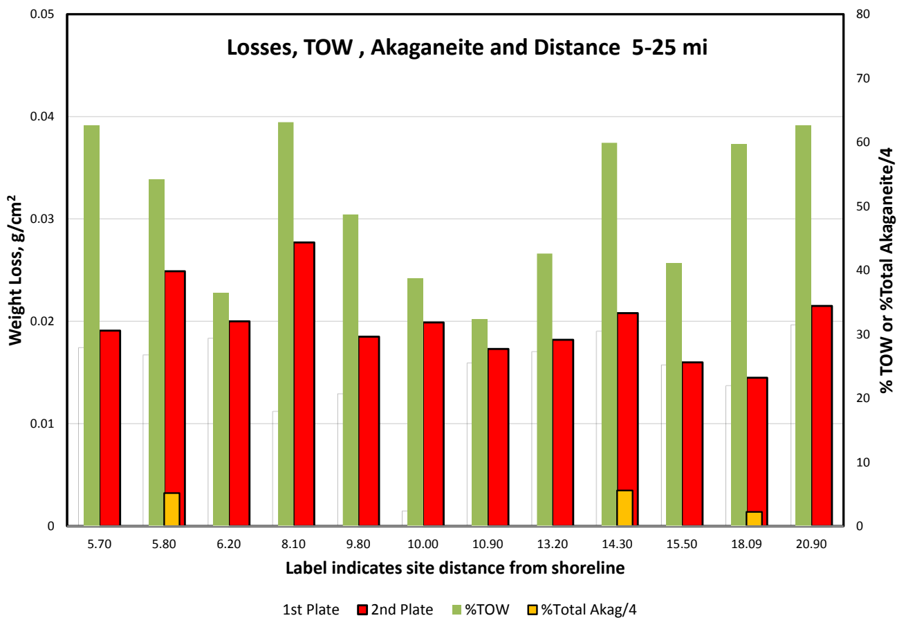
Figure 29: Graphic of corrosion loss, TOW and akaganeite for shoreline distances of 5-25 mi.
