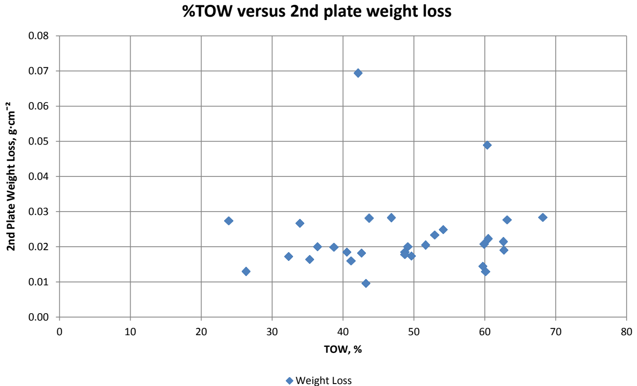
Figure 19: TOW versus weight losses for 2nd plate set.
