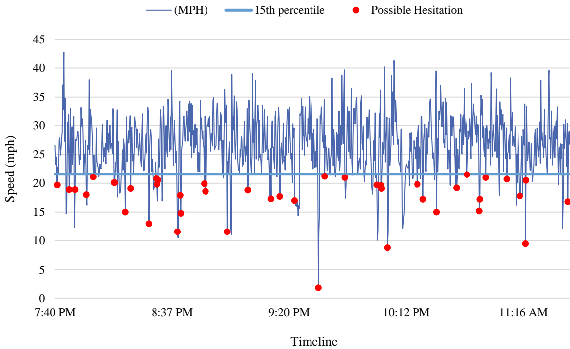
Figure 3-29 Speed profile at W Commercial Blvd @ I-95, Oakland Park, FL (before, night)
