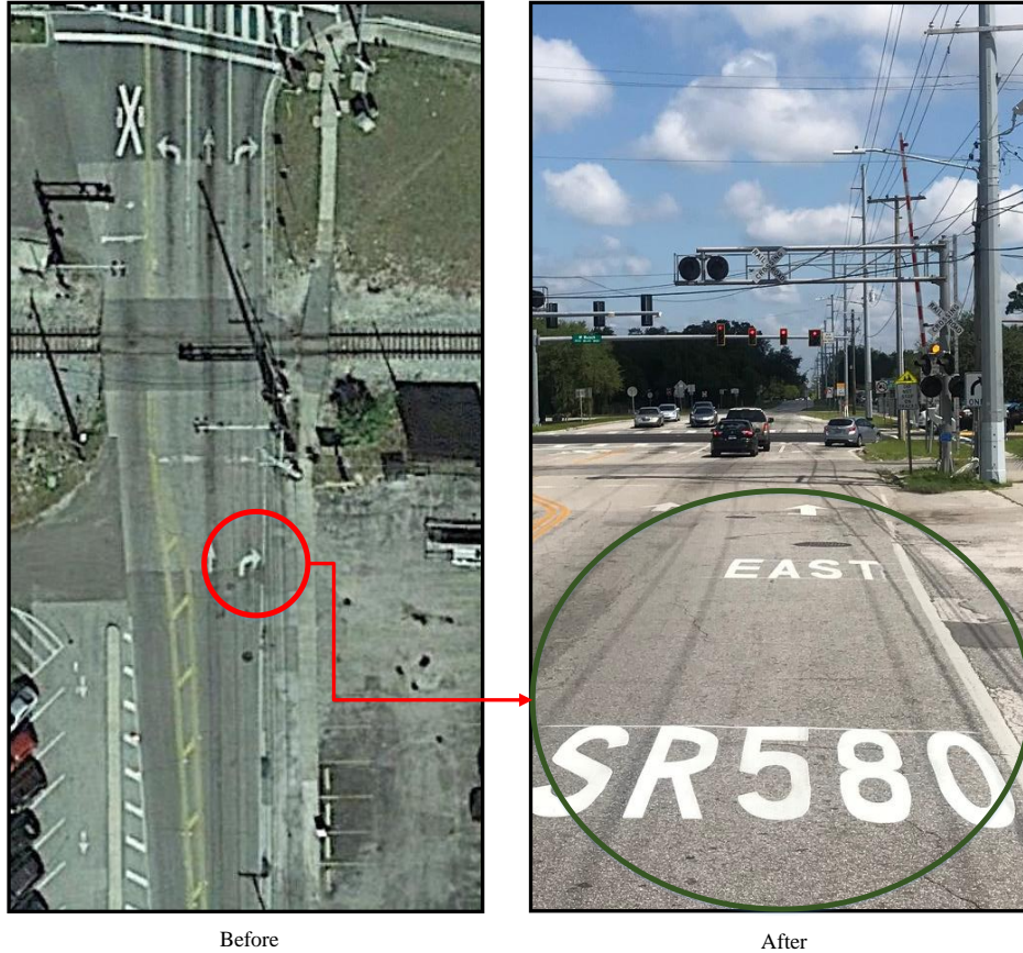
Figure 3-45 Countermeasures implemented at Site 8 (Busch Blvd @ N Boulevard, Tampa, FL)
