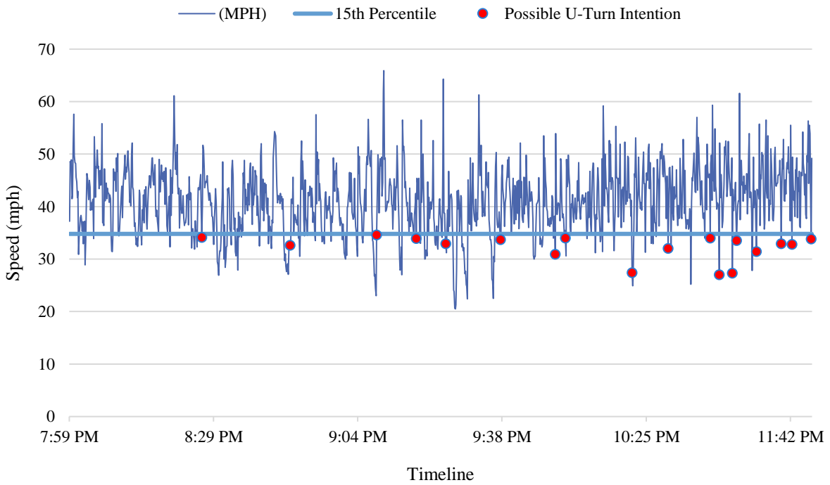
Figure 3-4 Speed profile at US-41 @ US-301, Bradenton, FL (before, night)
