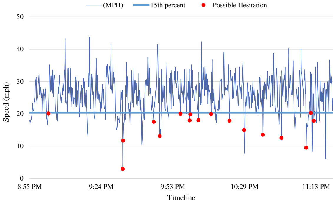
Figure 3-31 Speed profile at W Commercial Blvd @ I-95, Oakland Park, FL (after, night)
