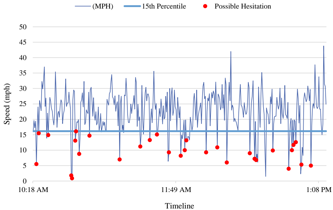
Figure 3-24 Speed profile at W Hallandale Beach Blvd @ I-95, Pembroke Park, FL (after, day)
