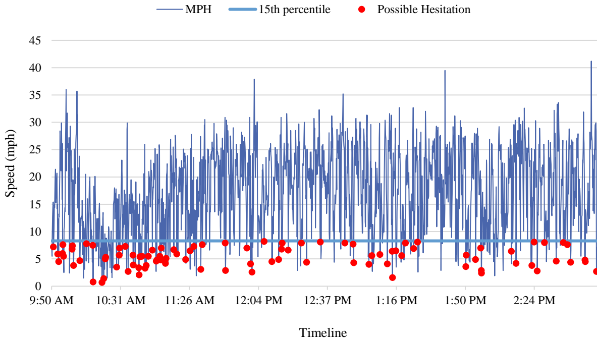
Figure 3-16 Speed profile at Forest Hill Blvd @ I-95, Lake Clarke Shores, FL (before, day)
