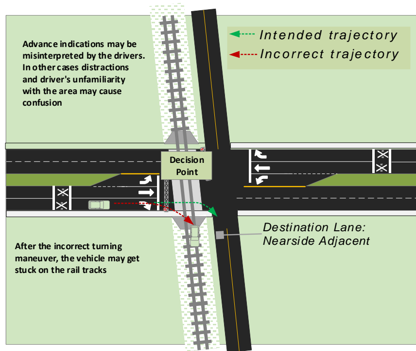
Figure 1-1 Illustration of incorrect turning maneuver near an intersection
