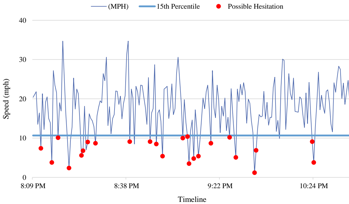
Figure 3-49 Speed profile at Busch Blvd @ N Boulevard, Tampa, FL (after, night)
