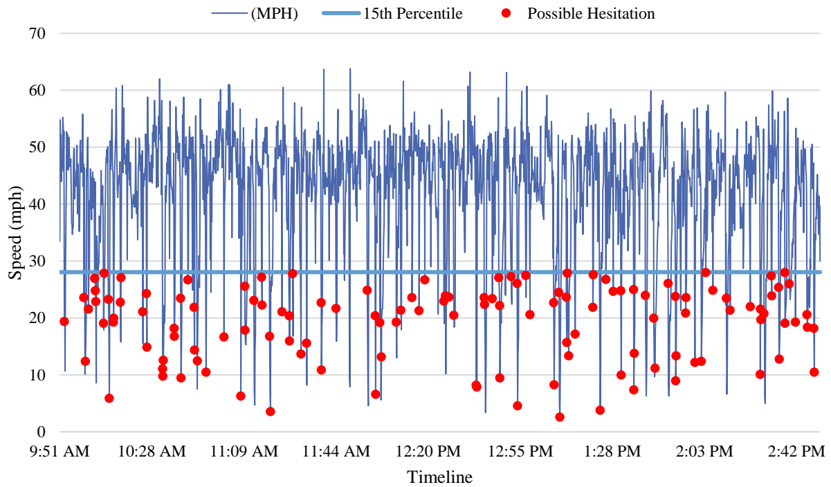
Figure 3-41 Speed profile at Tampa Rd @ State St W, Oldsmar, FL (before, night)
