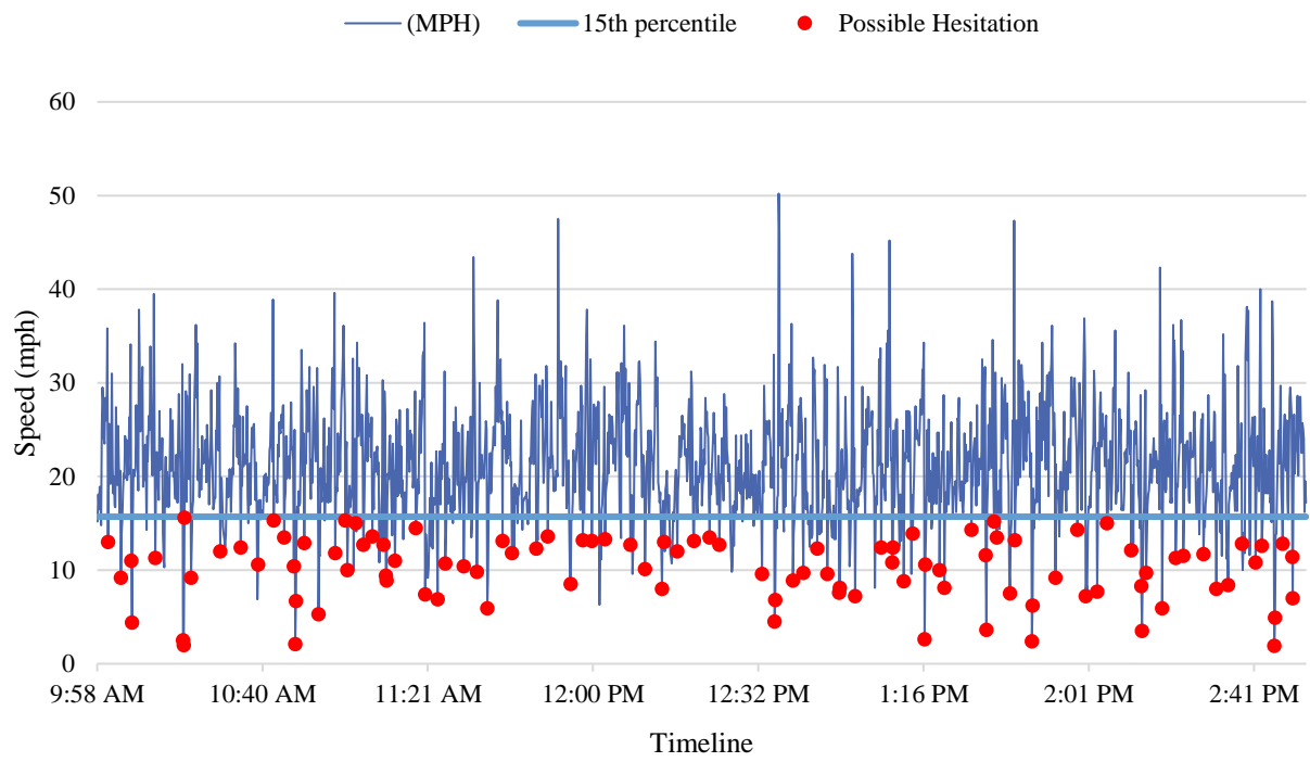
Figure 3-10 Speed profile at Hollywood Blvd @ I-95 (before, daytime)
