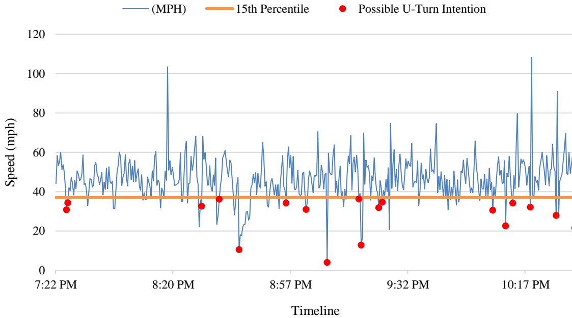
Figure 3-6 Speed profile at US-41 @ US-301, Bradenton, FL (after, nighttime)
