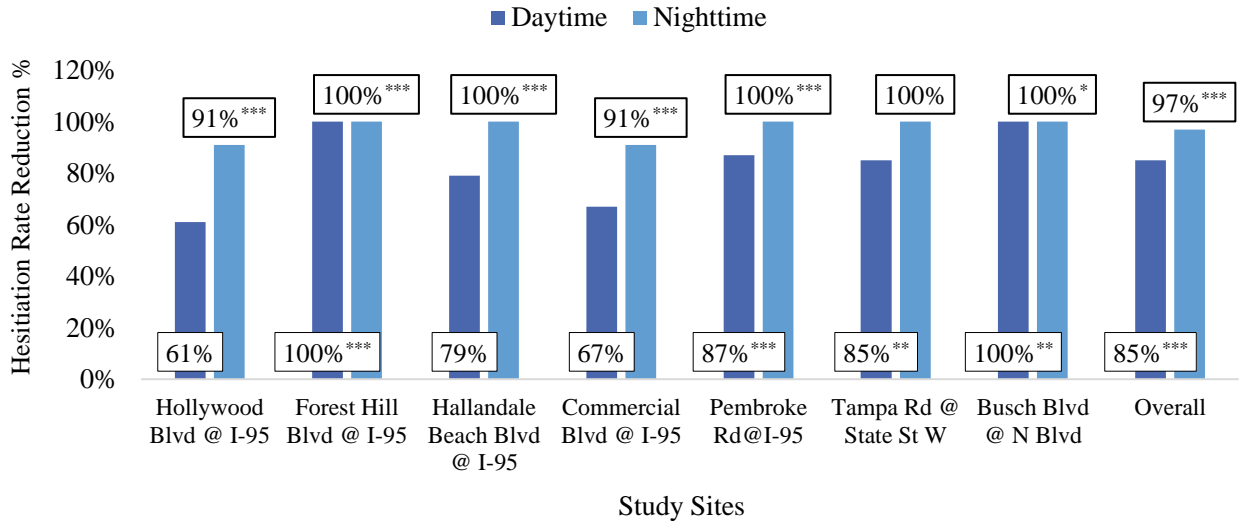
Figure ES-1 Relative reduction of hesitation rates for pavement marking of straight arrow plus guidance information
