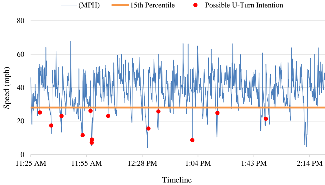
Figure 3-5 Speed profile at US-41 @ US-301, Bradenton, FL (after, daytime)
