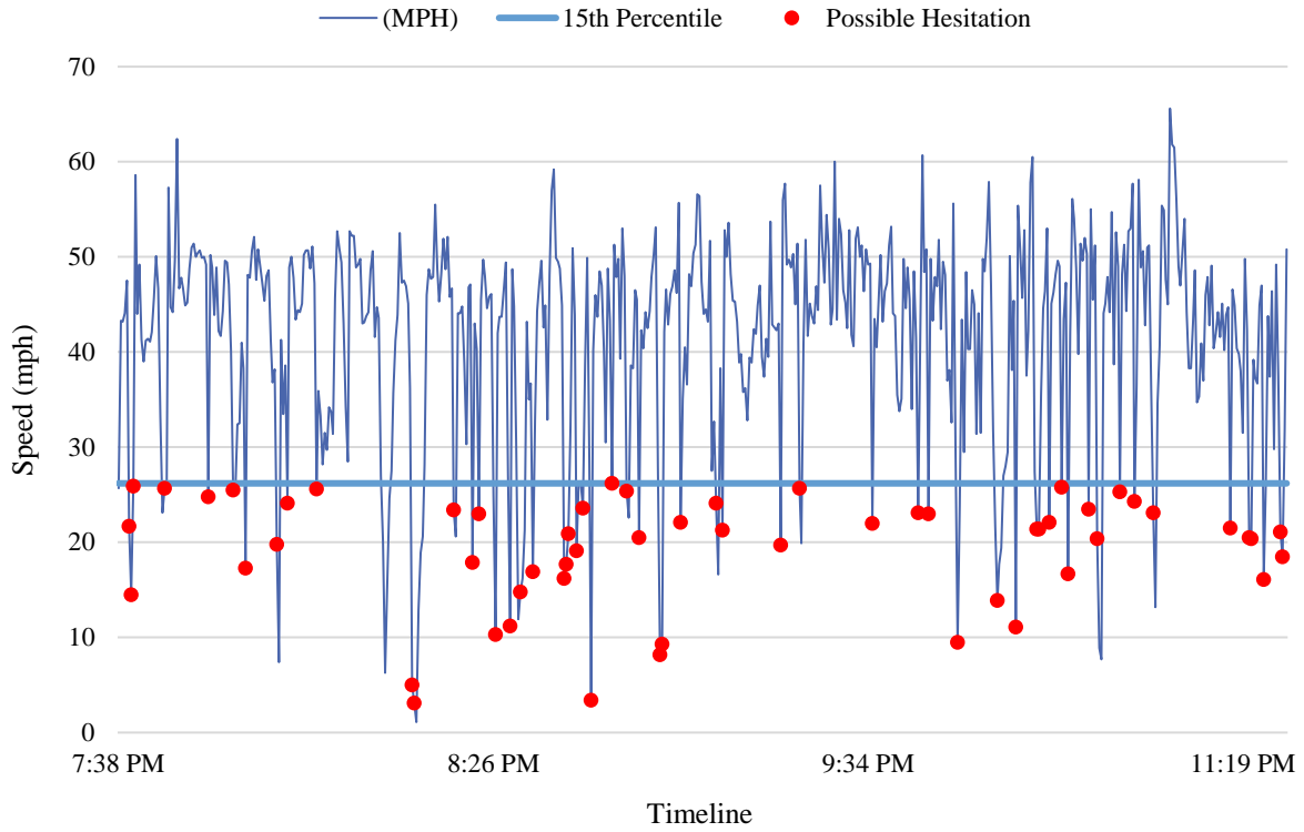
Figure 3-40 Speed profile at Tampa Rd @ State St W, Oldsmar, FL (before, day)
