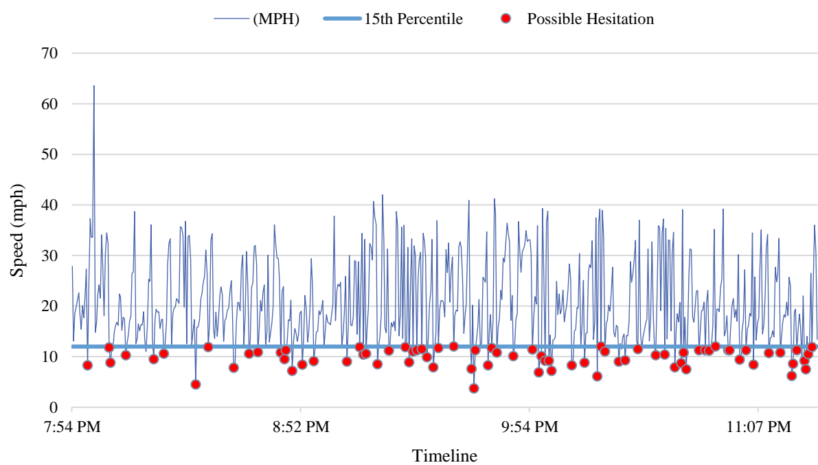
Figure 3-37 Speed profile at W Pembroke Rd @ I-95, Hollywood (after, night)
