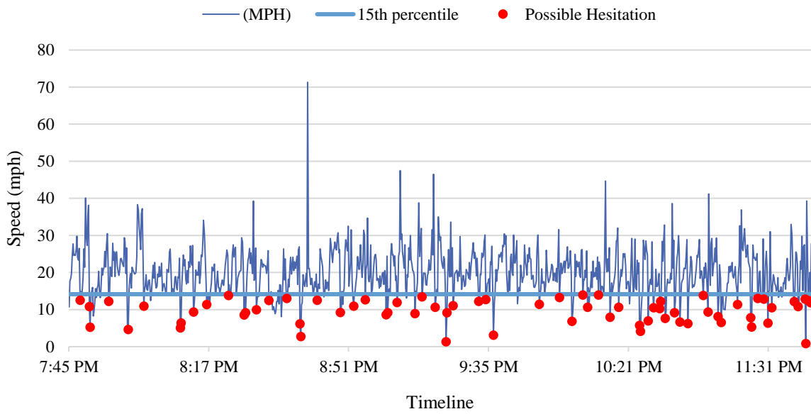
Figure 3-11 Speed profile at Hollywood Blvd @ I-95 (before, nighttime)
