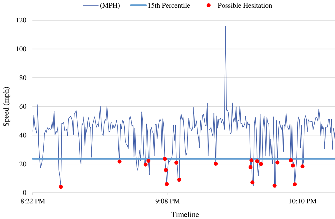
Figure 3-43 Speed profile at Tampa Rd @ State St W, Oldsmar, FL (night)
