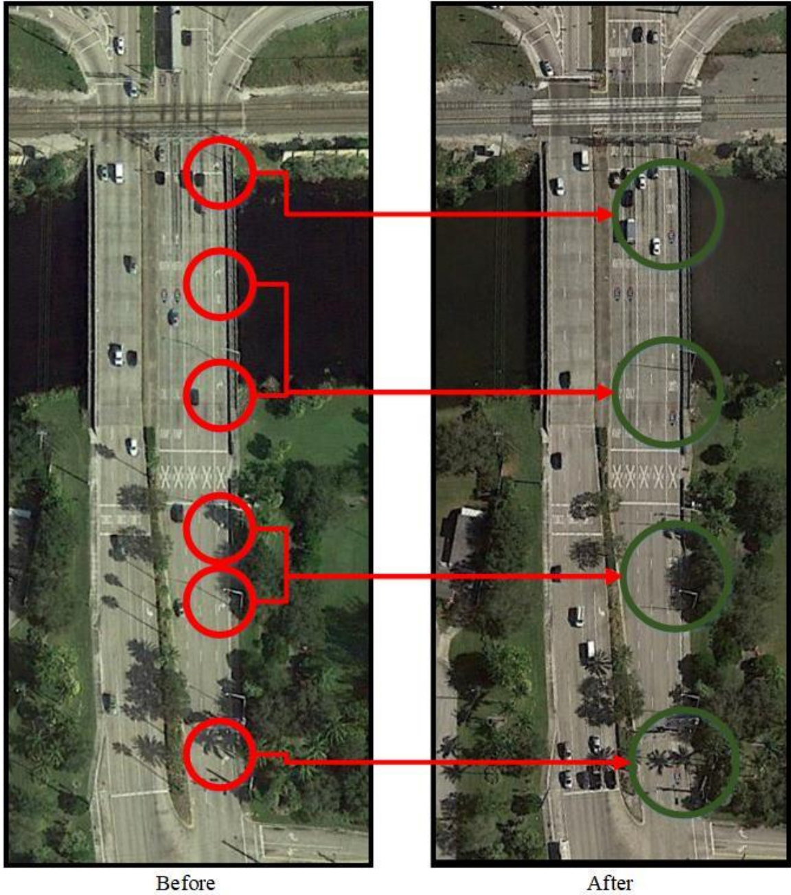
Figure 3-15 Countermeasures implemented at Site 3 (Forest Hill Blvd @ I-95, Lake Clarke Shores, FL)
