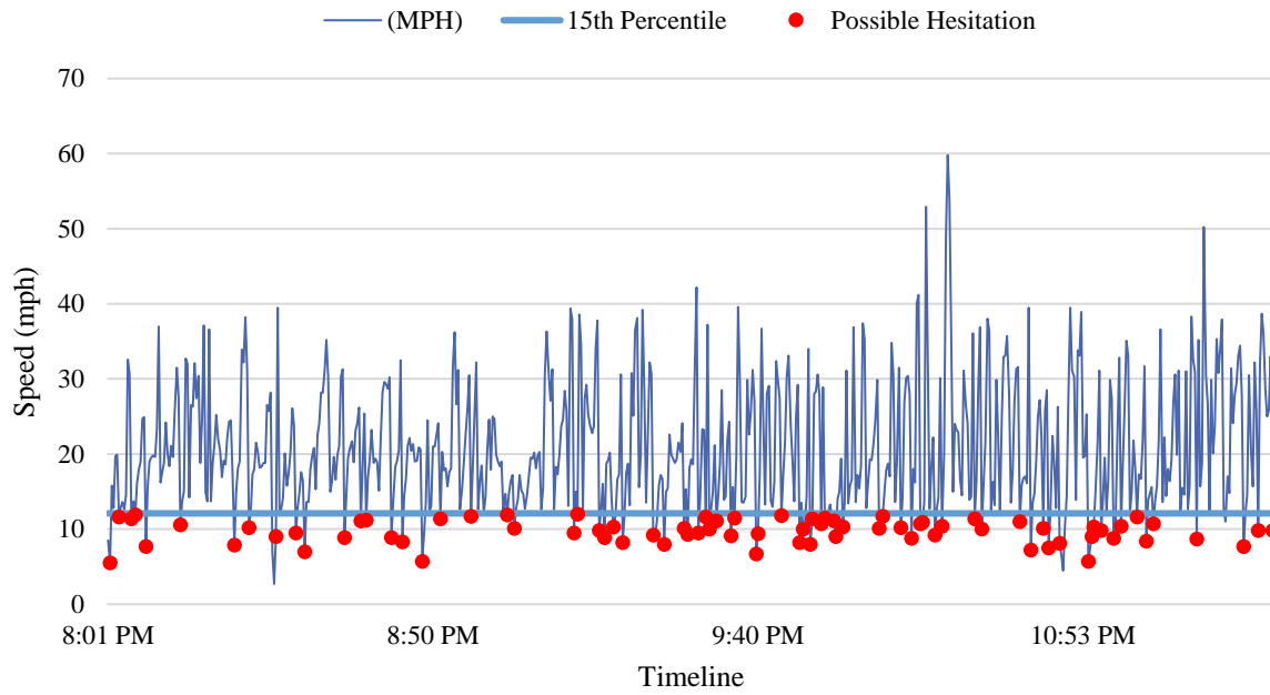
Figure 3-35 Speed profile at W Pembroke Rd @ I-95, Hollywood (before, night)
