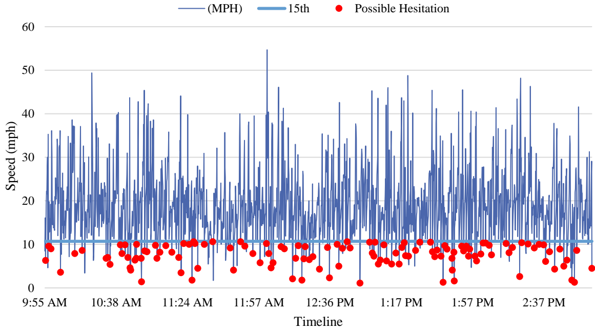
Figure 3-34 Speed profile at W Pembroke Rd @ I-95, Hollywood (before, day)
