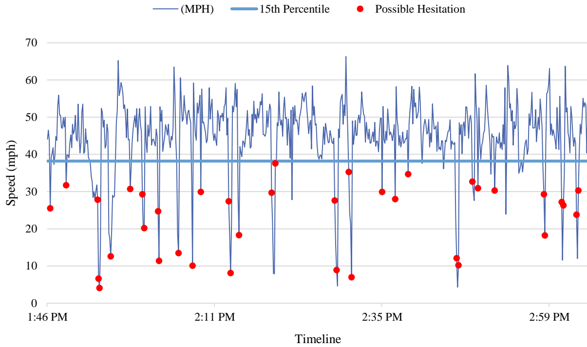
Figure 3-42 Speed profile at Tampa Rd @ State St W, Oldsmar, FL (after, day)
