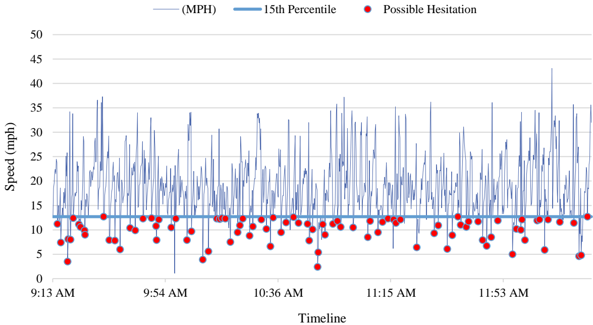
Figure 3-36 Speed profile at W Pembroke Rd @ I-95, Hollywood (after, day)
