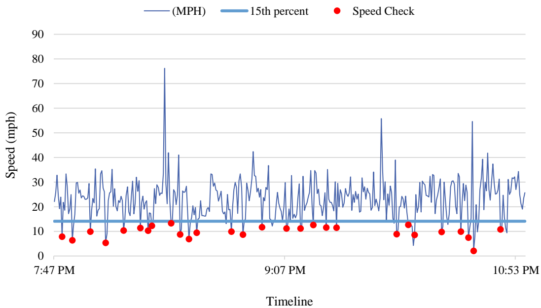
Figure 3-25 Speed profile at W Hallandale Beach Blvd @ I-95, Pembroke Park, FL (after, night)
