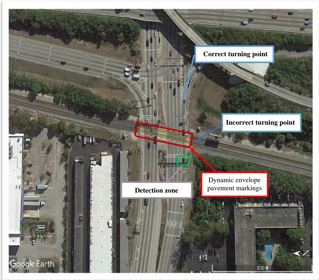
Figure 3-26 Layout of Site 5 (W Commercial Blvd @ I-95)
