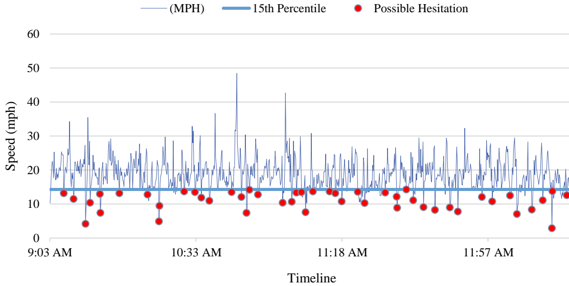
Figure 3-12 Speed profile at Hollywood Blvd @ I-95 (after, daytime)
