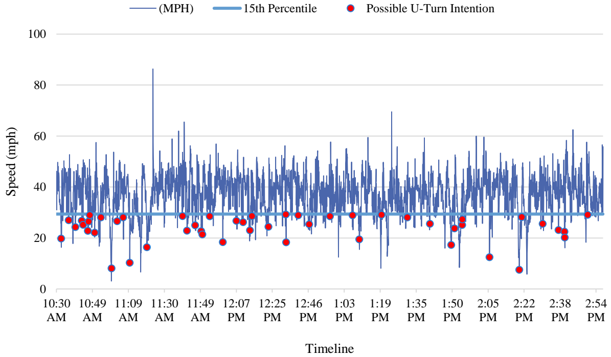
Figure 3-3 Speed profile at US-41 @ US-301, Bradenton, FL (before, daytime)
