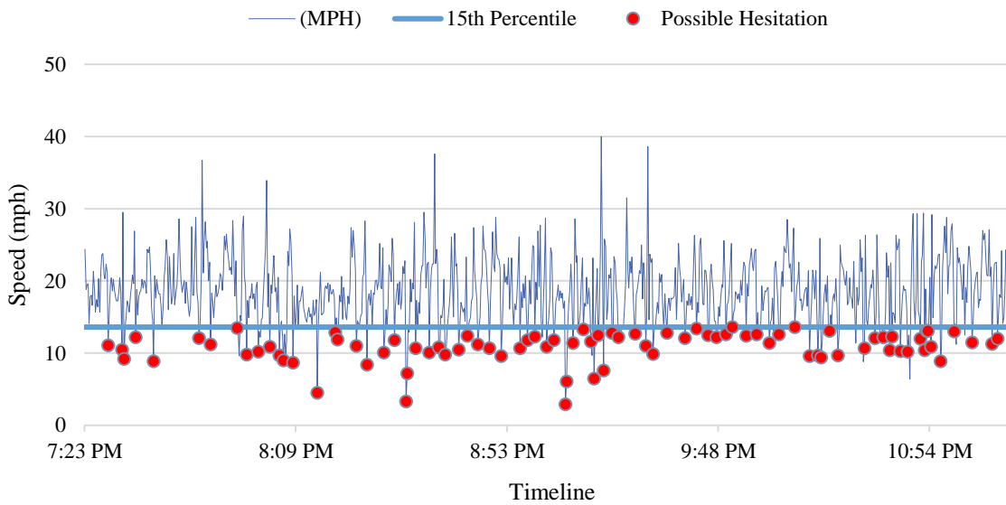
Figure 3-13 Speed profile at Hollywood Blvd @ I-95 (after, nighttime)
