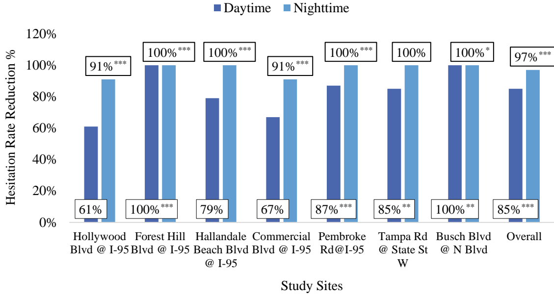
Figure 3-50 Relative reduction of hesitation rates for pavement marking of straight arrow plus guidance information
