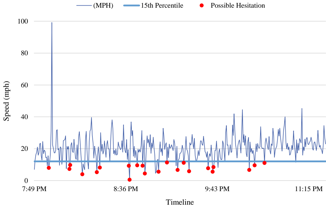
Figure 3-47 Speed profile at Busch Blvd @ N Boulevard, Tampa, FL (before, night)
