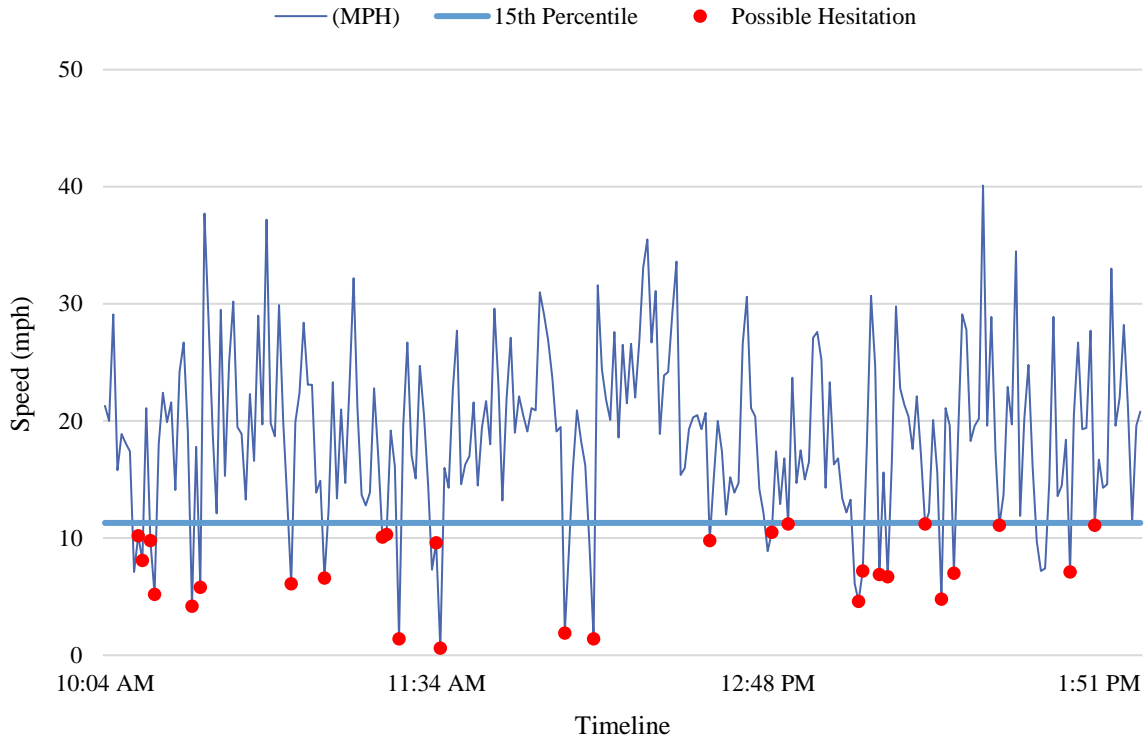
Figure 3-46 Speed profile at Busch Blvd @ N Boulevard, Tampa, FL (before, day)
