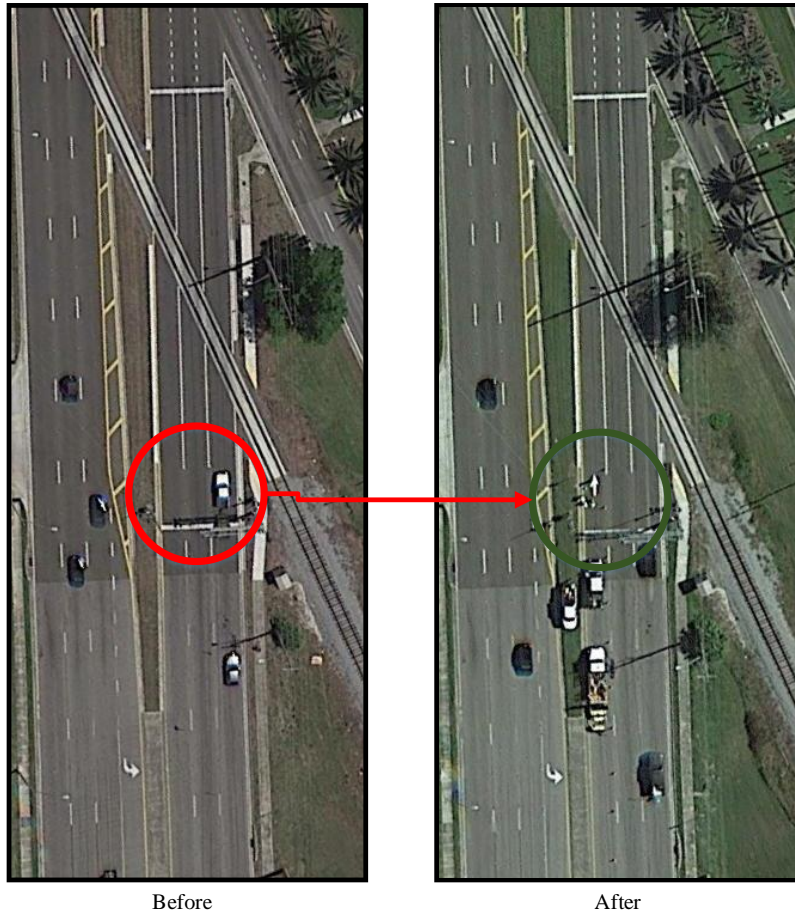
Figure 3-39 Countermeasures implemented at Site 7 (Tampa Rd @ State St W, Oldsmar, FL)
