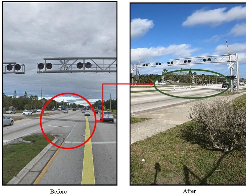
Figure 3-2 Countermeasure implemented at Site 1 (US-41@ US-301, Bradenton, FL)
