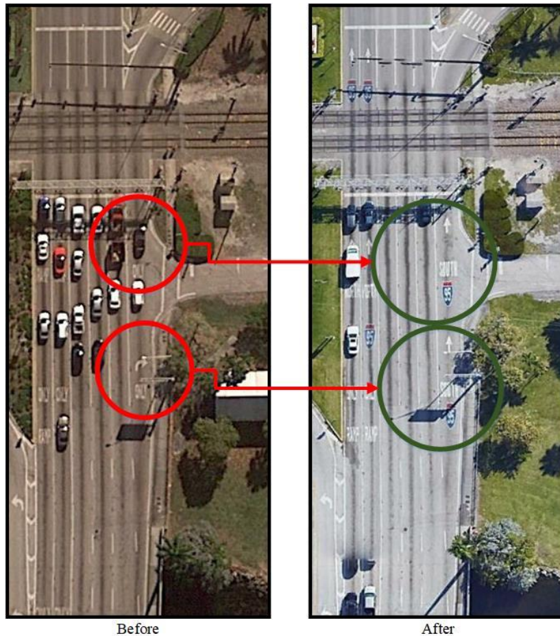
Figure 3-9 Countermeasures implemented at Site 2 (Hollywood Blvd @ I-95, Hollywood, FL)
