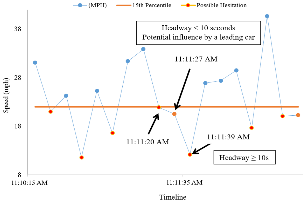
Figure 2-4 Example of visualization of Wavetronix speed data and potential hesitation filter
