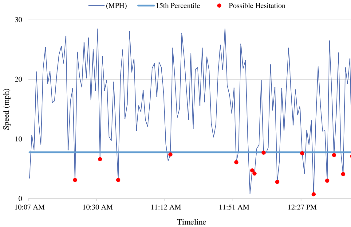
Figure 3-48 Speed profile at Busch Blvd @ N Boulevard, Tampa, FL (after, day)
