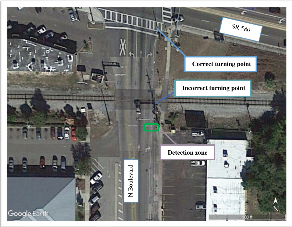
Figure 3-44 Layout of Site 8 (Busch Blvd @ N Boulevard)
