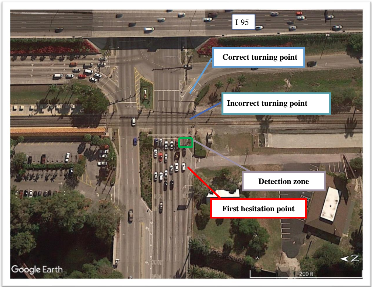
Figure 3-8 Layout of Site 2 (Hollywood Blvd @ I-95)
