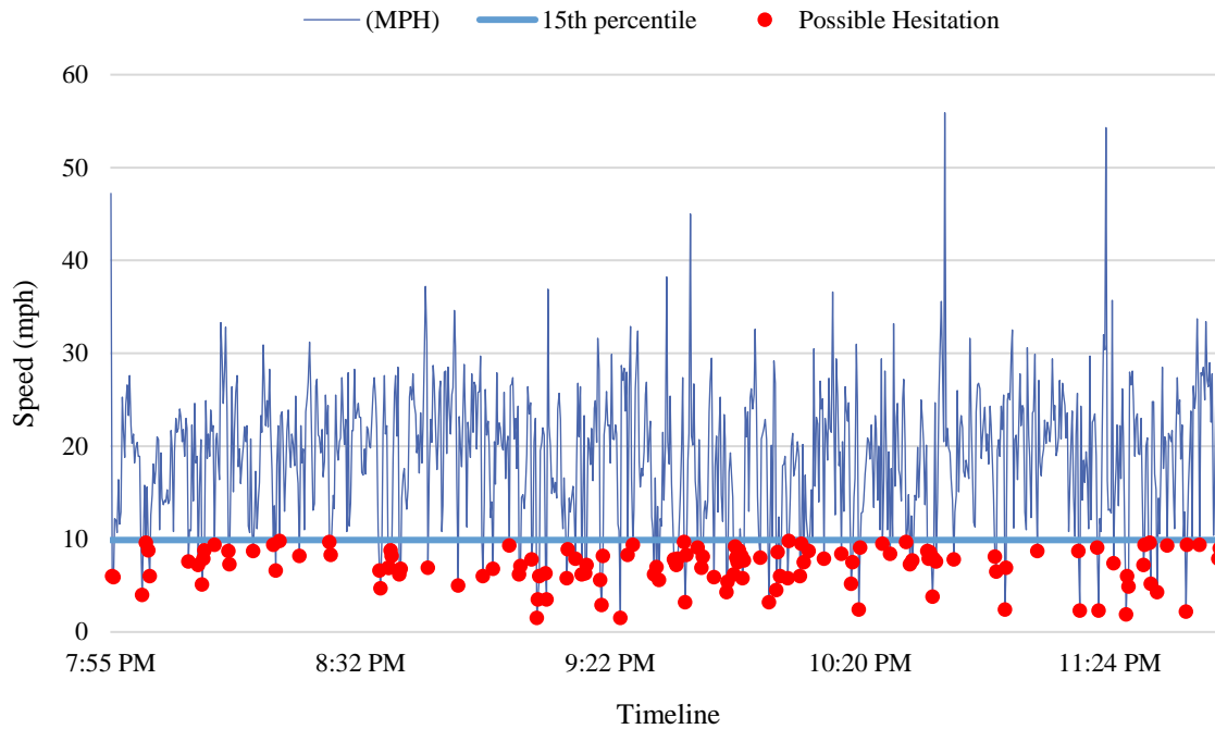
Figure 3-17 Speed profile at Forest Hill Blvd @ I-95, Lake Clarke Shores, FL (before, night)
