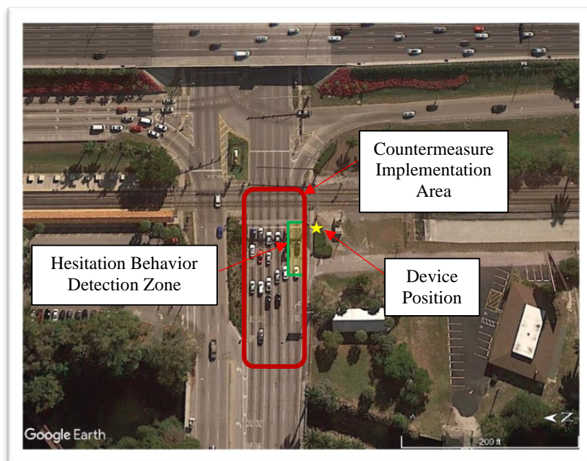
Figure 2-2 Example of data collection layout
