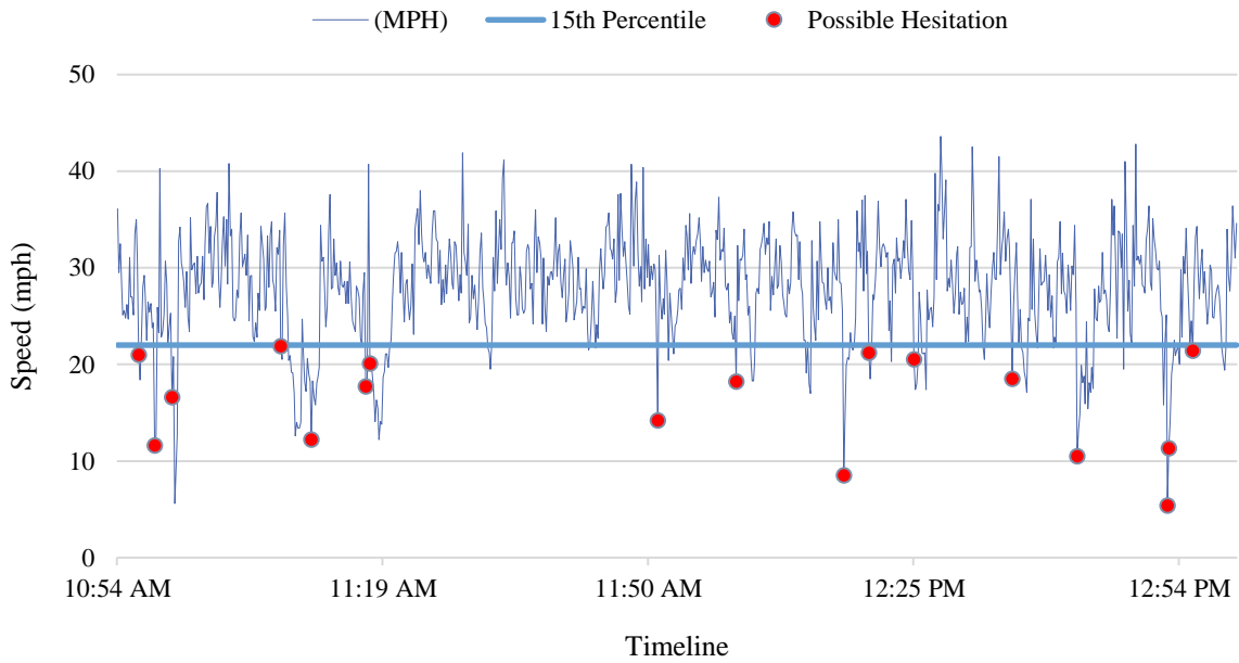
Figure 3-30 Speed profile at W Commercial Blvd @ I-95, Oakland Park, FL (after, day)
