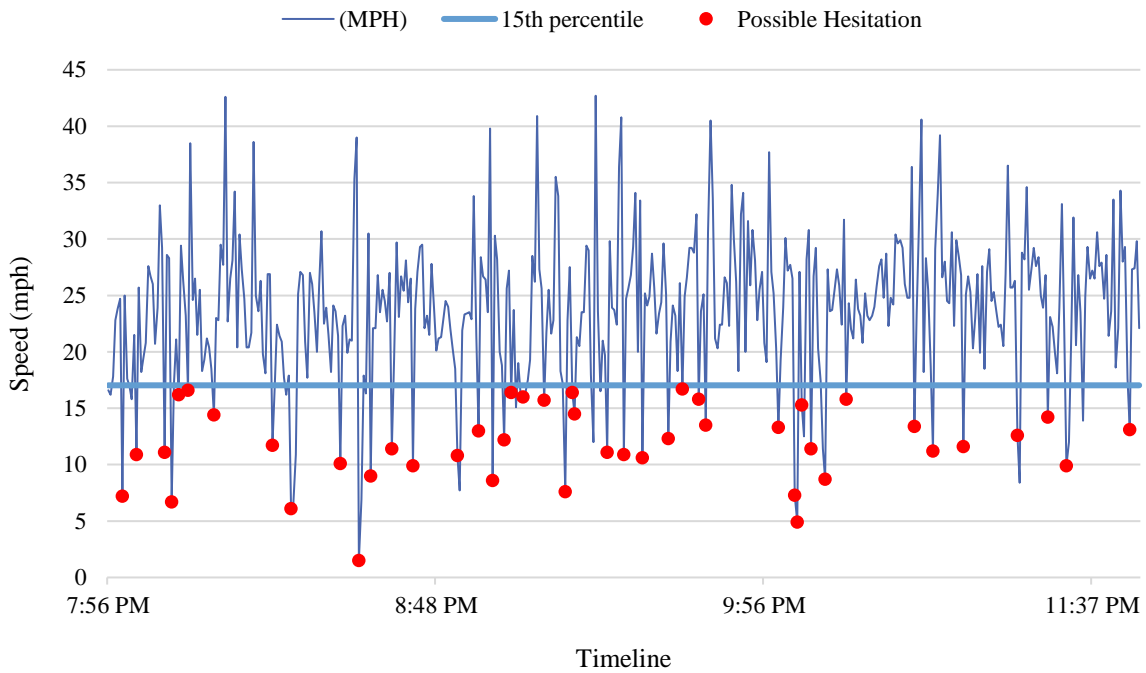
Figure 3-23 Speed profile at W Hallandale Beach Blvd @ I-95, Pembroke Park, FL (before, night)
