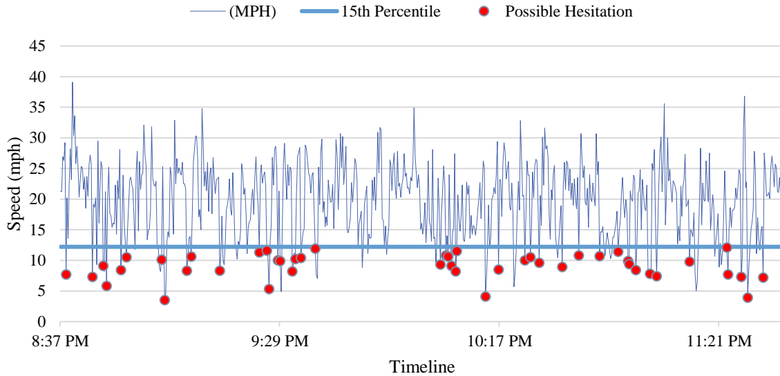
Figure 3-19 Speed profile at Forest Hill Blvd @ I-95, Lake Clarke Shores, FL (after, night)
