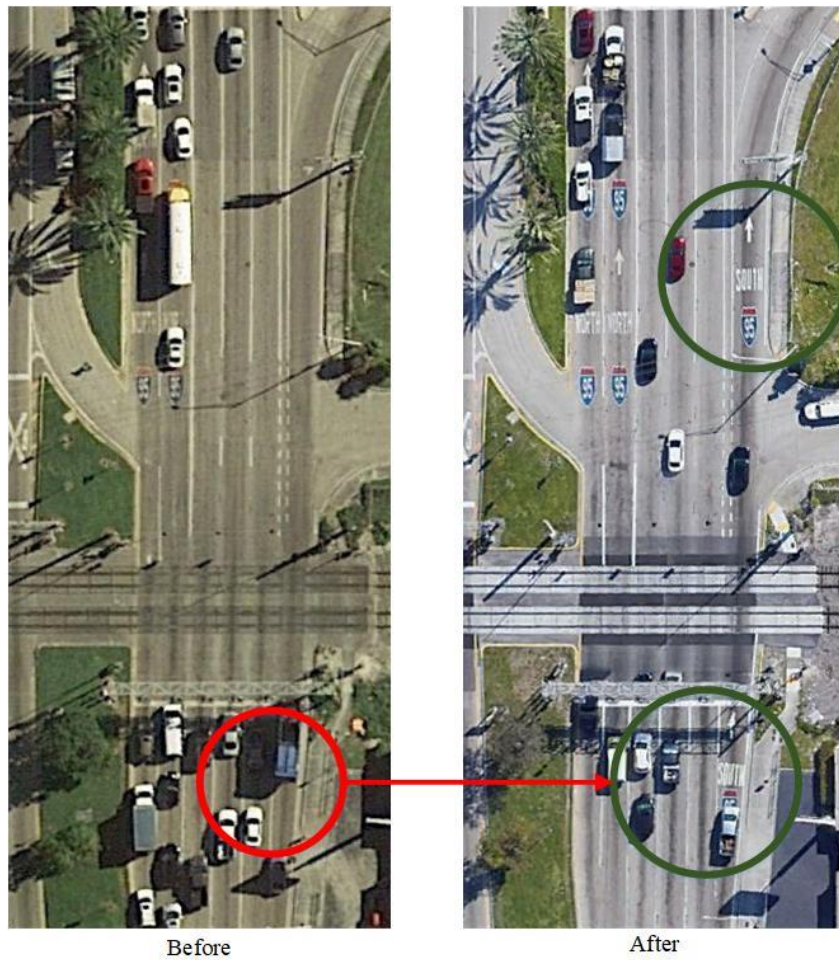
Figure 3-33 Countermeasures implemented at Site 6 (W Pembroke Rd @ I-95, Hollywood, FL)
