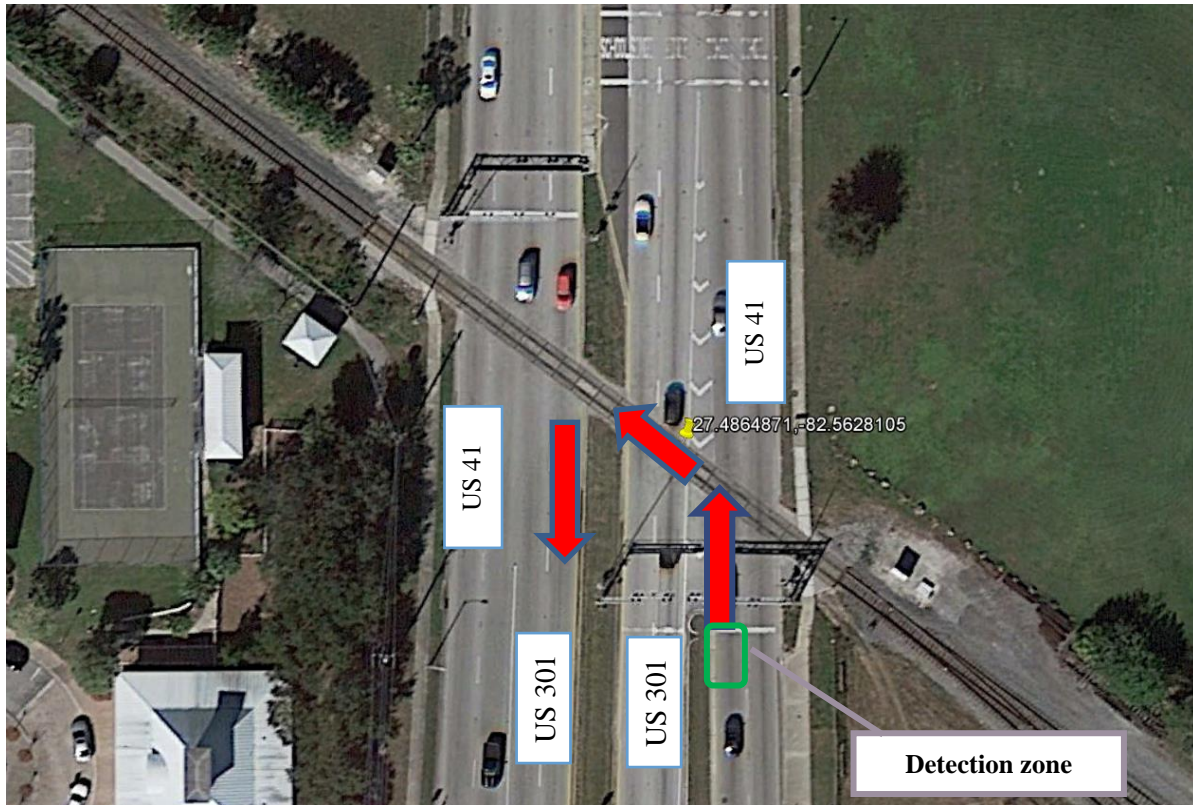
Figure 3-1 Potential incorrect U-turns at Site 1 (US-41 @ US-301, Bradenton, FL)
