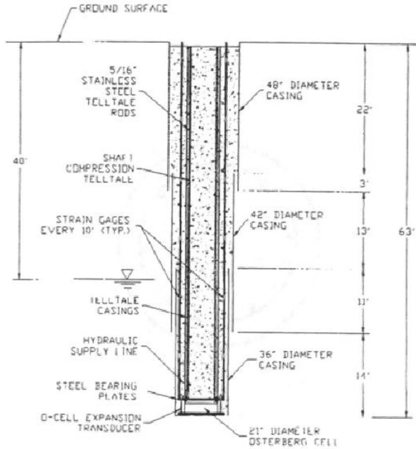
Figure 2.33 Scheme of the test shaft instrumented at CRC facility project (Hossain et al., 2007).
