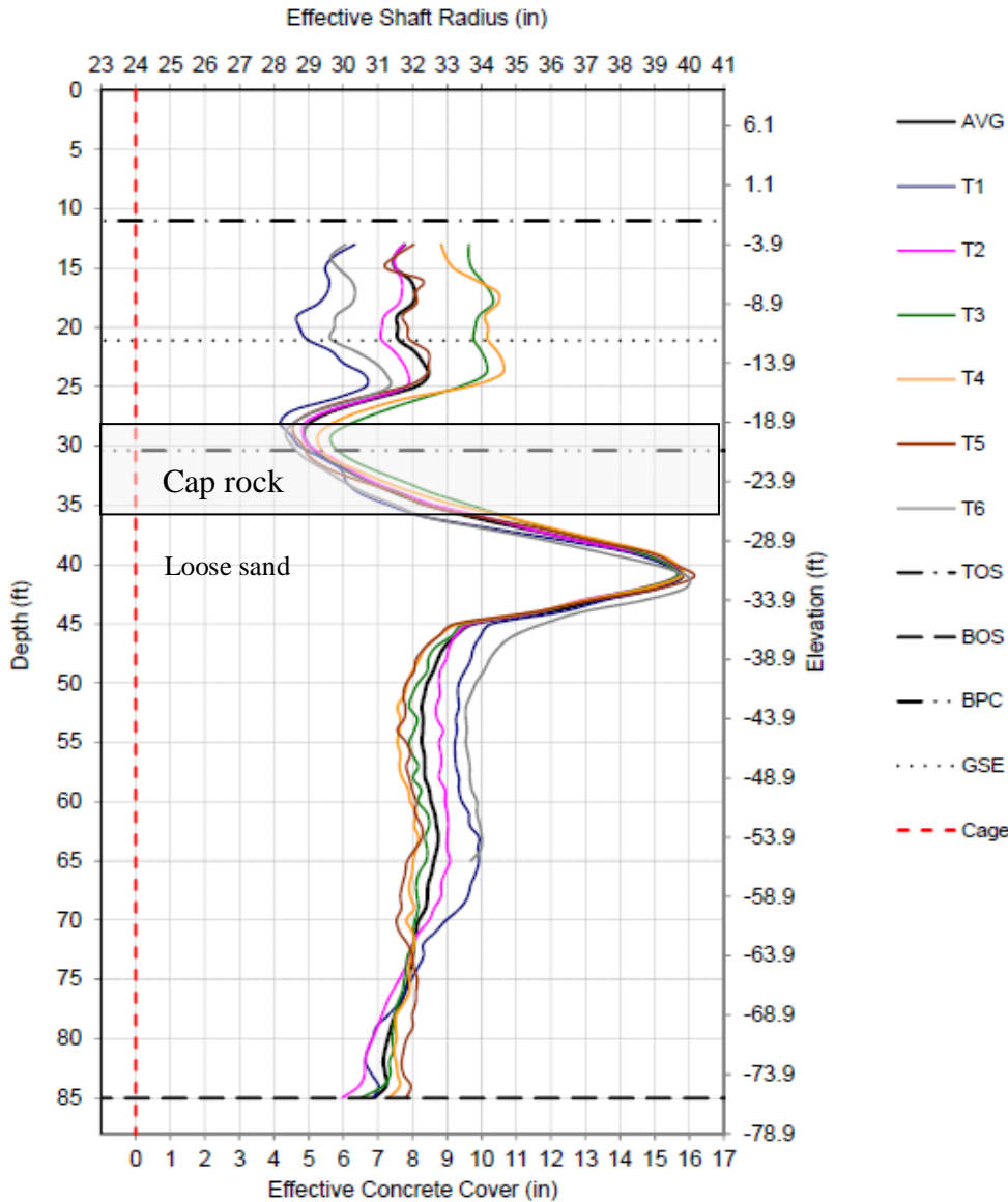
Figure 2.6 Example case where concrete / water exchange was detected by field integrity test; this a problem which can be a by-product of temporary casing.
