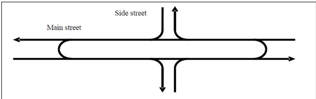
Figure 2-16: Basic RCUT intersection with no direct left turns (Hughes et al., 2010)
