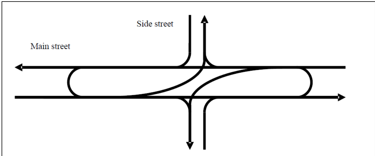
Figure 2-15: RCUT intersection configuration with direct left turns from the major road (Hughes et al., 2010)
