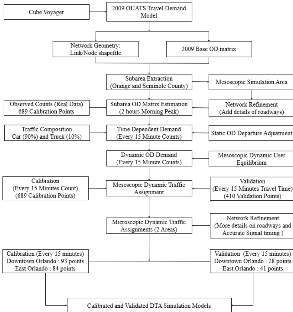
Figure 136. Modeling methods for the DTA-based simulation model.
