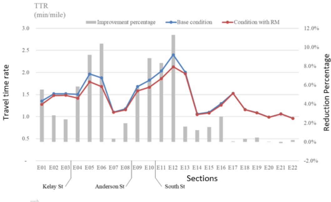
Figure 187. Improvement of travel time rate by RM according to sections
