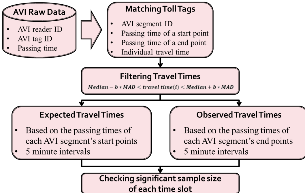
Figure 89. Flow chart of AVI data preparation
