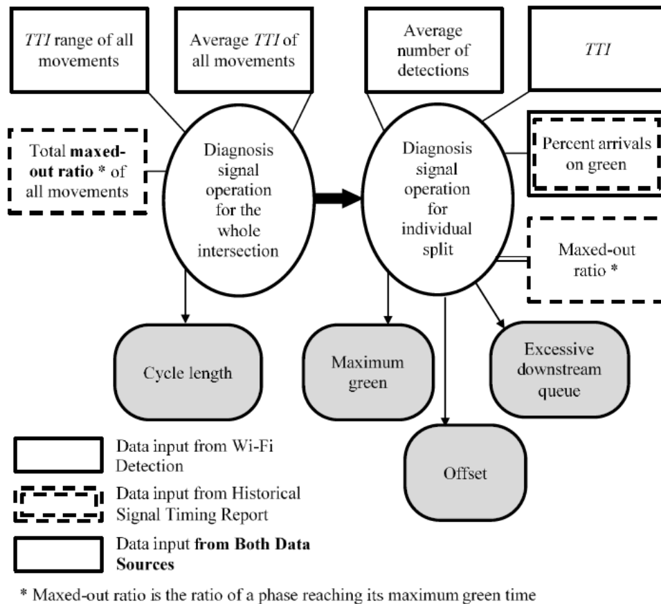
Figure 29. Proposed decision signal operation scheme
