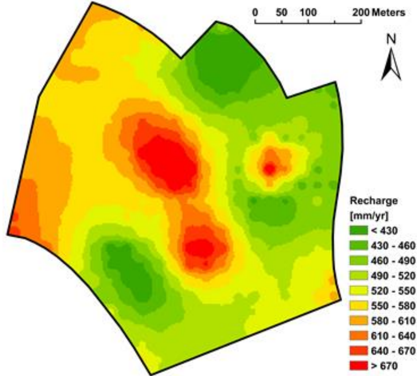
Figure 4-34. High-resolution recharge map for Site 1
