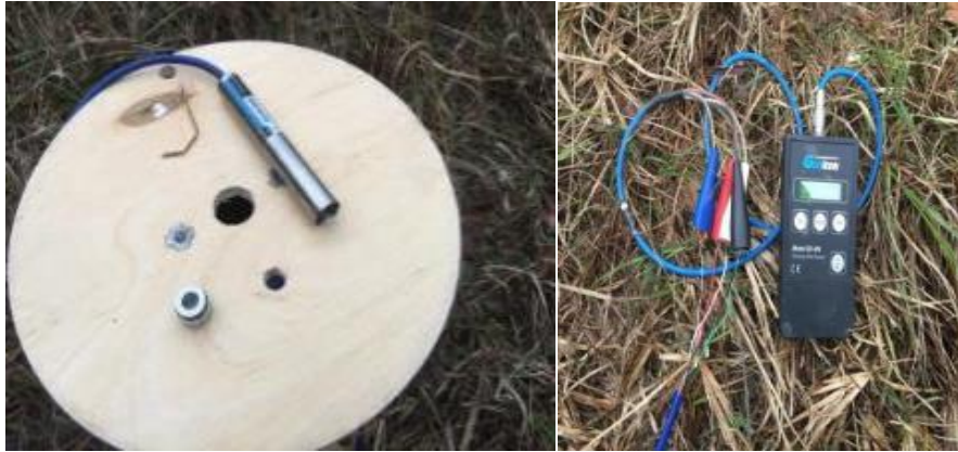
Figure 3-7. (left) Piezometer and rolled cable and (right) Geokon piezo handheld reader
