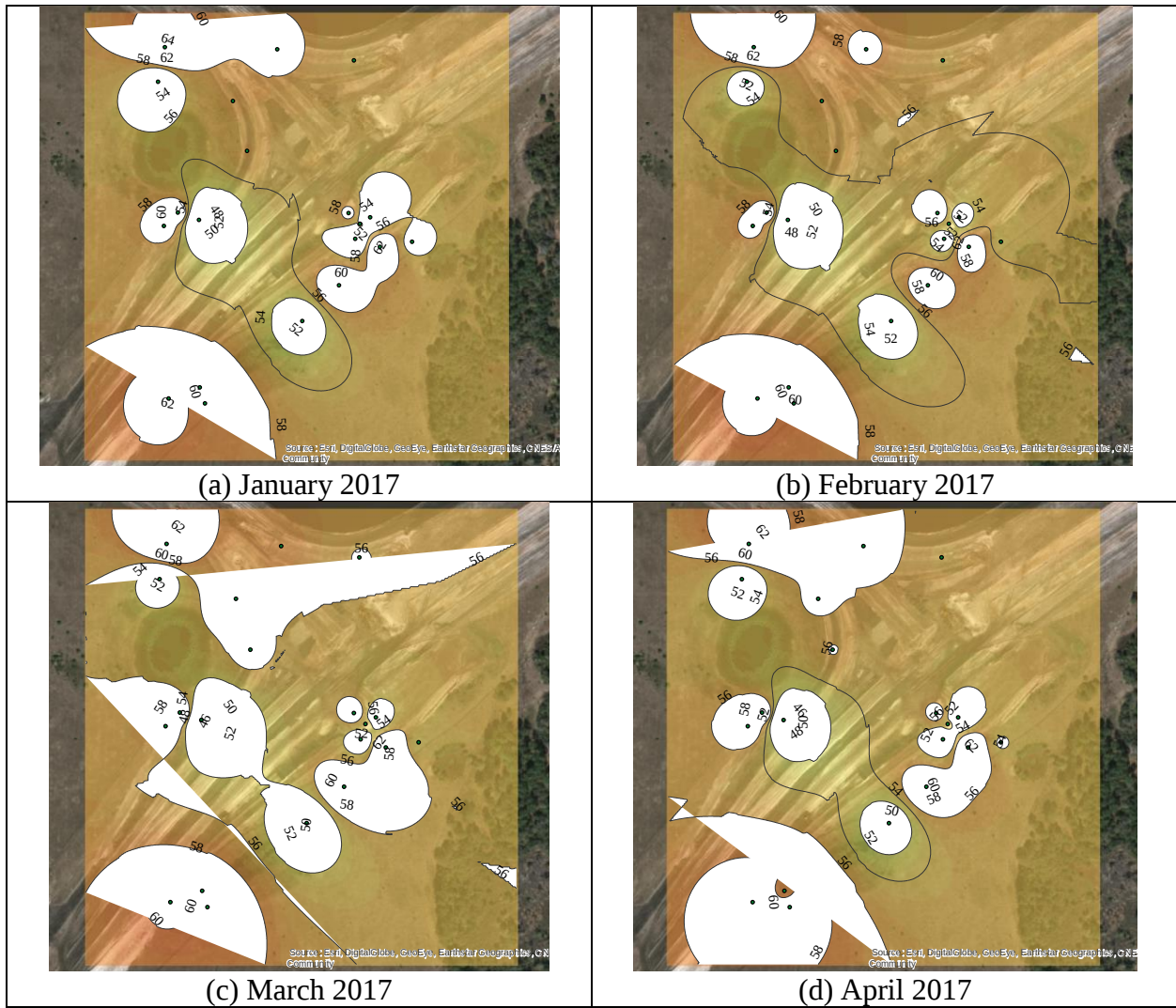
Figure A-1: Groundwater table contour of Wekiva Parkway site (January through April)
