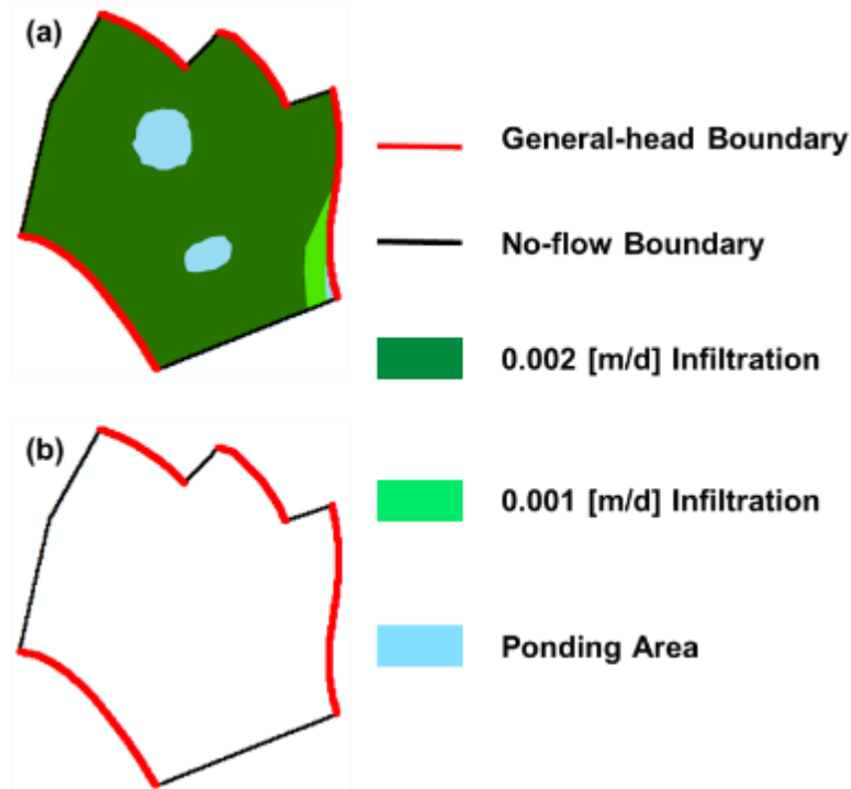
Figure 4-9. Boundary conditions applied to (a) Layer 1 and (b) Layer 2
