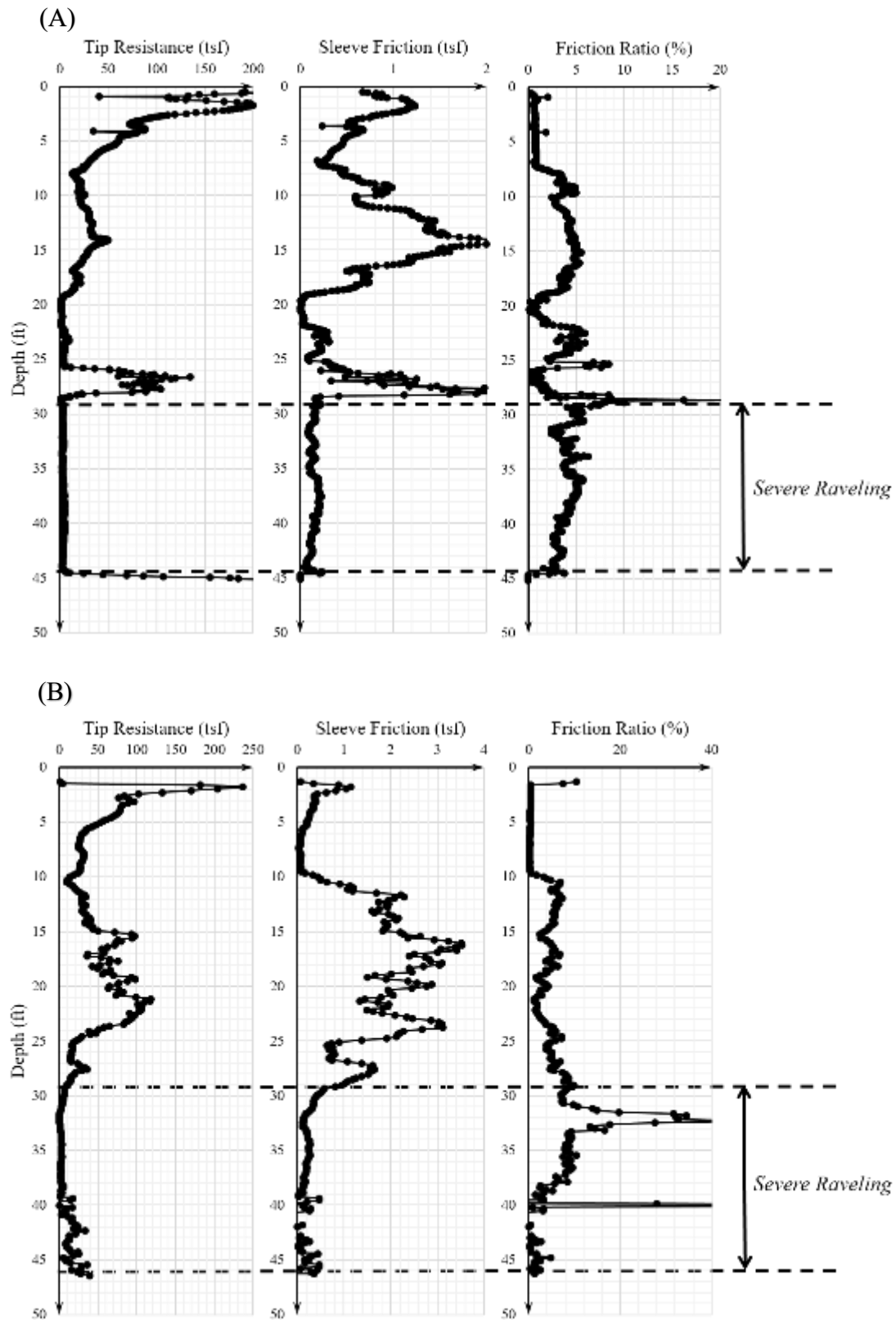
Figure 6-29. CPT resistance profiles at US-441 for (a) CPT-7 and (b) CPT-9 (in Figure 6-9)
