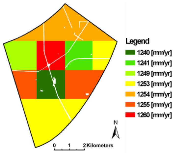
Figure 4-20. Evapotranspiration boundary map for Site 2
