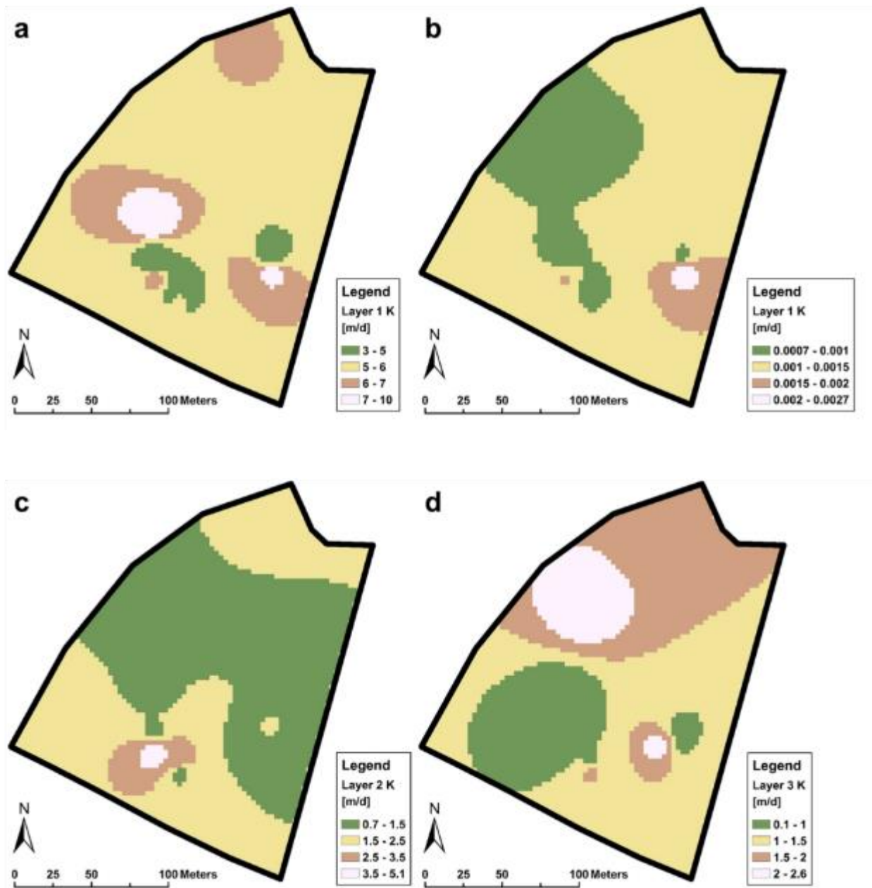
Figure 4-32. Calibrated hydraulic conductivities for Layer 1 (a) K_h and (b) K_v , Layer 2 (c), and Layer 3 (d)
