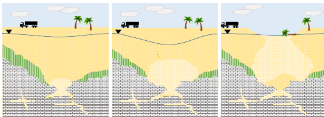
(a) Cover collapse sinkhole progression
