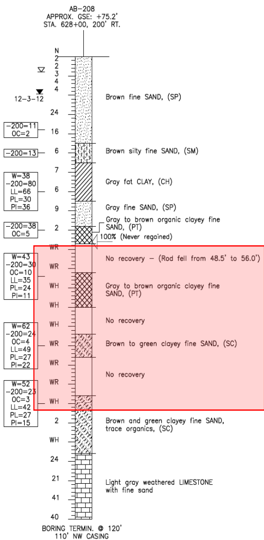
(b) Typical soil boring log suggesting raveled soil encountered
