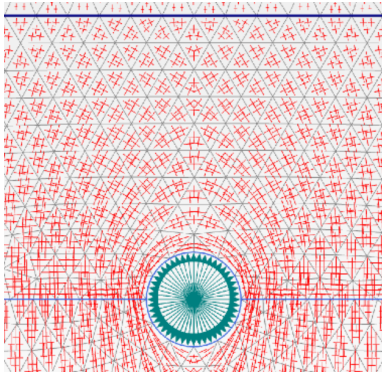
Figure 6-23. Tensor display of principal stress directions around the cavity - US-441
