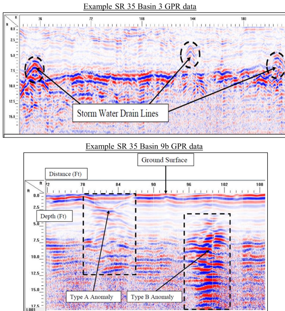
Figure 10: GPR data comparison of SR 35 Basin 3 (top) and SR 35 Basin 9b (bottom)
