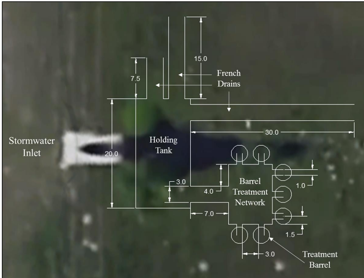
Figure 22: Plan view of potential French drains and barrel treatment network in parallel at SR 35 Basin 2. All dimensions are in feet and only for preliminary sizing.
