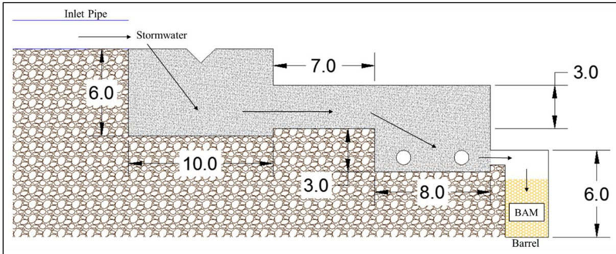
Figure 21: Section view of a potential barrel treatment network (dimensions in feet)
