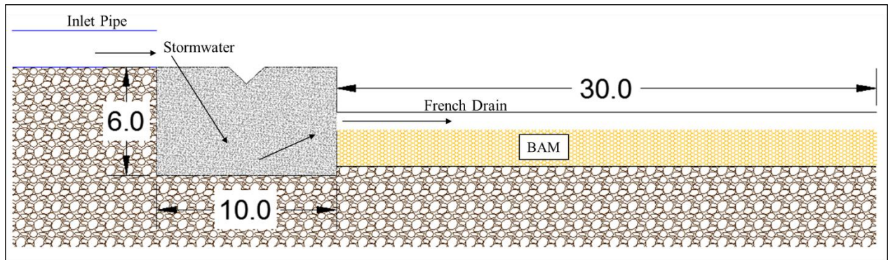
Figure 20: Section view of a potential French drain system (dimensions in feet)
