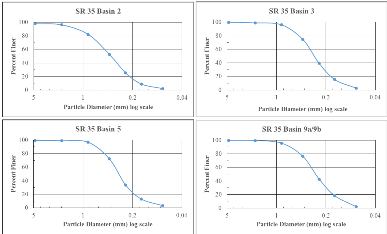
Figure 7: Sieve analysis results
