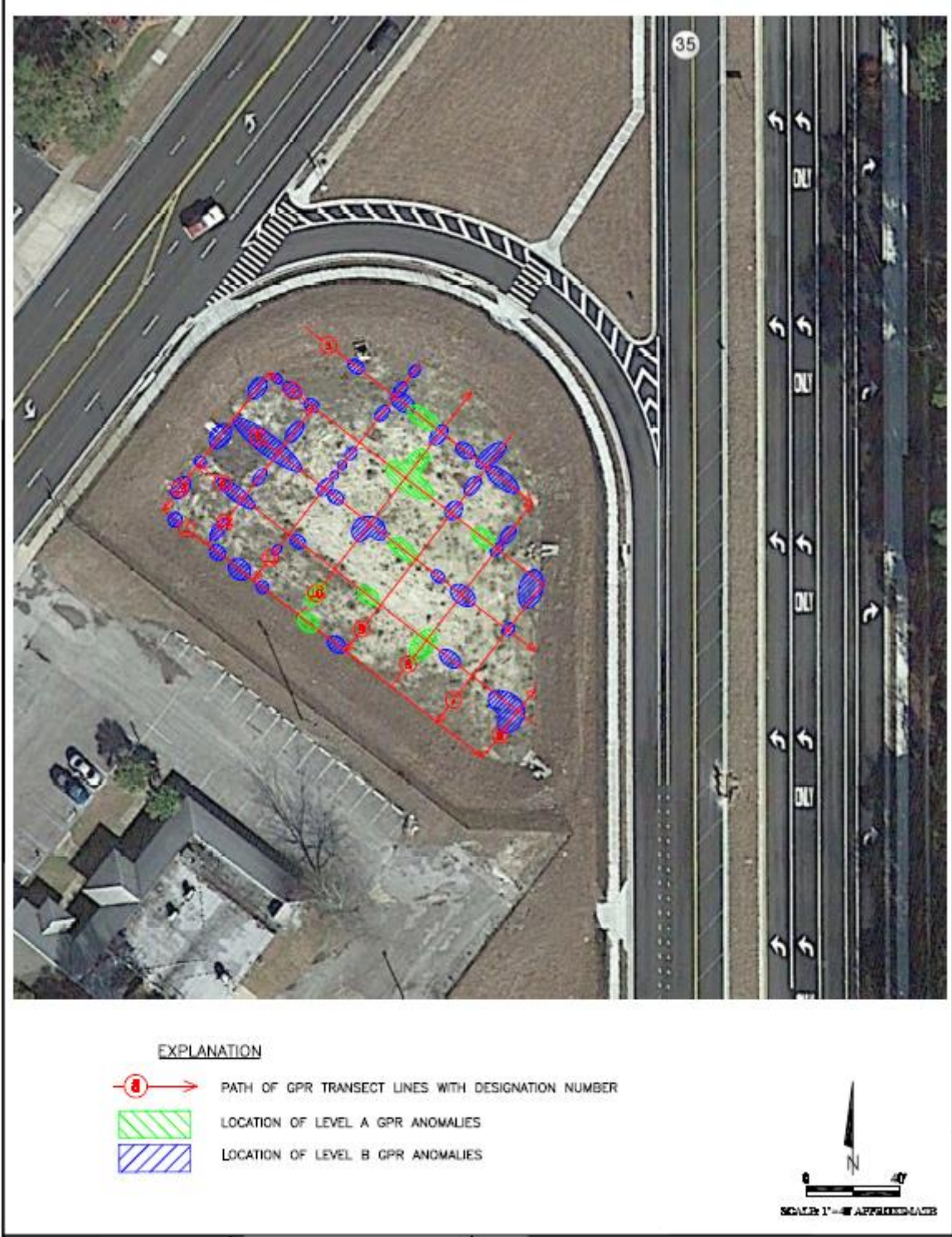
Figure 33: GPR anomalies of SR 35 Basin 9b
