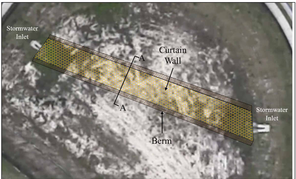
Figure 18: Plan view of a horizontal curtain wall in Basin 9b (dimensions in feet)
