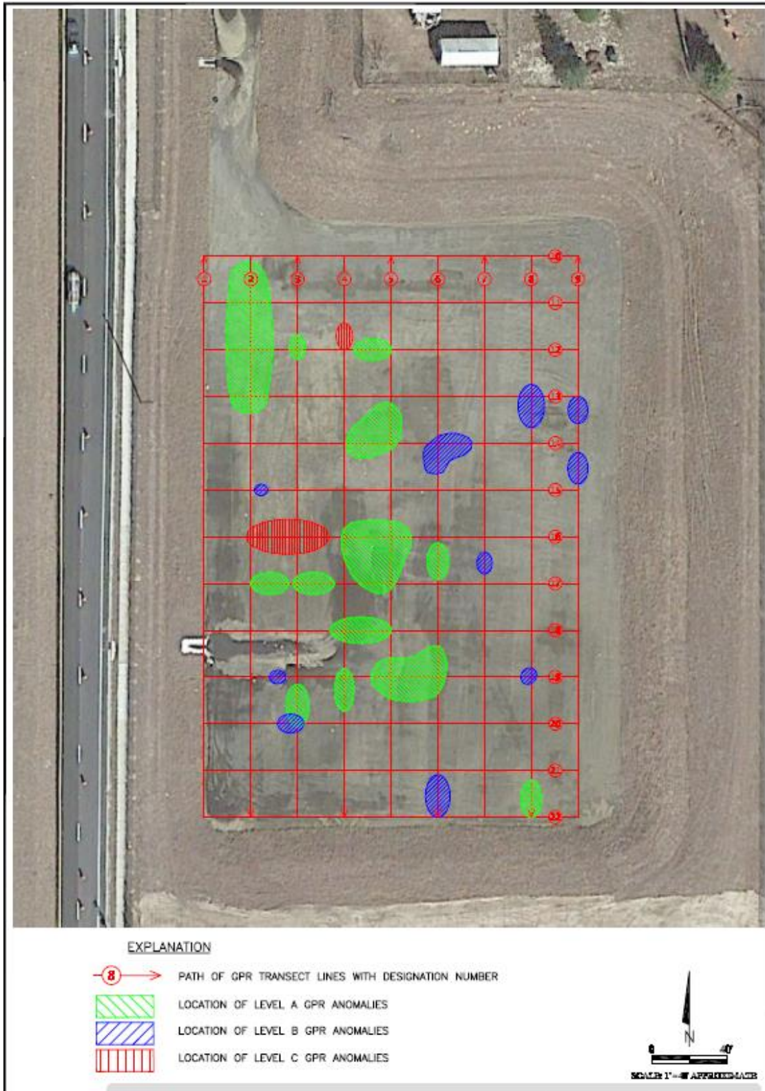
Figure 30: GPR anomalies of SR 35 Basin 2
