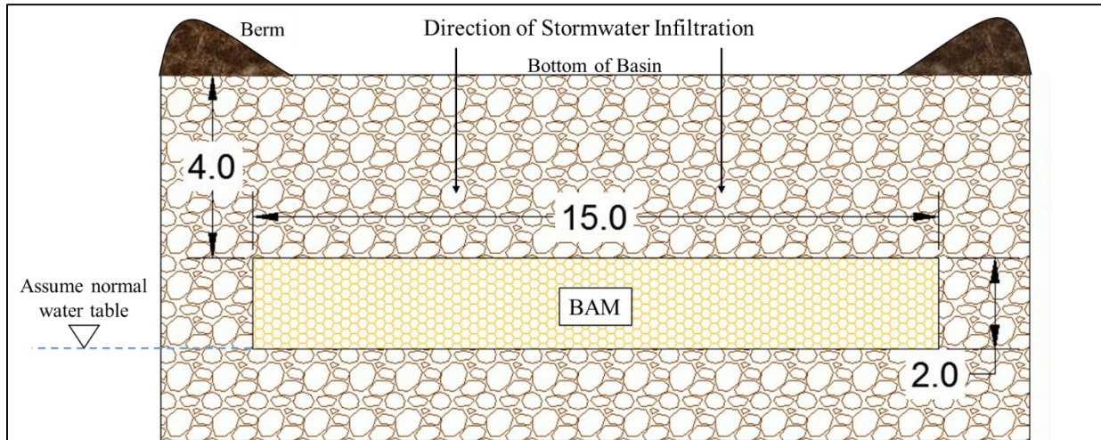
Figure 19: Section (A-A) view of a horizontal curtain wall in Basin 9b (dimensions in feet)
