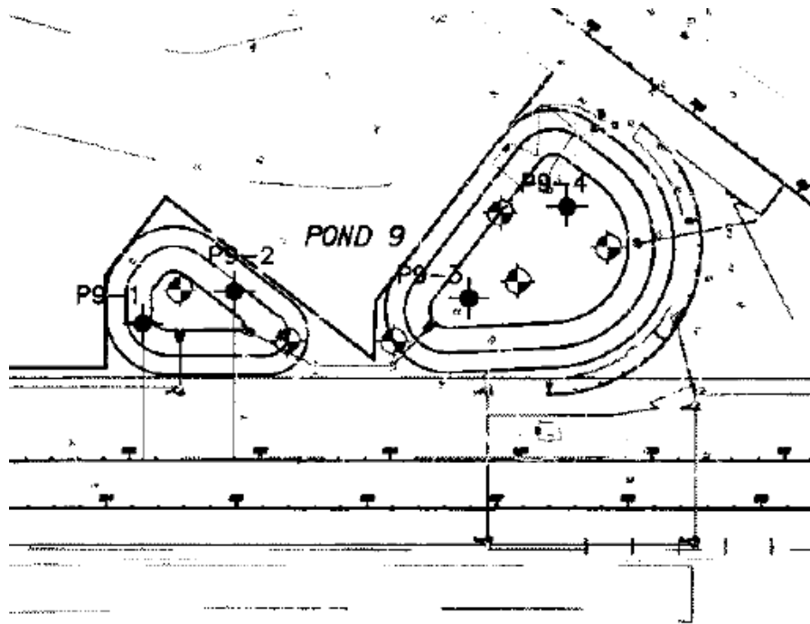
Figure 29: SR 35 Basin 9a (left) and 9b (right)
