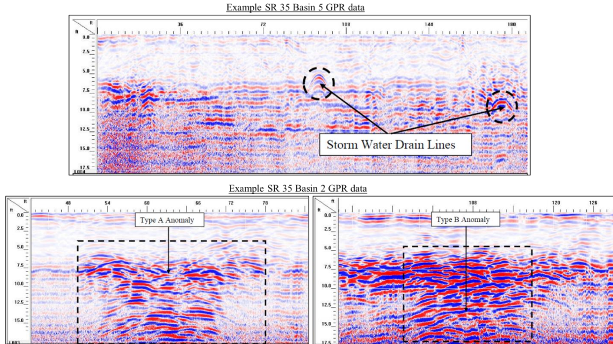
Figure 11: GPR data comparison of SR 35 Basin 5 (top) and SR 35 Basin 2 (bottom)
