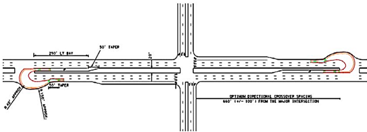
Figure 21: Loon Implementation at a MUT Intersection
