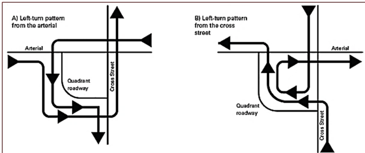
Figure 11: Movements in a QRI
