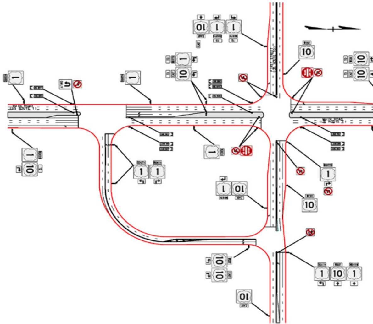
Figure 95: Typical Signing Plan for QRI
