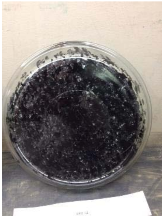
Figure 5.8 - Pie-Plate Test Results for White Rock Quarries FC-5 Mix at 0.6% Above Optimum Asphalt Content; a) PG 67-22; b) PG 76-22; c) ARB-12
