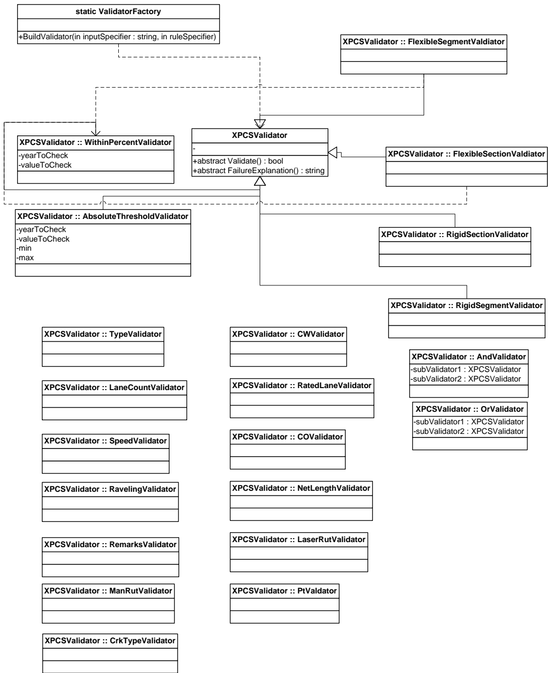
Figure C5. Validation model objects
