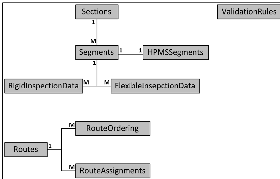
Figure 3. Business Tables
