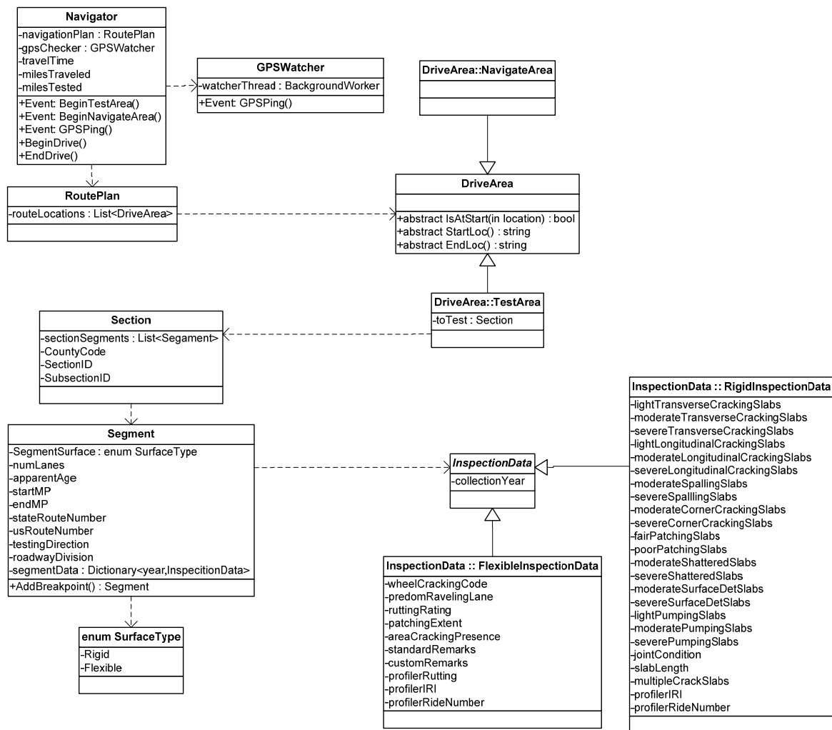
Figure C2. XPCSData module objects
