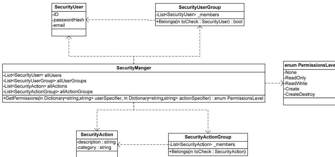
Figure D4. Security manager objects
