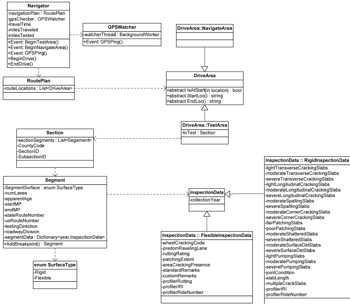
Figure D3. XPCSDData module objects
