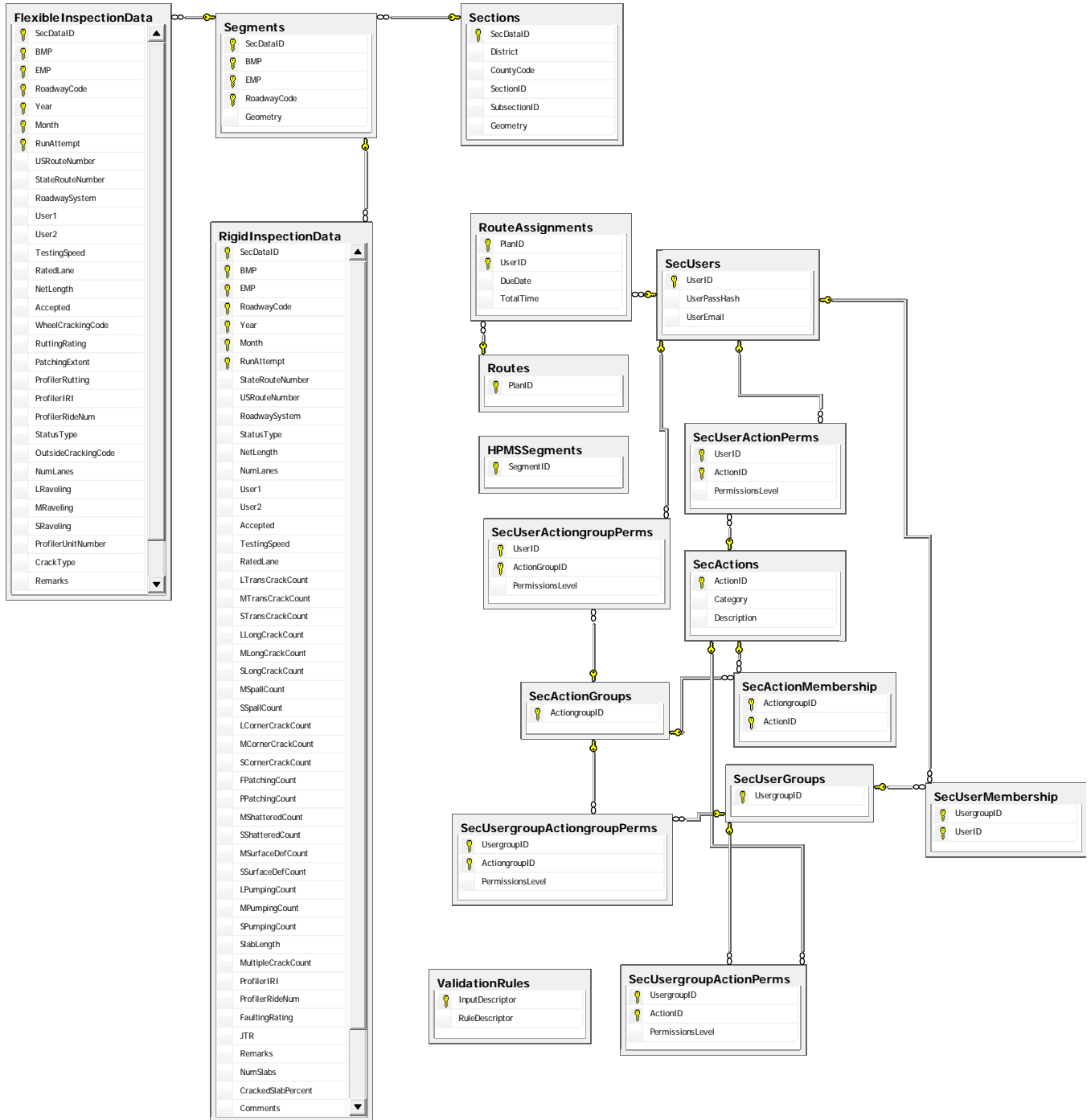
Figure C6. Overall database schema
