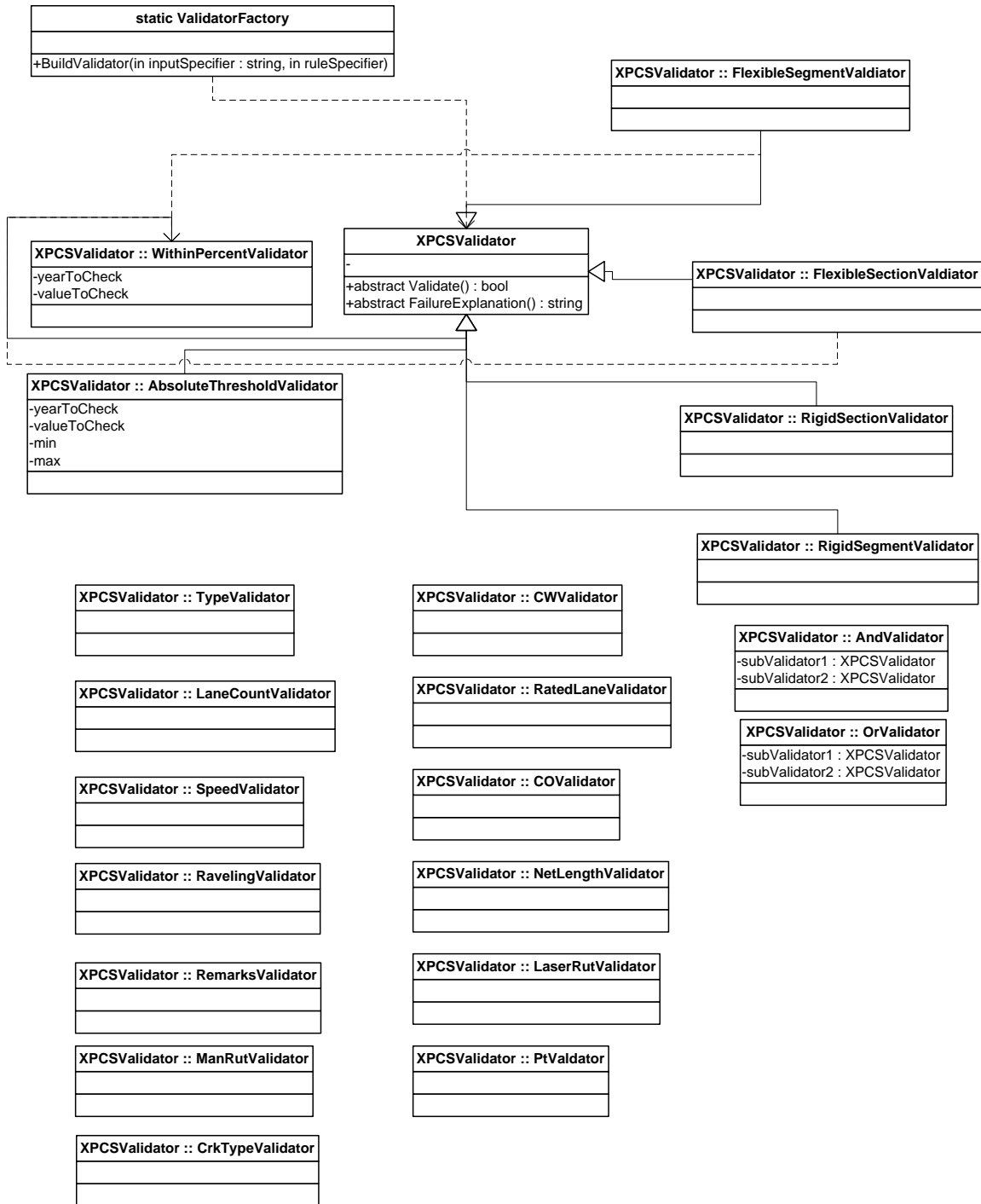
Figure D6. Validation module objects
