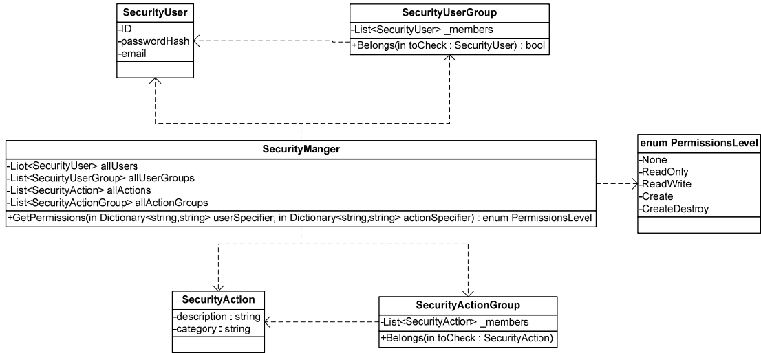
Figure C3. SecurityManager objects
