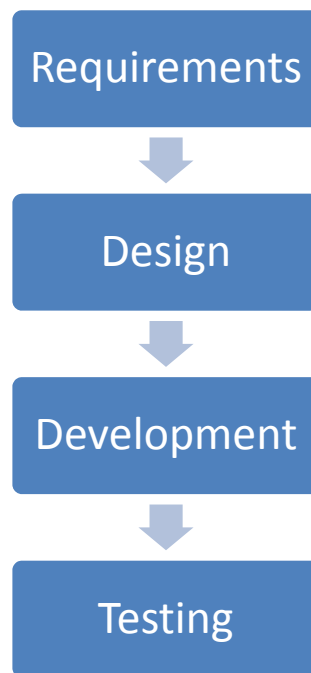
Figure 1. Project Approach
