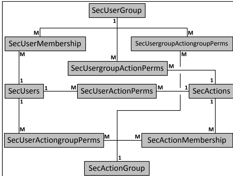
Figure 4. Security Tables
