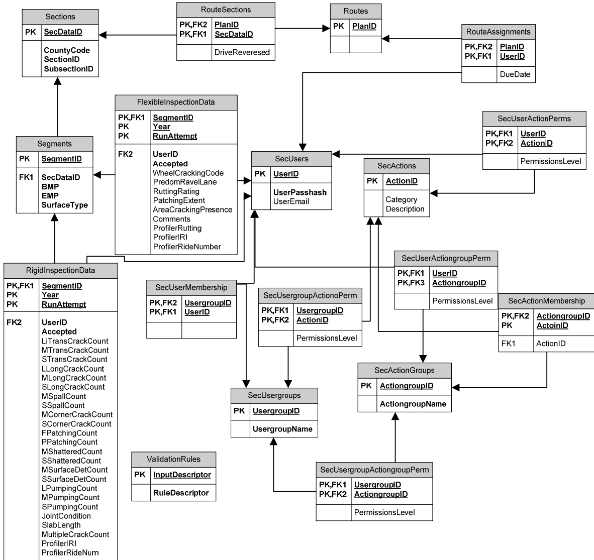
Figure D7. Overall database schema
