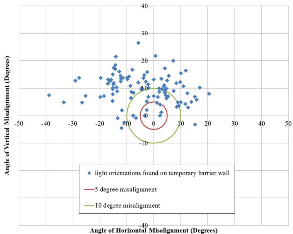
Figure 3-17. Methodology for Estimating Skew of Warning Lights on Barrier Wall.
