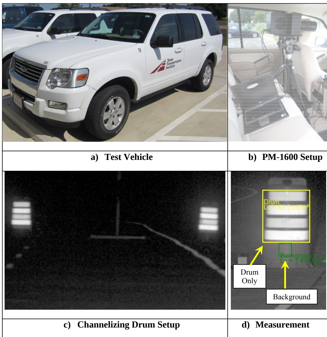
Figure 3-6. Dew Test Measurement Setup.
