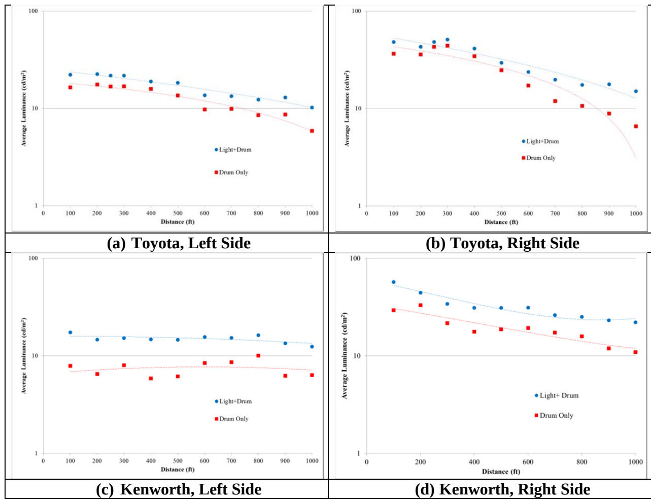
Figure 3-11. Average Luminance Values by Vehicle Type, Drum Placement, and Distance.
