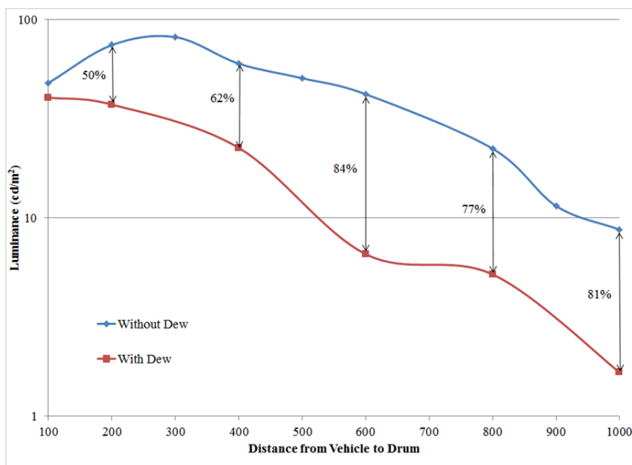
Figure 3-8. With Dew versus without Dew.
