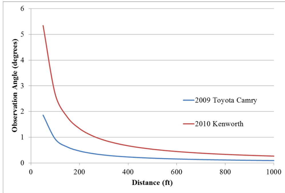
Figure 3-9. Observation Angle by Vehicle Type.
