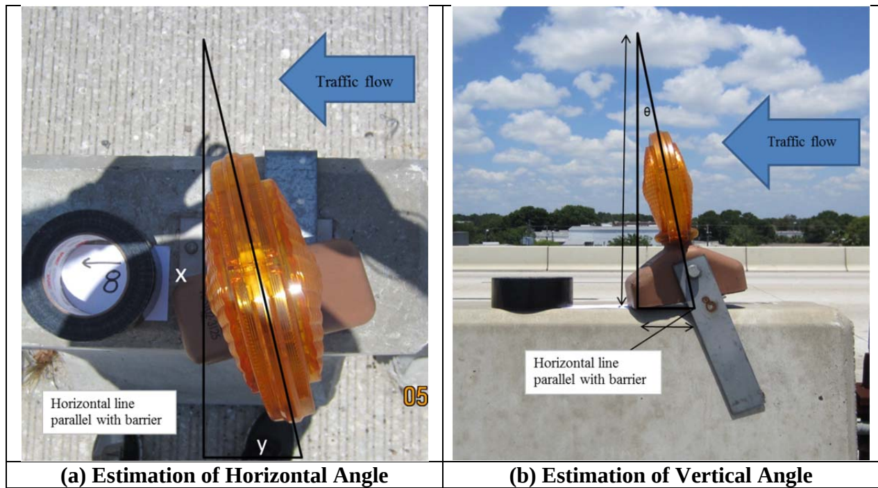
Figure 3-17. Methodology for Estimating Skew of Warning Lights on Barrier Wall.
