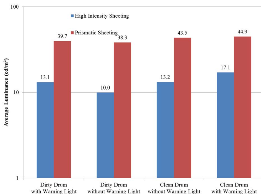
Figure 3-13. Average Luminance Results from Field Studies.
