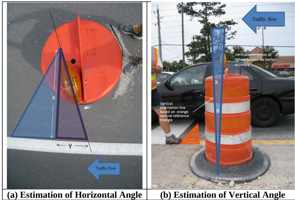
Figure 3-14. Methodology for Estimating Skew of Warning Lights on Drums.
