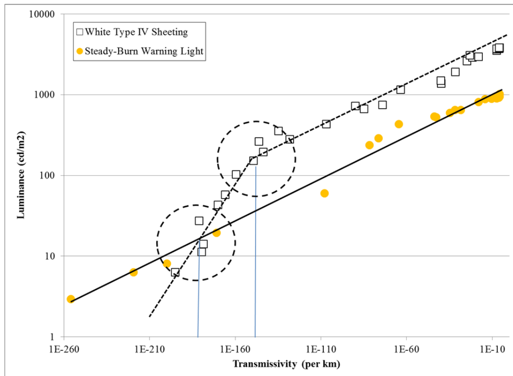
Figure 3-5. Device Luminance versus Fog Visibility Level.
