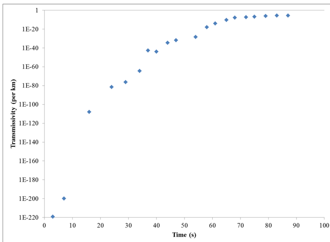
Figure 3-4. Dissipation of Transmissivity Levels Achieved in the VRL Fog Channel.
