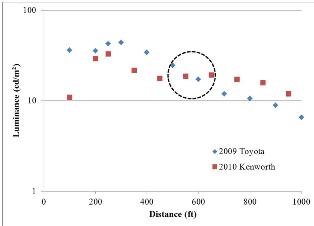
Figure 3-12. Average Luminance of Right Side Drum without Warning Light.
