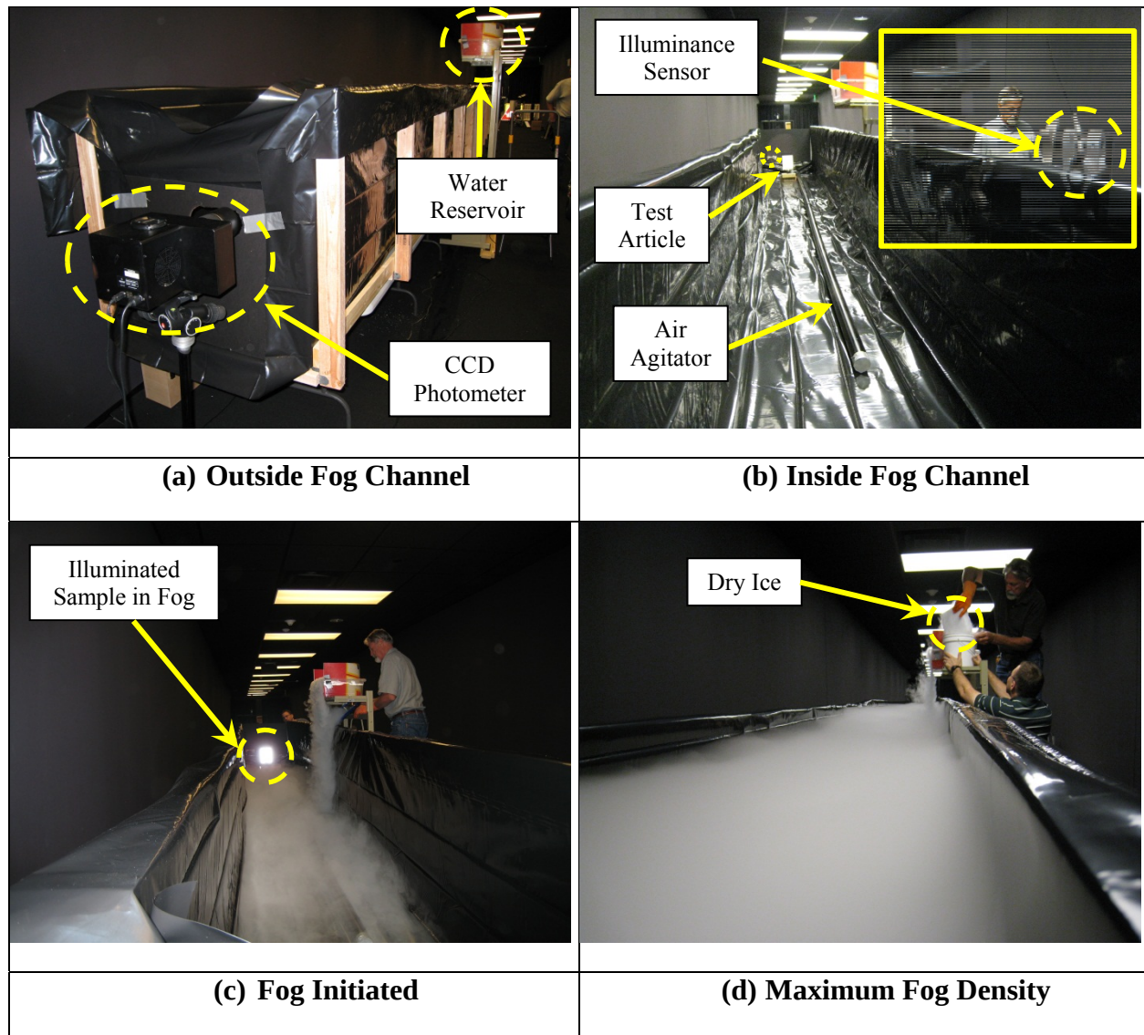
Figure 3-3. Fog Channel in TTI Visibility Research Laboratory (VRL).
