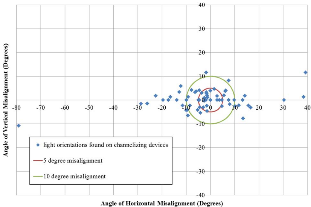
Figure 3-15. Orientations of Warning Lights on Drums from Field Study.
