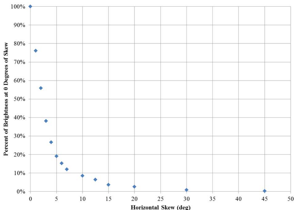
Figure 3-19. Impact of Horizontal Skew on Warning Light Brightness.
