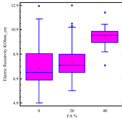
Figure 81. Box and Whisker Plot of Electric resistivity vs. Fly ash.
