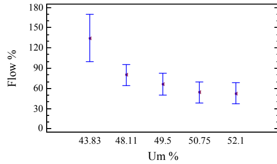
Figure 41. Means and 95 Percent LSD Intervals for Flow by Angularity Levels.
