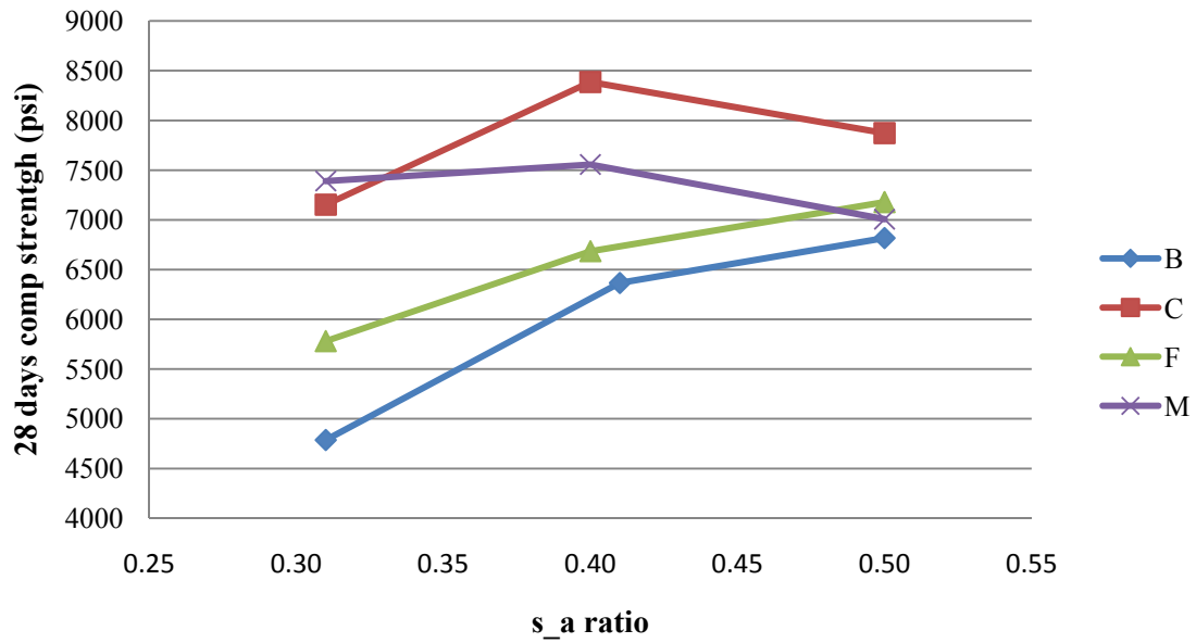
Figure 76. Influence of s_a ratio on compressive strength for w/c = .41 , c = 658 \text{ lb/yd}^3 .
