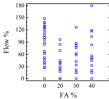
Figure 46. Scatter plot of Flow by Flyash Levels.
