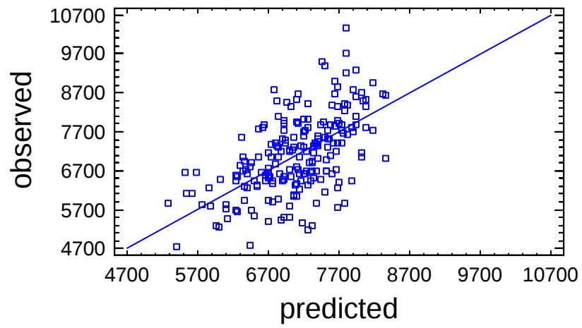
Figure 94. Plot of observed vs. Predicted Compressive Strength (psi).
