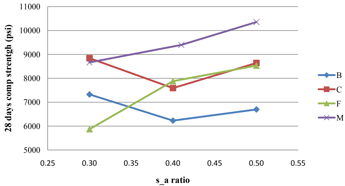
Figure 77. Influence of s_a ratio on compressive strength for w/c = .37 , c = 752 \text{ lb/yd}^3 .
