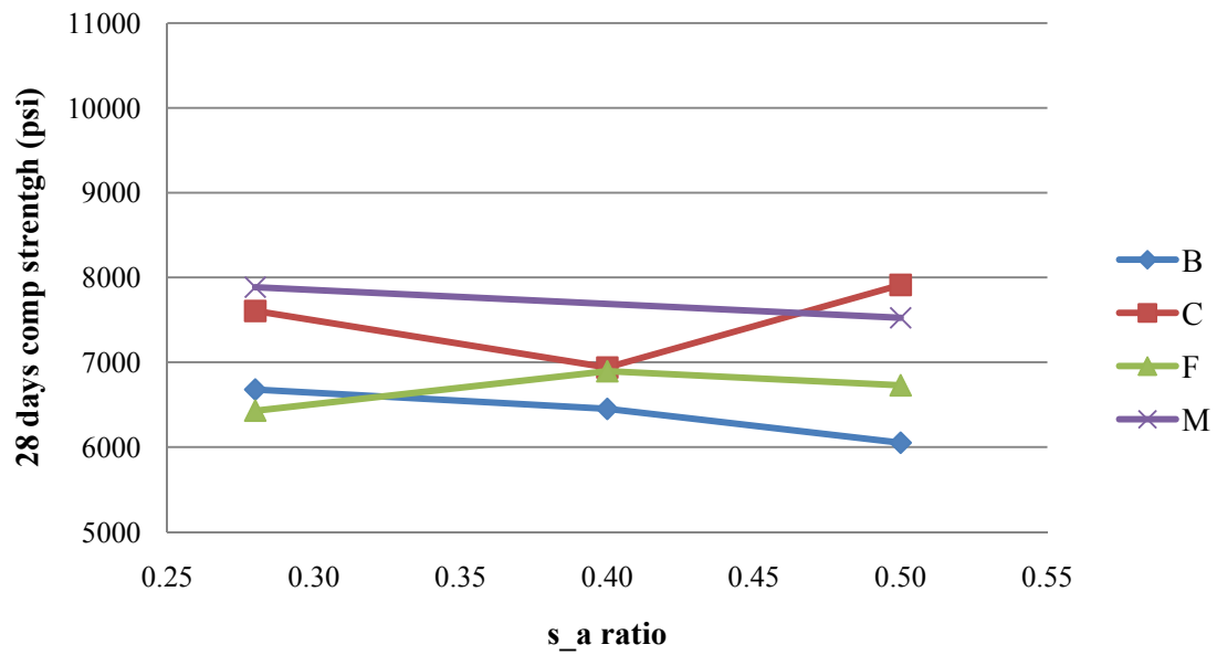
Figure 75. Influence of s_a ratio on compressive strength for w/c =.41, c=752lb/yd 3 .
