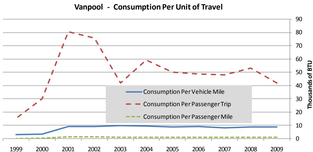
Figure 37 Volusia County Vanpool Energy Consumption Per Unit of Travel
