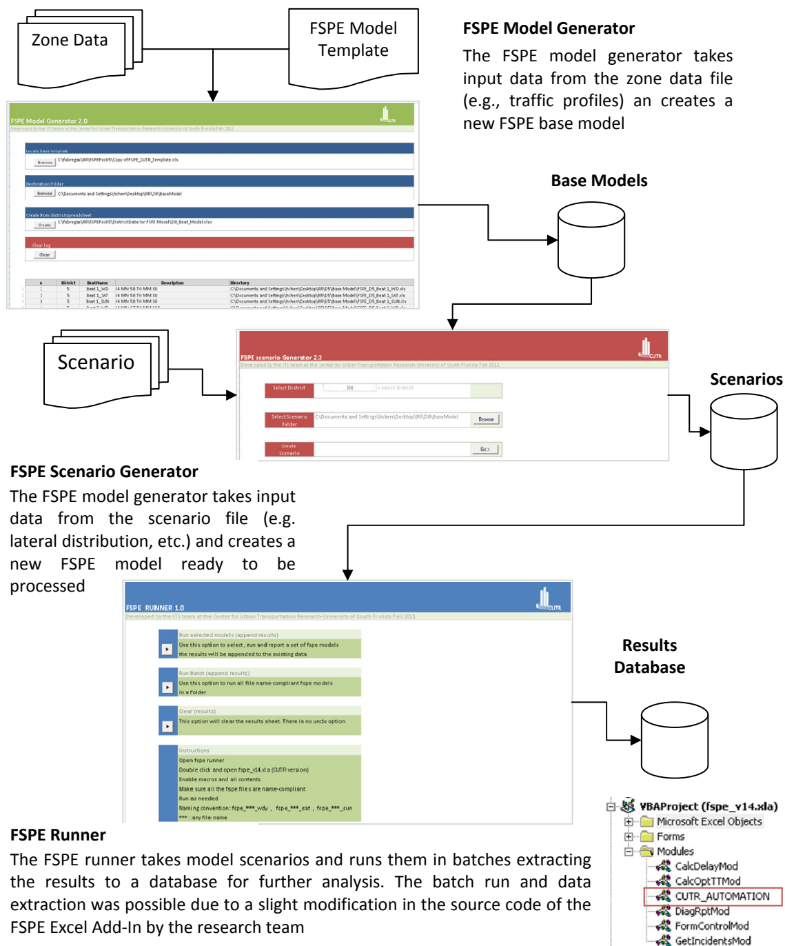
Figure 55: Modeling architecture
