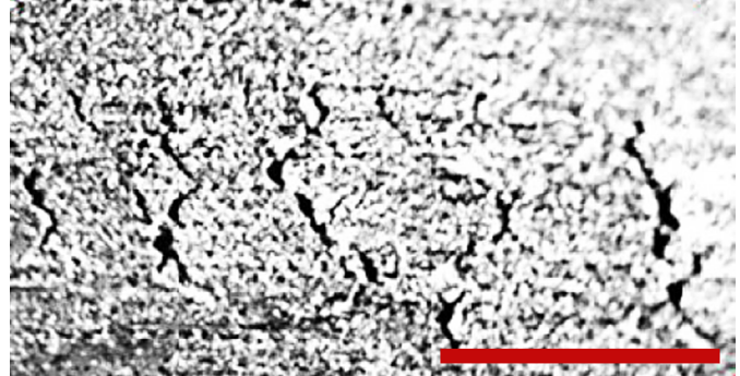
Stress applied to stainless steel can amplify the effects of corrosion, leading to the cracking shown above (bar = 1 mm).
