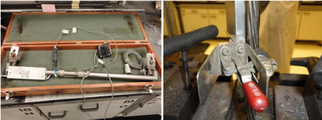
Figure 4.10 24in extensometer (left); close-up of extensometer strand clamp (right)
