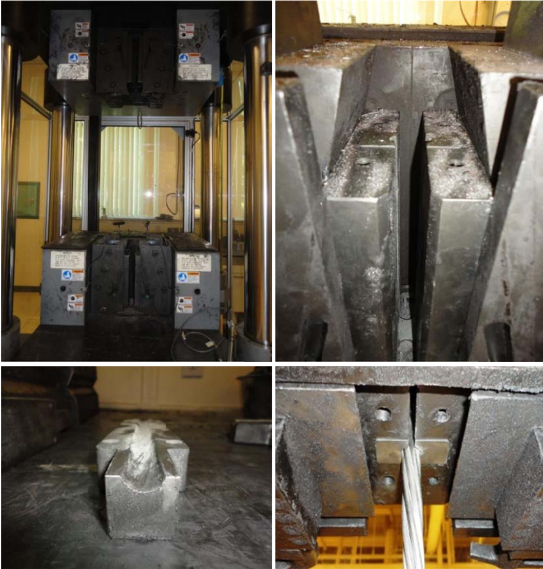
Figure 4.5 Universal Testing System (top left); testing jaws (top rt); tapered \frac{1}{2} in half-round insert (bot left); strand in jaws (bot rt).
