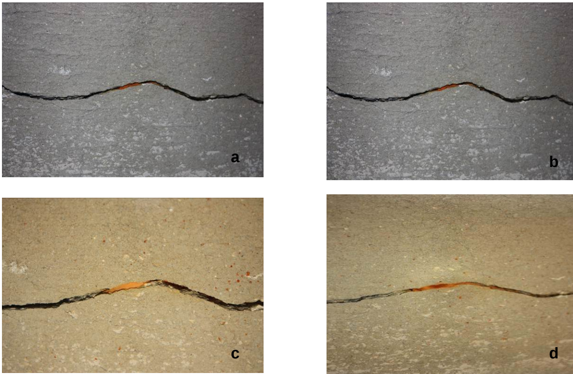
Figure (4.8) Specimen R12 with 0.100-in-wide crack showing a corrosion spot at an intersection of the steel wire with the crack (indicated by the arrow) (14 days after the ponding solution started to incorporate chloride ion)
