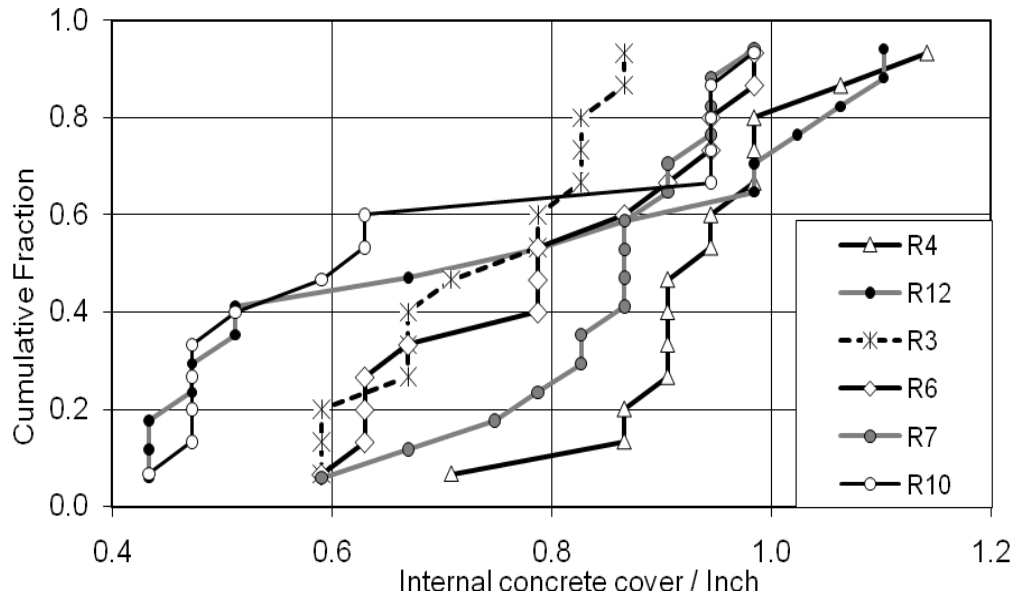
Figure (3.10) Interior concrete cover thickness for individual R-type quadrants to be used in the corrosion exposure experiment (values measured on the four edges of a specimen)
