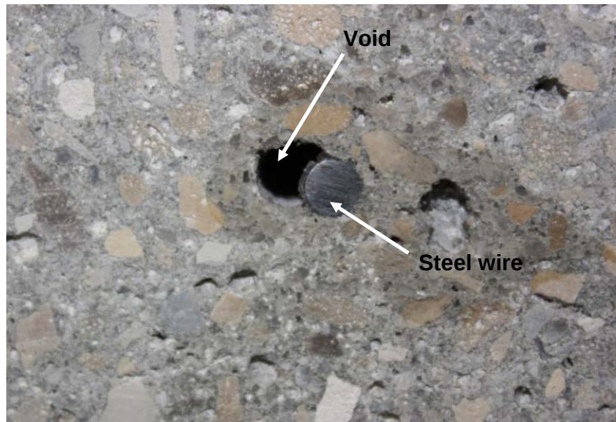
Figure (3.9) an example of a Z-type specimen showing consolidation voids next to circumferential wires with a magnified image showing the wire/void details
