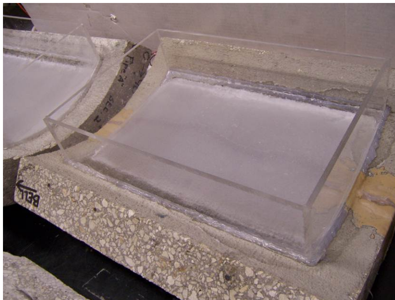
Figure (3.17) A cracked specimen during exposure to healing solution
